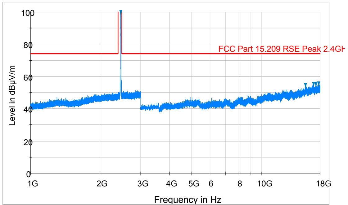
Plot 6-35. Radiated Spurious Plot above 1GHz (802.11b – Ch. 11, Ant. Pol. H)
