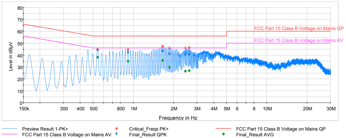
Plot 6-45. Line Conducted Plot with 802.11b (L1)
