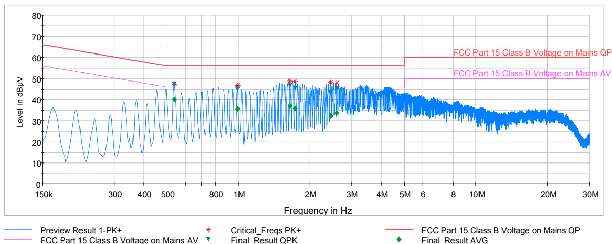
Plot 6-46. Line Conducted Plot with 802.11b (N)
