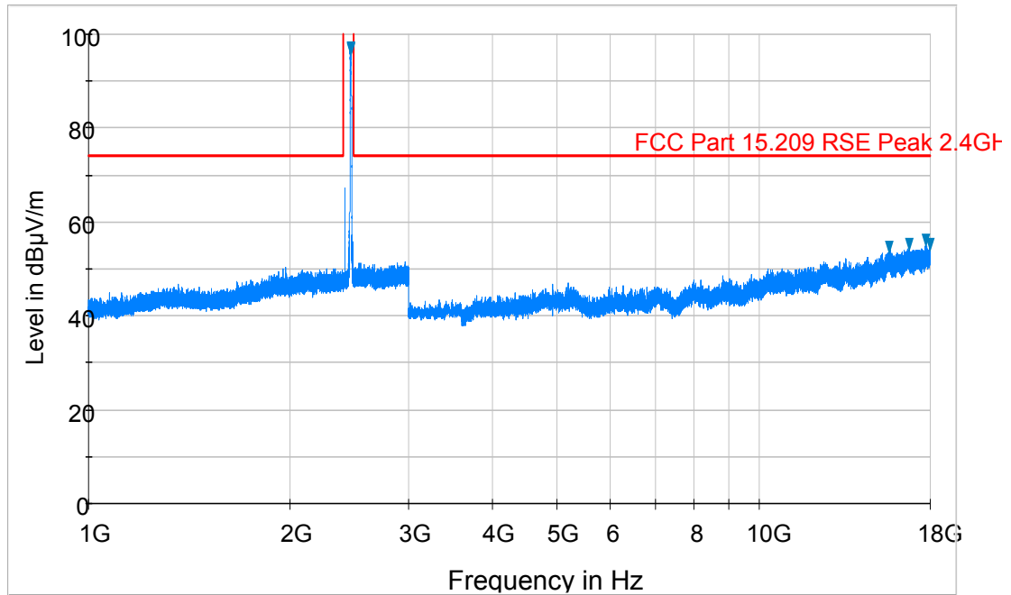
Plot 6-36. Radiated Spurious Plot above 1GHz (802.11b – Ch. 11, Ant. Pol. V)
