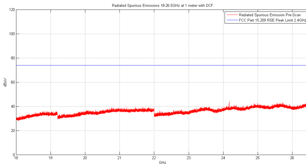
Plot 6-24. Radiated Spurious Plot above 18GHz (Pol. H)
