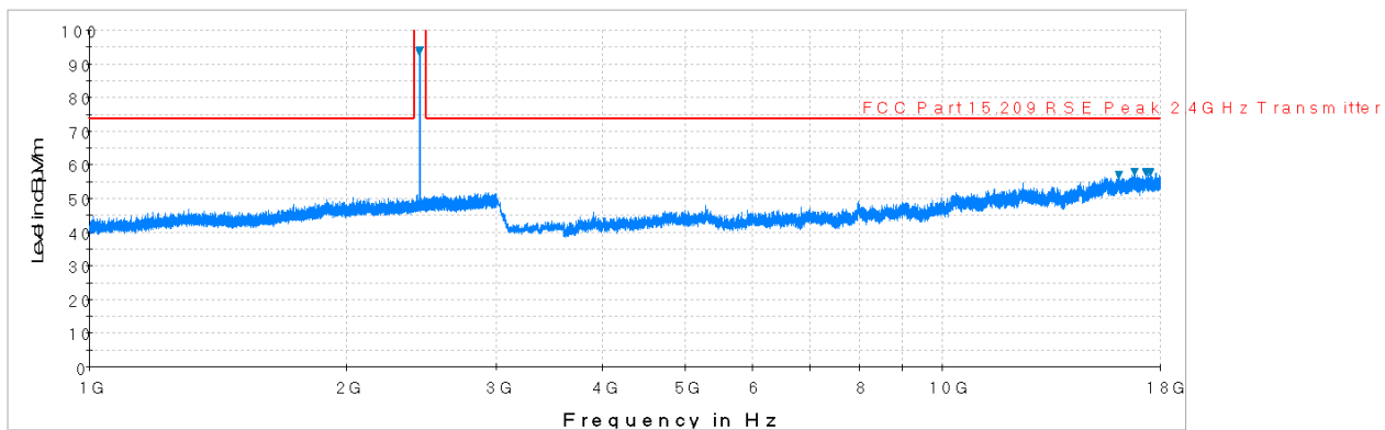
Plot 6-20. Radiated Spurious Plot above 1GHz (BTLE – Ch. 19, Ant. Pol. H)
