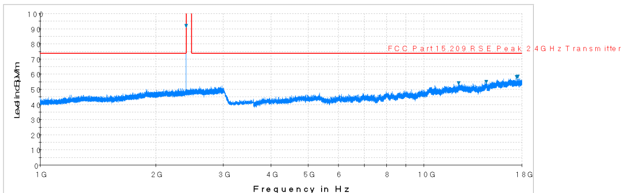
Plot 6-19. Radiated Spurious Plot above 1GHz (BTLE – Ch. 0, Ant. Pol. V)
