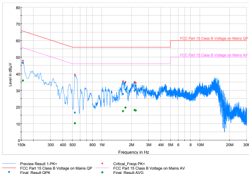
Plot 6-30. Line Conducted Plot with Bluetooth LE (L1)
