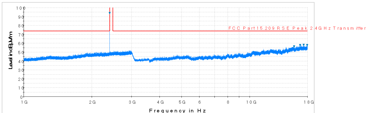
Plot 6-18. Radiated Spurious Plot above 1GHz (BTLE – Ch. 0, Ant. Pol. H)
