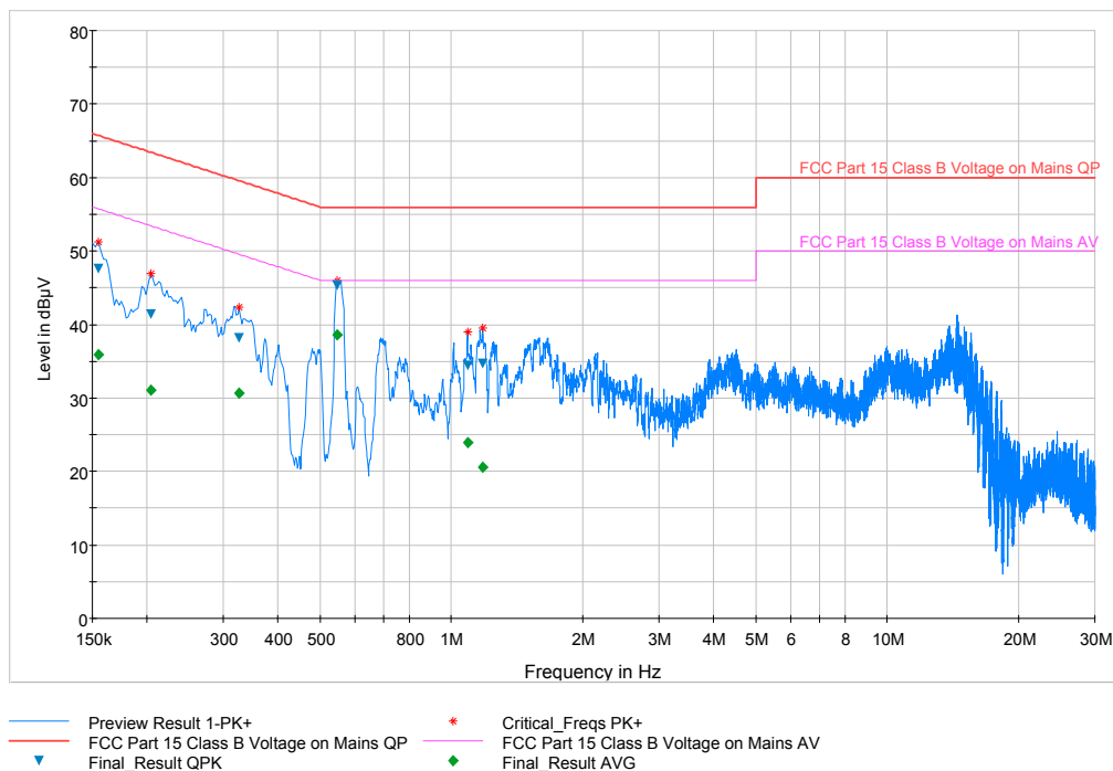
Plot 6-31. Line Conducted Plot with Bluetooth LE (N)
