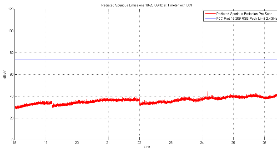
Plot 6-25. Radiated Spurious Plot above 18GHz (Pol. V)
