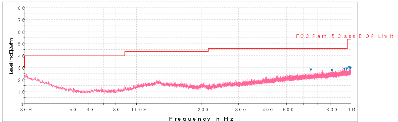
Plot 6-28. Radiated Spurious Plot below 1GHz (Pol. H)
