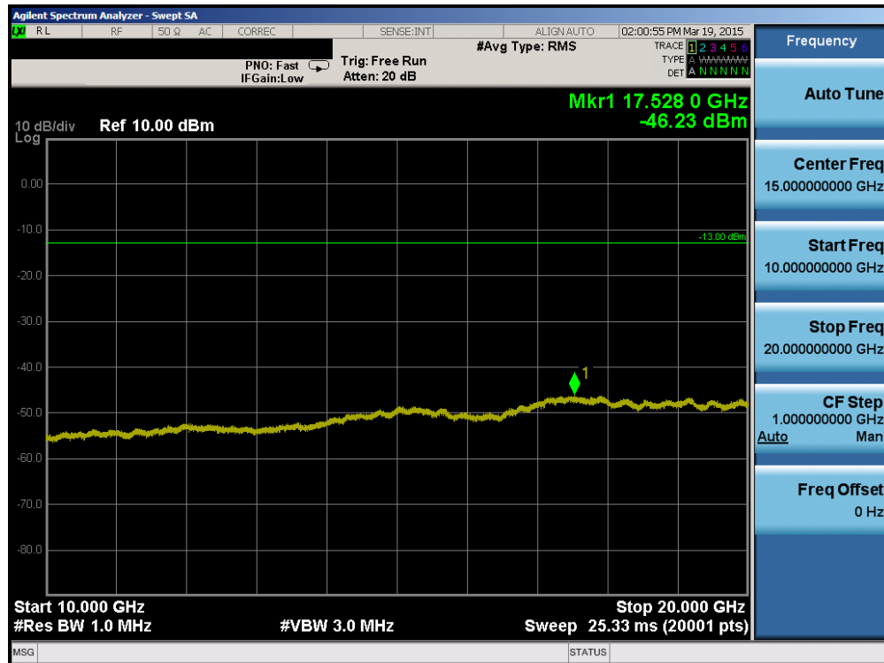
Plot 6-21. Conducted Spurious Plot (AWS WCDMA Mode – Ch. 1862)
