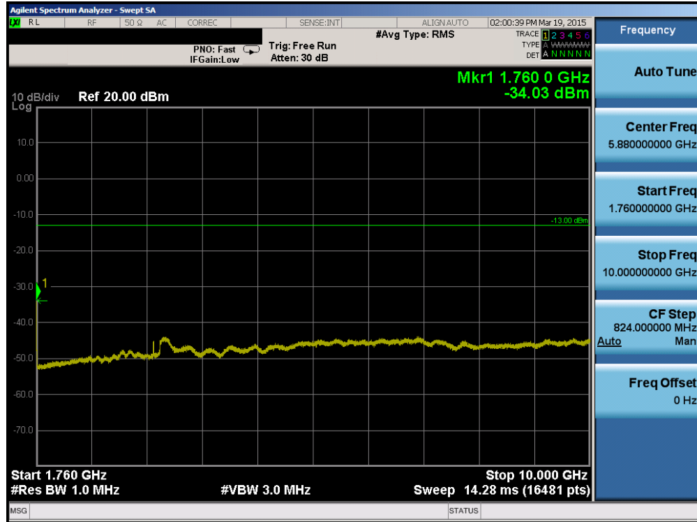
Plot 6-20. Conducted Spurious Plot (AWS WCDMA Mode – Ch. 1862)
