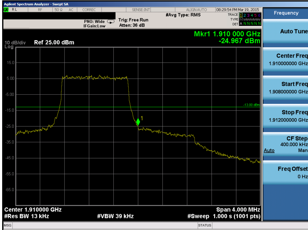
Plot 6-102. Upper Band Edge Plot (Band 2 – 1.4MHz QPSK – RB Size 6)
