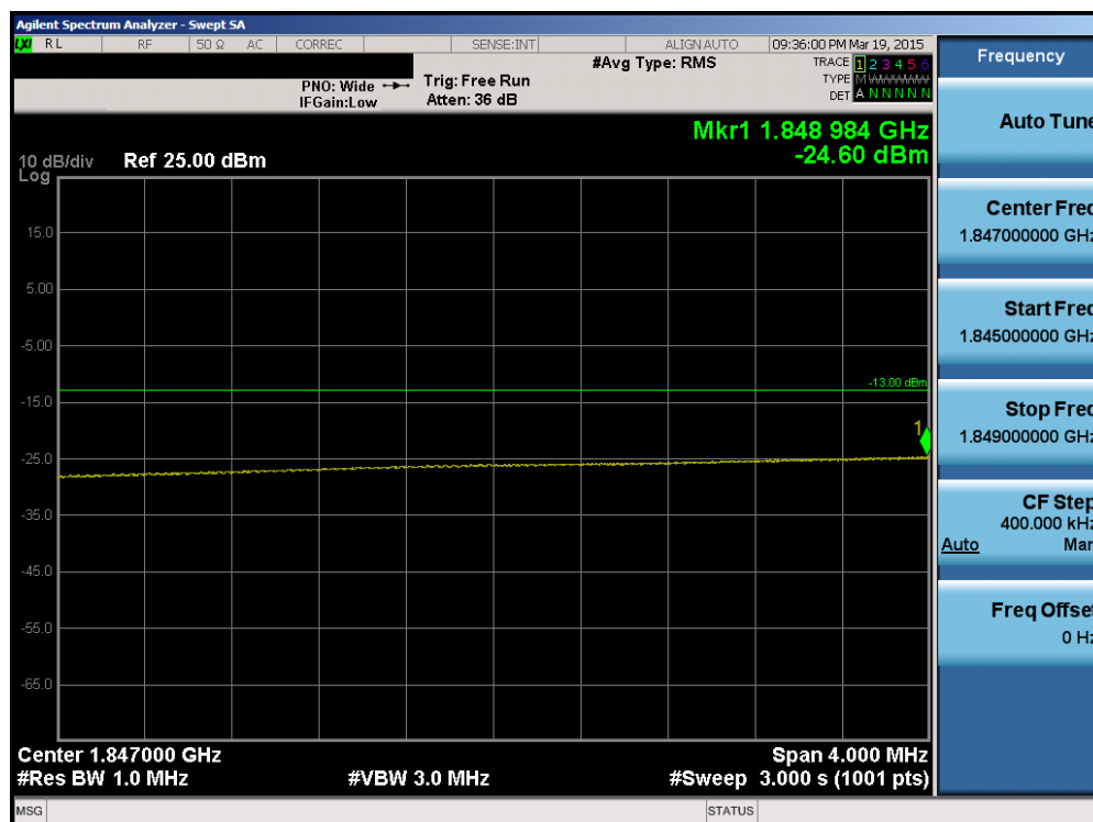
Plot 6-121. Lower Extended Band Edge Plot (Band 2 – 20.0MHz QPSK – RB Size 100)
