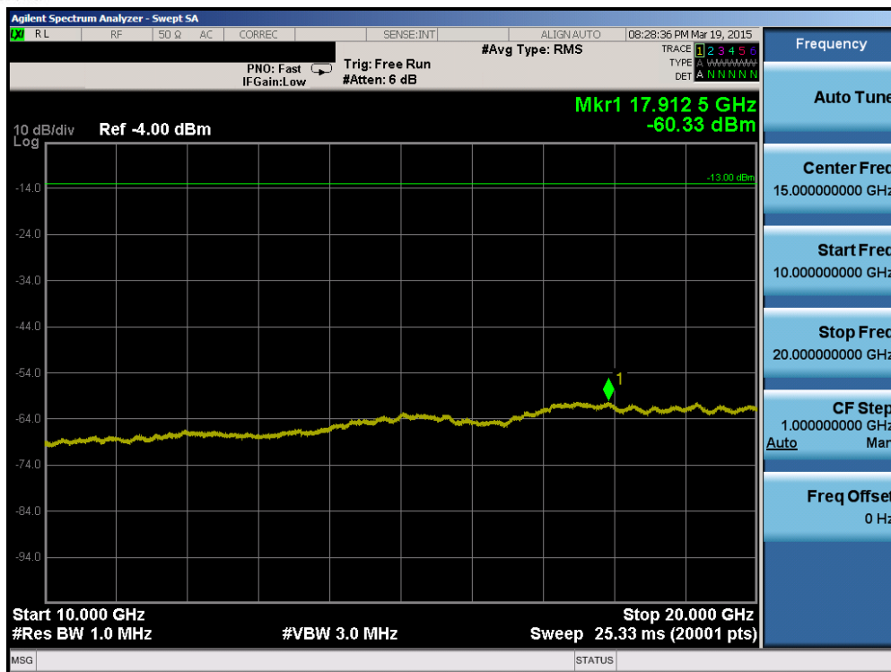
Plot 6-59. Conducted Spurious Plot (Band 2 – 1.4MHz QPSK – RB Size 1, RB Offset 0 – High Channel)
