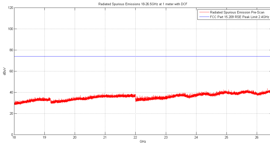
Plot 6-49. Radiated Spurious Plot above 18GHz (Pol. V)
