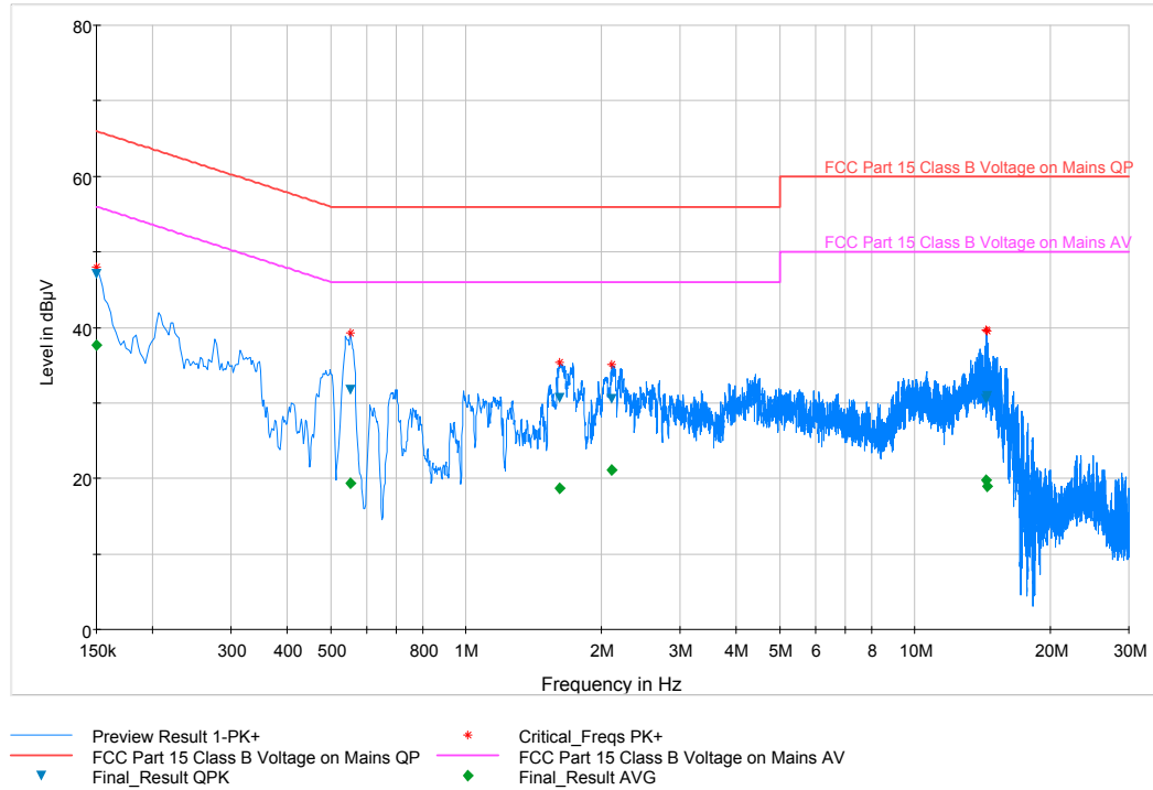
Plot 6-54. Line Conducted Plot with Bluetooth LE (L1)
