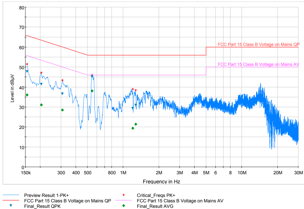
Plot 6-55. Line Conducted Plot with Bluetooth LE (N)
