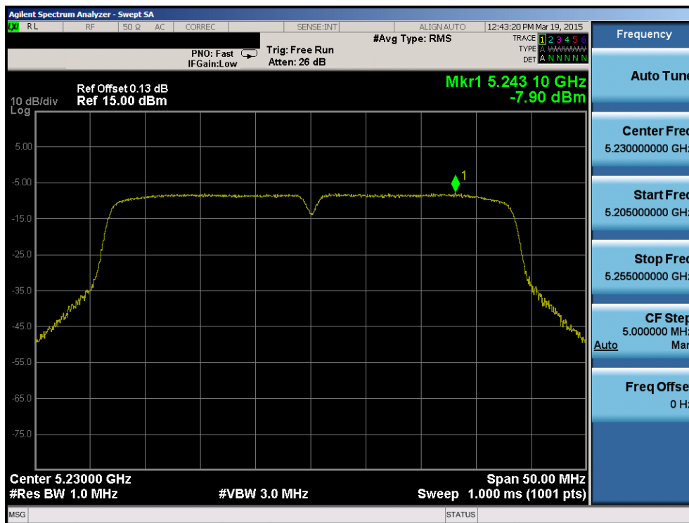
Plot 6-41. Power Spectral Density Plot (40MHz BW 802.11n (UNII Band 1) – Ch. 46)
