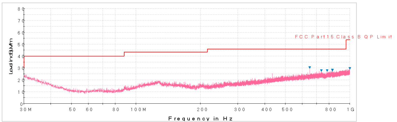
Plot 6-68. Radiated Spurious Plot below 1GHz (802.11a – U3 Ch. 157, Ant. Pol. V)
