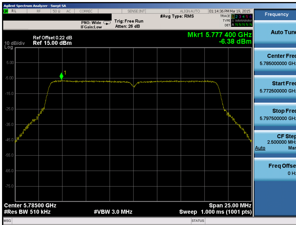
Plot 6-63. Power Spectral Density Plot (802.11n (UNII Band 3) – Ch. 157)
