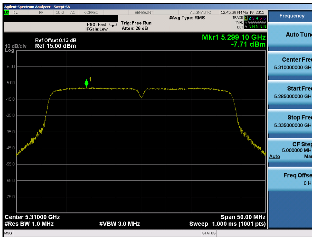
Plot 6-49. Power Spectral Density Plot (40MHz BW 802.11n (UNII Band 2A) – Ch. 62)
