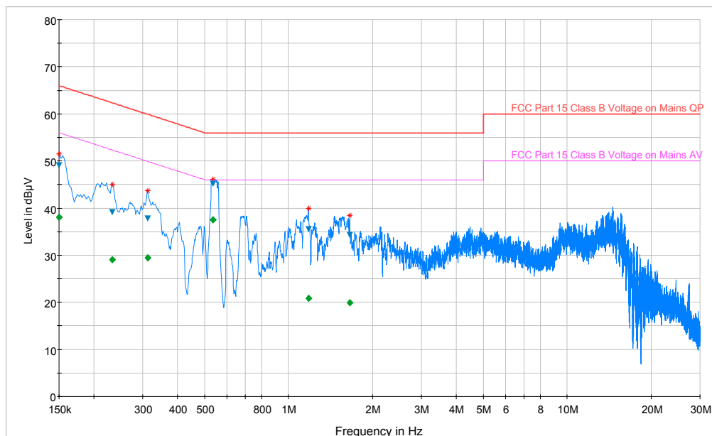
Plot 6-100. Line Conducted Plot with 802.11a UNII Band 2A (N)
