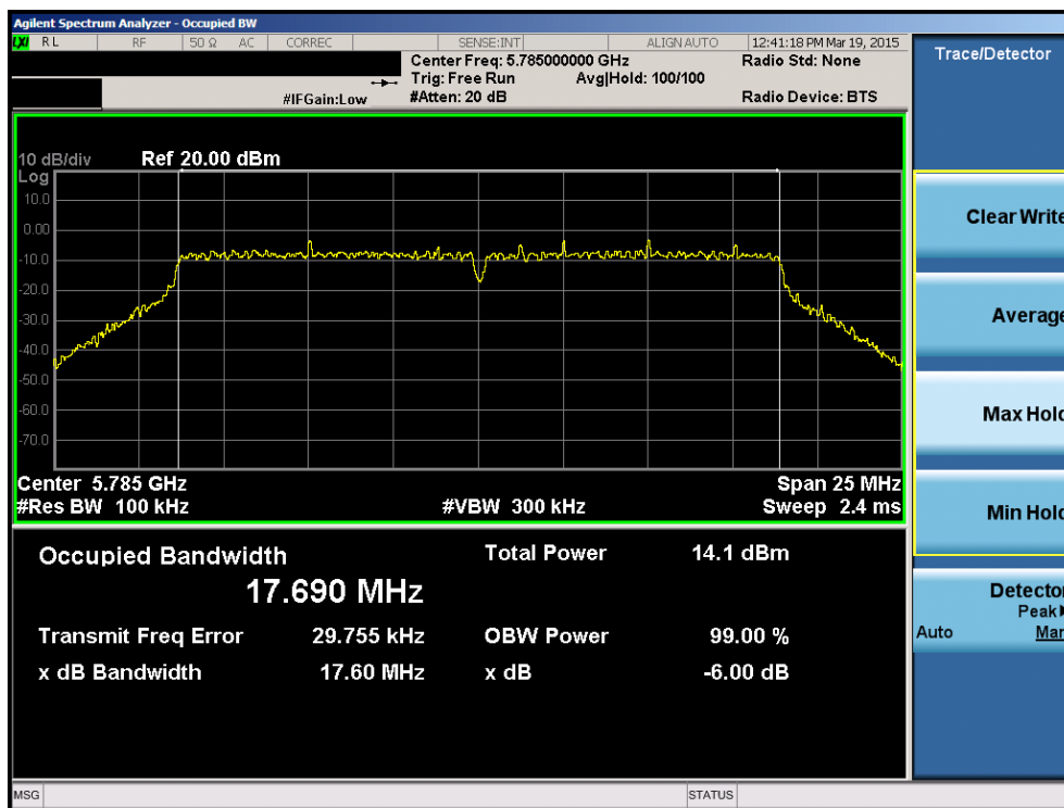
Plot 6-30. 6dB Bandwidth Plot (802.11n (UNII Band 3) – Ch. 157)
