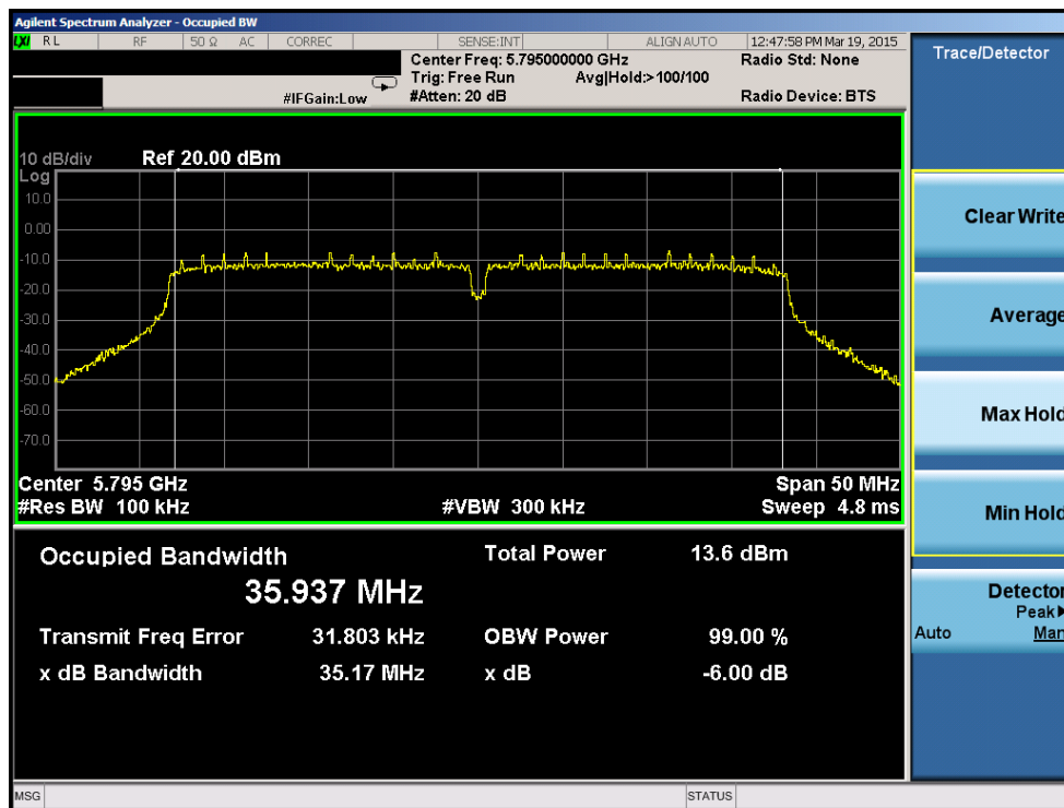
Plot 6-33. 6dB Bandwidth Plot (802.11a (UNII Band 3) – Ch. 159)
