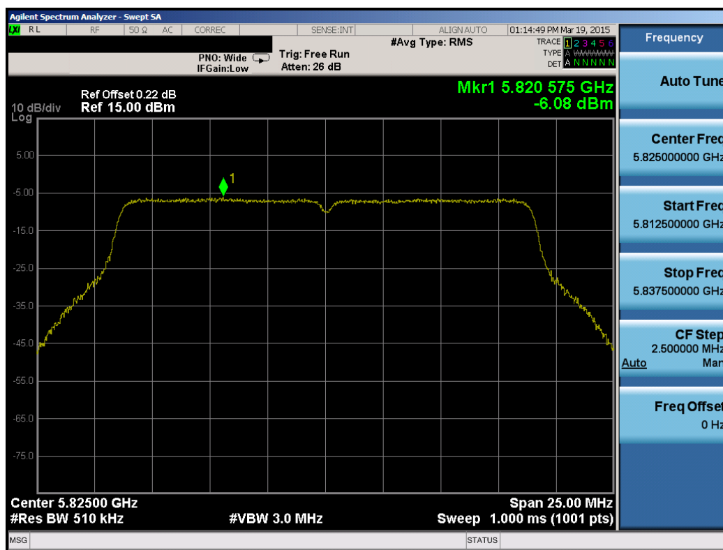
Plot 6-64. Power Spectral Density Plot (802.11n (UNII Band 3) – Ch. 165)
