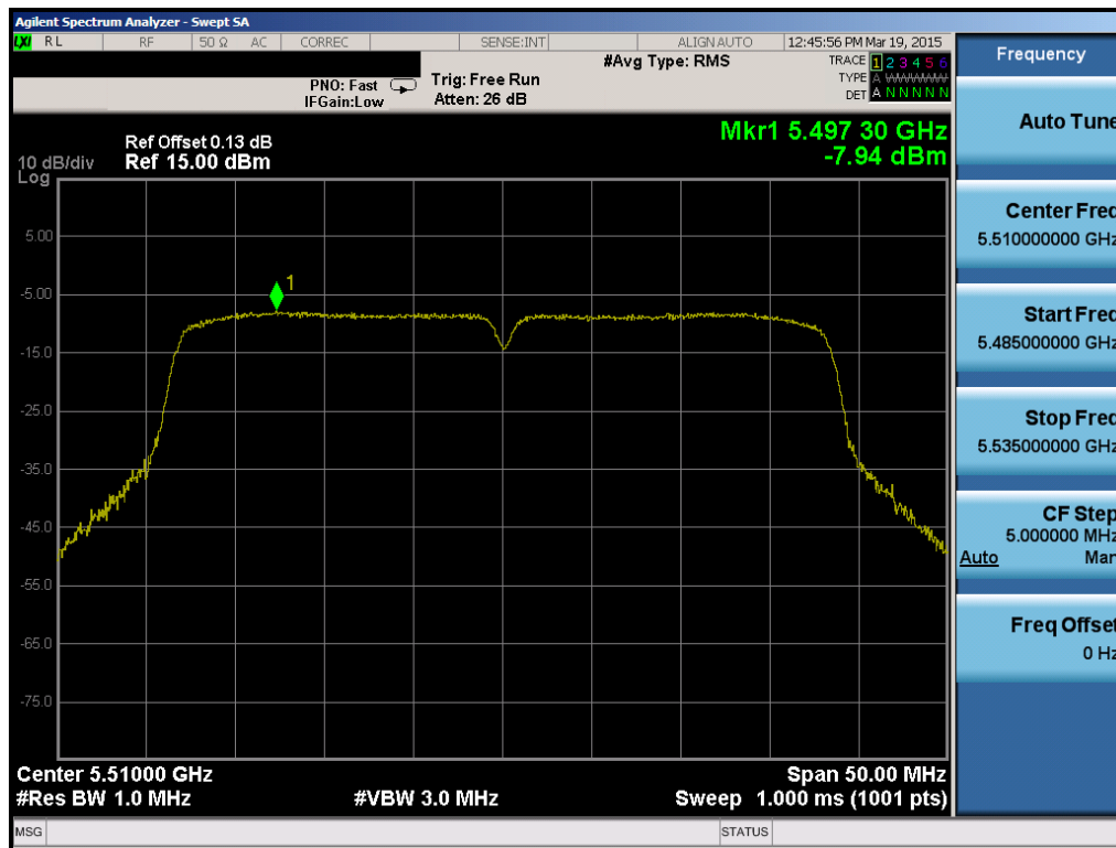
Plot 6-56. Power Spectral Density Plot (40MHz BW 802.11n (UNII Band 2C) – Ch. 102)
