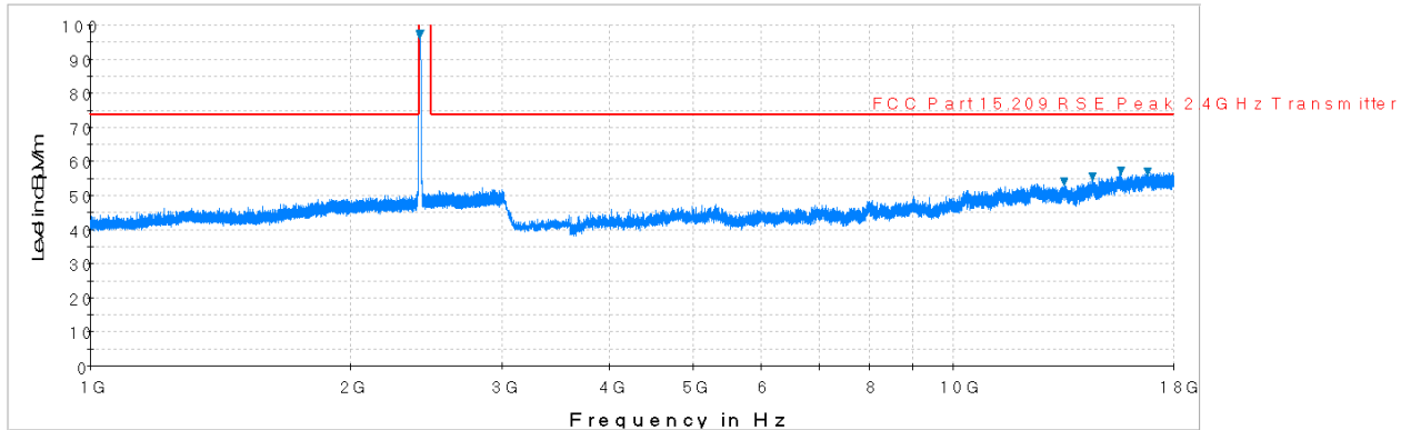
Plot 6-31. Radiated Spurious Plot above 1GHz (802.11b – Ch. 1, Ant. Pol. H)
