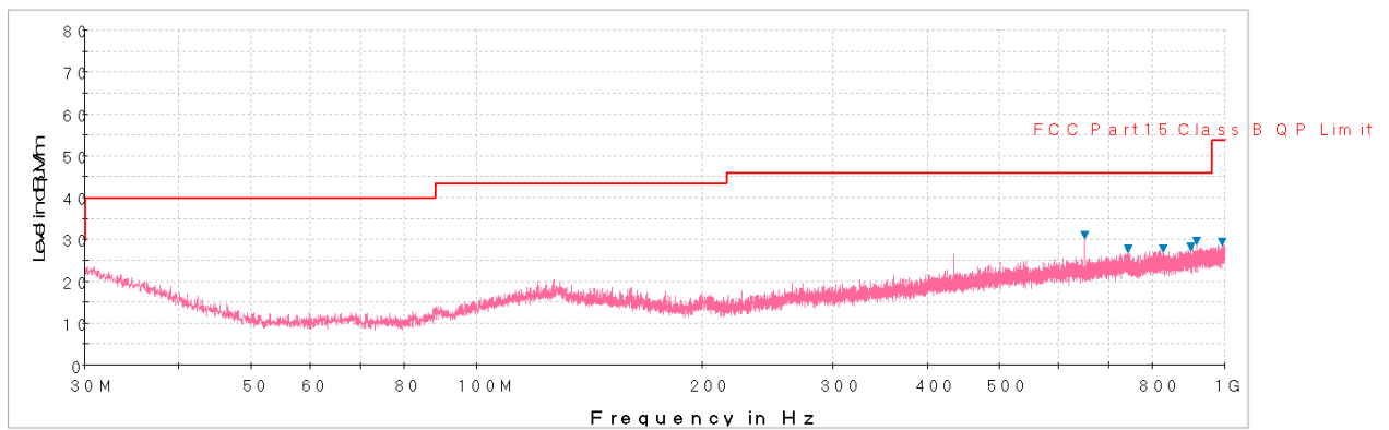
Plot 6-44. Radiated Spurious Plot below 1GHz (Pol. V)
