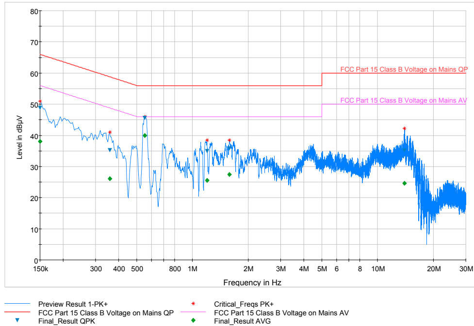
Plot 6-46. Line Conducted Plot with 802.11b (N)
