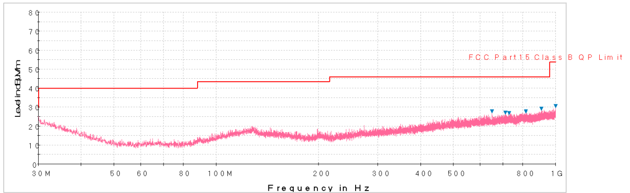
Plot 6-43. Radiated Spurious Plot below 1GHz (Pol. H)
