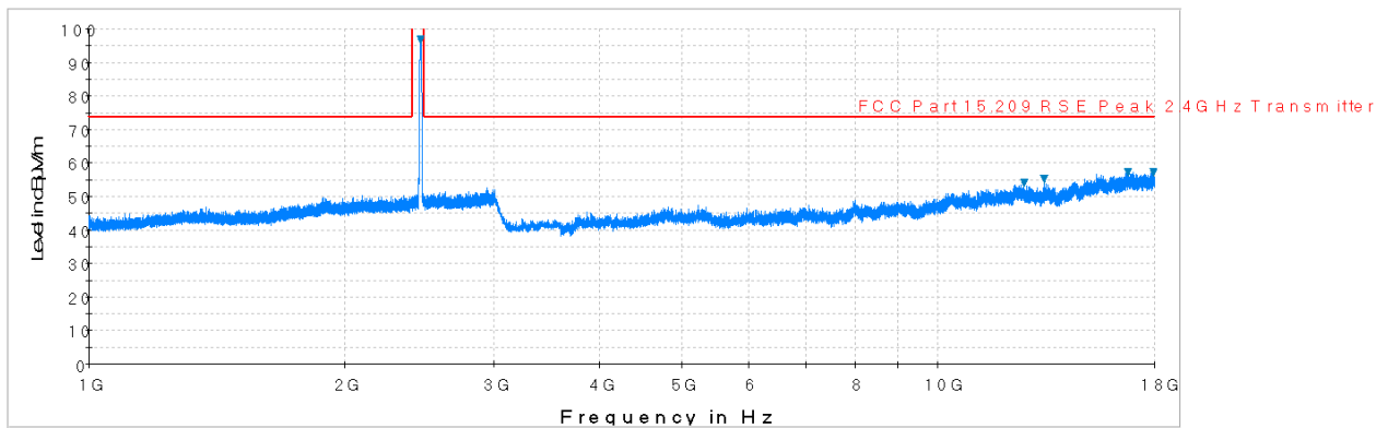
Plot 6-32. Radiated Spurious Plot above 1GHz (802.11b – Ch. 1, Ant. Pol. V)
