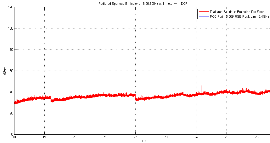
Plot 6-37. Radiated Spurious Plot above 18GHz (Pol. H)
