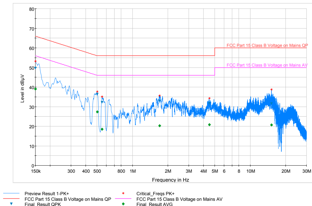
Plot 6-45. Line Conducted Plot with 802.11b (L1)
