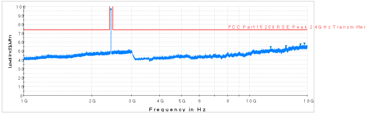
Plot 6-34. Radiated Spurious Plot above 1GHz (802.11b – Ch. 6, Ant. Pol. V)
