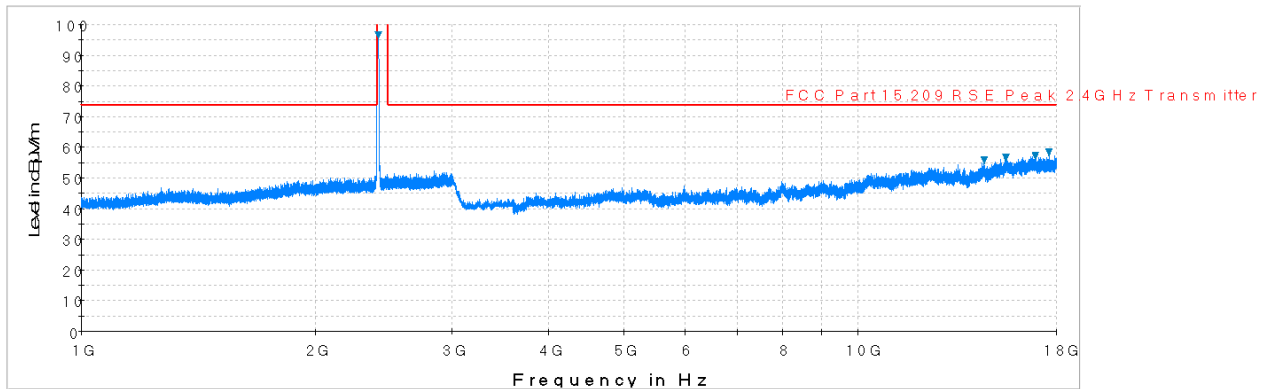
Plot 6-36. Radiated Spurious Plot above 1GHz (802.11b – Ch. 11, Ant. Pol. V)
