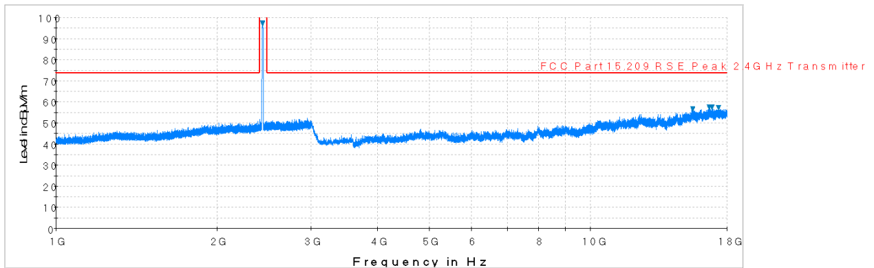
Plot 6-33. Radiated Spurious Plot above 1GHz (802.11b – Ch. 6, Ant. Pol. H)
