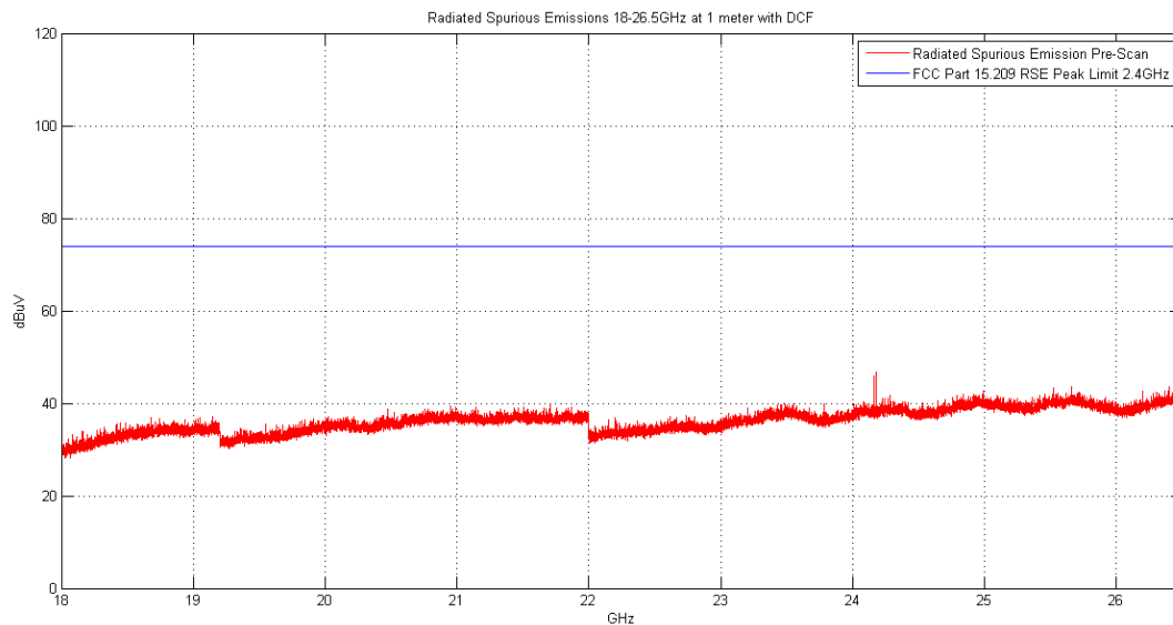
Plot 6-38. Radiated Spurious Plot above 18GHz (Pol. V)
