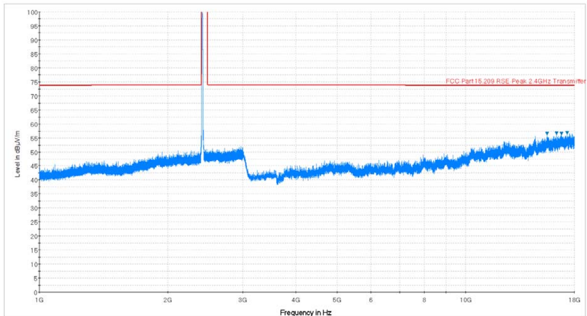
Plot 6-31. Radiated Spurious Plot above 1GHz (802.11b – Ch. 1, Ant. Pol. H)
