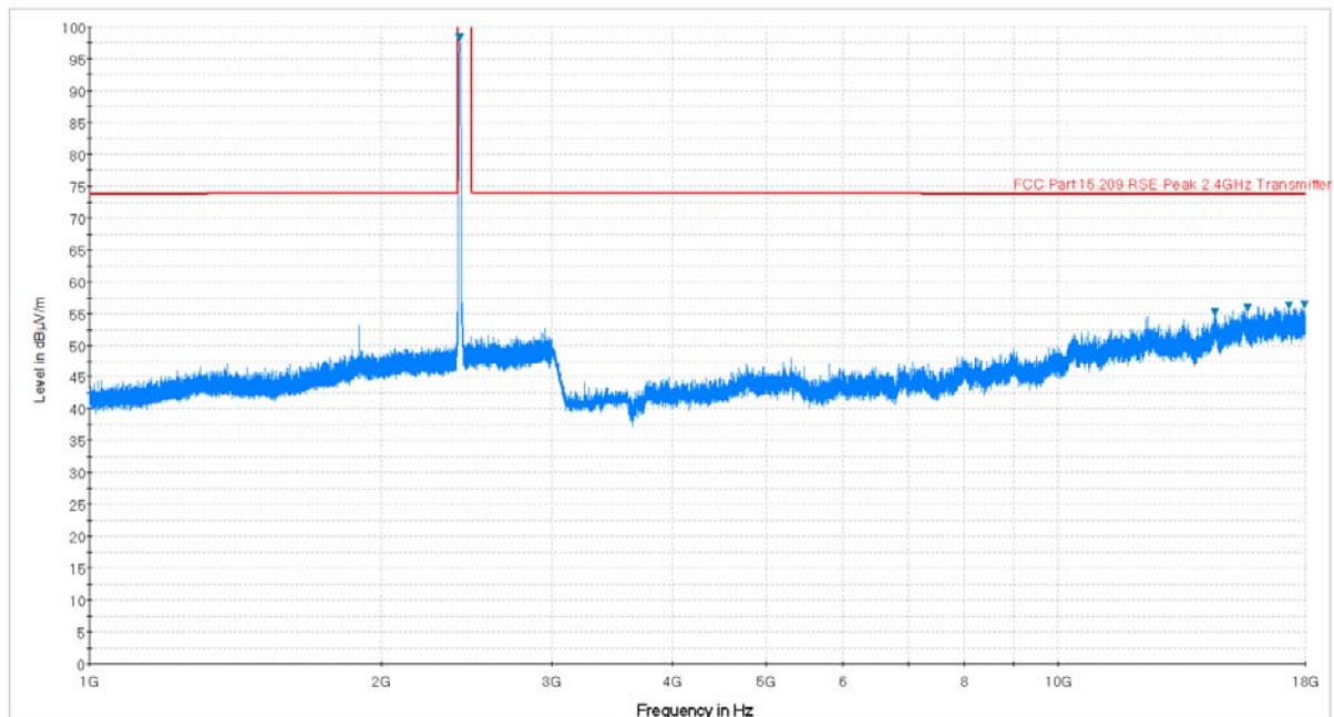
Plot 6-32. Radiated Spurious Plot above 1GHz (802.11b – Ch. 1, Ant. Pol. V)
