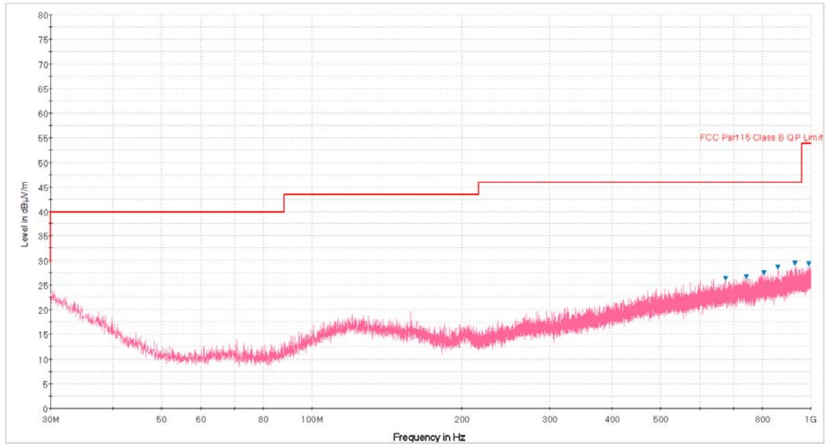
Plot 6-43. Radiated Spurious Plot below 1GHz (Pol. H)
