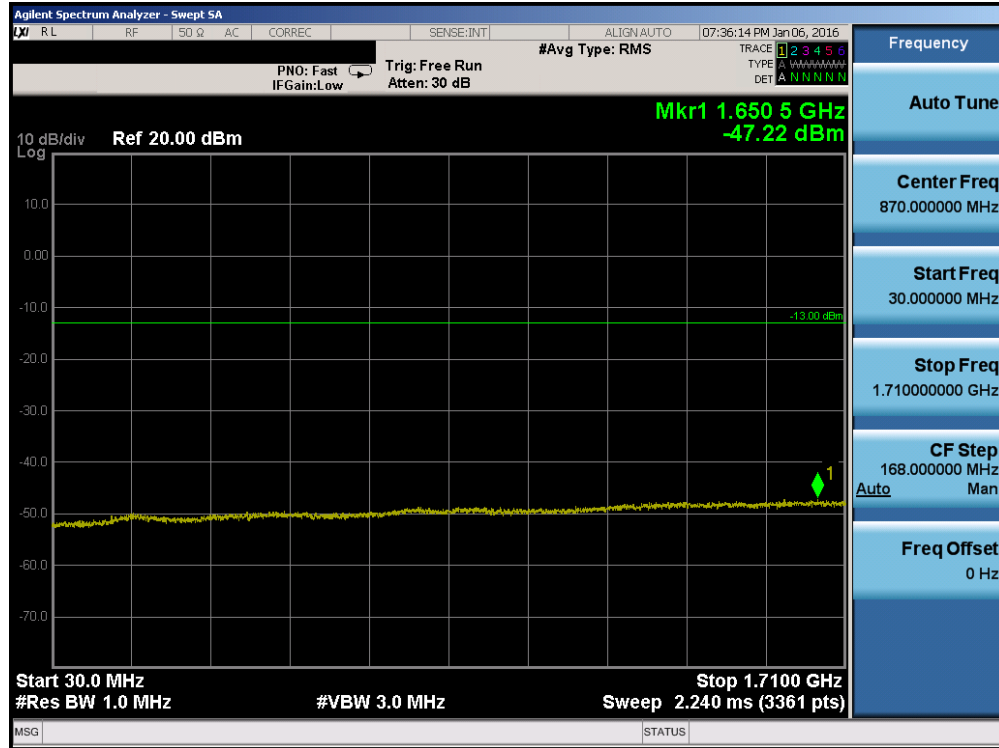
Plot 7-16. Conducted Spurious Plot (AWS WCDMA Mode – Ch. 1412)
