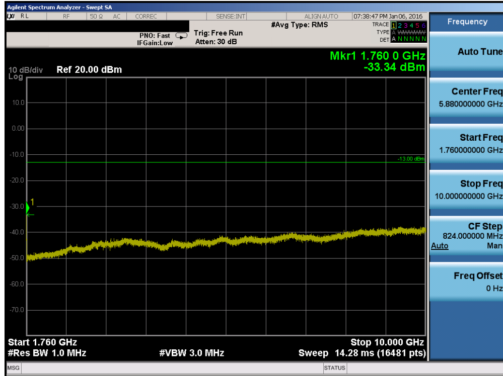
Plot 7-20. Conducted Spurious Plot (AWS WCDMA Mode – Ch. 1862)
