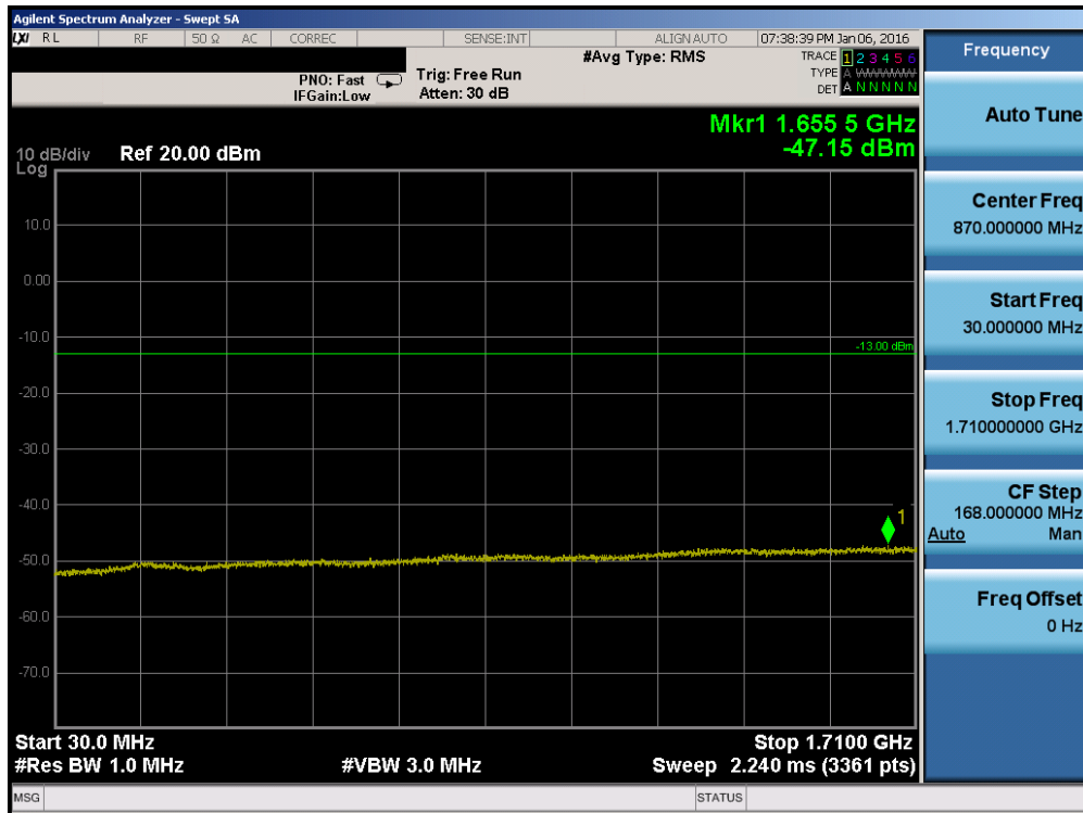
Plot 7-19. Conducted Spurious Plot (AWS WCDMA Mode – Ch. 1862)
