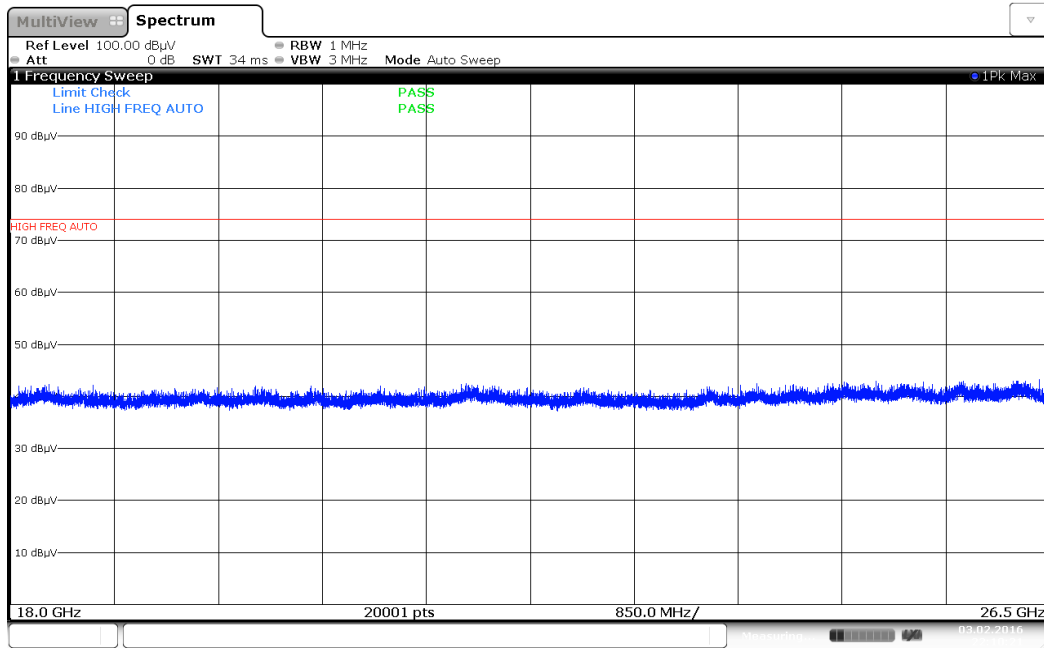
Plot 7-25. Radiated Spurious Plot above 18GHz (Pol. V)
