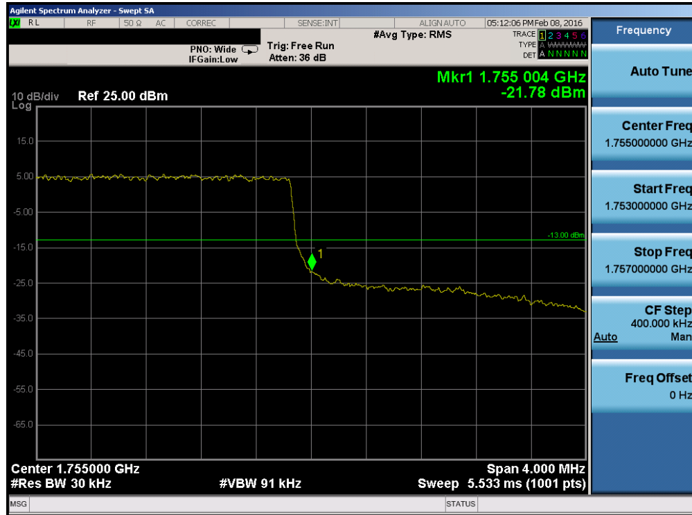
Plot 7-75. Upper Band Edge Plot (Band 4 – 3.0MHz QPSK – RB Size 15)
