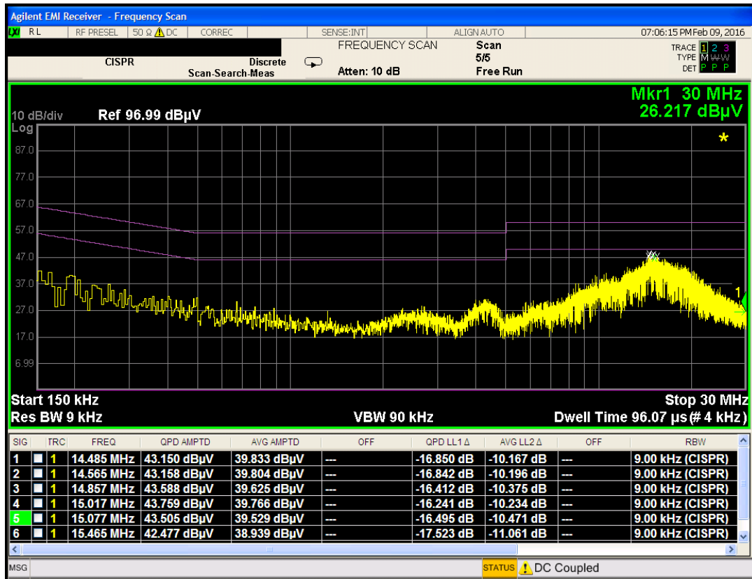
Plot 7-55. Line-Conducted Test Plot (N)
