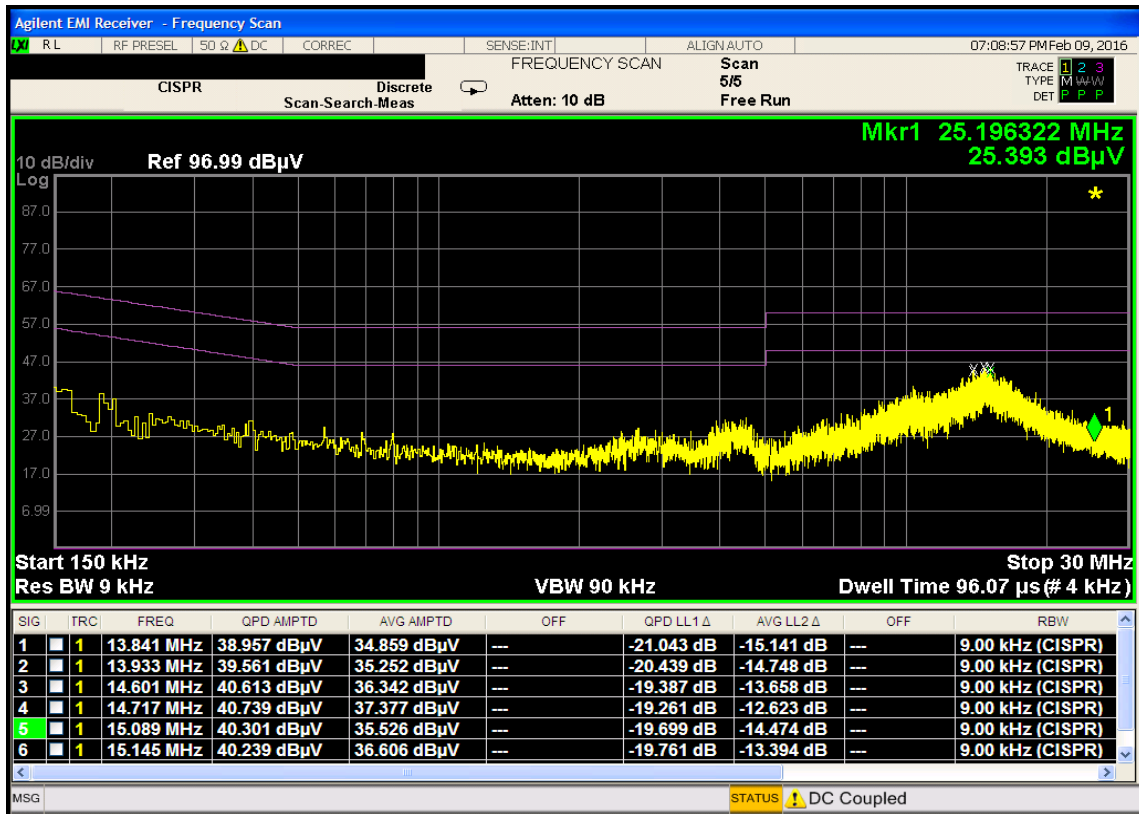
Plot 7-54. Line-Conducted Test Plot (L1)
