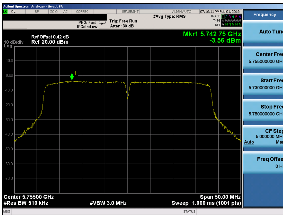
Plot 7-72. Power Spectral Density Plot (40MHz BW 802.11n (UNII Band 3) – Ch. 151)
