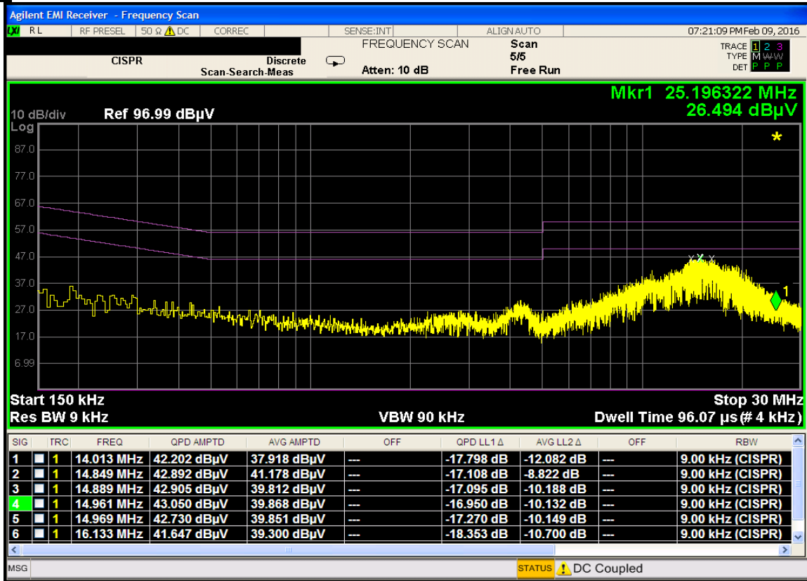
Plot 7-46. Line Conducted Plot with 802.11b (N)
