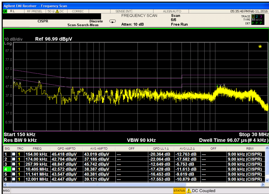
Plot 7-45. Line Conducted Plot with 802.11b (L1)
