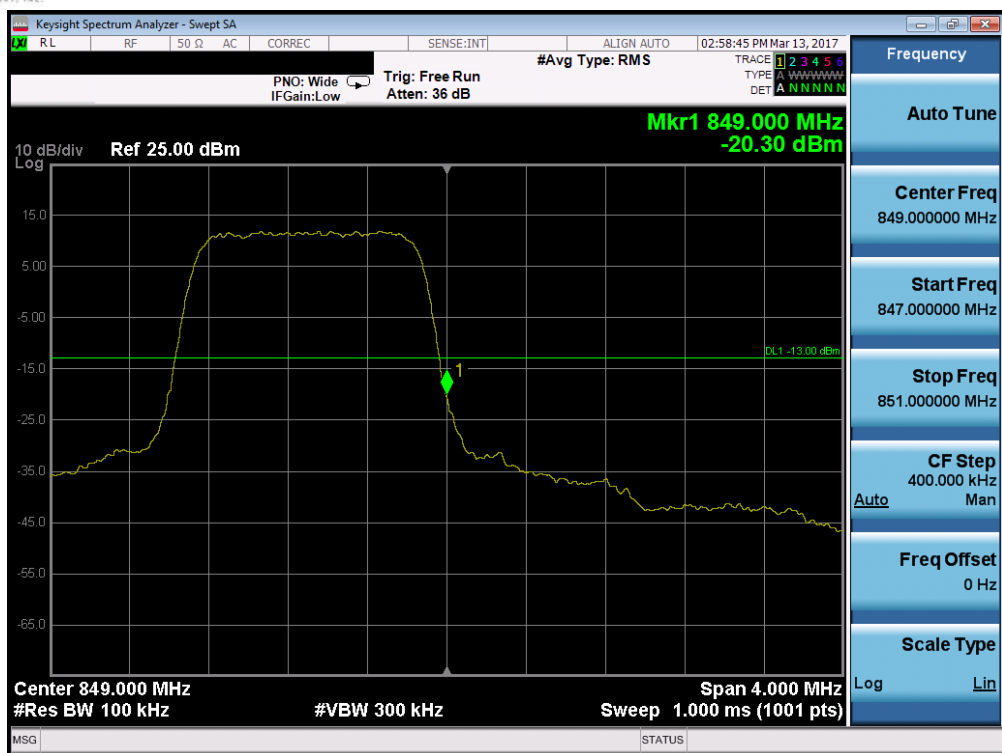
Plot 7-103. Upper Band Edge Plot (Band 5 – 1.4MHz QPSK – RB Size 6)
