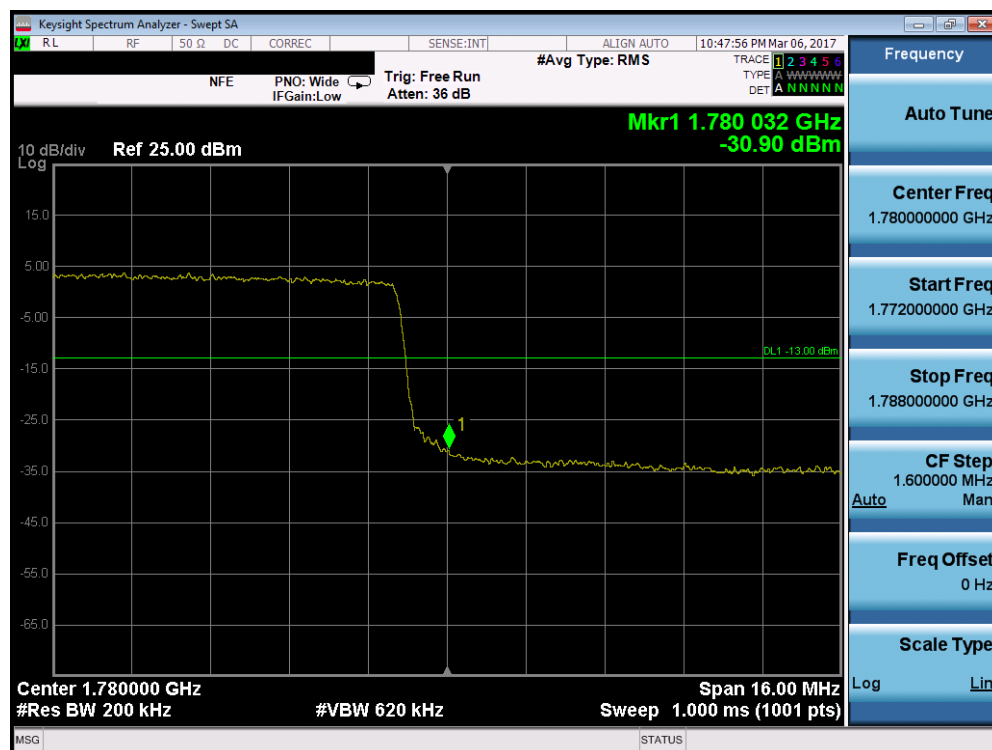
Plot 7-156. Upper Band Edge Plot (Band 66 – 20.0MHz QPSK – RB Size 100)
