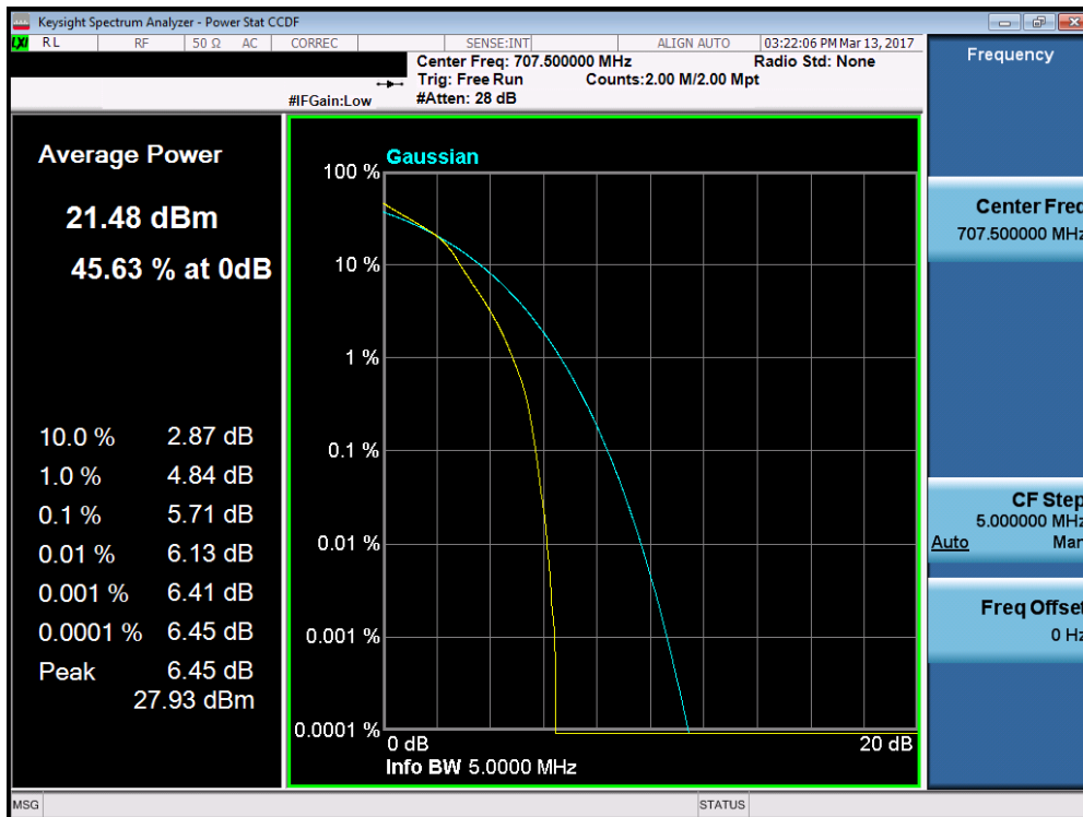
Plot 7-171. PAR Plot (Band 12 – 5.0MHz 16-QAM – RB Size 25)
