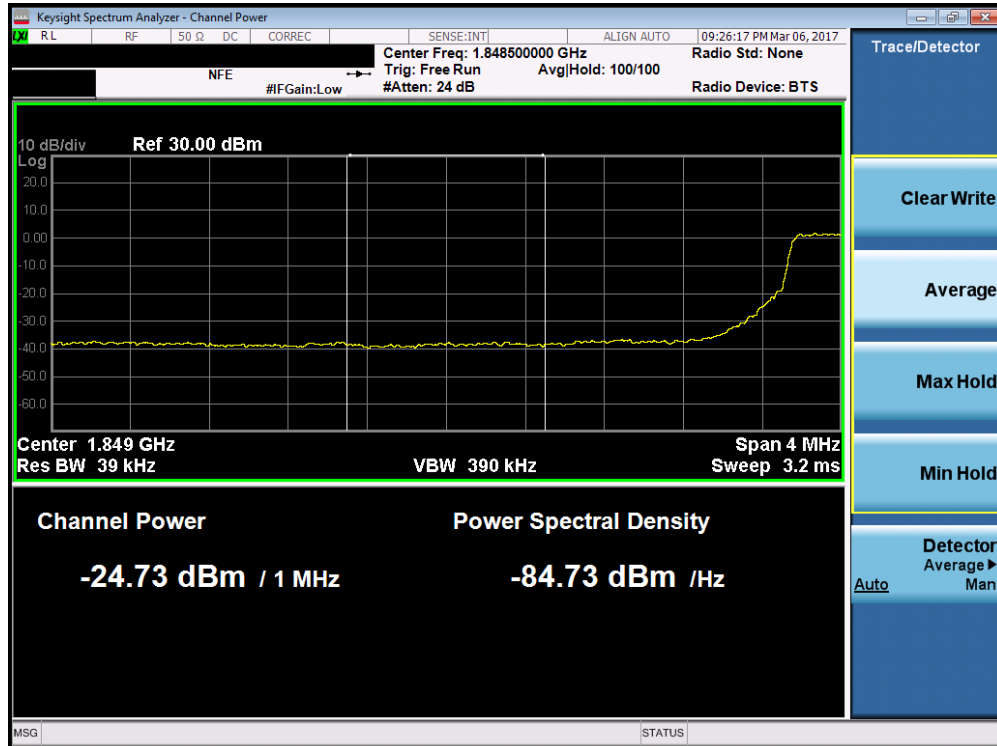
Plot 7-119. Lower Extended Band Edge Plot (Band 2 – 5.0MHz QPSK – RB Size 25)
