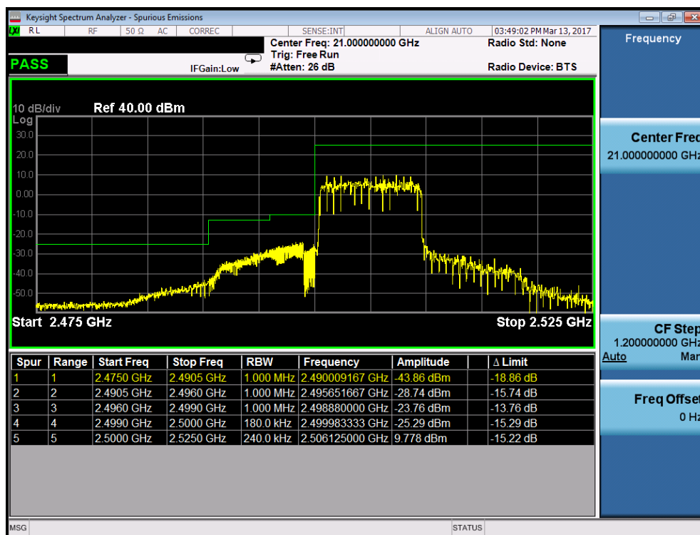
Plot 7-160. Lower ACP Plot (Band 7 – 10.0MHz QPSK – RB Size 50)
