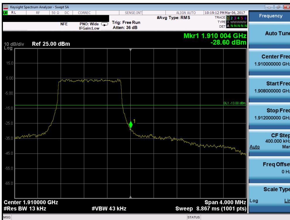
Plot 7-112. Upper Band Edge Plot (Band 2 – 1.4MHz QPSK – RB Size 6)
