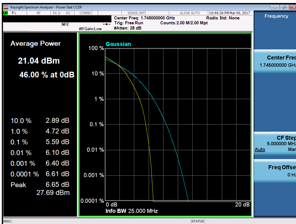
Plot 7-205. PAR Plot (Band 66 – 20.0MHz 16-QAM – RB Size 100)
