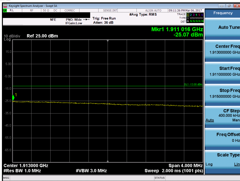
Plot 7-129. Upper Extended Band Edge Plot (Band 2 – 15.0MHz QPSK – RB Size 75)
