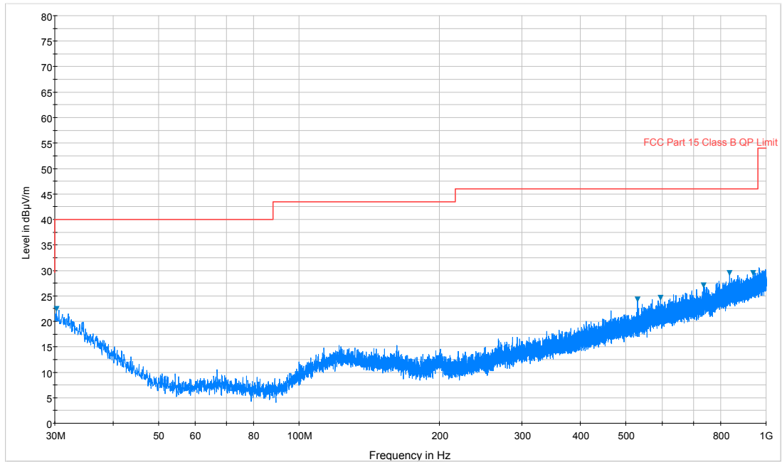
Plot 7-107. Radiated Spurious Plot below 1GHz (802.11a – U3 Ch. 157, Ant. Pol. H)
