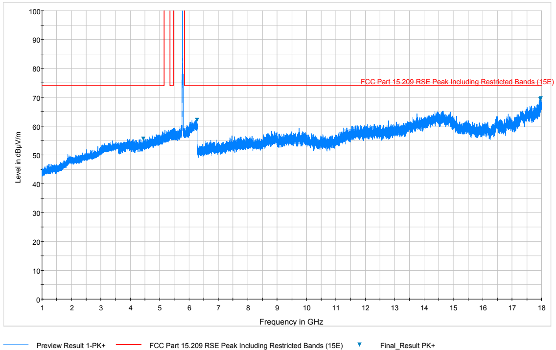
Plot 7-81. Radiated Spurious Plot above 1GHz (802.11a – U3 Ch. 157, Ant. Pol. H)
