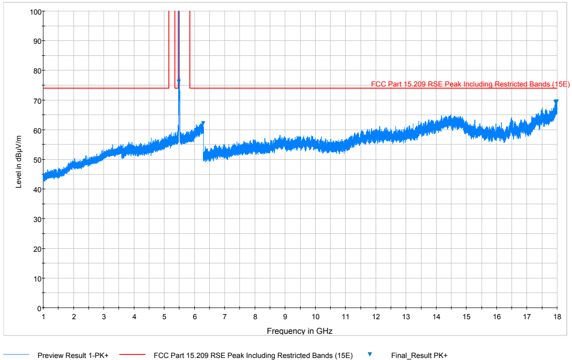
Plot 7-79. Radiated Spurious Plot above 1GHz (802.11a – U2C Ch. 116, Ant. Pol. H)
