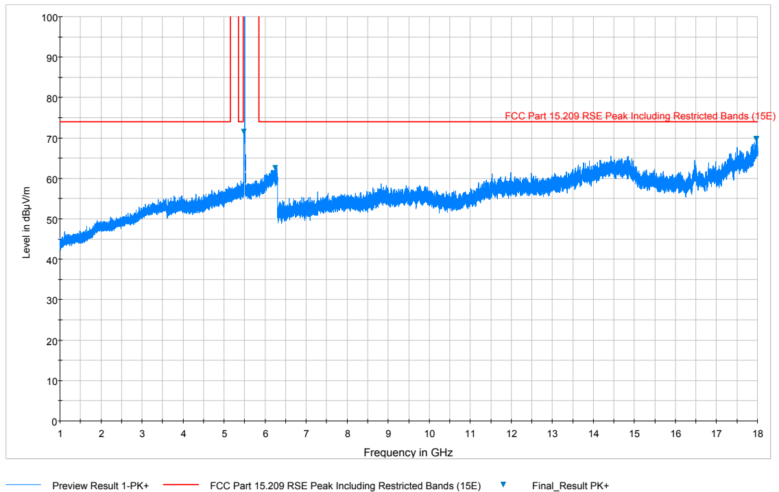
Plot 7-80. Radiated Spurious Plot above 1GHz (802.11a – U2C Ch. 116, Ant. Pol. V)
