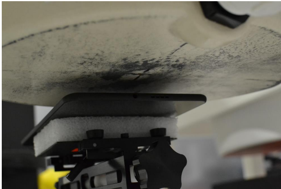
SAR Test Setup Photo 2 – Back side at 14 mm
