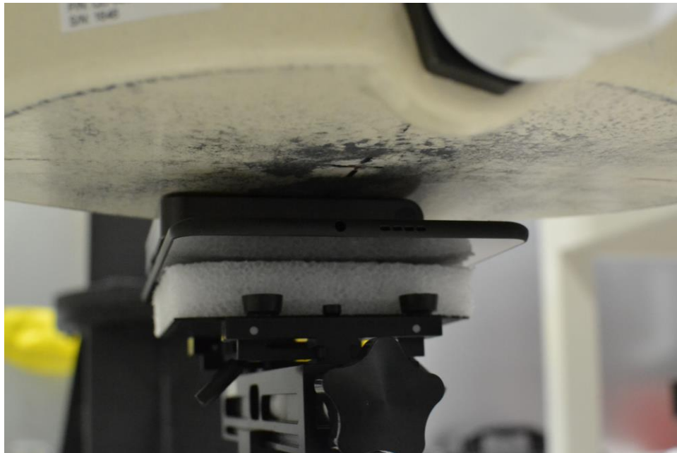
SAR Test Setup Photo 4 – Back side at 0 mm with Sound Pack
