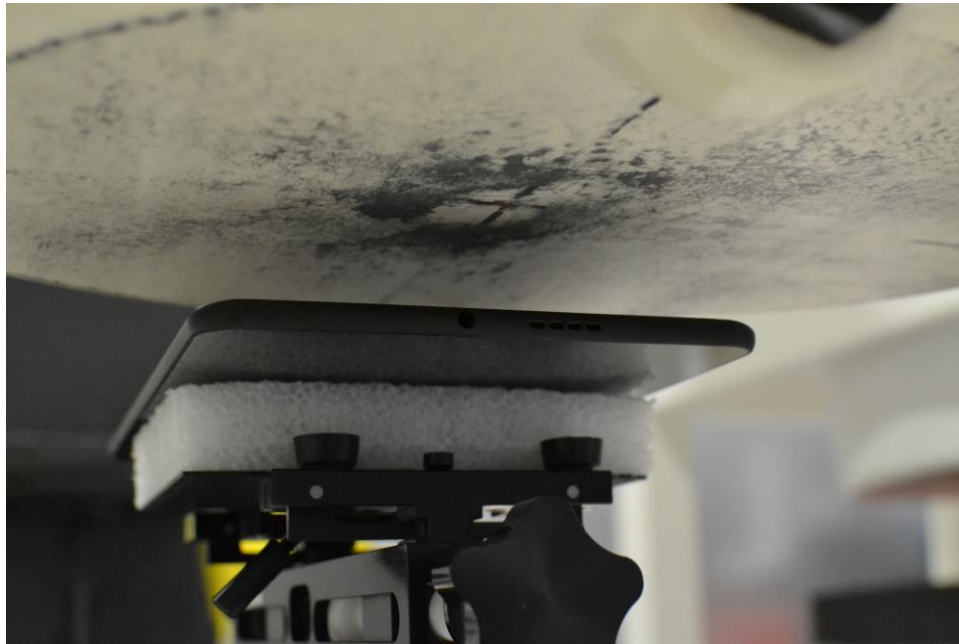
SAR Test Setup Photo 1 – Back side at 22 mm
