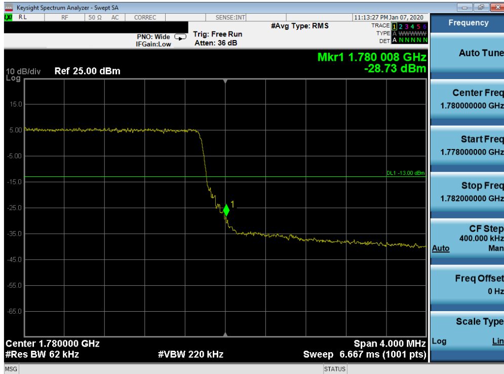
Plot 7-177. Upper Band Edge Plot (Band 66/4 - 5.0MHz QPSK - Full RB Configuration)
