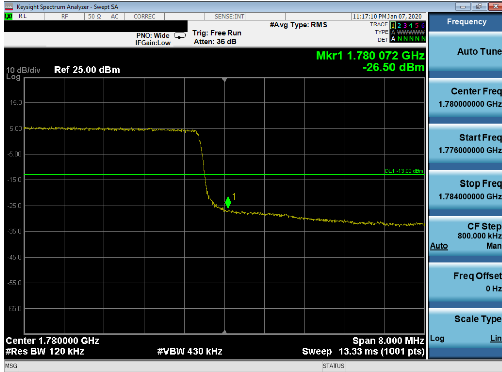
Plot 7-183. Upper Band Edge Plot (Band 66/4 - 10.0MHz QPSK - Full RB Configuration)
