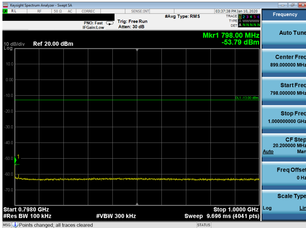
Plot 7-10. Conducted Spurious Plot (Band 14 - 10MHz QPSK - RB Size 1, RB Offset 0 - Mid Channel)
