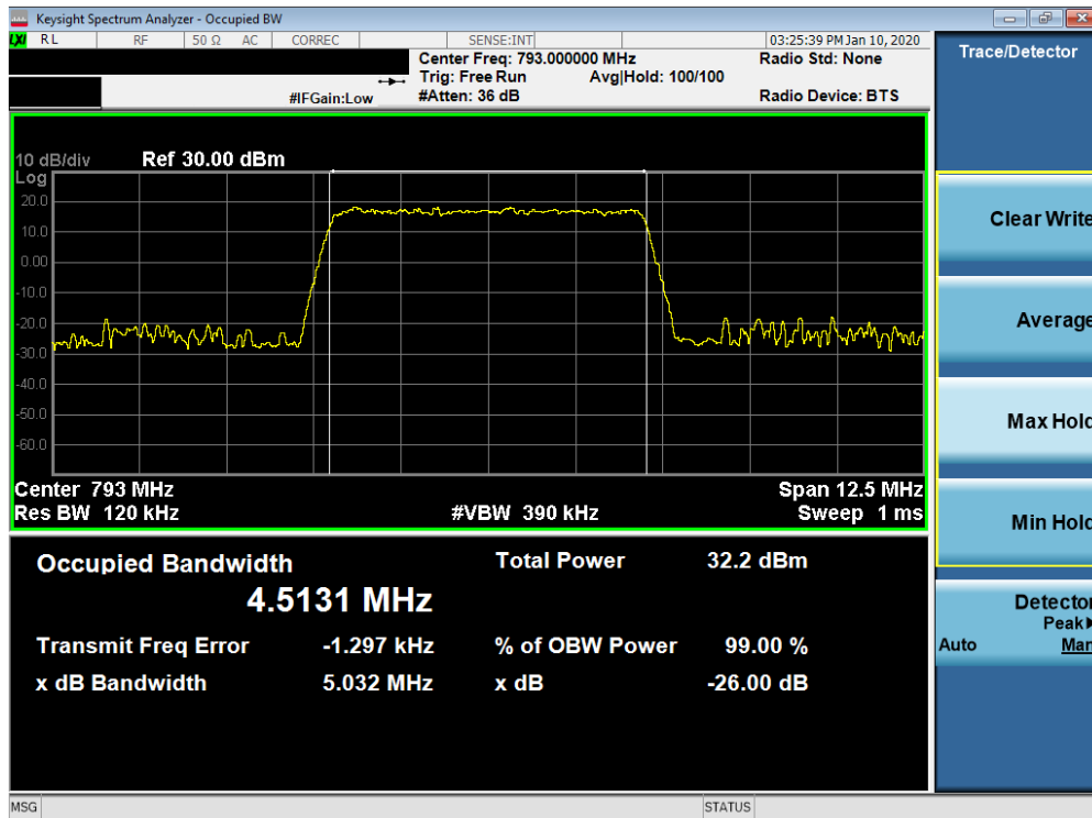
Plot 7-5. Occupied Bandwidth Plot (Band 14 - 5MHz QPSK - Full RB Configuration)
