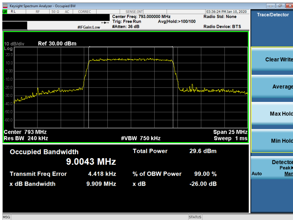
Plot 7-3. Occupied Bandwidth Plot (Band 14 - 10MHz 64-QAM - Full RB Configuration)
