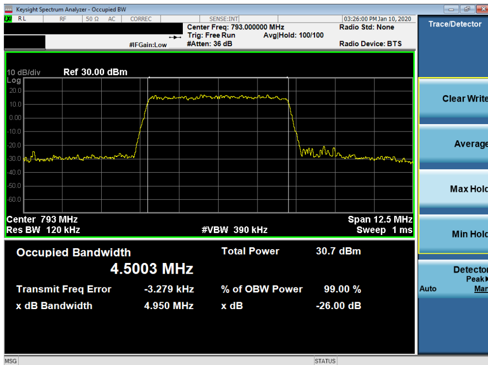
Plot 7-6. Occupied Bandwidth Plot (Band 14 - 5MHz 16-QAM - Full RB Configuration)
