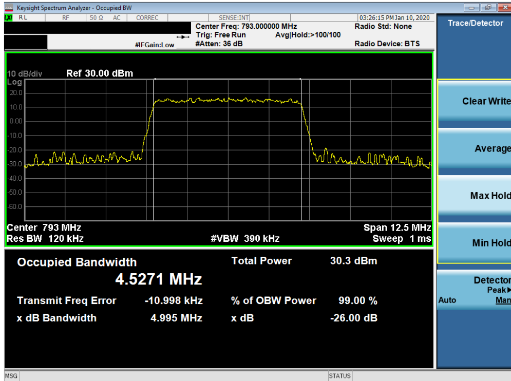
Plot 7-7. Occupied Bandwidth Plot (Band 14 - 5MHz 64-QAM - Full RB Configuration)
