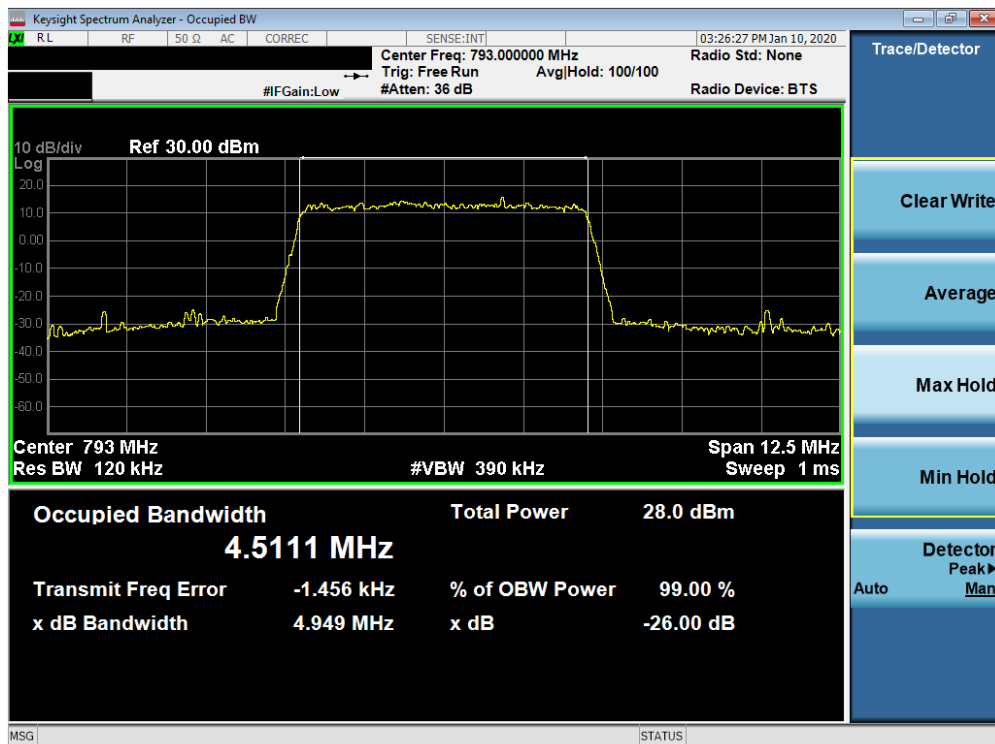
Plot 7-8. Occupied Bandwidth Plot (Band 14 - 5MHz 256-QAM - Full RB Configuration)
