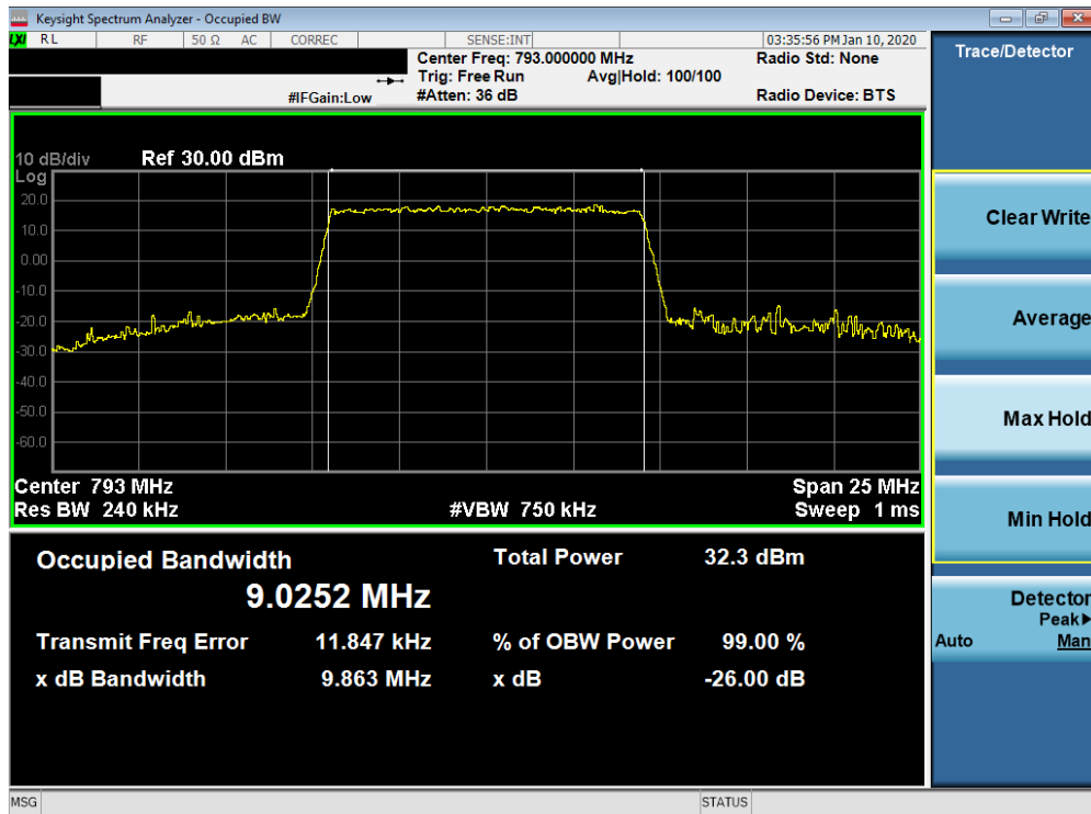
Plot 7-1. Occupied Bandwidth Plot (Band 14 - 10MHz QPSK - Full RB Configuration)
