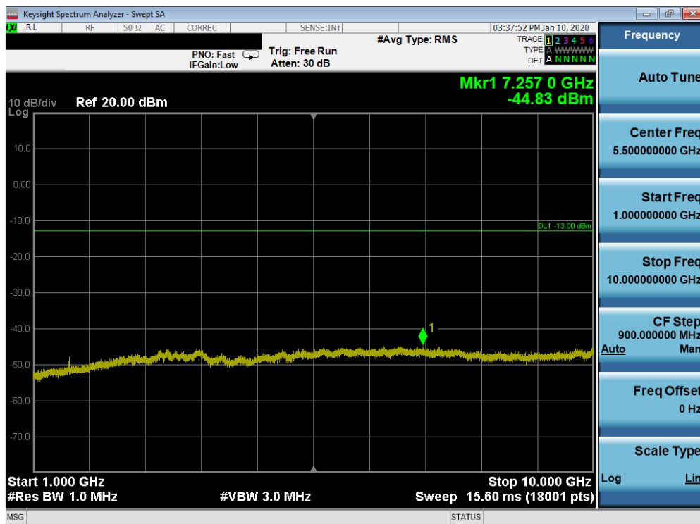
Plot 7-11. Conducted Spurious Plot (Band 14 - 10MHz QPSK - RB Size 1, RB Offset 0 - Mid Channel)
