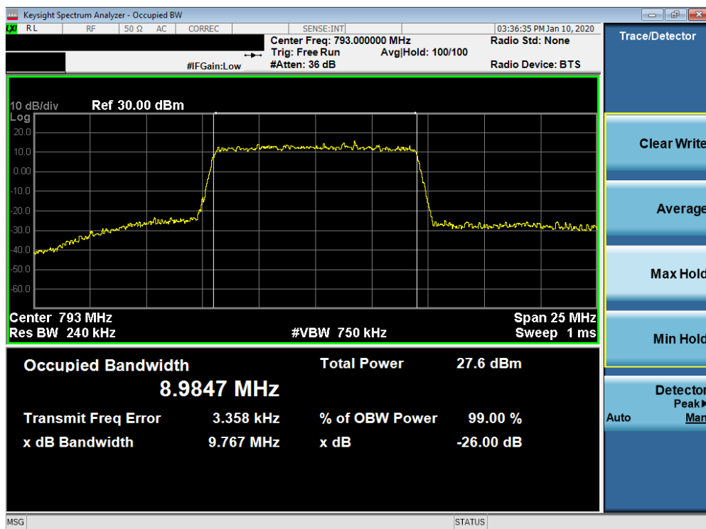
Plot 7-4. Occupied Bandwidth Plot (Band 14 - 10MHz 256-QAM - Full RB Configuration)
