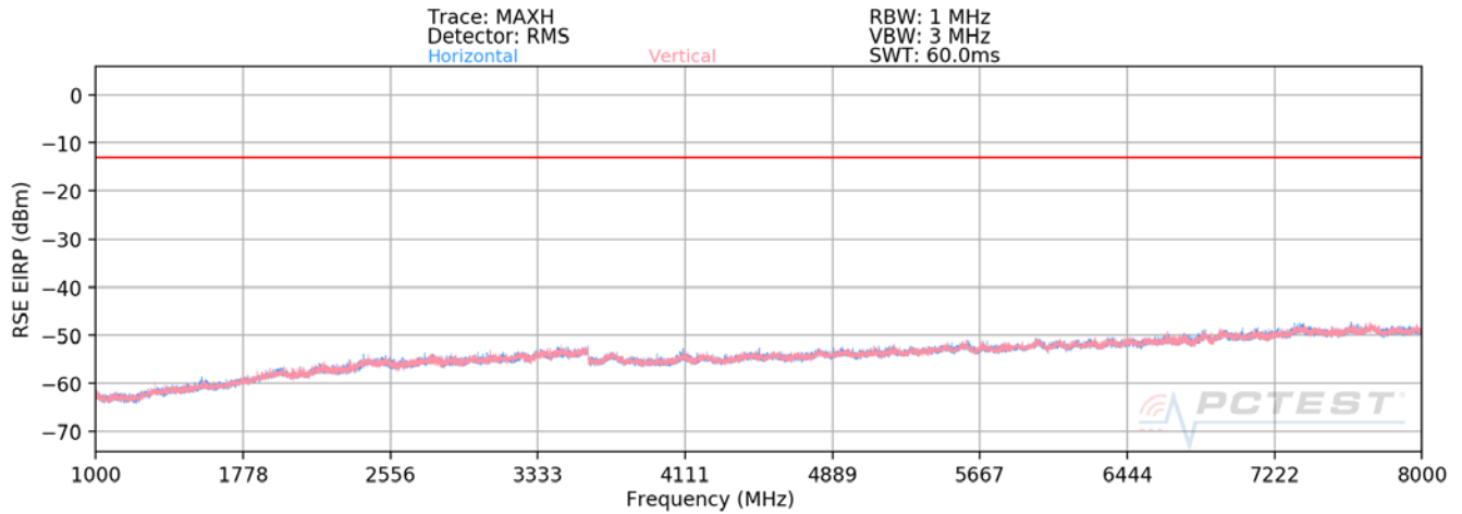
Plot 7-17. Radiated Spurious Plot (Band 14)
