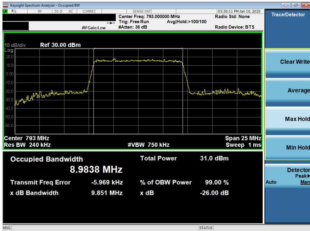
Plot 7-2. Occupied Bandwidth Plot (Band 14 - 10MHz 16-QAM - Full RB Configuration)
