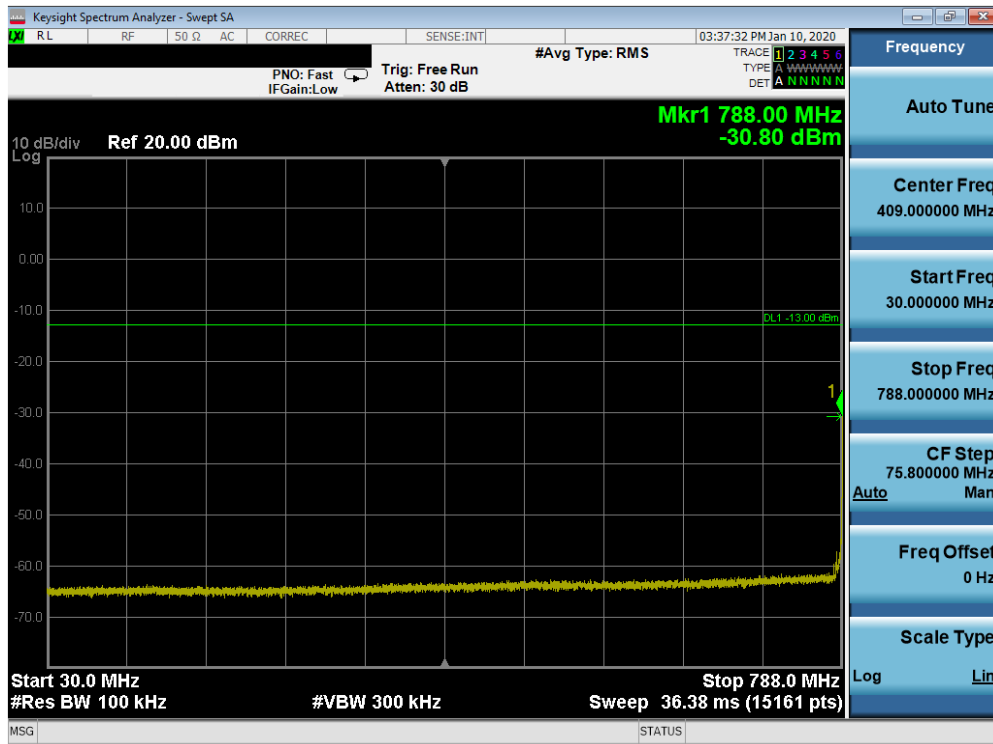
Plot 7-9. Conducted Spurious Plot (Band 14 - 10MHz QPSK - RB Size 1, RB Offset 0 - Mid Channel)
