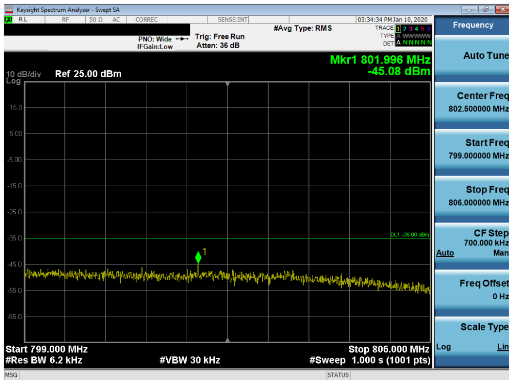
Plot 7-15. Upper Extended Band Edge Plot (Band 14 - 10MHz QPSK - Full RB Configuration)
