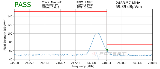
Plot 7-51. Radiated Restricted Upper Band Edge Measurement with WCP + DD (Peak)
