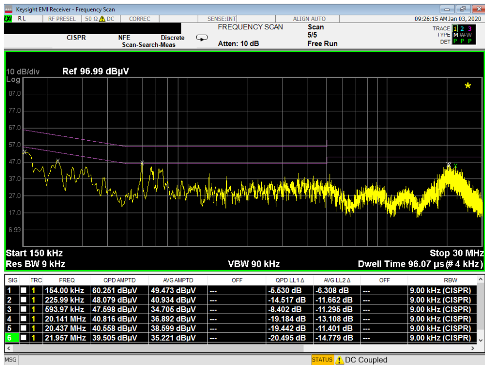
Plot 7-54. Line-Conducted Test Plot (N)
