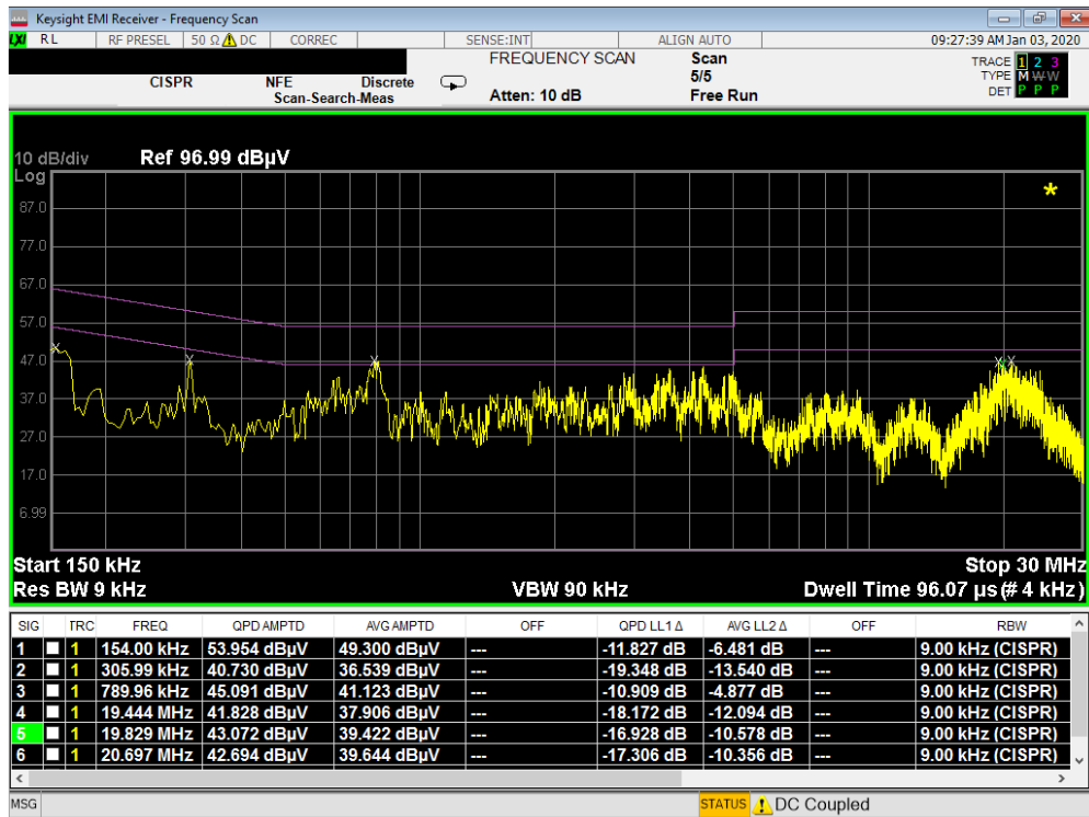
Plot 7-53. Line-Conducted Test Plot (L1)
