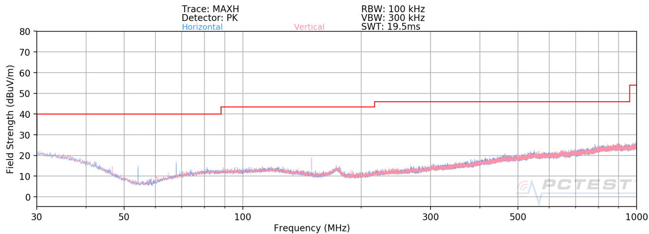
Plot 7-52. Radiated Spurious Plot below 1GHz
