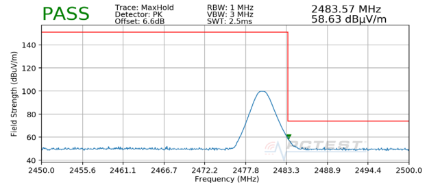
Plot 7-49. Radiated Restricted Upper Band Edge Measurement with WCP (Peak)
