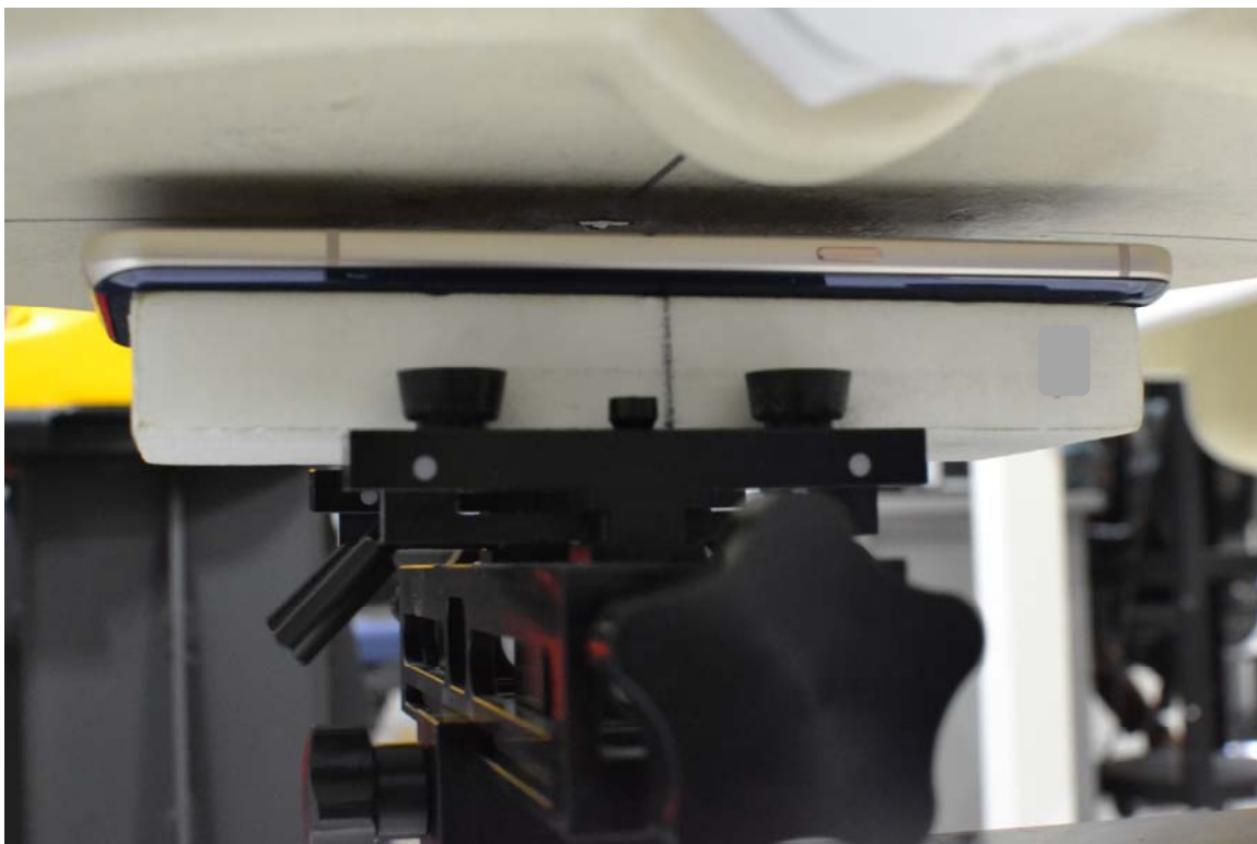
SAR Test Setup Photo 13 – Front Side at 10 mm
