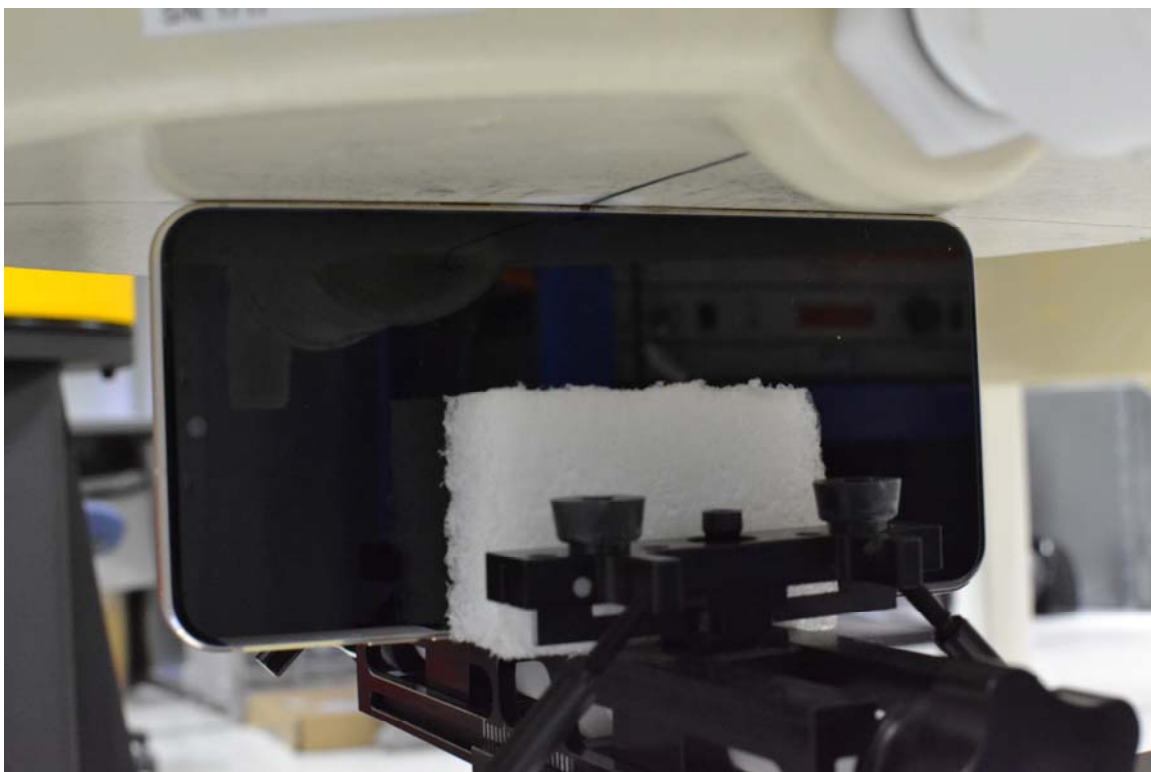
SAR Test Setup Photo 28 – Right Side at 0 mm
