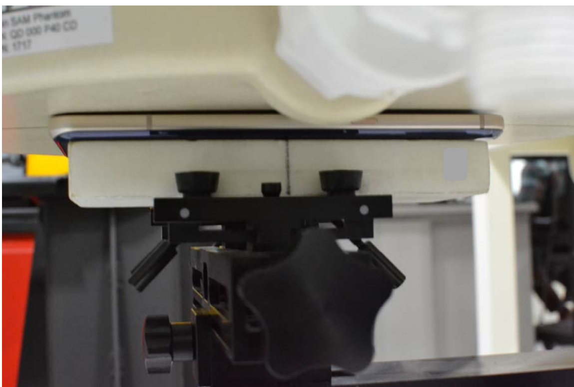
SAR Test Setup Photo 14 – Front Side at 1 mm
