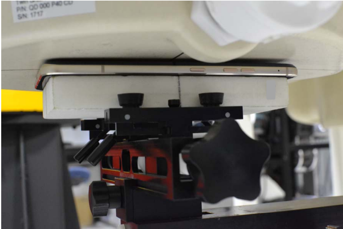
SAR Test Setup Photo 11 – Back Side at 2 mm
