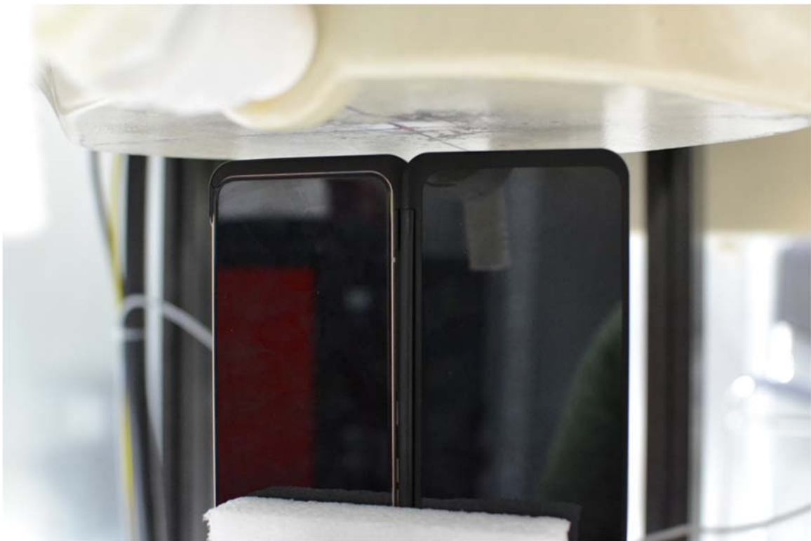
SAR Test Setup Photo 20 – Bottom Side at 10 mm with Dual Display Cover Position #2 (180 degrees)
