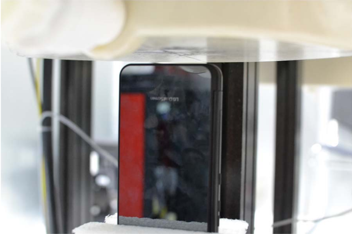
SAR Test Setup Photo 19 – Bottom Side at 10 mm with Dual Display Cover Position #1 (0 degrees)
