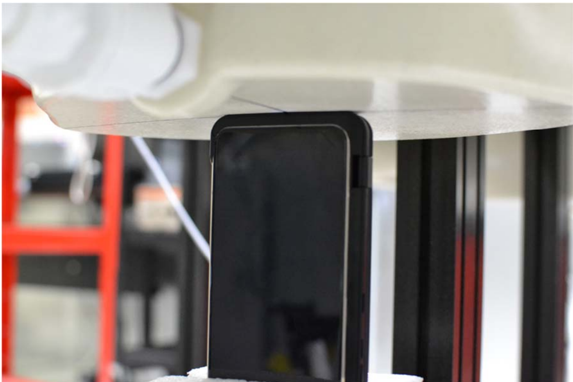
SAR Test Setup Photo 26 – Bottom Side at 0 mm with Dual Display Cover Position #3 (360 degrees)
