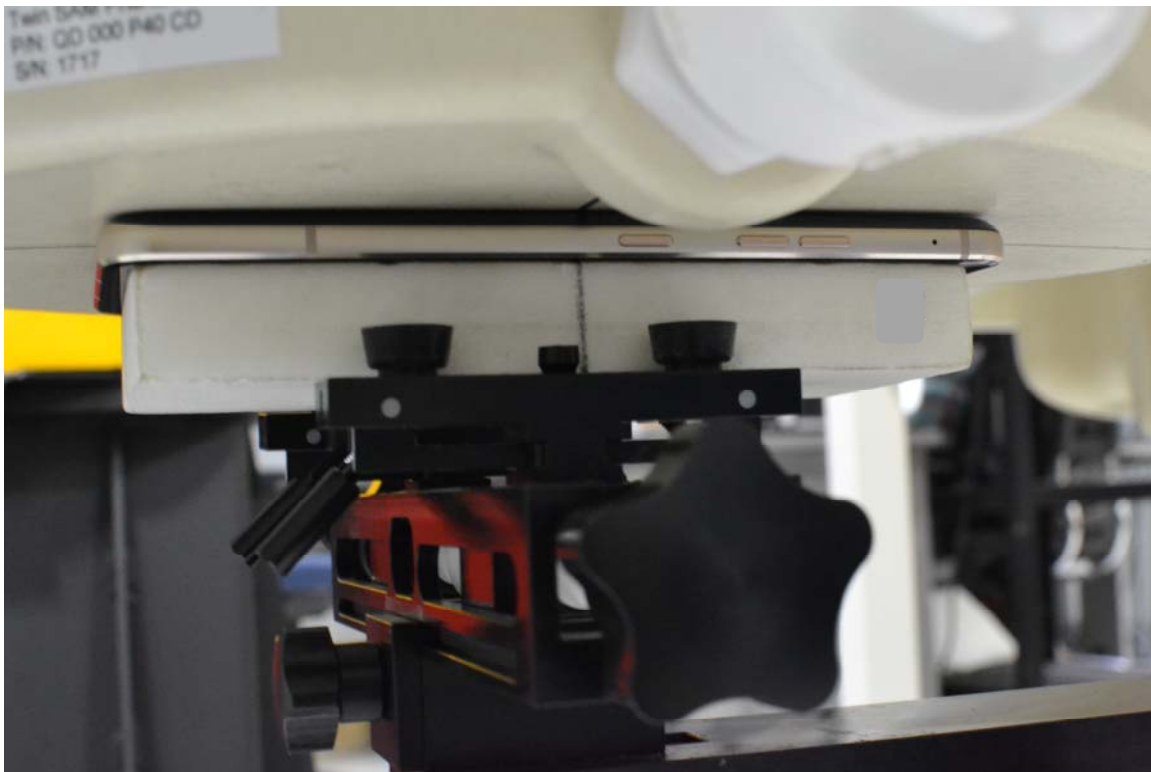
SAR Test Setup Photo 12 – Back Side at 0 mm
