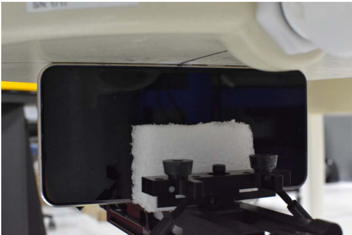
SAR Test Setup Photo 30 – Left Side at 0 mm
