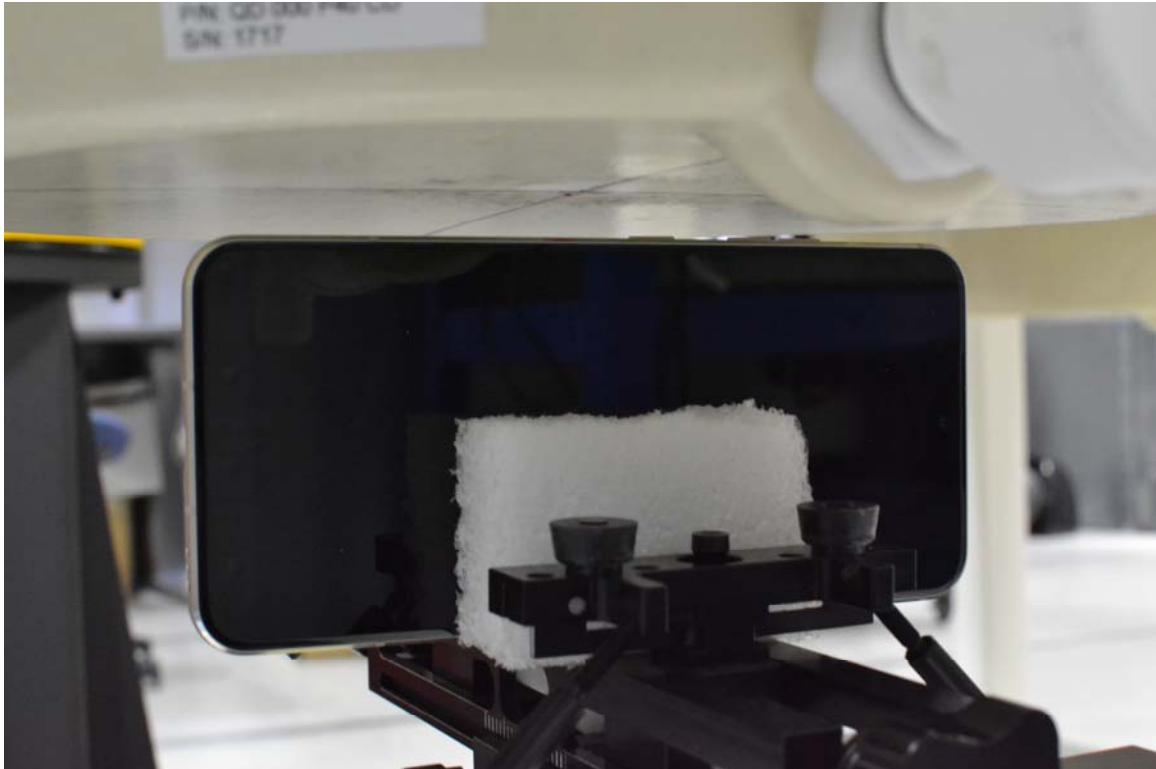
SAR Test Setup Photo 29 – Left Side at 10 mm
