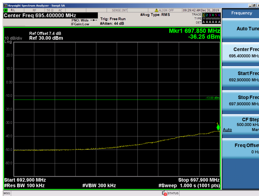
LTE Band 12 / 3MHz / 64QAM - RB Size/Offset (8/0)
