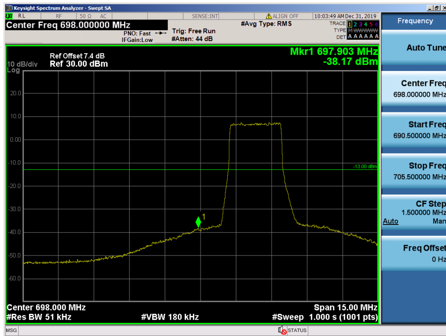
LTE Band 12, 17 / 5MHz / 64QAM - RB Size/Offset (12/0)
