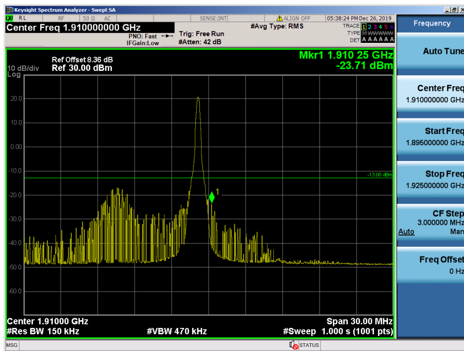
LTE Band 2 / 15MHz / 64QAM - RB Size/Offset (1/74)
