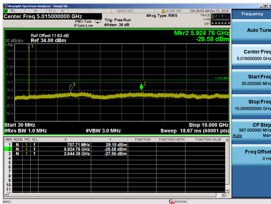
LTE Band 12 / 3MHz / 64QAM - RB Size/Offset (8/4) – Mid Channel
