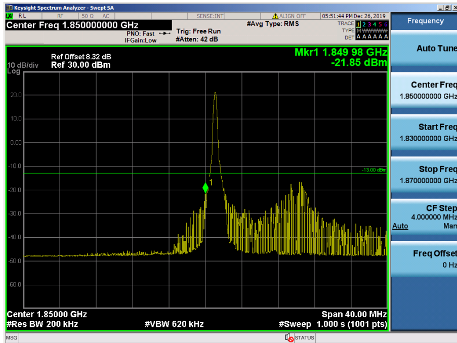
LTE Band 2 / 20MHz / 64QAM - RB Size/Offset (1/0)
