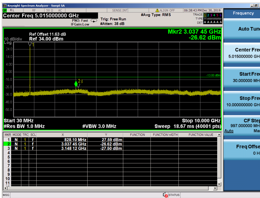
LTE Band 5 / 10MHz / QPSK - RB Size/Offset (25/12) – Low Channel
