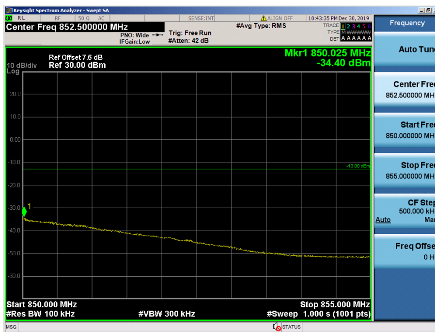
LTE Band 5 / 3MHz / 64QAM - RB Size/Offset (15/0)
