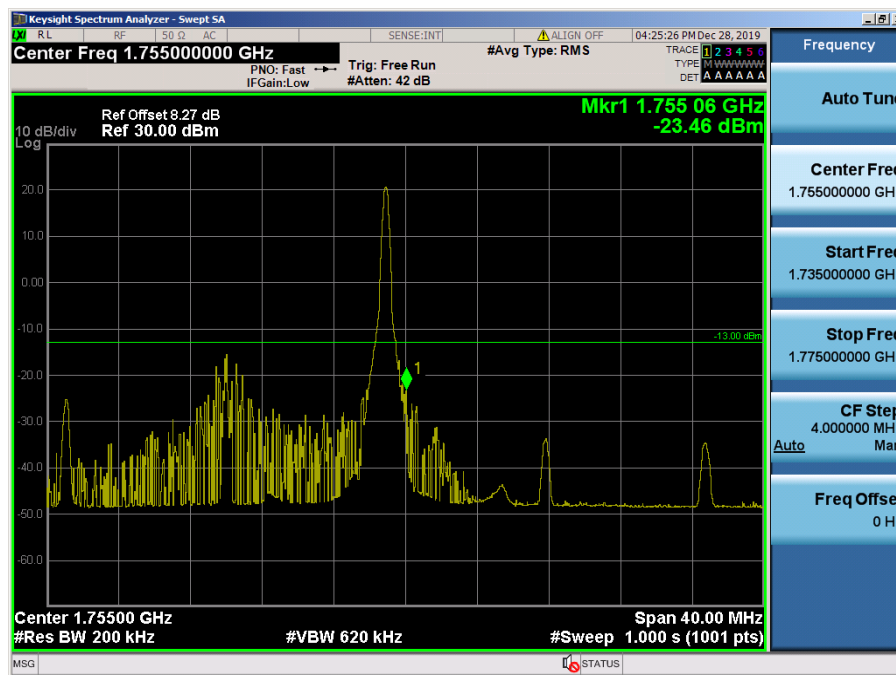
LTE Band 4 / 20MHz / 64QAM - RB Size/Offset (1/99)
