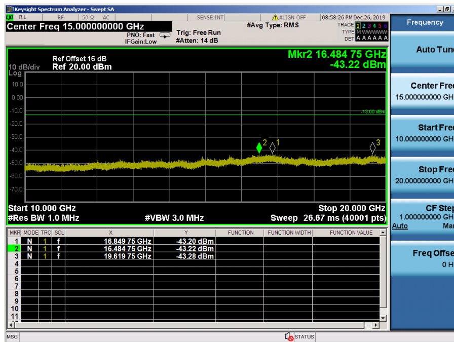
LTE Band 4 / 10MHz / QPSK - RB Size/Offset (1/0)– Mid Channel
