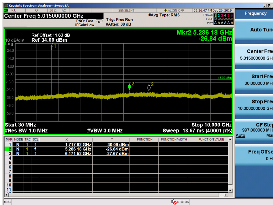
LTE Band 4 / 15MHz / QPSK - RB Size/Offset (1/36)–Low Channel
