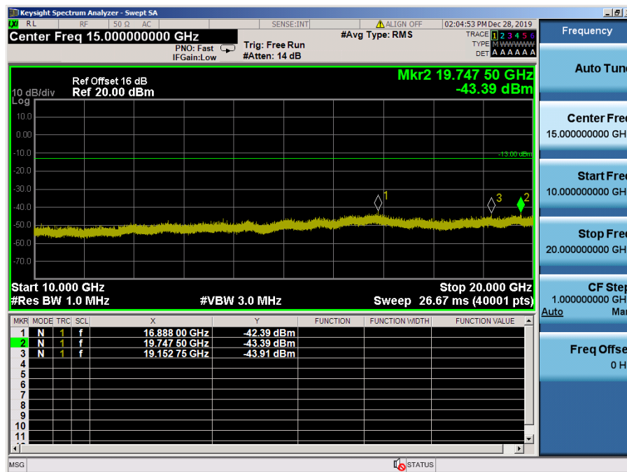
LTE Band 4 / 5MHz / 64QAM - RB Size/Offset (12/13) – Low Channel
