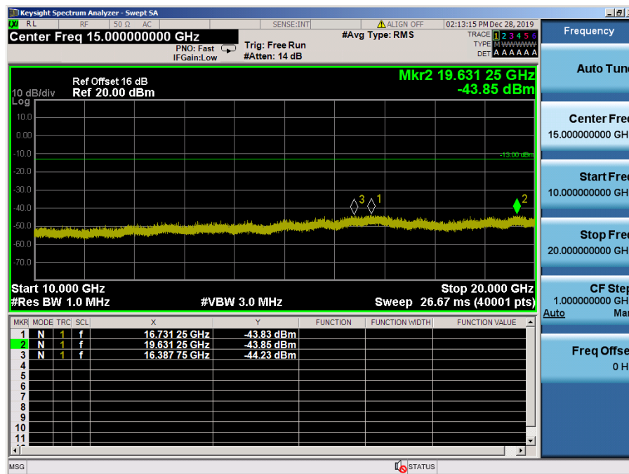
LTE Band 4 / 5MHz / 64QAM - RB Size/Offset (25/0) – Mid Channel
