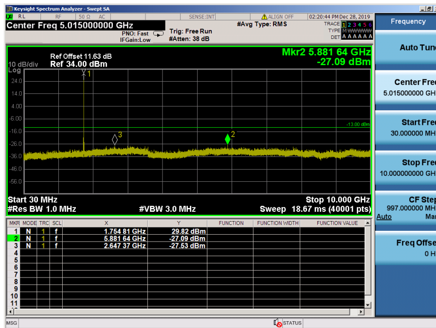
LTE Band 4 / 5MHz / 64QAM - RB Size/Offset (1/24) – High Channel
