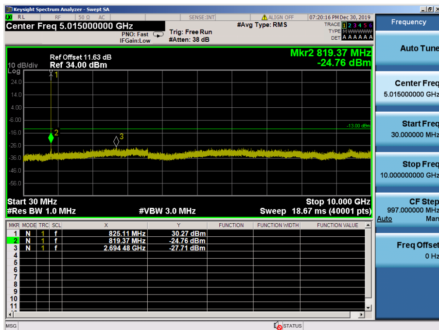
LTE Band 5 / 1.4MHz / 16QAM - RB Size/Offset (6/0) – Low Channel
