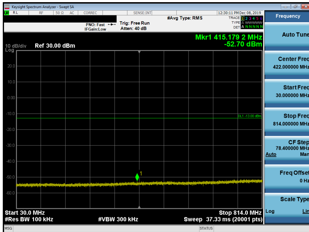
Plot 7-26. Conducted Spurious Plot (CDMA/EvDO, Ch. 684)
