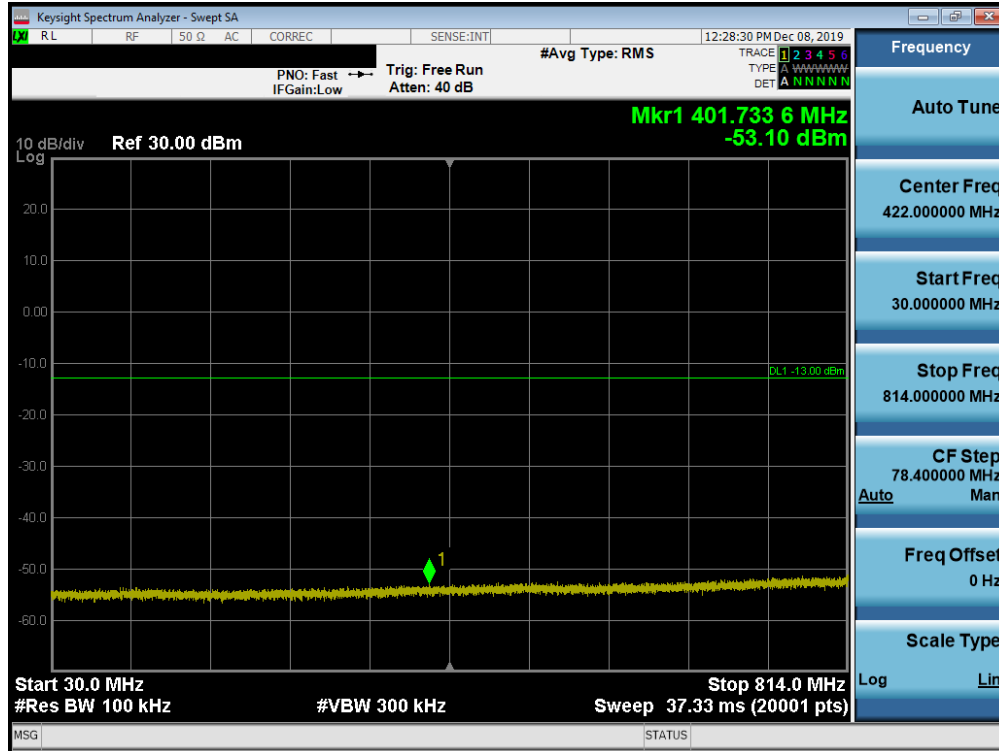
Plot 7-23. Conducted Spurious Plot (CDMA/EvDO, Ch. 476)
