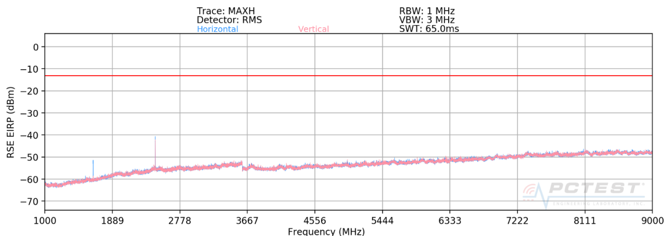
Plot 7-43. Radiated Spurious Plot (CDMA BC10)
