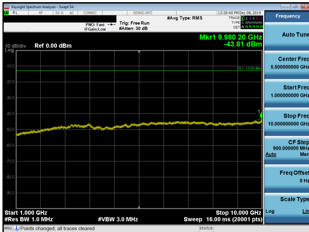
Plot 7-28. Conducted Spurious Plot (CDMA/EvDO, Ch. 684)
