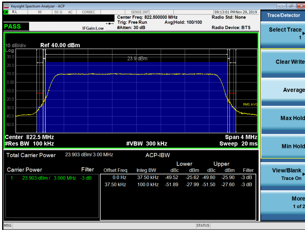
Plot 7-39. Channel Edge Plot (LTE Band 26 - 3MHz QPSK - High Channel)
