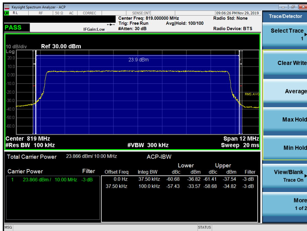
Plot 7-35. Channel Edge Plot (LTE Band 26 - 10MHz QPSK)
