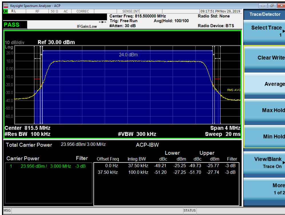
Plot 7-38. Channel Edge Plot (LTE Band 26 - 3MHz QPSK - Low Channel)
