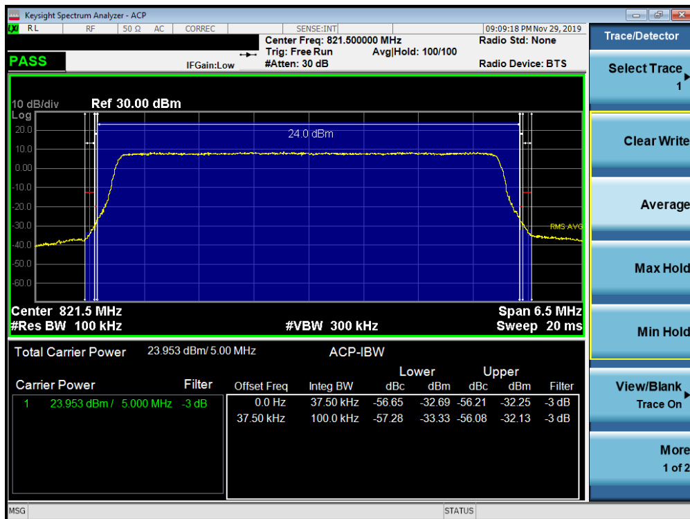
Plot 7-37. Channel Edge Plot (LTE Band 26 - 5MHz QPSK - High Channel)
