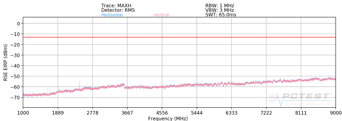
Plot 7-44. Radiated Spurious Plot (Band 26)
