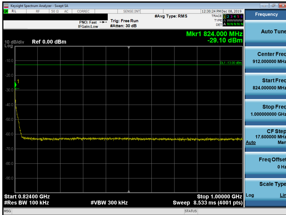
Plot 7-27. Conducted Spurious Plot (CDMA/EvDO, Ch. 684)
