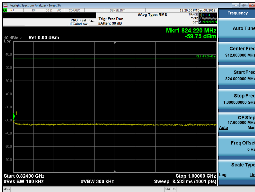
Plot 7-24. Conducted Spurious Plot (CDMA/EvDO, Ch. 476)
