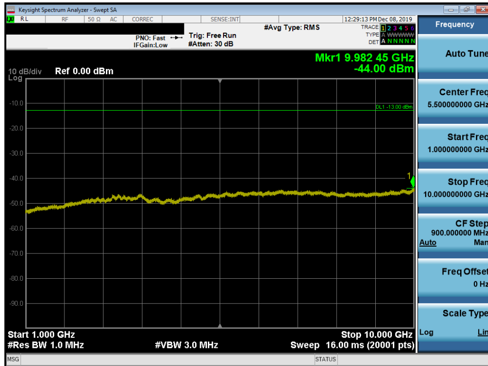
Plot 7-25. Conducted Spurious Plot (CDMA/EvDO, Ch. 476)
