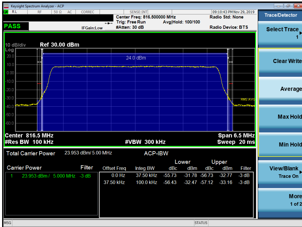
Plot 7-36. Channel Edge Plot (LTE Band 26 - 5MHz QPSK - Low Channel)
