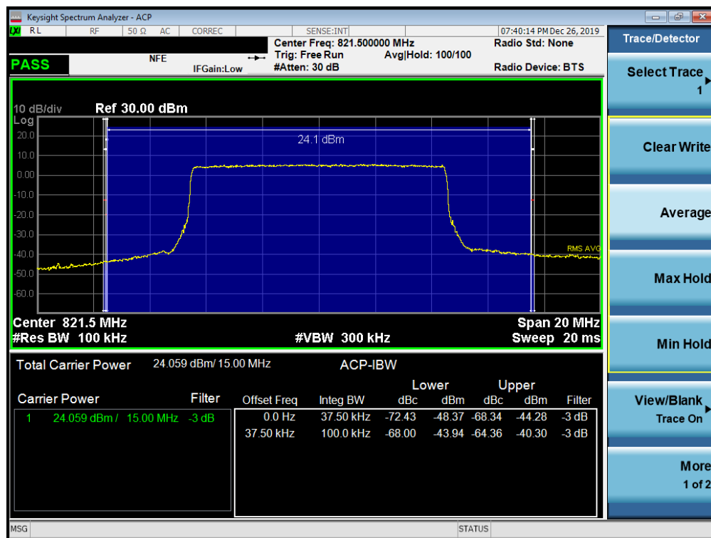
Plot 7-34. Channel Edge Plot (LTE Band 26 - 15MHz QPSK)
