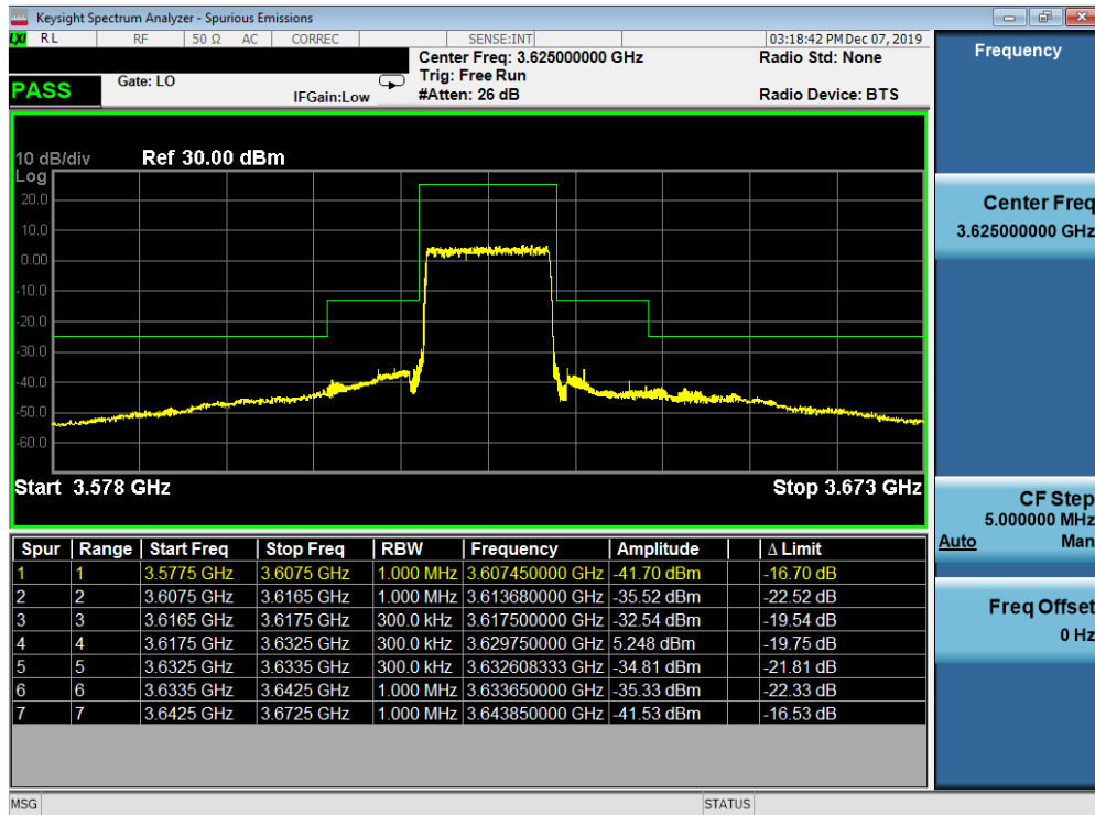
Plot 7-40. Mid ACP Plot (LTE Band 48 - 15.0MHz QPSK - Full RB Configuration)
