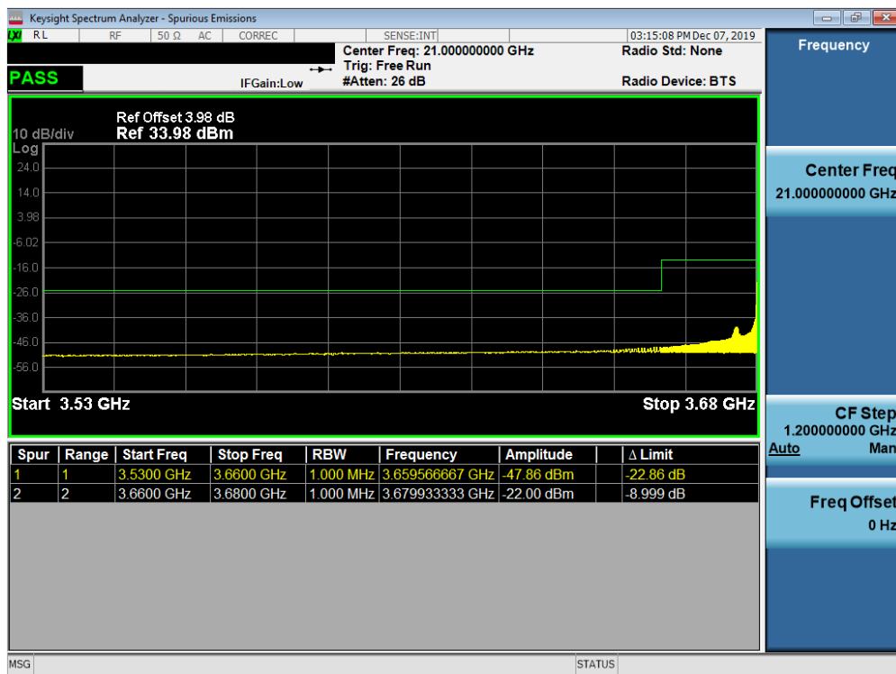
Plot 7-28. Conducted Spurious Plot (LTE Band 48 - 20.0MHz QPSK - RB Size 1, RB Offset 0 - High Channel)
