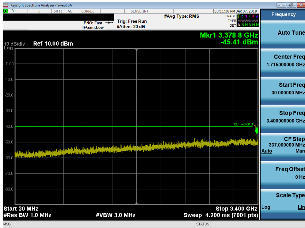
Plot 7-17. Conducted Spurious Plot (LTE Band 48 - 20.0MHz QPSK - RB Size 1, RB Offset 0 - Low Channel)
