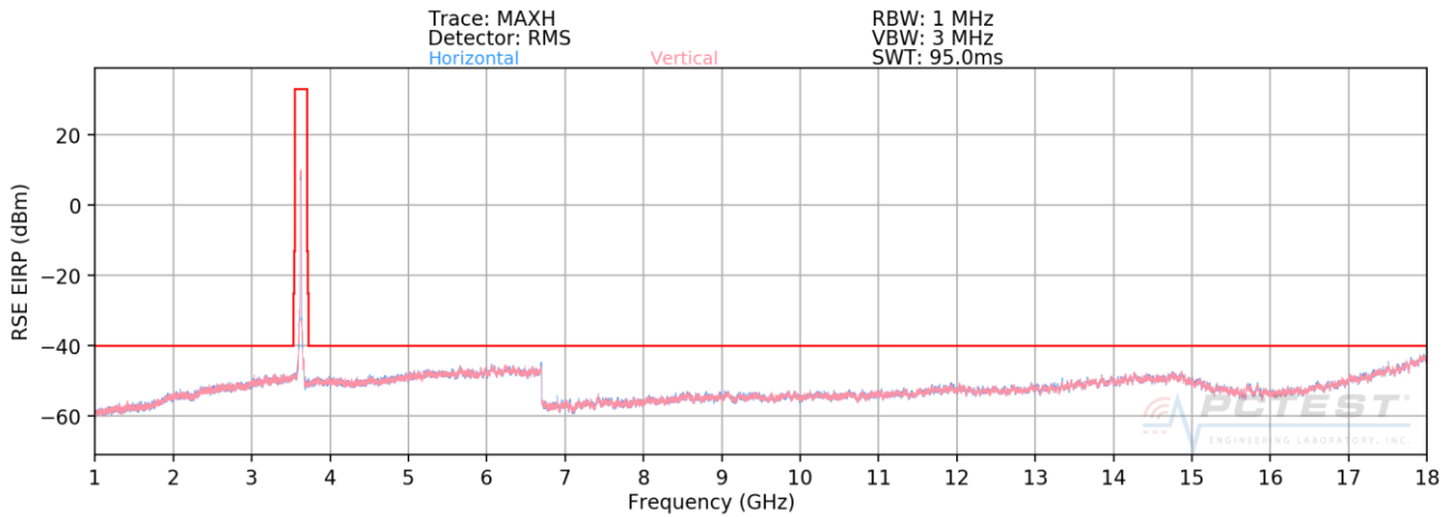
Plot 7-45. Radiated Spurious Plot 1 - 18GHz (Band 48)
