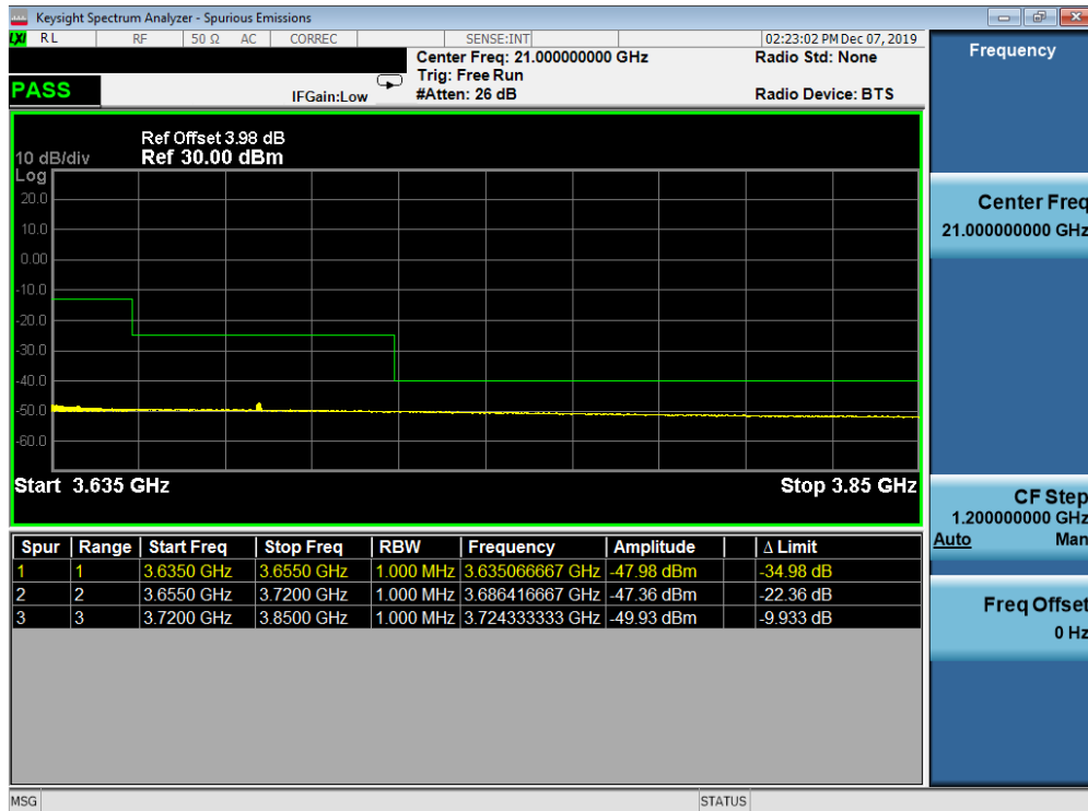
Plot 7-24. Conducted Spurious Plot (LTE Band 48 - 20.0MHz QPSK - RB Size 1, RB Offset 0 - Mid Channel)
