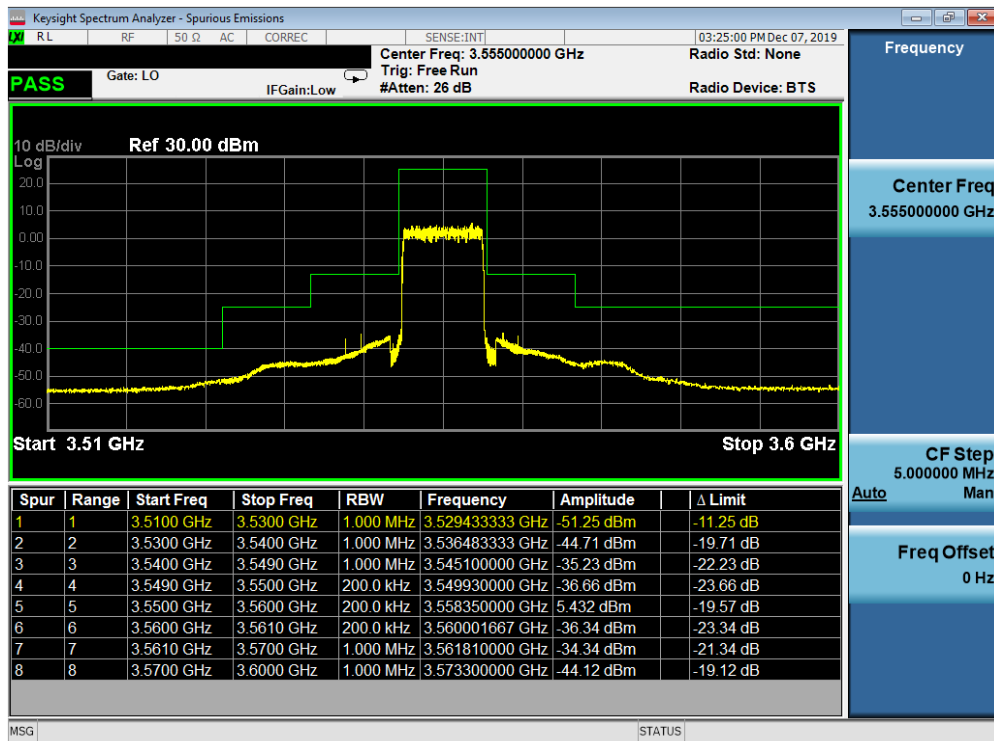
Plot 7-36. Lower ACP Plot (LTE Band 48 - 10.0MHz QPSK - Full RB Configuration)
