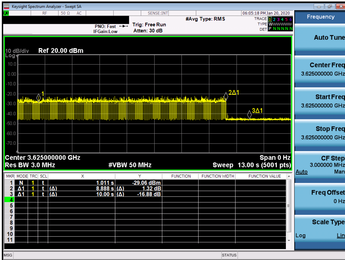
Plot 7-49. Run#1 End User Device Discontinues Operations within 10s
