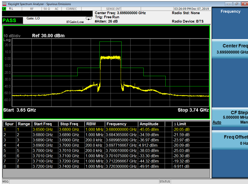
Plot 7-38. Upper ACP Plot (LTE Band 48 - 10.0MHz QPSK - Full RB Configuration)
