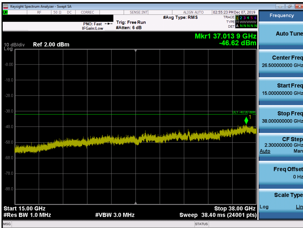
Plot 7-32. Conducted Spurious Plot (LTE Band 48 - 20.0MHz QPSK - RB Size 1, RB Offset 0 - High Channel)
