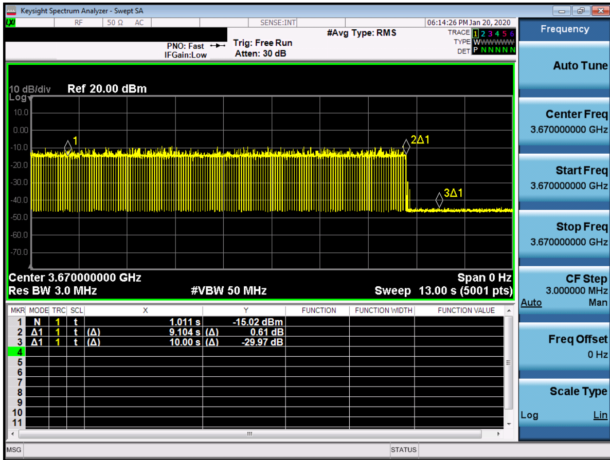
Plot 7-51. Run#2 End User Device Discontinues Operations within 10s
