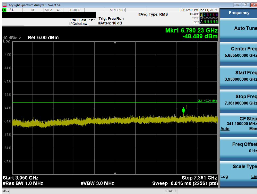
Plot 7-30. Conducted Spurious Plot (LTE Band 48 - 20.0MHz QPSK - RB Size 1, RB Offset 0 - High Channel)
