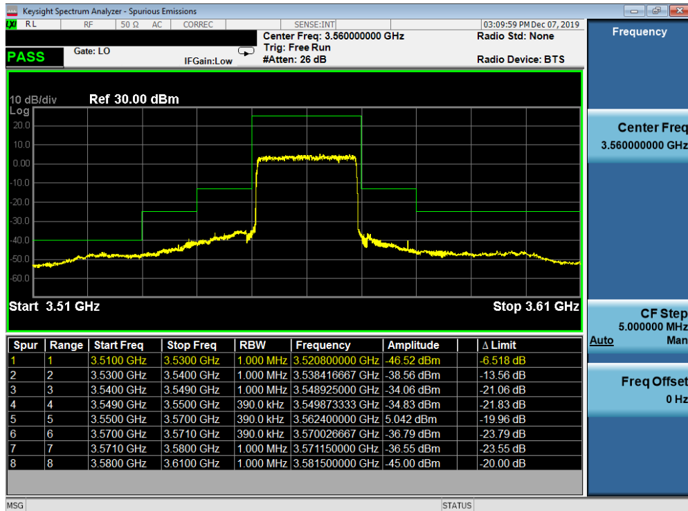
Plot 7-42. Lower ACP Plot (LTE Band 48 - 20.0MHz QPSK - Full RB Configuration)
