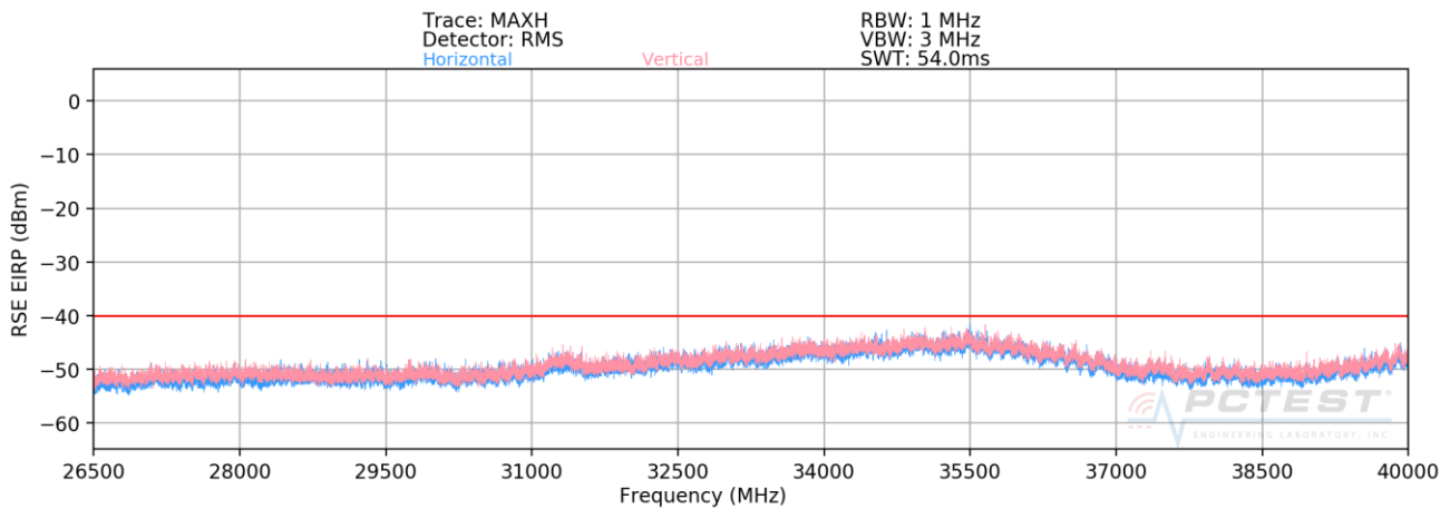
Plot 7-47. Radiated Spurious Plot 26.5 - 40GHz (Band 48)
