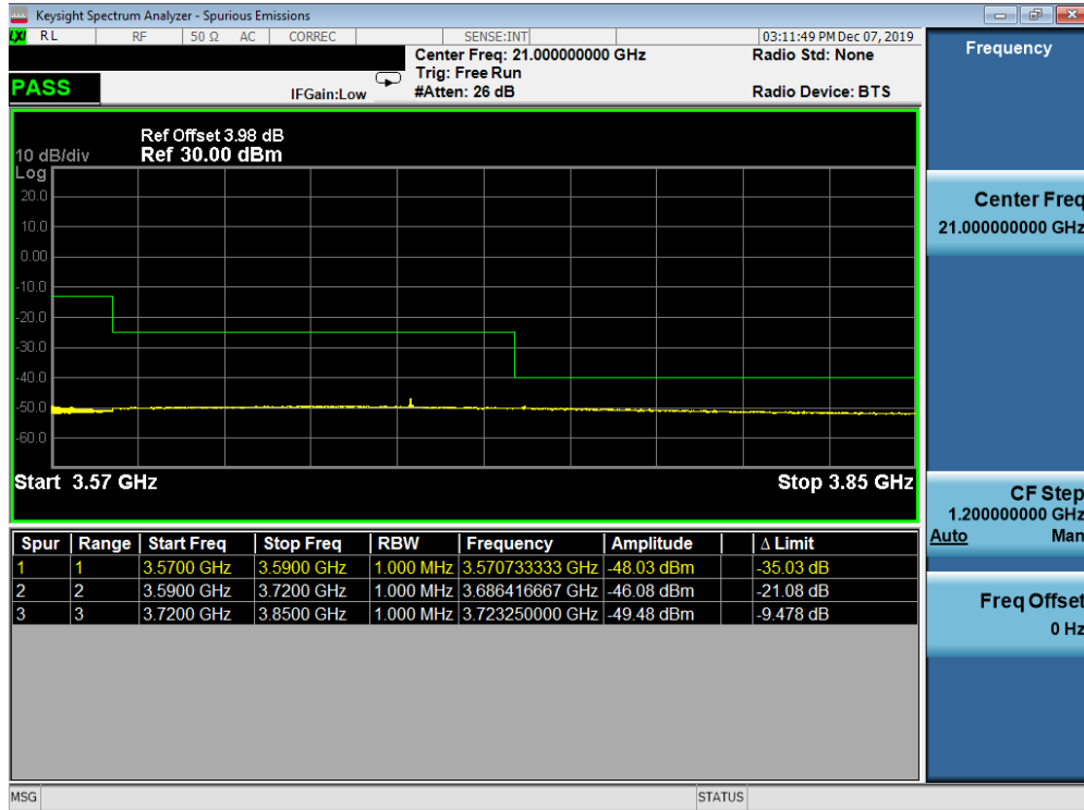
Plot 7-19. Conducted Spurious Plot (LTE Band 48 - 20.0MHz QPSK - RB Size 1, RB Offset 0 - Low Channel)
