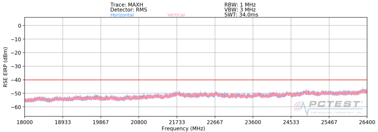
Plot 7-46. Radiated Spurious Plot 18 - 26.5GHz (Band 48)
