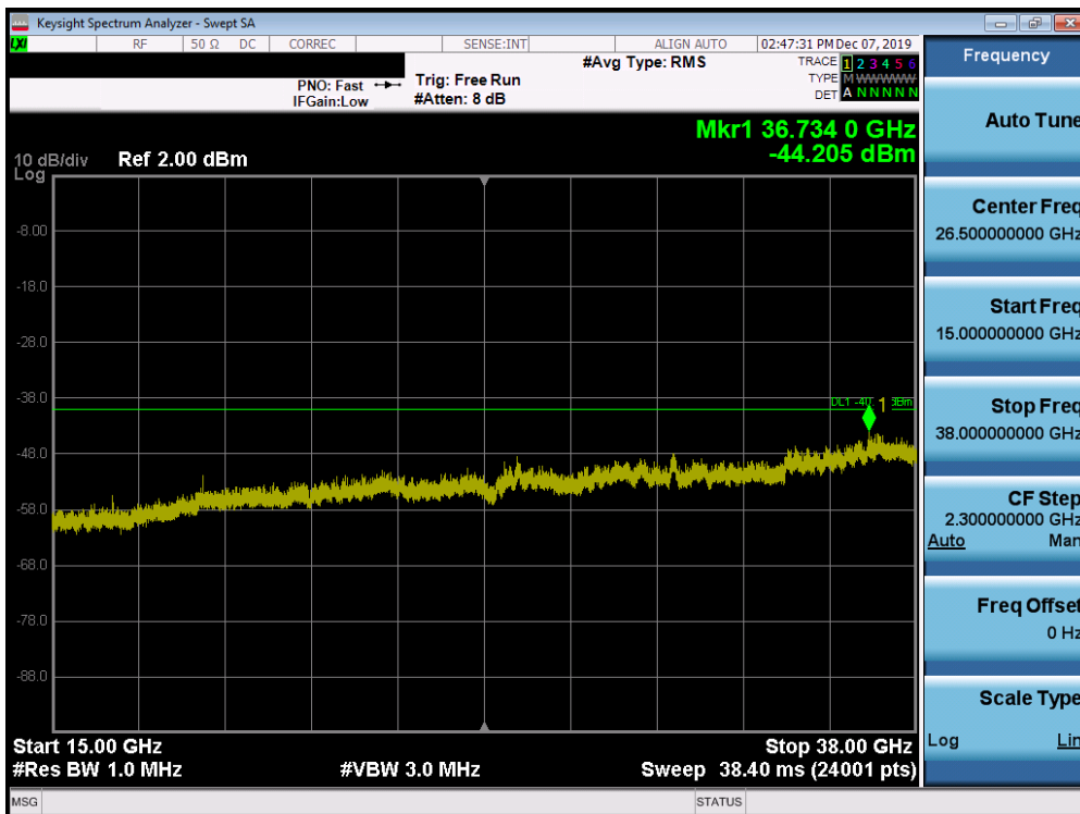
Plot 7-26. Conducted Spurious Plot (LTE Band 48 - 20.0MHz QPSK - RB Size 1, RB Offset 0 - Mid Channel)
