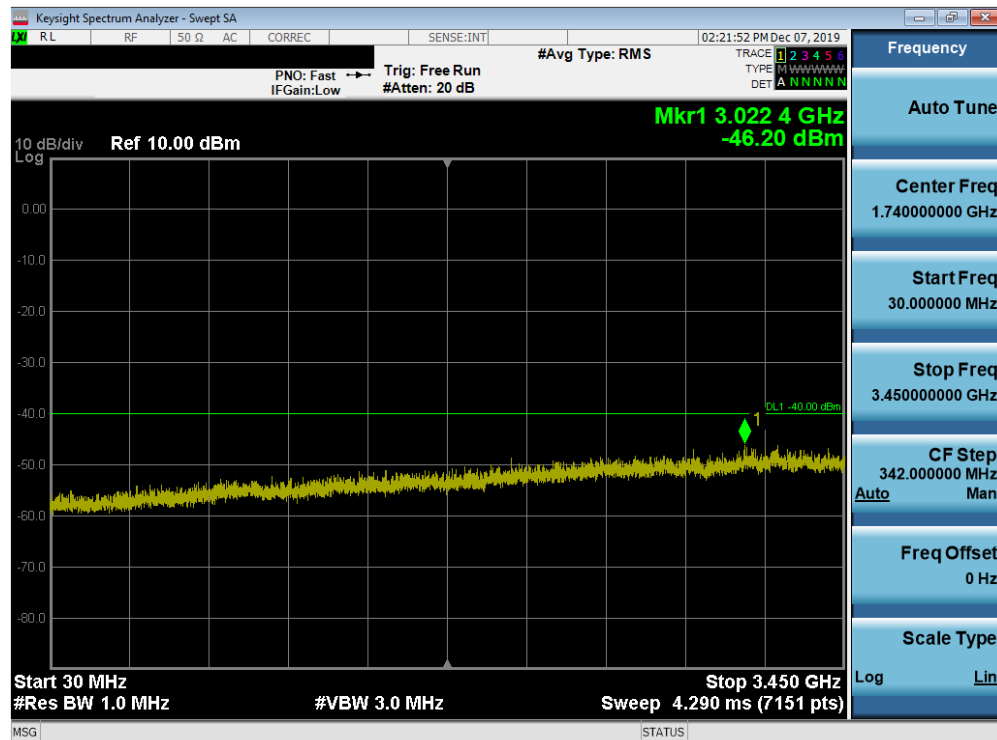
Plot 7-22. Conducted Spurious Plot (LTE Band 48 - 20.0MHz QPSK - RB Size 1, RB Offset 0 - Mid Channel)
