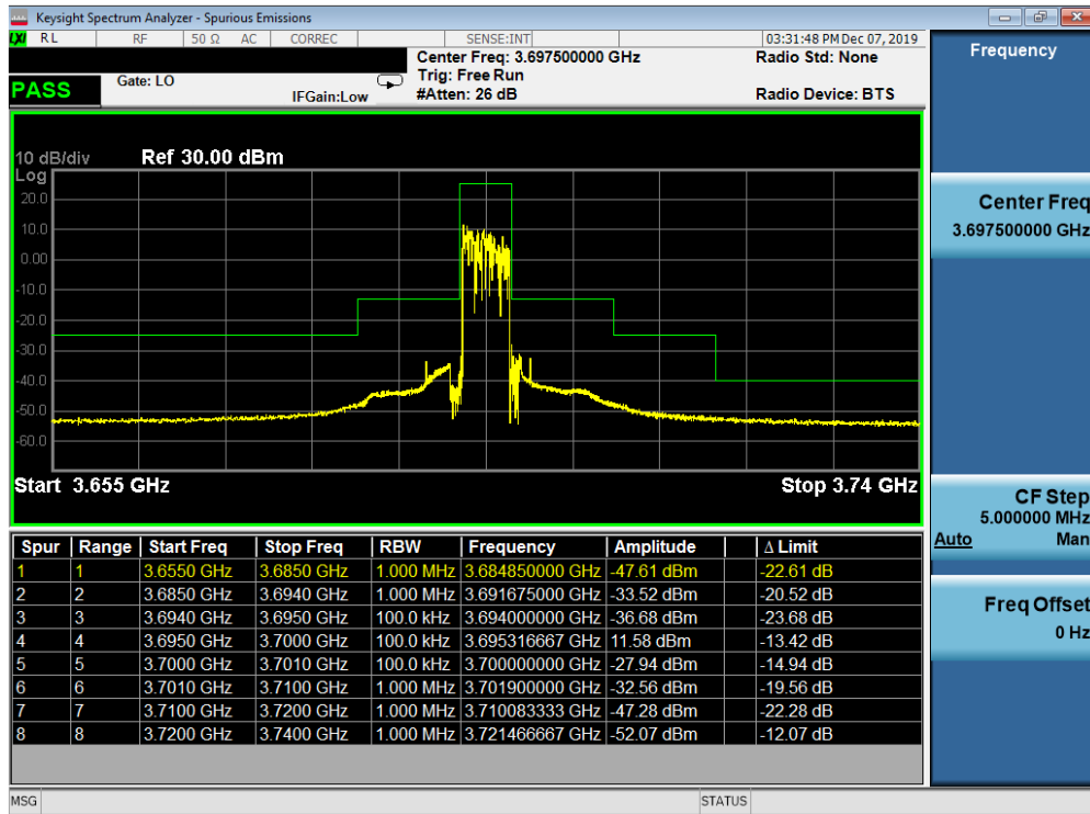
Plot 7-35. Upper ACP Plot (LTE Band 48 - 5.0MHz QPSK - Full RB Configuration)
