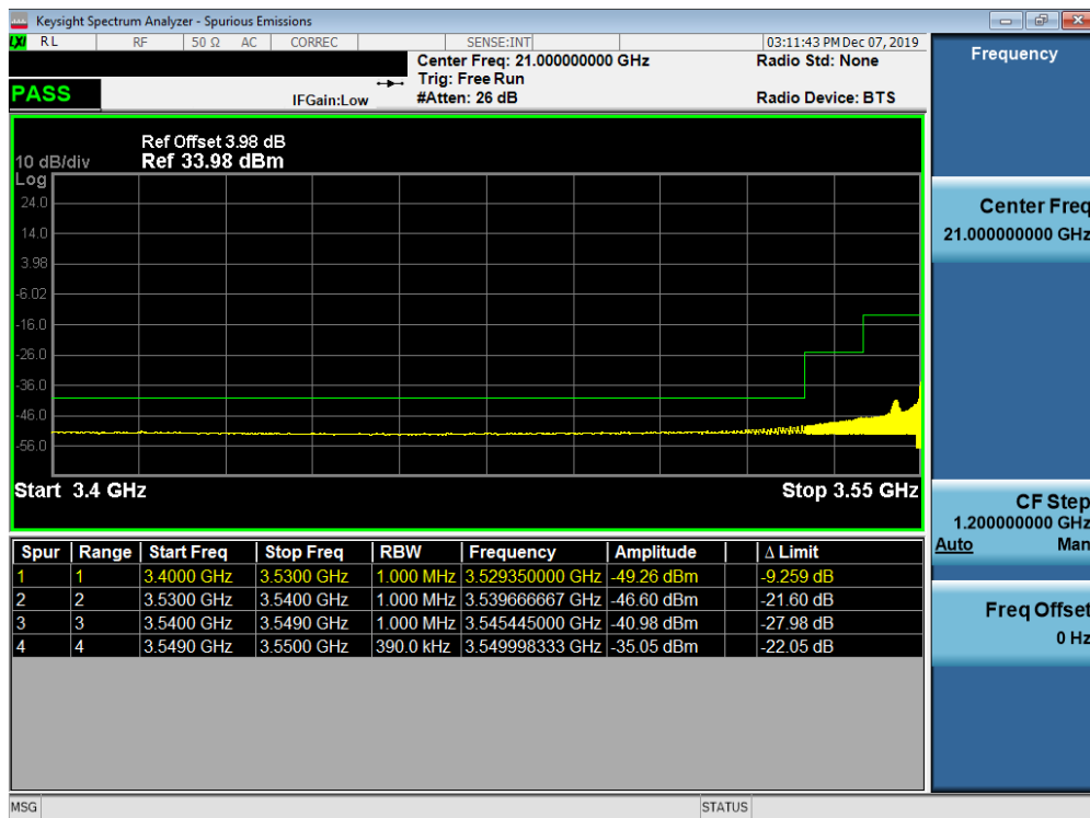
Plot 7-18. Conducted Spurious Plot (LTE Band 48 - 20.0MHz QPSK - RB Size 1, RB Offset 0 - Low Channel)
