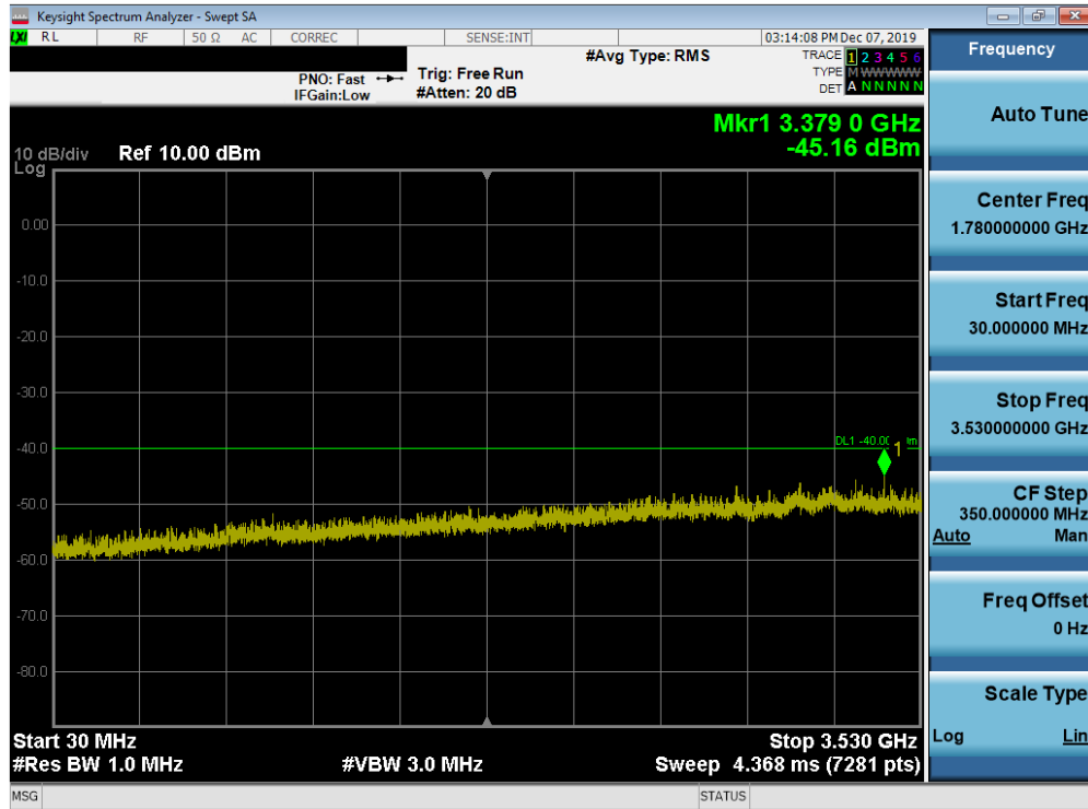
Plot 7-27. Conducted Spurious Plot (LTE Band 48 - 20.0MHz QPSK - RB Size 1, RB Offset 0 - High Channel)
