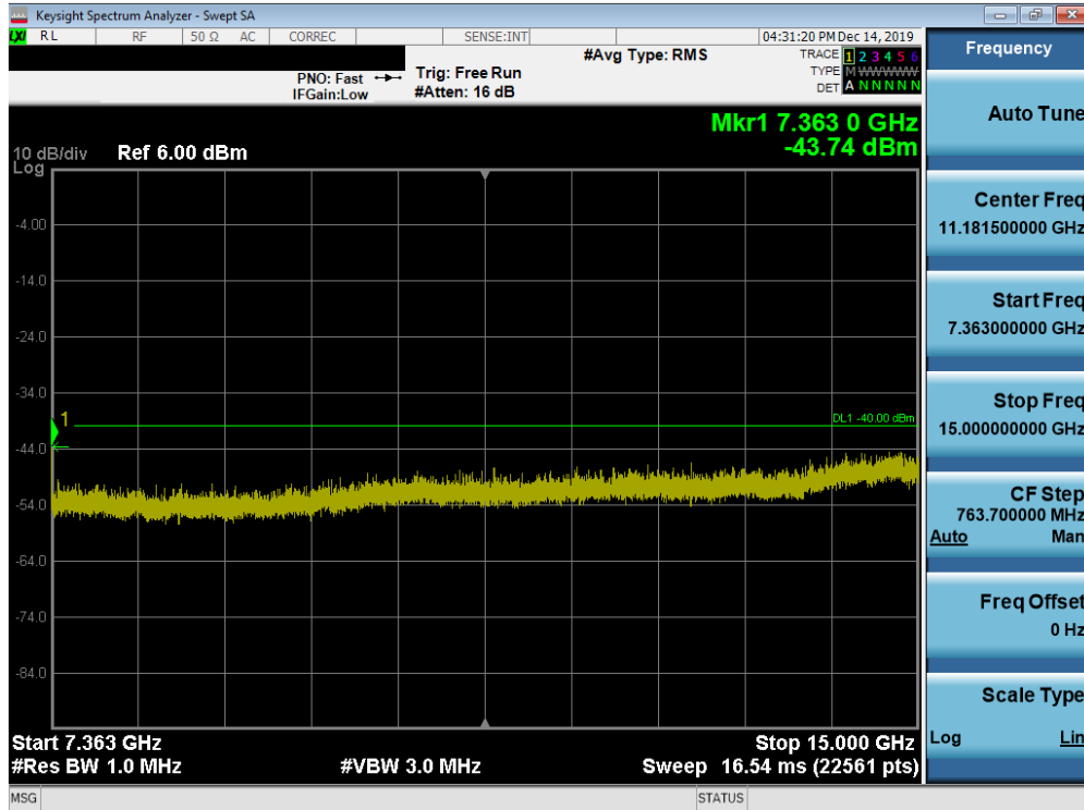
Plot 7-31. Conducted Spurious Plot (LTE Band 48 - 20.0MHz QPSK - RB Size 1, RB Offset 0 - High Channel)
