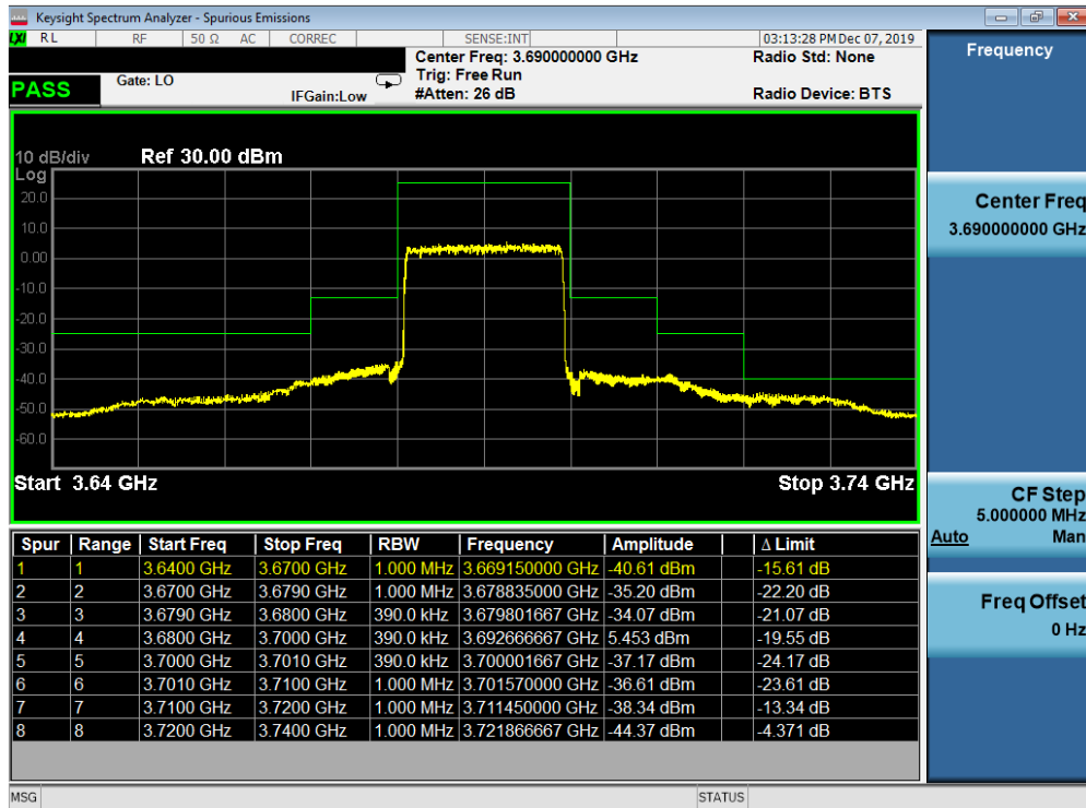
Plot 7-44. Upper ACP Plot (LTE Band 48 - 20.0MHz QPSK - Full RB Configuration)
