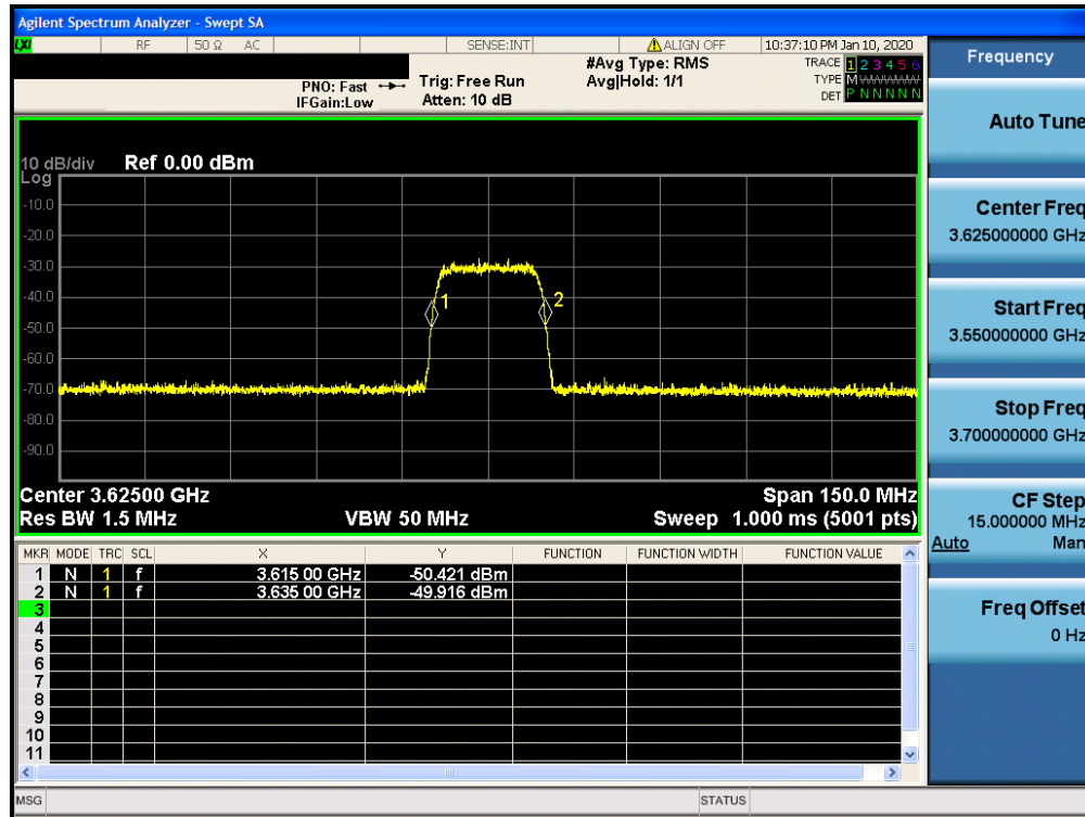
Plot 7-48. Run#1 End User Device Frequency of Operations
