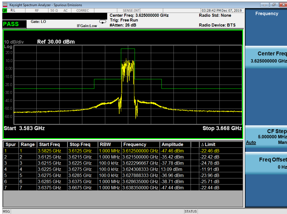
Plot 7-34. Mid ACP Plot (LTE Band 48 - 5.0MHz QPSK - Full RB Configuration)
