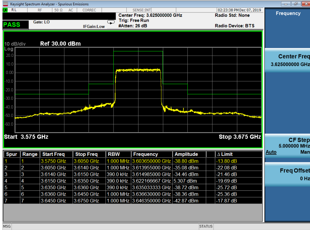
Plot 7-43. Mid ACP Plot (LTE Band 48 - 20.0MHz QPSK - Full RB Configuration)
