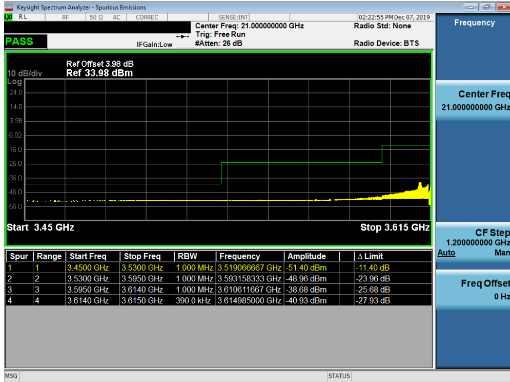
Plot 7-23. Conducted Spurious Plot (LTE Band 48 - 20.0MHz QPSK - RB Size 1, RB Offset 0 - Mid Channel)
