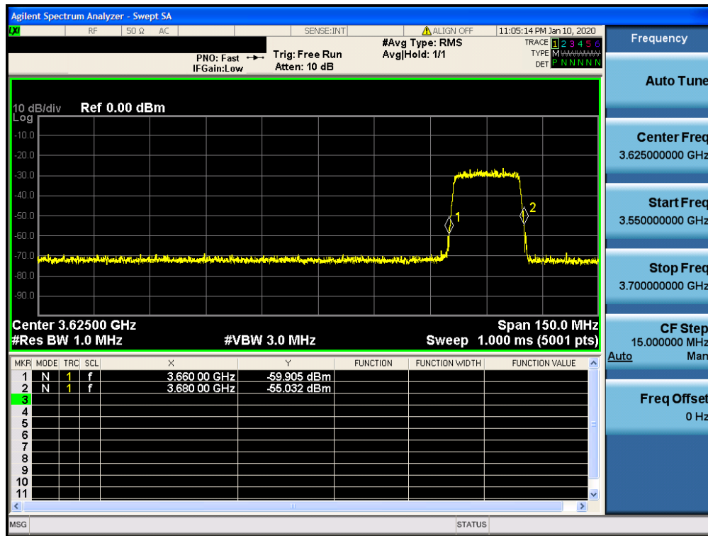
Plot 7-50. Run#2 End User Device Frequency of Operations
