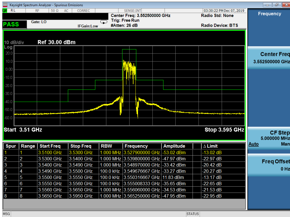
Plot 7-33. Lower ACP Plot (LTE Band 48 - 5.0MHz QPSK - Full RB Configuration)
