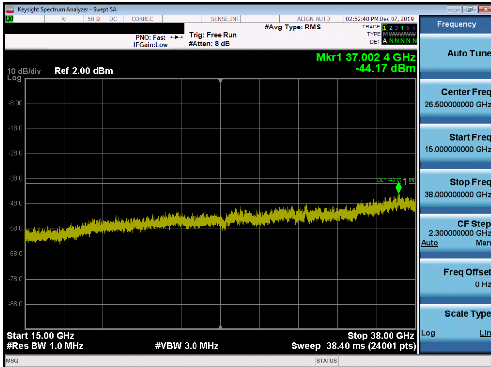
Plot 7-21. Conducted Spurious Plot (LTE Band 48 - 20.0MHz QPSK - RB Size 1, RB Offset 0 - Low Channel)
