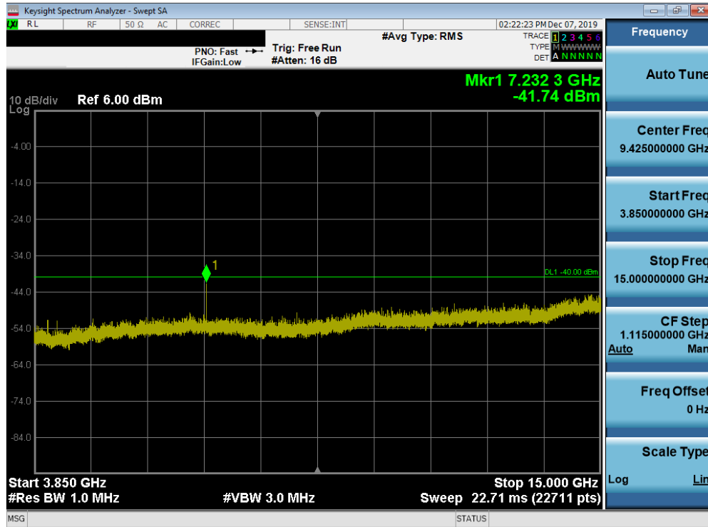
Plot 7-25. Conducted Spurious Plot (LTE Band 48 - 20.0MHz QPSK - RB Size 1, RB Offset 0 - Mid Channel)
