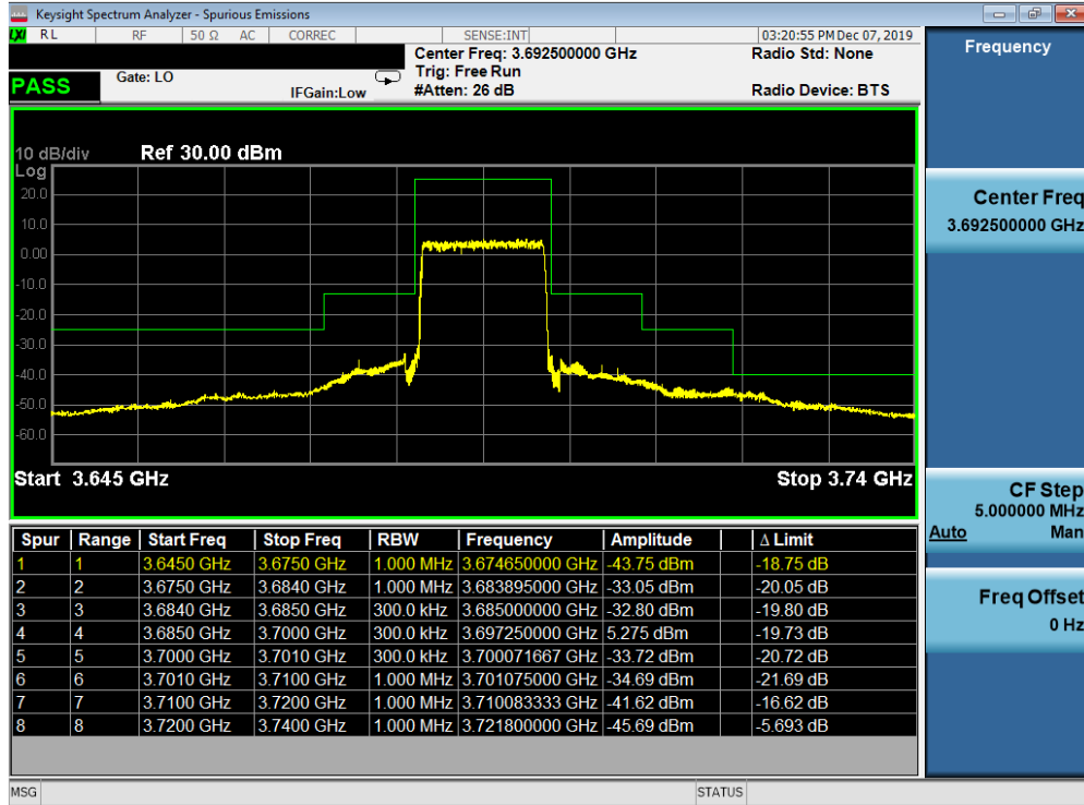
Plot 7-41. Upper ACP Plot (LTE Band 48 - 15.0MHz QPSK - Full RB Configuration)
