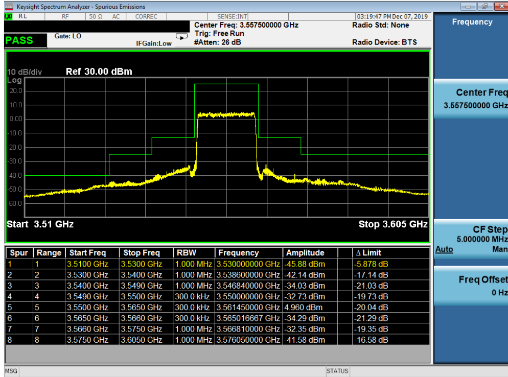
Plot 7-39. Lower ACP Plot (LTE Band 48 - 15.0MHz QPSK - Full RB Configuration)
