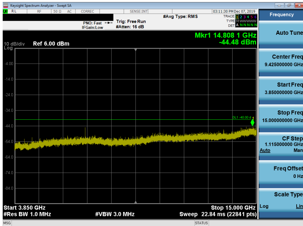
Plot 7-20. Conducted Spurious Plot (LTE Band 48 - 20.0MHz QPSK - RB Size 1, RB Offset 0 - Low Channel)
