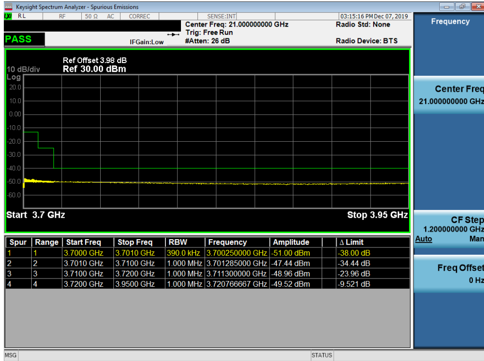
Plot 7-29. Conducted Spurious Plot (LTE Band 48 - 20.0MHz QPSK - RB Size 1, RB Offset 0 - High Channel)
