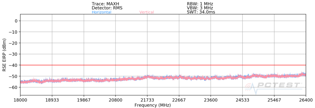
Plot 7-2. Radiated Spurious Plot 18 - 26.5GHz (Band 48)
