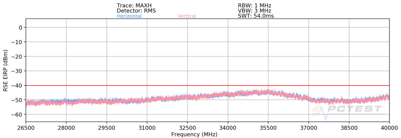
Plot 7-3. Radiated Spurious Plot 26.5 - 40GHz (Band 48)
