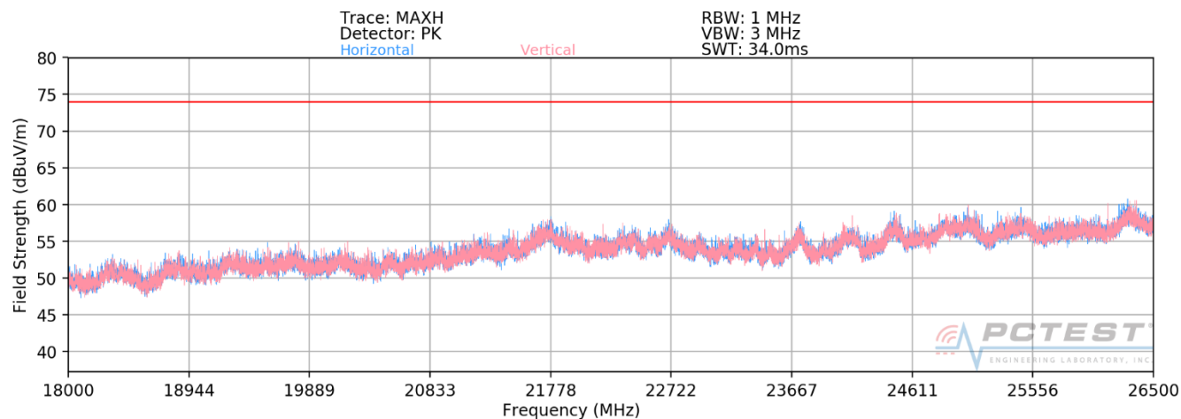
Plot 7-185. Radiated Spurious Plot 18GHz - 26.5GHz SISO ANT2 (802.11ax – 242 Tones)
