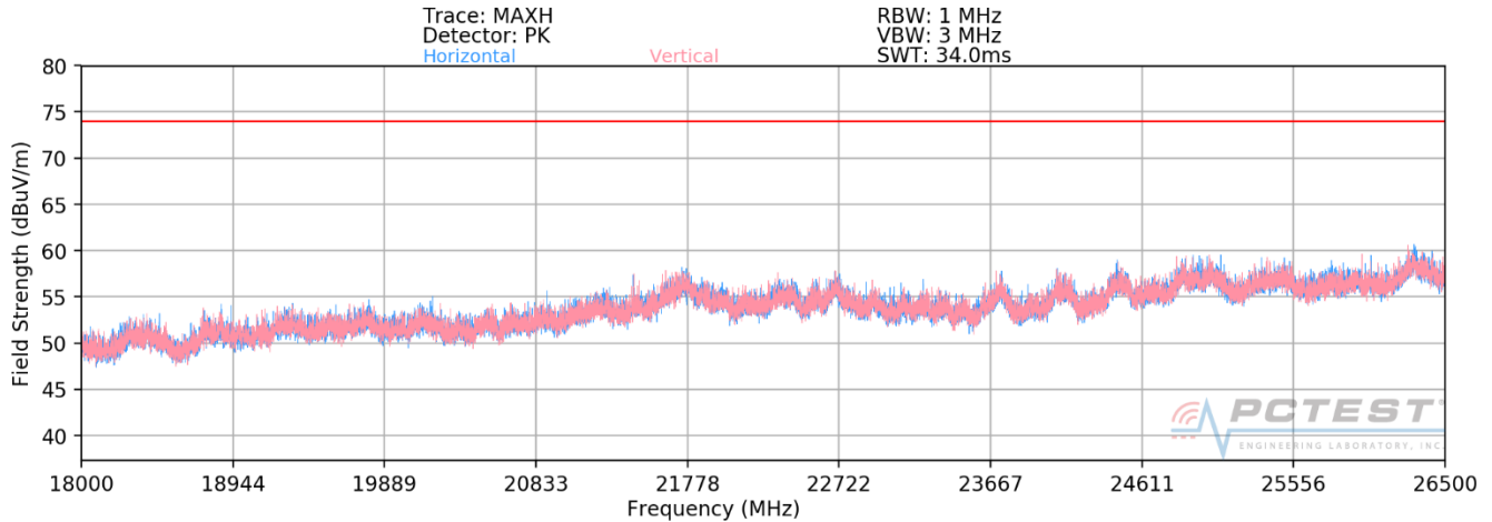
Plot 7-179. Radiated Spurious Plot 18GHz - 26.5GHz SISO ANT2 (802.11ax – 26 Tones)
