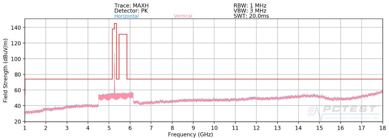
Plot 7-188. Radiated Spurious Plot above 1GHz MIMO (802.11ax – U2A Ch. 56 – 26 Tones)
