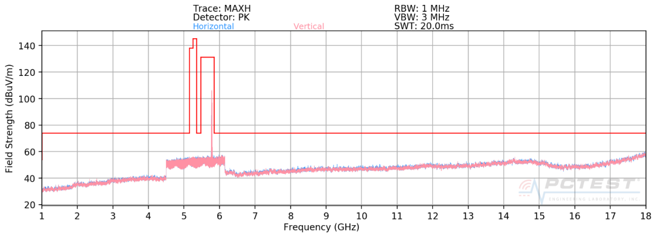
Plot 7-190. Radiated Spurious Plot above 1GHz MIMO (802.11ax – U3 Ch. 157 – 26 Tones)
