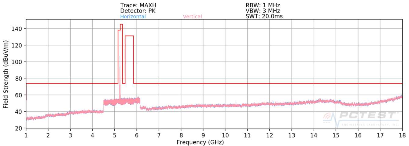
Plot 7-187. Radiated Spurious Plot above 1GHz MIMO (802.11ax – U1 Ch. 40 – 26 Tones)
