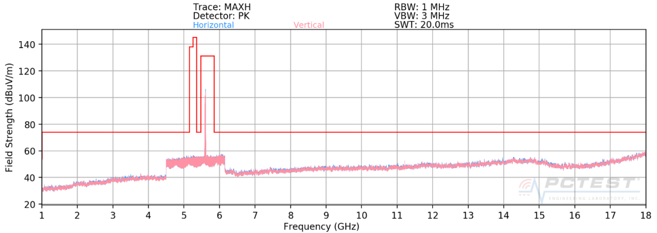
Plot 7-189. Radiated Spurious Plot above 1GHz MIMO (802.11ax – U2C Ch. 120 – 26 Tones)
