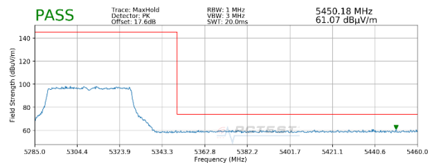
Plot 7-89. Radiated Upper Band Edge Plot MIMO (Peak – UNII Band 2A – 484 Tones)
