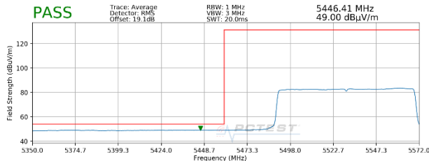
Plot 7-76. Radiated Lower Band Edge Plot SISO ANT2 (Average – UNII Band 2C – 996 Tones)
