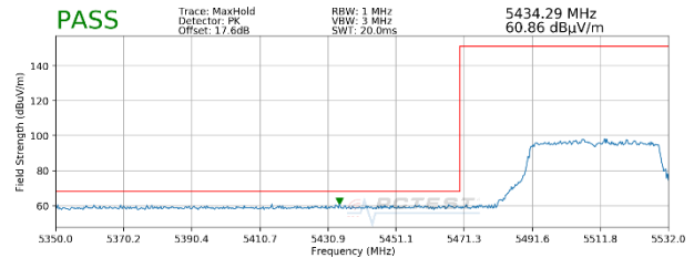
Plot 7-70. Radiated Lower Band Edge Plot SISO ANT2 (Peak – UNII Band 2C – 484 Tones)
