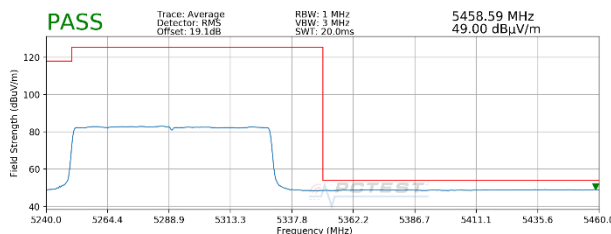
Plot 7-74. Radiated Upper Band Edge Plot SISO ANT2 (Average – UNII Band 2A – 996 Tones)
