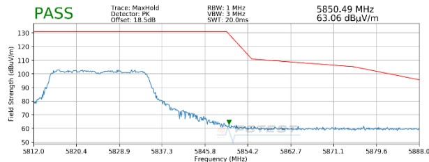
Plot 7-85. Radiated Upper Band Edge Plot MIMO (Peak – UNII Band 3 – 242 Tones)
