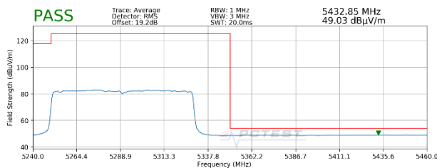
Plot 7-95. Radiated Upper Band Edge Plot MIMO (Average – UNII Band 2A – 996 Tones)
