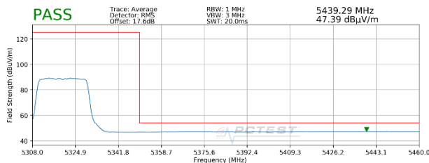
Plot 7-81. Radiated Upper Band Edge Plot MIMO (Average – UNII Band 2A – 242 Tones)
