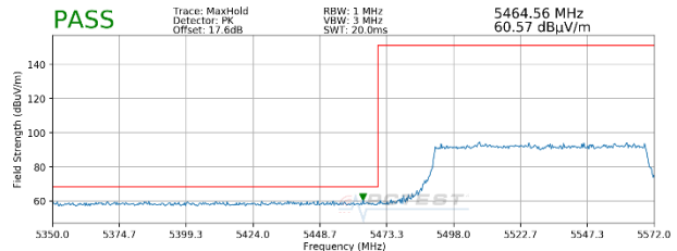
Plot 7-77. Radiated Lower Band Edge Plot SISO ANT2 (Peak – UNII Band 2C – 996 Tones)
