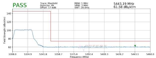
Plot 7-82. Radiated Upper Band Edge Plot MIMO (Peak – UNII Band 2A – 242 Tones)
