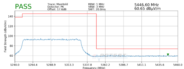
Plot 7-75. Radiated Upper Band Edge Plot SISO ANT2 (Peak – UNII Band 2A – 996 Tones)
