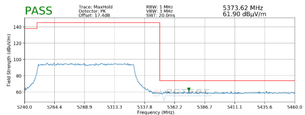
Plot 7-96. Radiated Upper Band Edge Plot MIMO (Peak – UNII Band 2A – 996 Tones)
