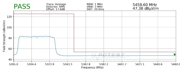
Plot 7-88. Radiated Upper Band Edge Plot MIMO (Average – UNII Band 2A – 484 Tones)
