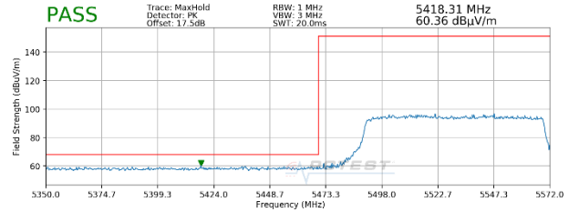
Plot 7-98. Radiated Lower Band Edge Plot MIMO (Peak - UNII Band 2C - 996 Tones)
