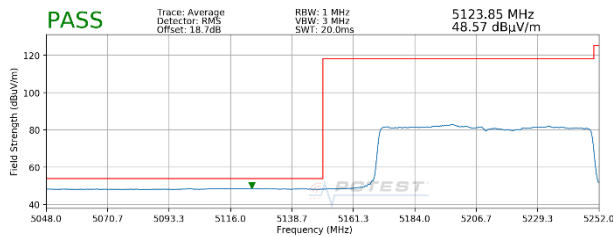
Plot 7-93. Radiated Lower Band Edge Plot MIMO (Average – UNII Band 1 – 996 Tones)
