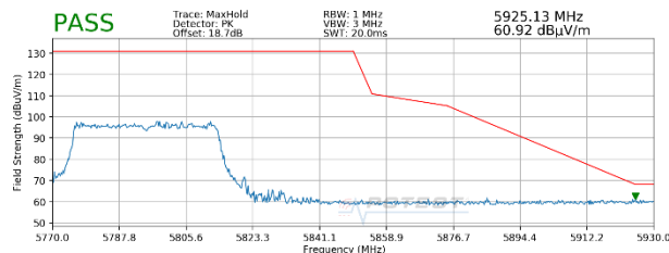
Plot 7-71. Radiated Upper Band Edge Plot SISO ANT2 (Peak – UNII Band 3 – 484 Tones)
