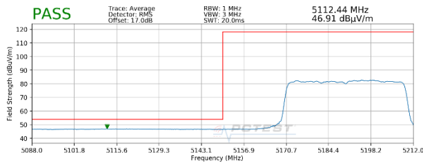
Plot 7-86. Radiated Lower Band Edge Plot MIMO (Average – UNII Band 1 – 484 Tones)
