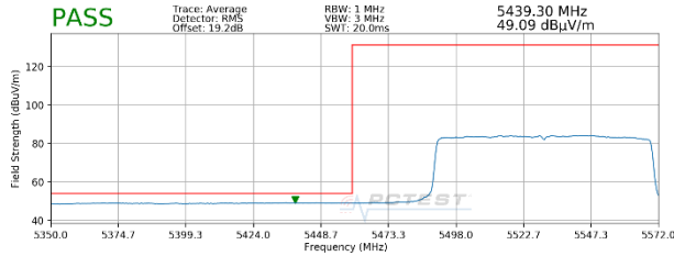
Plot 7-97. Radiated Lower Band Edge Plot MIMO (Average - UNII Band 2C - 996 Tones)
