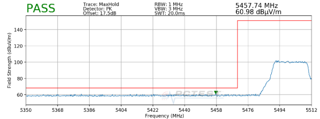
Plot 7-84. Radiated Lower Band Edge Plot MIMO (Peak – UNII Band 2C – 242 Tones)
