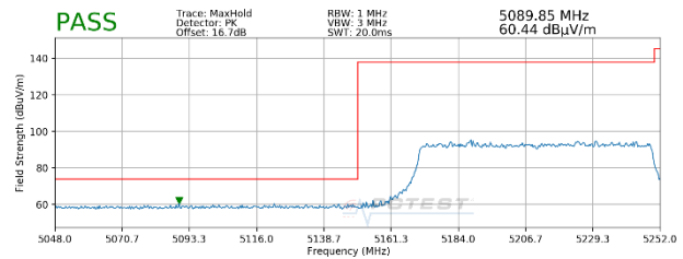
Plot 7-73. Radiated Lower Band Edge Plot SISO ANT2 (Peak – UNII Band 1 – 996 Tones)
