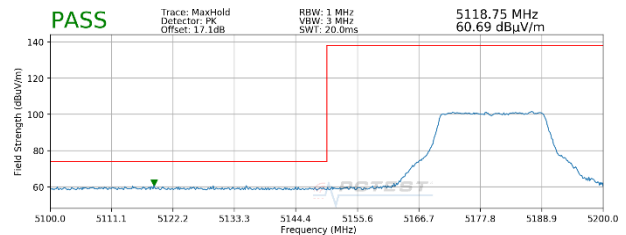
Plot 7-80. Radiated Lower Band Edge Plot MIMO (Peak – UNII Band 1 – 242 Tones)
