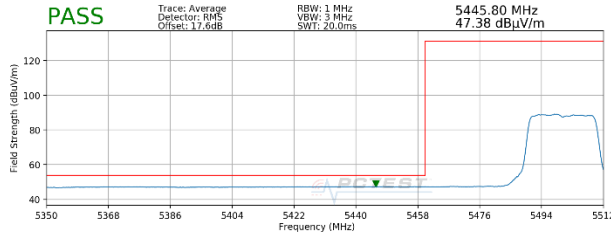
Plot 7-83. Radiated Lower Band Edge Plot MIMO (Average – UNII Band 2C – 242 Tones)
