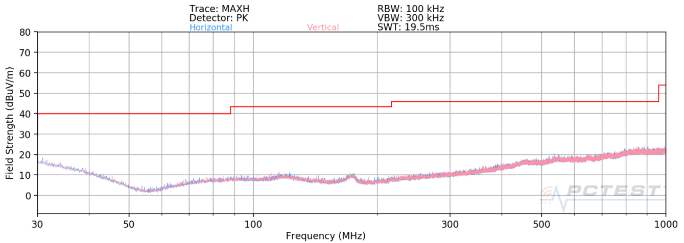
Plot 7-100. Radiated Spurious Plot below 1GHz MIMO (802.11ax – 26 Tones – U3 Ch. 157)
