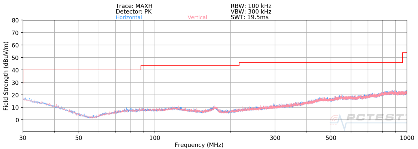
Plot 7-101. Radiated Spurious Plot below 1GHz MIMO (802.11ax – 242 Tones – U3 Ch. 157)
