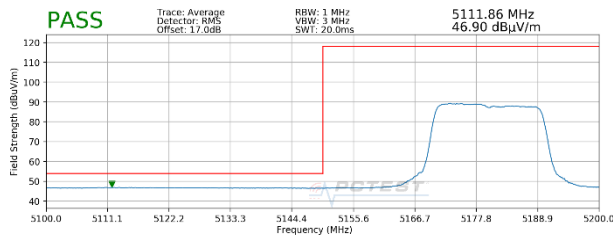
Plot 7-79. Radiated Lower Band Edge Plot MIMO (Average – UNII Band 1 – 242 Tones)
