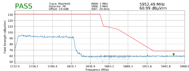
Plot 7-78. Radiated Upper Band Edge Plot SISO ANT2 (Peak – UNII Band 3 – 996 Tones)
