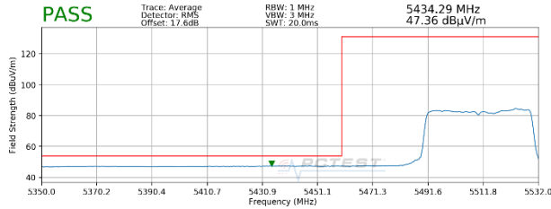
Plot 7-90. Radiated Lower Band Edge Plot MIMO (Average - UNII Band 2C - 484 Tones)
