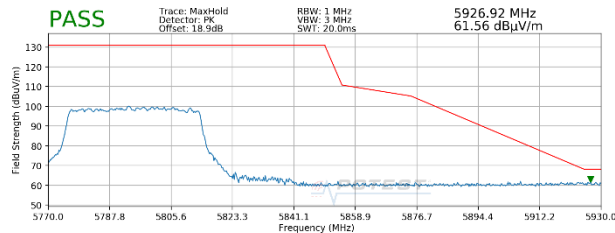
Plot 7-92. Radiated Upper Band Edge Plot MIMO (Peak - UNII Band 3 - 484 Tones)
