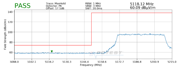
Plot 7-87. Radiated Lower Band Edge Plot MIMO (Peak – UNII Band 1 – 484 Tones)
