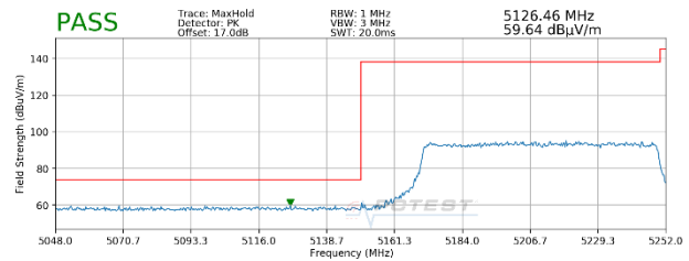
Plot 7-94. Radiated Lower Band Edge Plot MIMO (Peak – UNII Band 1 – 996 Tones)
