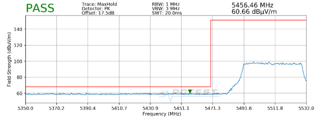
Plot 7-91. Radiated Lower Band Edge Plot MIMO (Peak - UNII Band 2C - 484 Tones)
