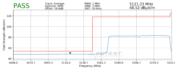
Plot 7-72. Radiated Lower Band Edge Plot SISO ANT2 (Average – UNII Band 1 – 996 Tones)
