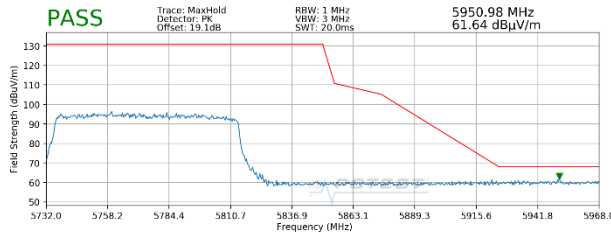
Plot 7-99. Radiated Upper Band Edge Plot MIMO (Peak - UNII Band 3 - 996 Tones)
