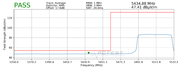
Plot 7-69. Radiated Lower Band Edge Plot SISO ANT2 (Average – UNII Band 2C – 484 Tones)
