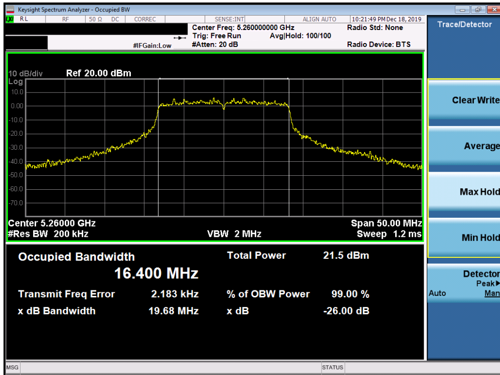
Plot 7-88. 26dB Bandwidth Plot SISO ANT2 (802.11a (UNII Band 2A) – Ch. 52)
