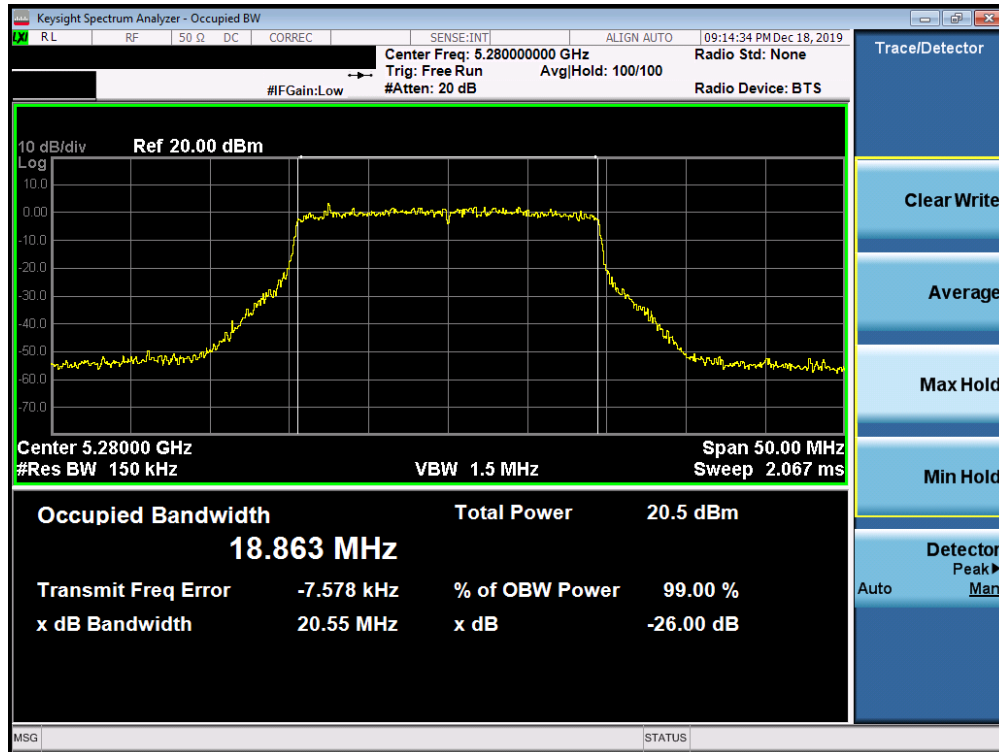
Plot 7-31. 26dB Bandwidth Plot SISO ANT1 (20MHz BW 802.11ax (UNII Band 2A) – Ch. 56)
