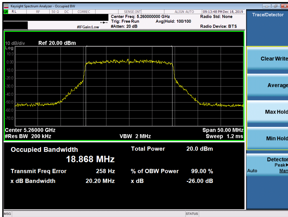
Plot 7-30. 26dB Bandwidth Plot SISO ANT1 (20MHz BW 802.11ax (UNII Band 2A) – Ch. 52)
