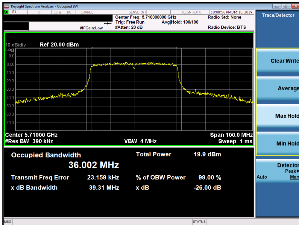
Plot 7-58. 26dB Bandwidth Plot SISO ANT1 (40MHz BW 802.11ac (UNII Band 2C) – Ch. 142)
