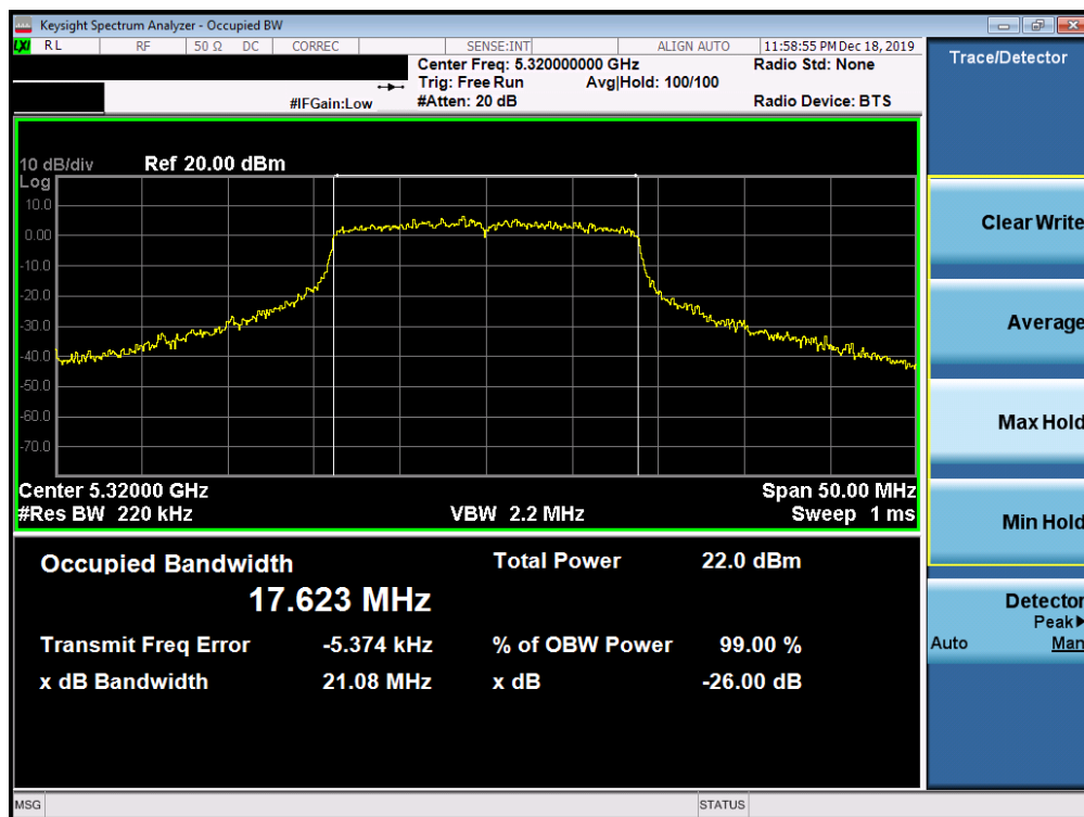
Plot 7-96. 26dB Bandwidth Plot SISO ANT2 (20MHz BW 802.11ac (UNII Band 2A) – Ch. 64)
