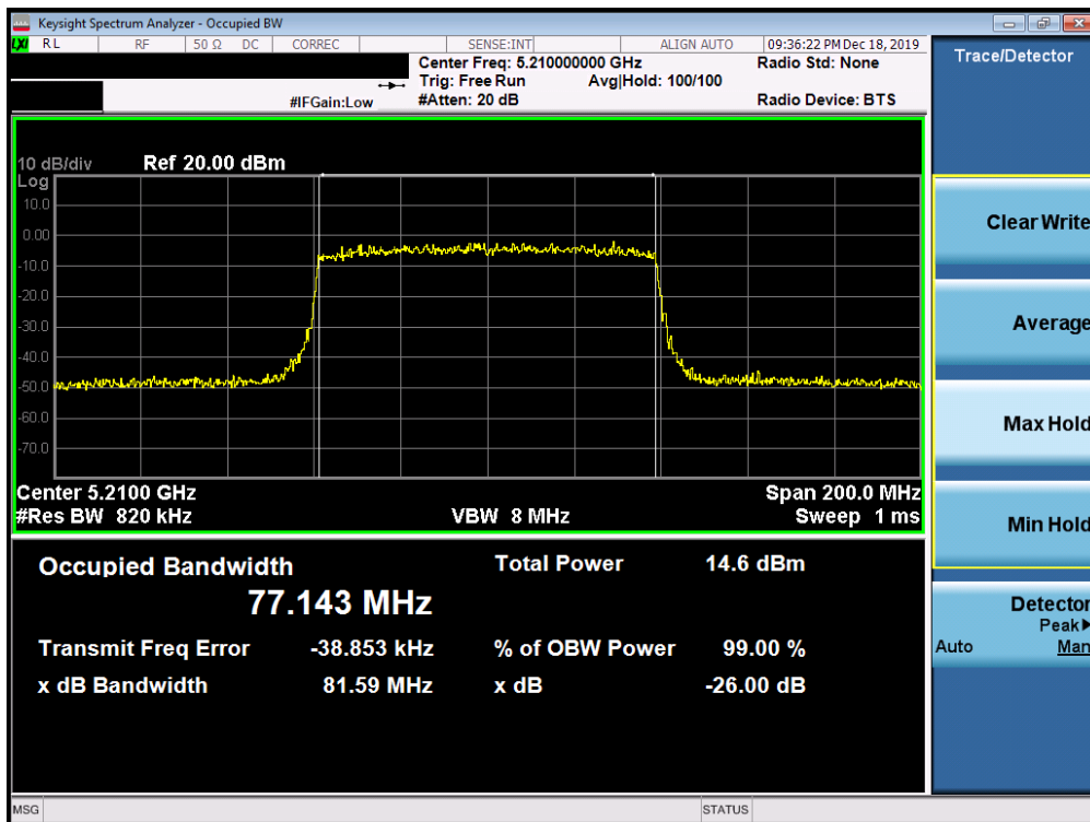
Plot 7-20. 26dB Bandwidth Plot SISO ANT1 (80MHz BW 802.11ax (UNII Band 1) – Ch. 42)
