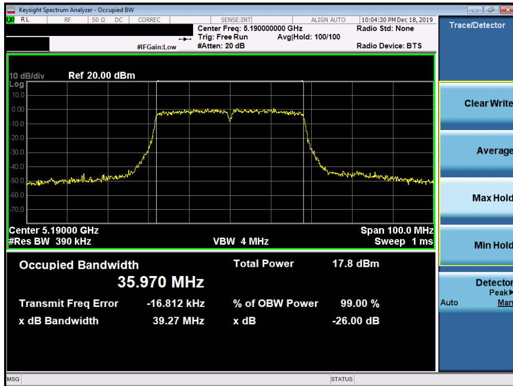
Plot 7-15. 26dB Bandwidth Plot SISO ANT1 (40MHz BW 802.11ac (UNII Band 1) – Ch. 38)
