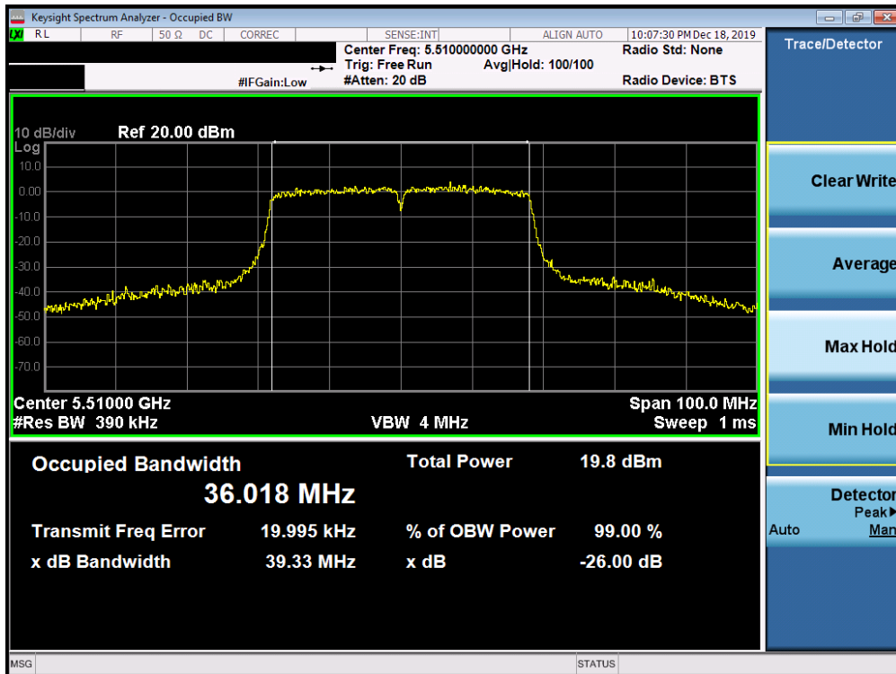
Plot 7-56. 26dB Bandwidth Plot SISO ANT1 (40MHz BW 802.11ac (UNII Band 2C) – Ch. 102)
