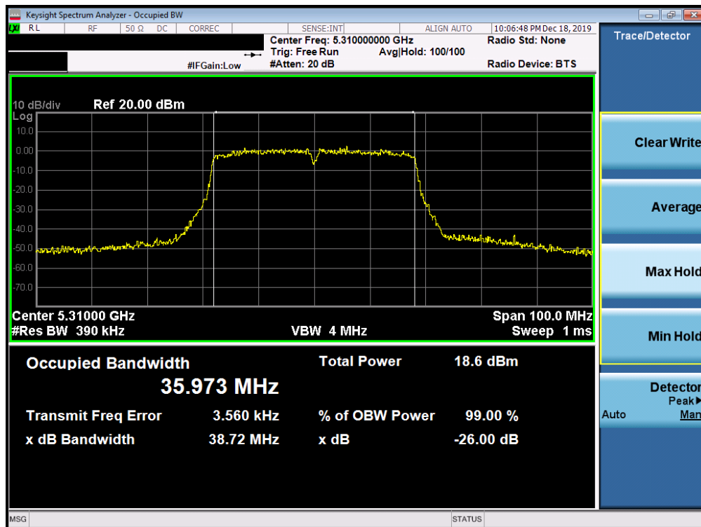
Plot 7-36. 26dB Bandwidth Plot SISO ANT1 (40MHz BW 802.11ac (UNII Band 2A) – Ch. 62)
