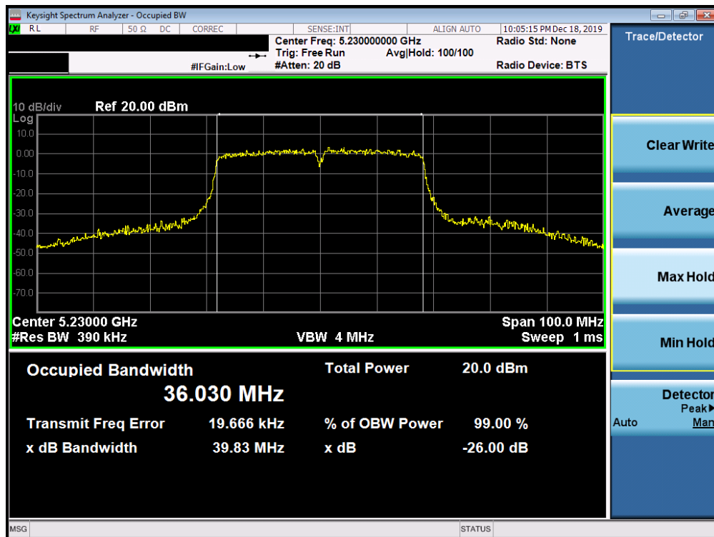
Plot 7-16. 26dB Bandwidth Plot SISO ANT1 (40MHz BW 802.11ac (UNII Band 1) – Ch. 46)
