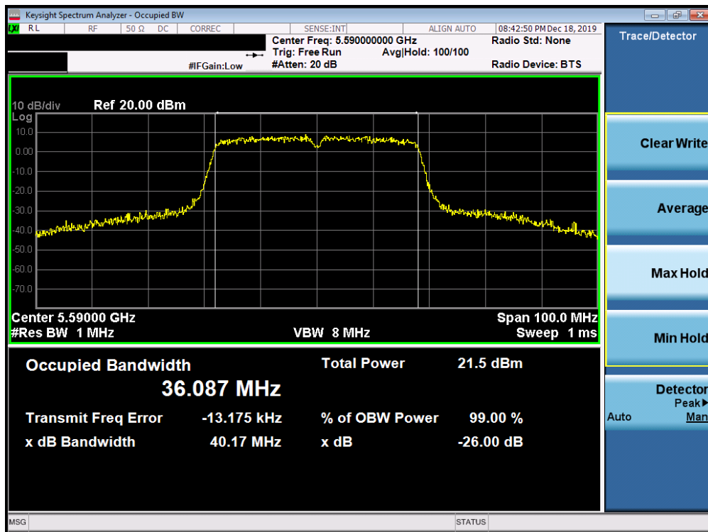
Plot 7-54. 26dB Bandwidth Plot SISO ANT1 (40MHz BW 802.11n (UNII Band 2C) – Ch. 118)
