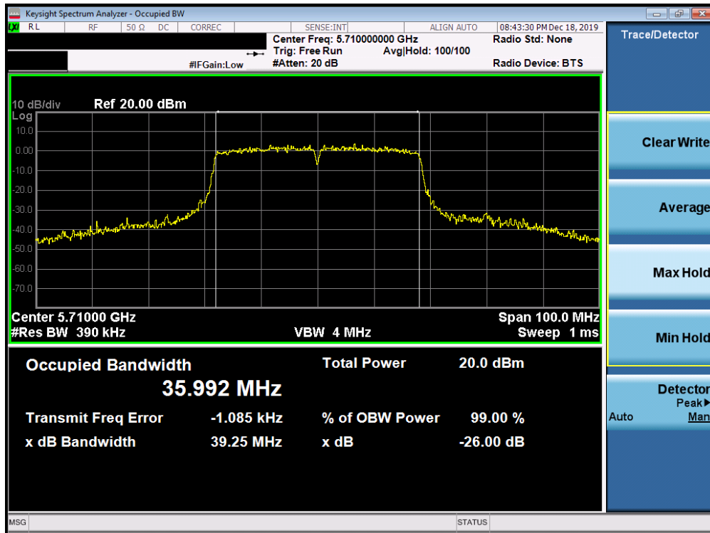
Plot 7-55. 26dB Bandwidth Plot SISO ANT1 (40MHz BW 802.11n (UNII Band 2C) – Ch. 142)
