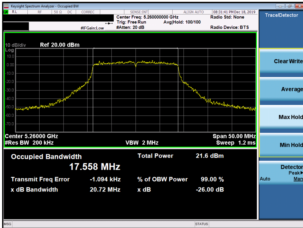
Plot 7-24. 26dB Bandwidth Plot SISO ANT1 (20MHz BW 802.11n (UNII Band 2A) – Ch. 52)
