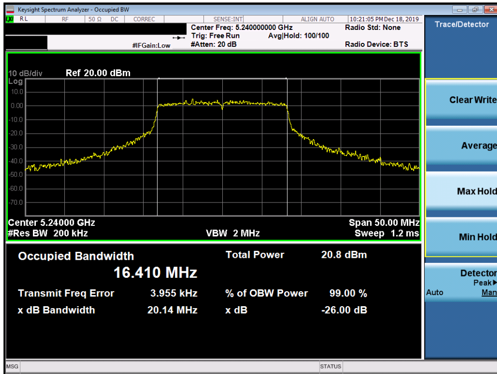
Plot 7-70. 26dB Bandwidth Plot SISO ANT2 (802.11a (UNII Band 1) – Ch. 48)
