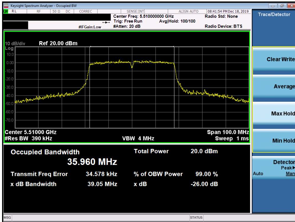
Plot 7-53. 26dB Bandwidth Plot SISO ANT1 (40MHz BW 802.11n (UNII Band 2C) – Ch. 102)
