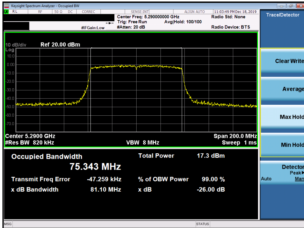
Plot 7-106. 26dB Bandwidth Plot SISO ANT2 (80MHz BW 802.11ac (UNII Band 2A) – Ch. 58)
