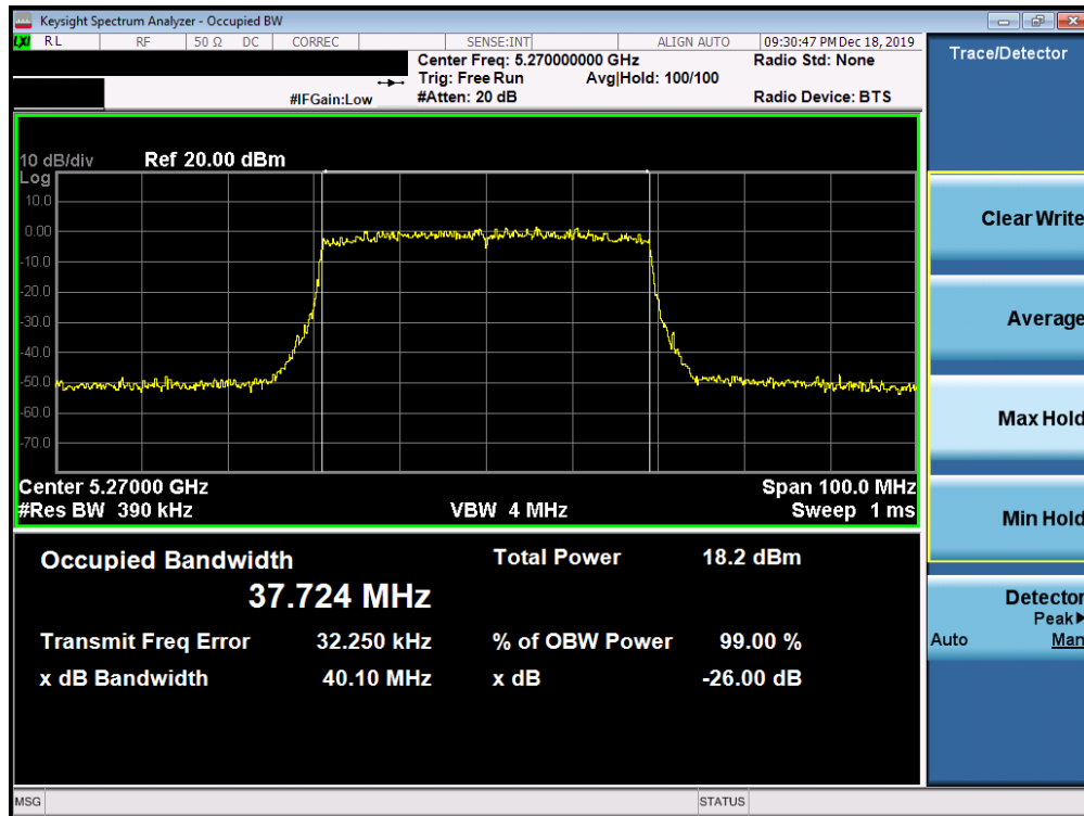
Plot 7-37. 26dB Bandwidth Plot SISO ANT1 (40MHz BW 802.11ax (UNII Band 2A) – Ch. 54)
