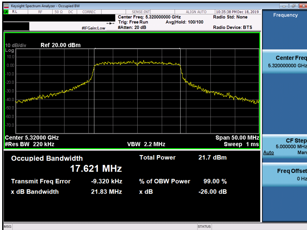
Plot 7-93. 26dB Bandwidth Plot SISO ANT2 (20MHz BW 802.11n (UNII Band 2A) – Ch. 64)
