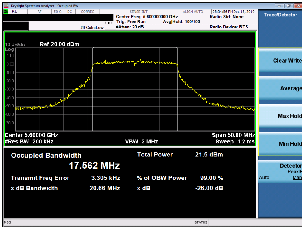
Plot 7-45. 26dB Bandwidth Plot SISO ANT1 (20MHz BW 802.11n (UNII Band 2C) – Ch. 120)
