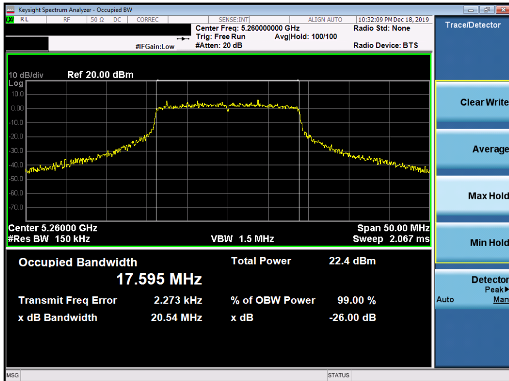
Plot 7-91. 26dB Bandwidth Plot SISO ANT2 (20MHz BW 802.11n (UNII Band 2A) – Ch. 52)
