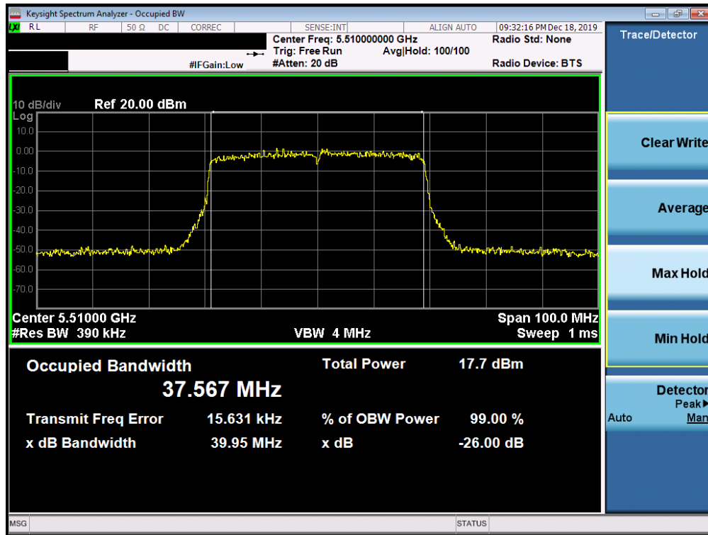
Plot 7-59. 26dB Bandwidth Plot SISO ANT1 (40MHz BW 802.11ax (UNII Band 2C) – Ch. 102)
