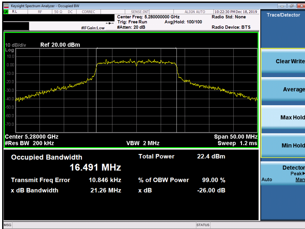
Plot 7-89. 26dB Bandwidth Plot SISO ANT2 (802.11a (UNII Band 2A) – Ch. 56)
