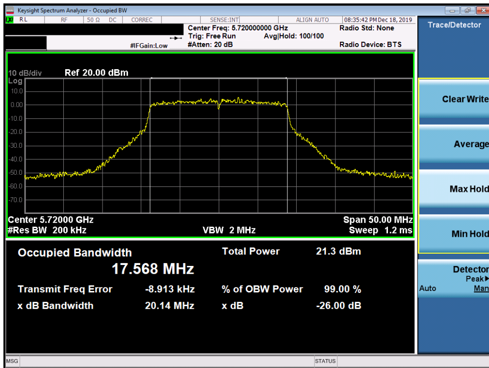
Plot 7-46. 26dB Bandwidth Plot SISO ANT1 (20MHz BW 802.11n (UNII Band 2C) – Ch. 144)
