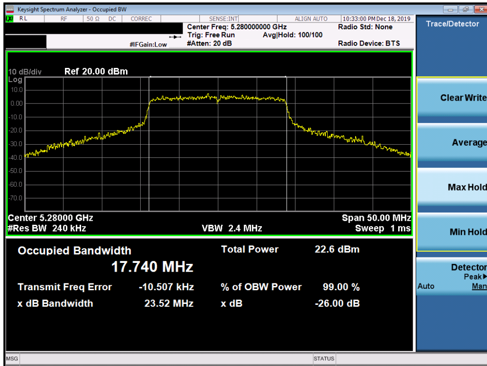
Plot 7-92. 26dB Bandwidth Plot SISO ANT2 (20MHz BW 802.11n (UNII Band 2A) – Ch. 56)
