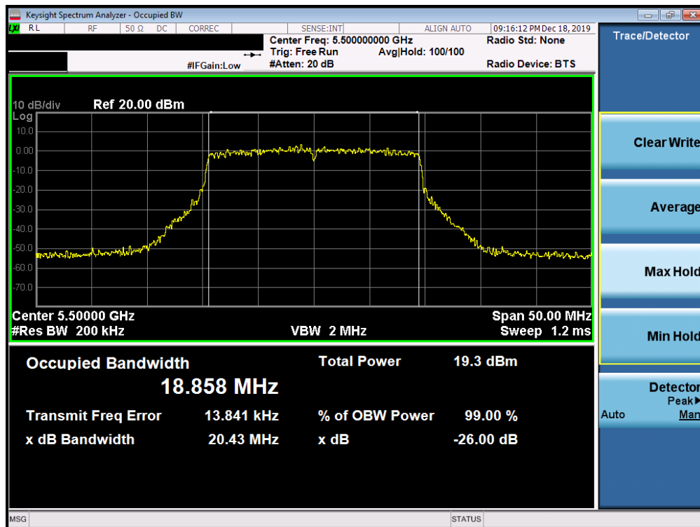
Plot 7-50. 26dB Bandwidth Plot SISO ANT1 (20MHz BW 802.11ax (UNII Band 2C) – Ch. 100)
