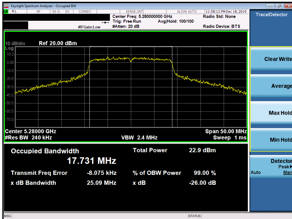
Plot 7-95. 26dB Bandwidth Plot SISO ANT2 (20MHz BW 802.11ac (UNII Band 2A) – Ch. 56)
