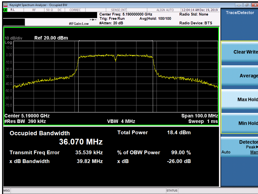
Plot 7-82. 26dB Bandwidth Plot SISO ANT2 (40MHz BW 802.11ac (UNII Band 1) – Ch. 38)
