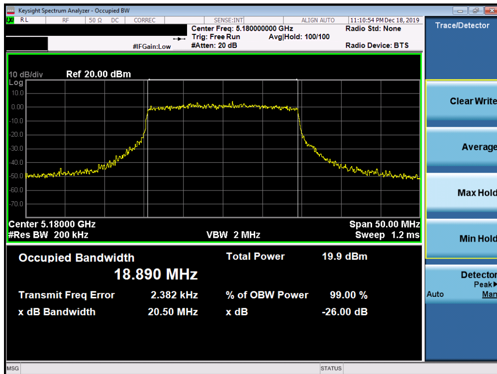
Plot 7-77. 26dB Bandwidth Plot SISO ANT2 (20MHz BW 802.11ax (UNII Band 1) – Ch. 36)
