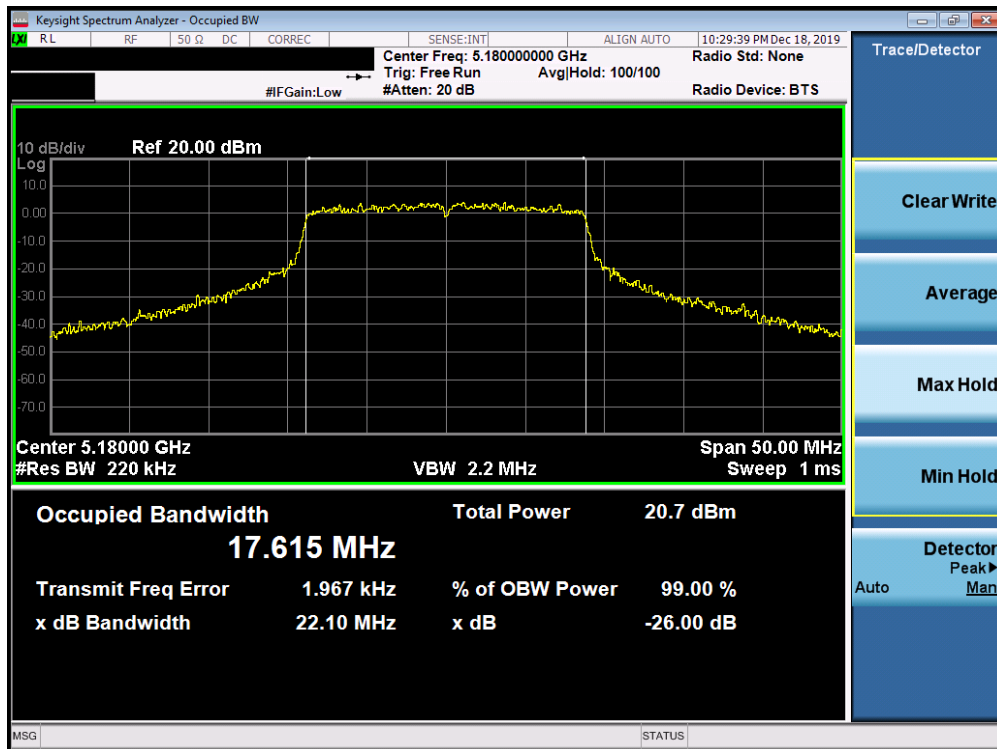
Plot 7-71. 26dB Bandwidth Plot SISO ANT2 (20MHz BW 802.11n (UNII Band 1) – Ch. 36)
