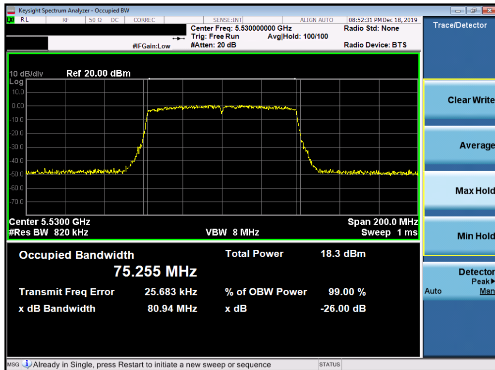
Plot 7-62. 26dB Bandwidth Plot SISO ANT1 (80MHz BW 802.11ac (UNII Band 2C) – Ch. 106)
