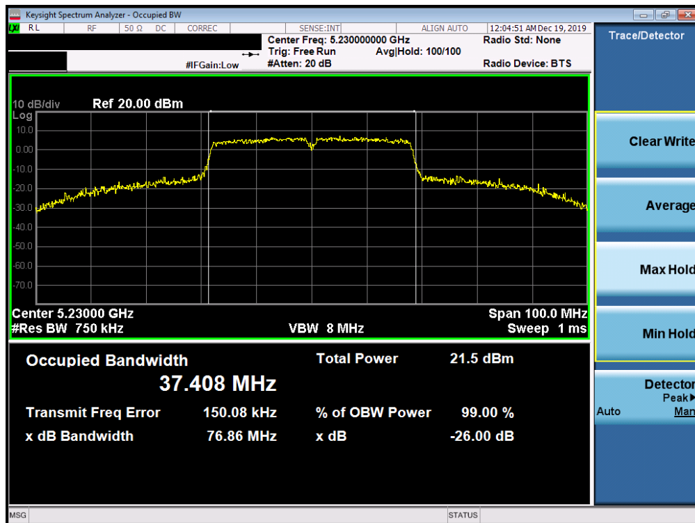
Plot 7-83. 26dB Bandwidth Plot SISO ANT2 (40MHz BW 802.11ac (UNII Band 1) – Ch. 46)
