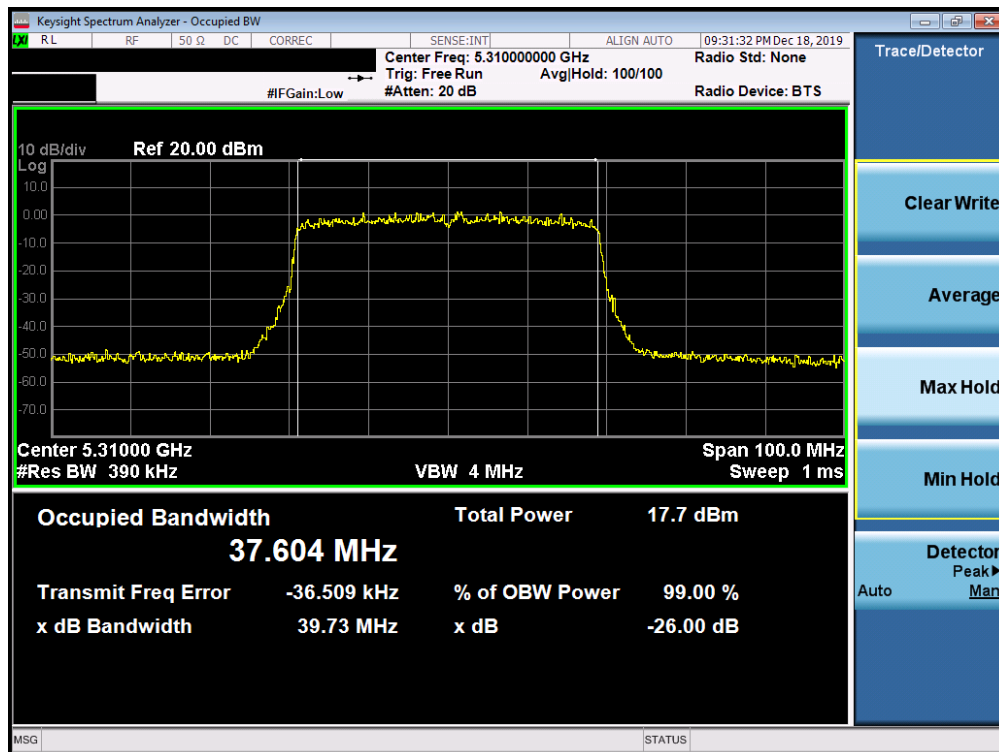
Plot 7-38. 26dB Bandwidth Plot SISO ANT1 (40MHz BW 802.11ax (UNII Band 2A) – Ch. 62)
