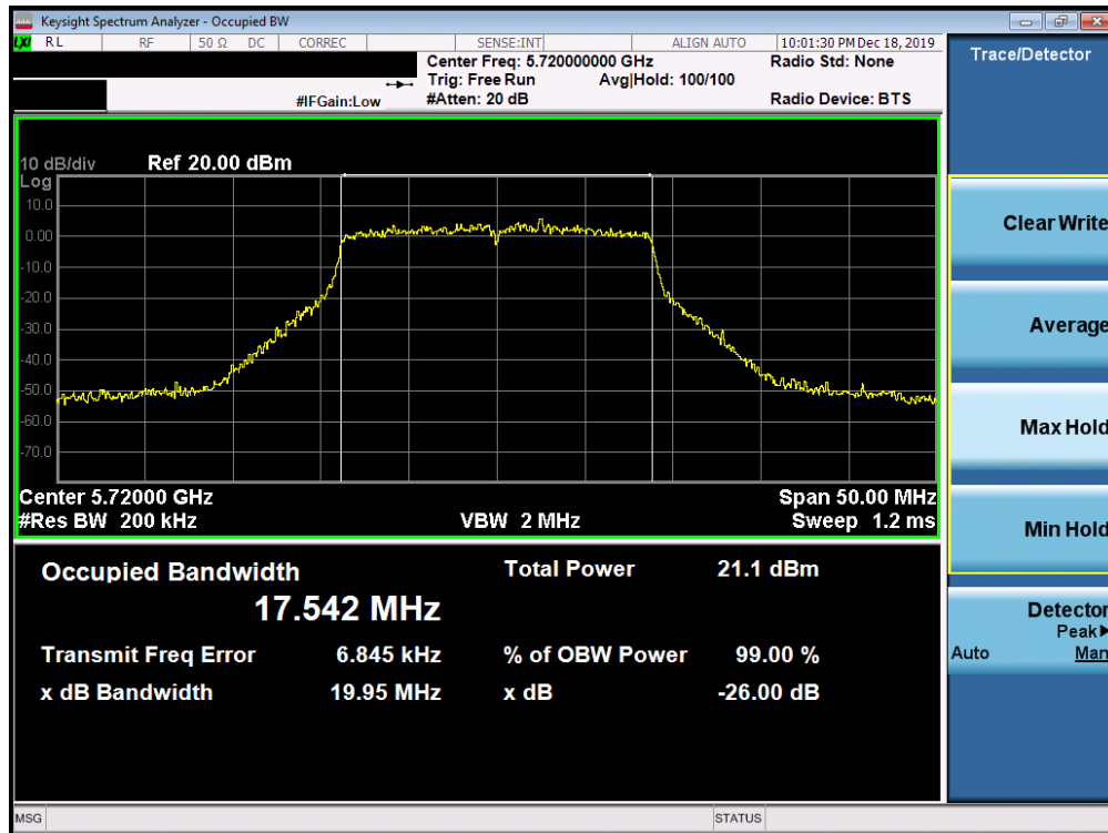
Plot 7-49. 26dB Bandwidth Plot SISO ANT1 (20MHz BW 802.11ac (UNII Band 2C) – Ch. 144)
