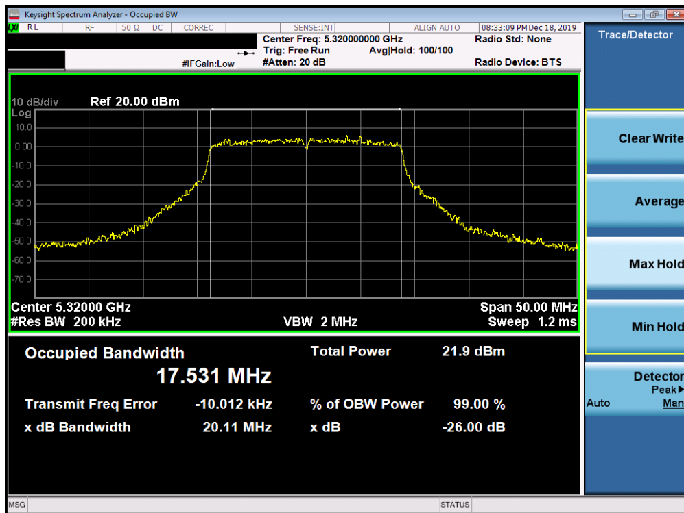
Plot 7-26. 26dB Bandwidth Plot SISO ANT1 (20MHz BW 802.11n (UNII Band 2A) – Ch. 64)
