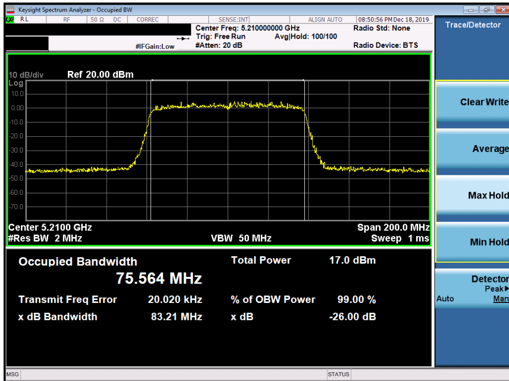
Plot 7-19. 26dB Bandwidth Plot SISO ANT1 (80MHz BW 802.11ac (UNII Band 1) – Ch. 42)
