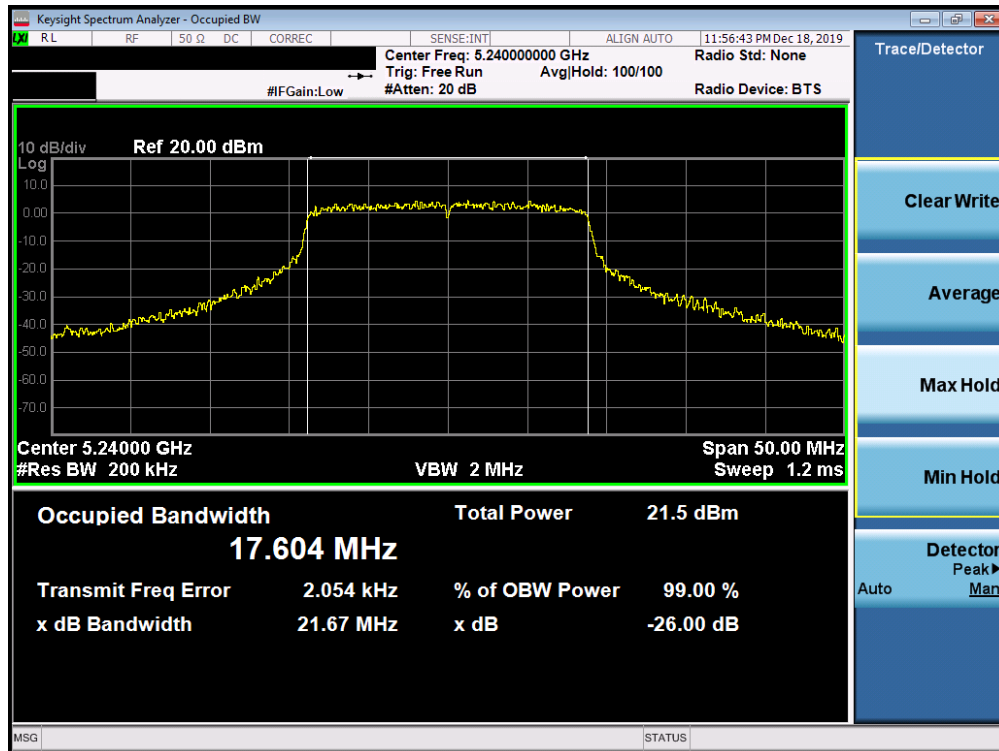
Plot 7-76. 26dB Bandwidth Plot SISO ANT2 (20MHz BW 802.11ac (UNII Band 1) – Ch. 48)
