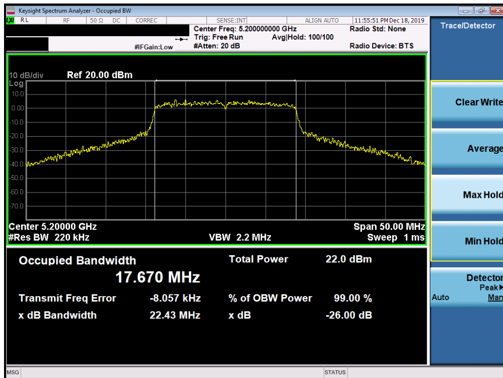
Plot 7-75. 26dB Bandwidth Plot SISO ANT2 (20MHz BW 802.11ac (UNII Band 1) – Ch. 40)
