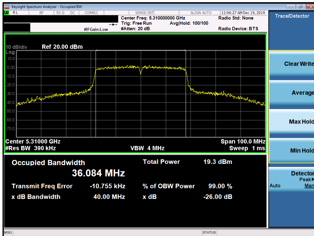
Plot 7-103. 26dB Bandwidth Plot SISO ANT2 (40MHz BW 802.11ac (UNII Band 2A) – Ch. 62)
