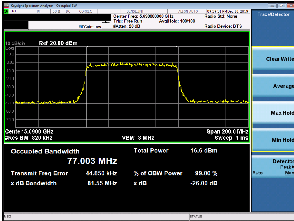
Plot 7-67. 26dB Bandwidth Plot SISO ANT1 (80MHz BW 802.11ax (UNII Band 2C) – Ch. 138)
