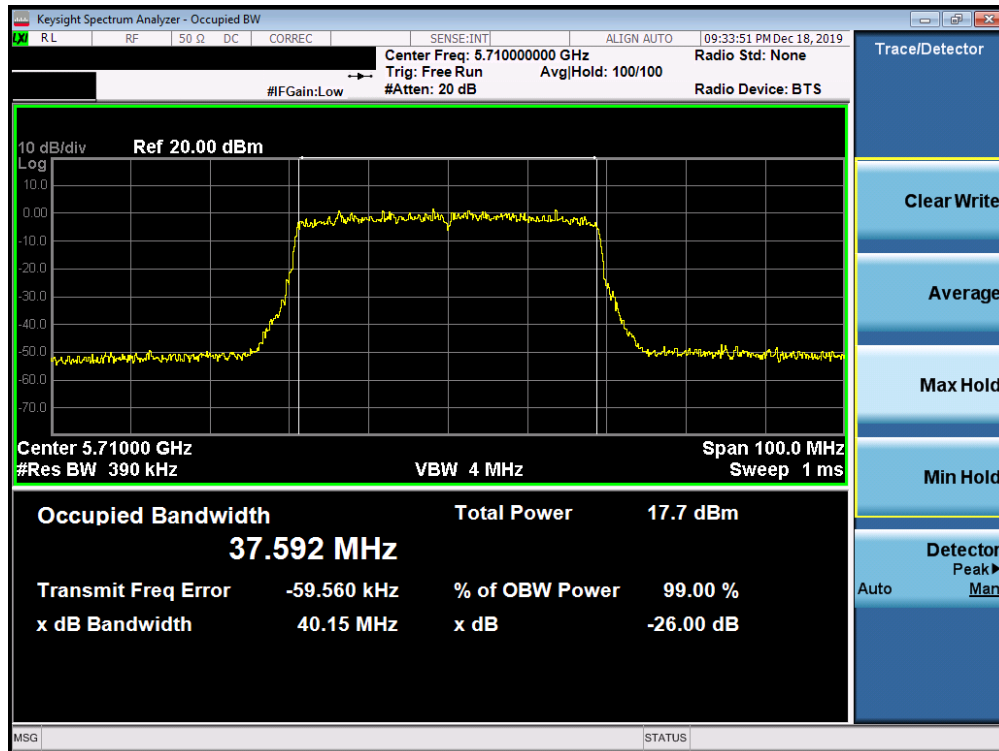
Plot 7-61. 26dB Bandwidth Plot SISO ANT1 (40MHz BW 802.11ax (UNII Band 2C) – Ch. 142)
