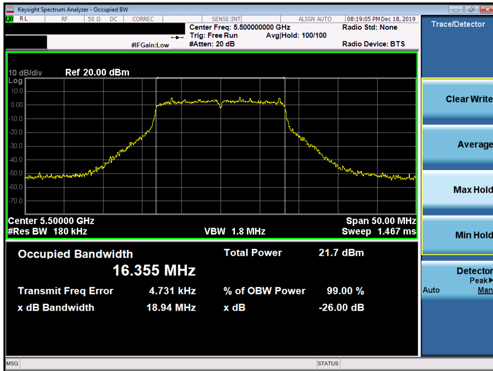
Plot 7-41. 26dB Bandwidth Plot SISO ANT1 (802.11a (UNII Band 2C) – Ch. 100)
