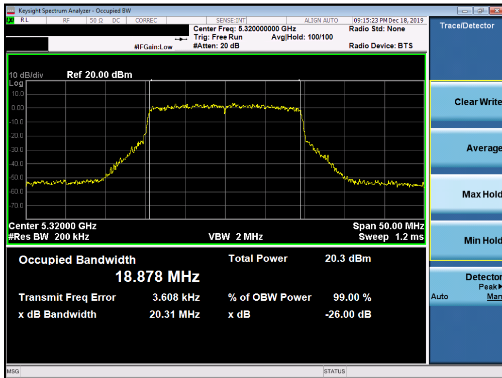
Plot 7-32. 26dB Bandwidth Plot SISO ANT1 (20MHz BW 802.11ax (UNII Band 2A) – Ch. 64)
