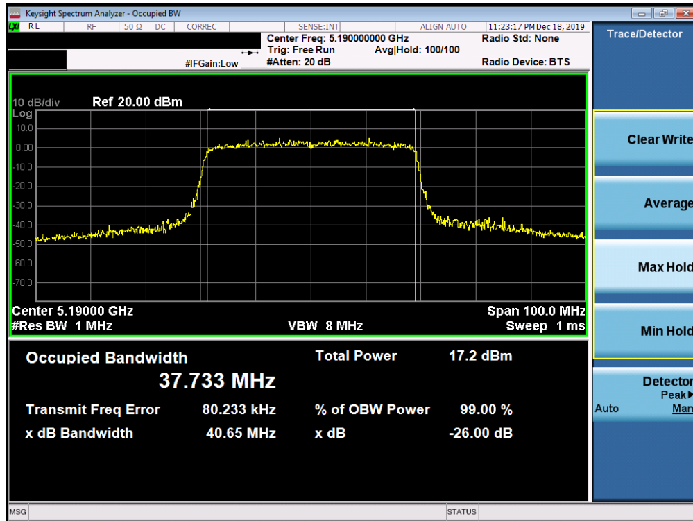
Plot 7-84. 26dB Bandwidth Plot SISO ANT2 (40MHz BW 802.11ax (UNII Band 1) – Ch. 38)
