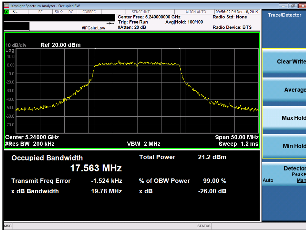
Plot 7-9. 26dB Bandwidth Plot SISO ANT1 (20MHz BW 802.11ac (UNII Band 1) – Ch. 48)
