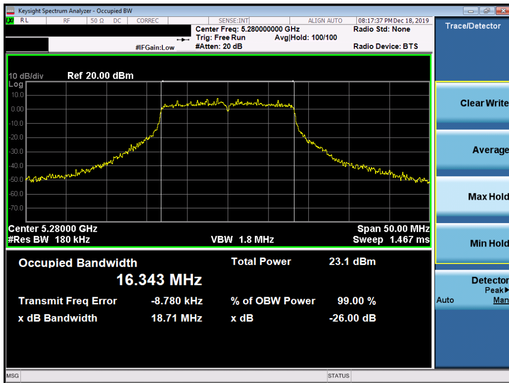
Plot 7-22. 26dB Bandwidth Plot SISO ANT1 (802.11a (UNII Band 2A) – Ch. 56)
