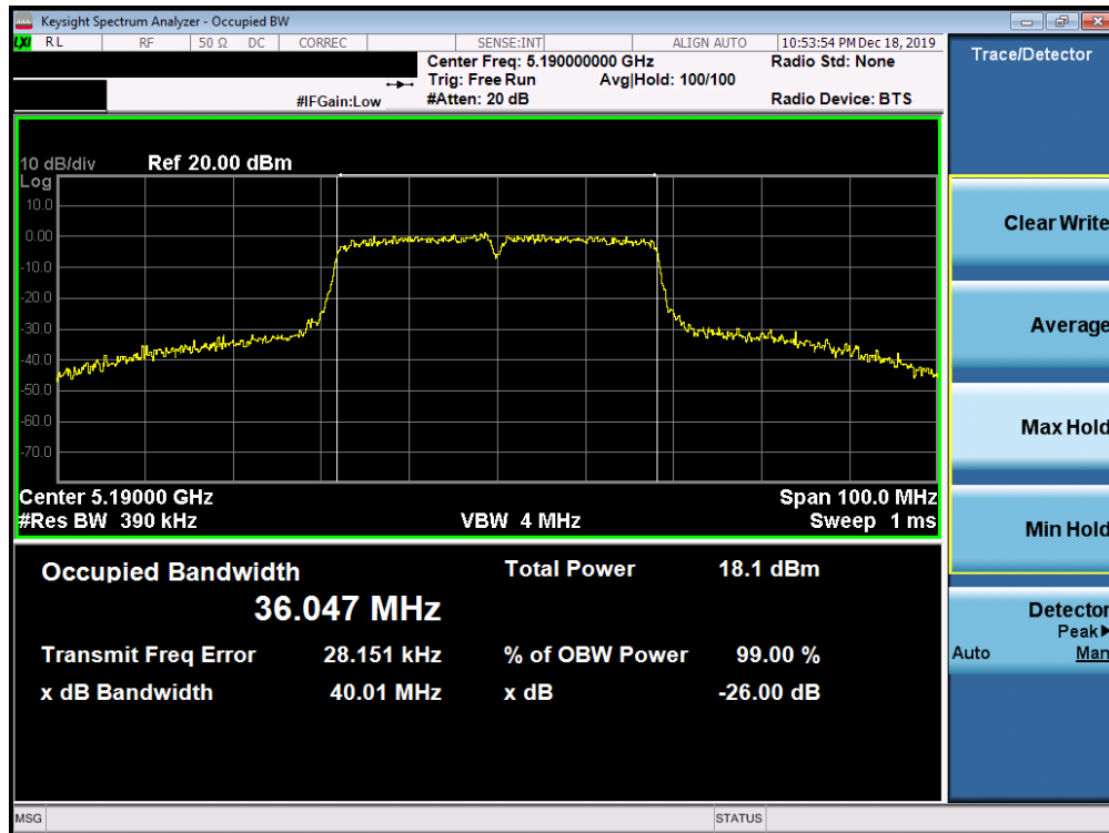
Plot 7-80. 26dB Bandwidth Plot SISO ANT2 (40MHz BW 802.11n (UNII Band 1) – Ch. 38)
