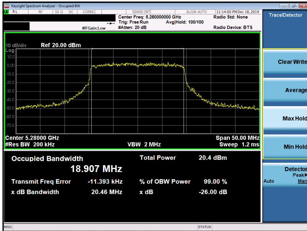
Plot 7-98. 26dB Bandwidth Plot SISO ANT2 (20MHz BW 802.11ax (UNII Band 2A) – Ch. 56)
