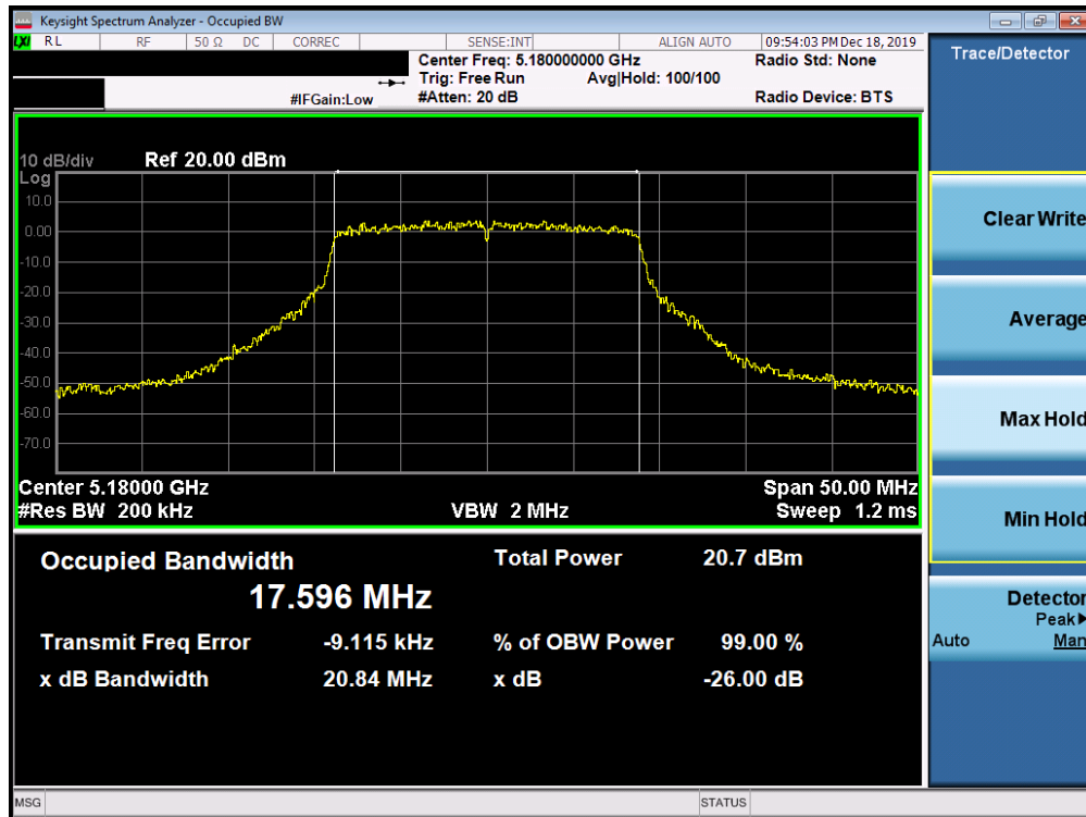
Plot 7-7. 26dB Bandwidth Plot SISO ANT1 (20MHz BW 802.11ac (UNII Band 1) – Ch. 36)
