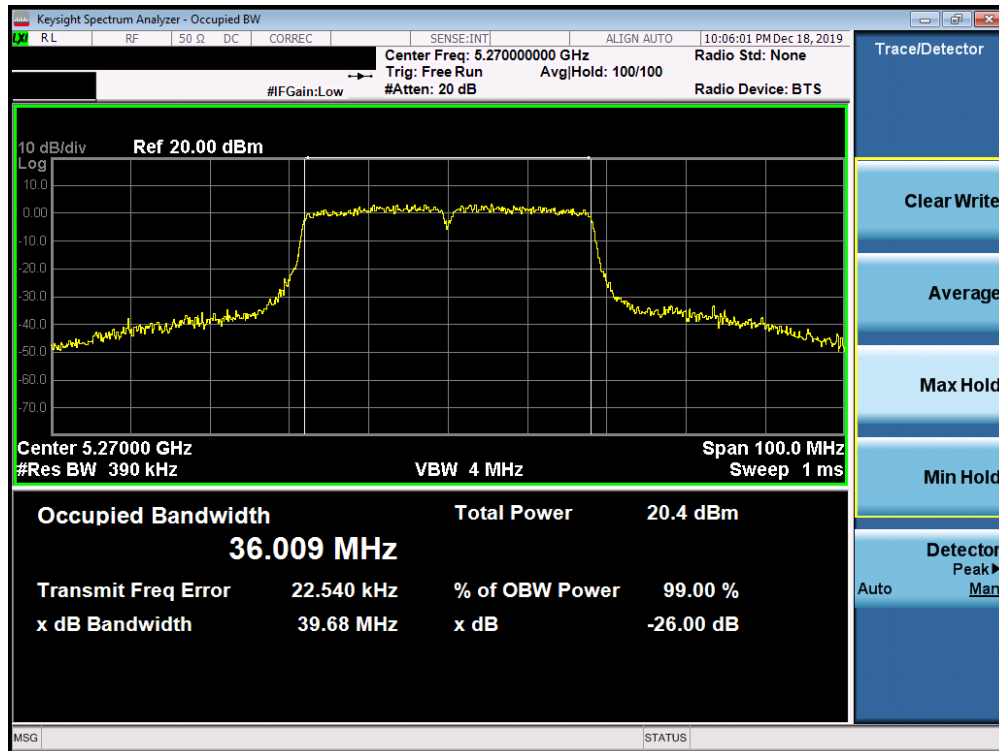
Plot 7-35. 26dB Bandwidth Plot SISO ANT1 (40MHz BW 802.11ac (UNII Band 2A) – Ch. 54)
