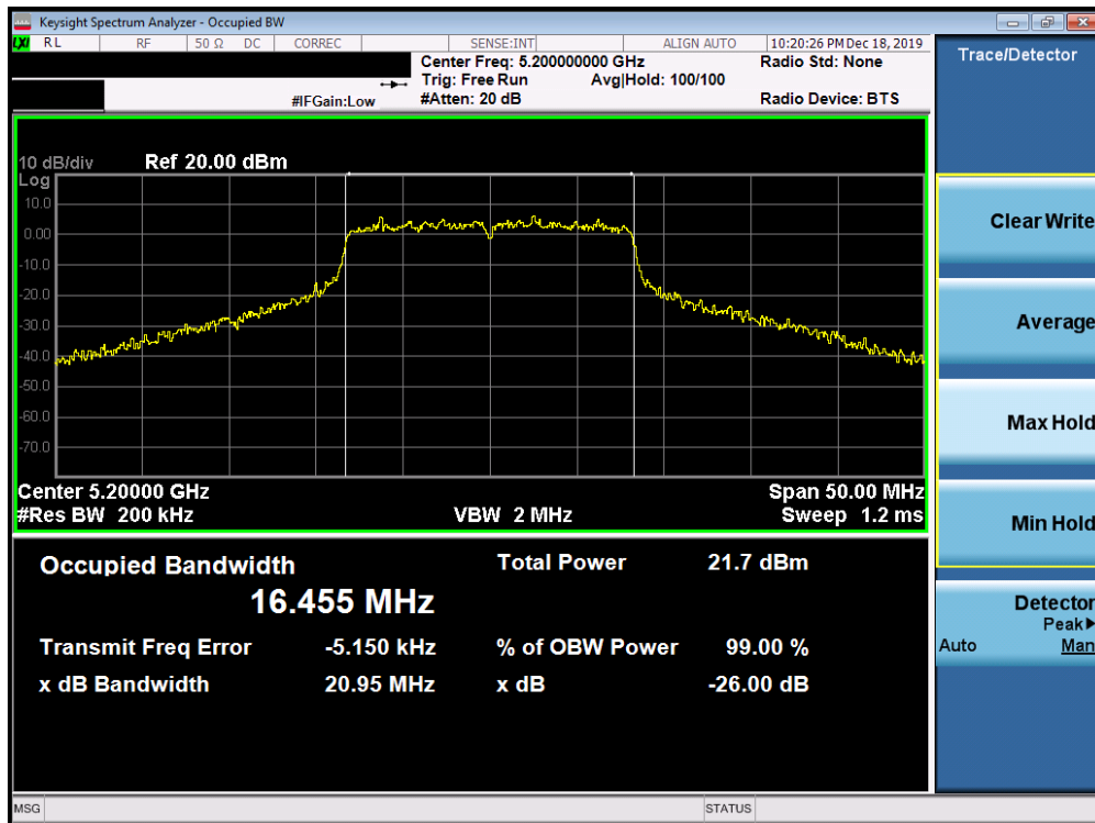
Plot 7-69. 26dB Bandwidth Plot SISO ANT2 (802.11a (UNII Band 1) – Ch. 40)
