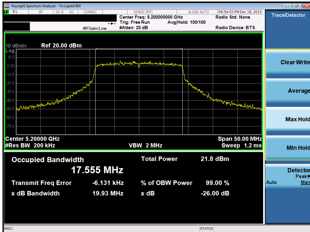
Plot 7-8. 26dB Bandwidth Plot SISO ANT1 (20MHz BW 802.11ac (UNII Band 1) – Ch. 40)
