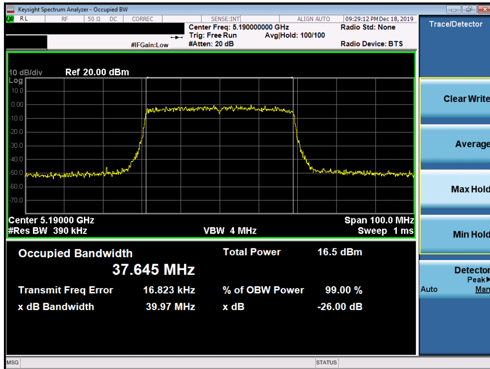
Plot 7-17. 26dB Bandwidth Plot SISO ANT1 (40MHz BW 802.11ax (UNII Band 1) – Ch. 38)
