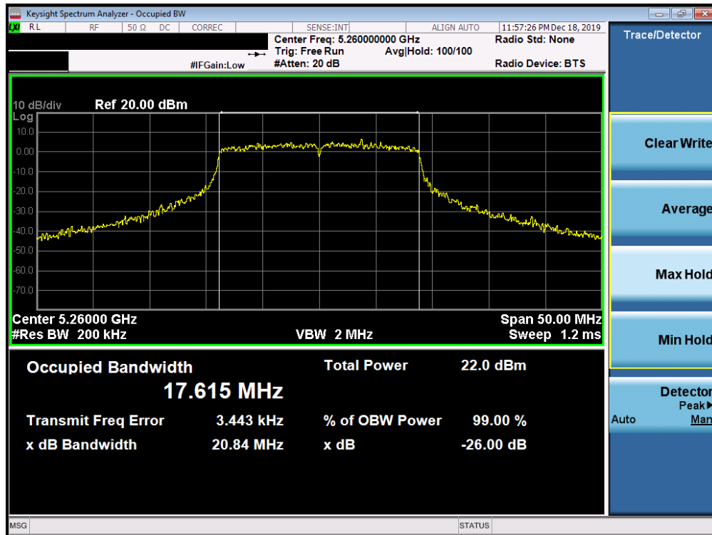
Plot 7-94. 26dB Bandwidth Plot SISO ANT2 (20MHz BW 802.11ac (UNII Band 2A) – Ch. 52)
