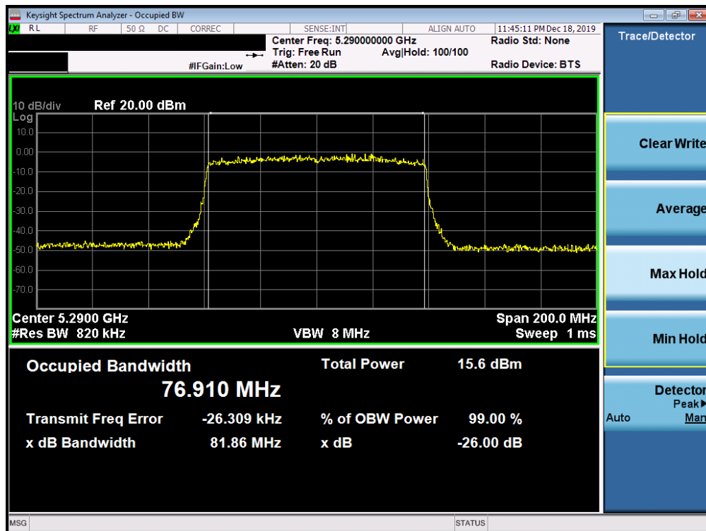
Plot 7-107. 26dB Bandwidth Plot SISO ANT2 (80MHz BW 802.11ax (UNII Band 2A) – Ch. 58)
