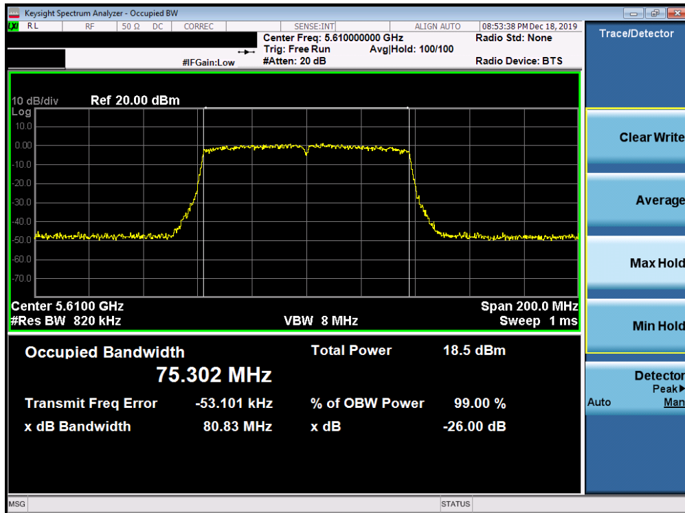
Plot 7-63. 26dB Bandwidth Plot SISO ANT1 (80MHz BW 802.11ac (UNII Band 2C) – Ch. 122)
