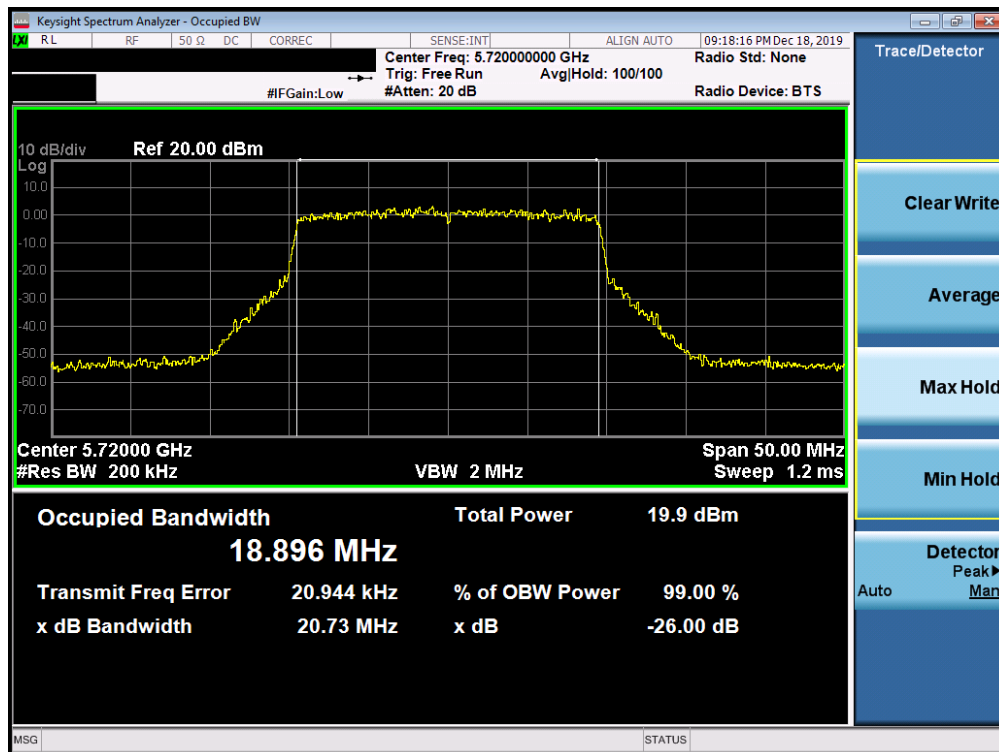
Plot 7-52. 26dB Bandwidth Plot SISO ANT1 (20MHz BW 802.11ax (UNII Band 2C) – Ch. 144)
