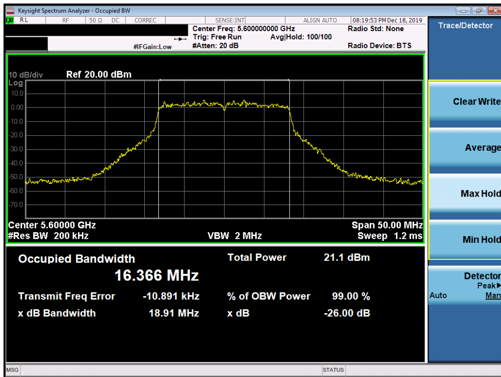
Plot 7-42. 26dB Bandwidth Plot SISO ANT1 (802.11a (UNII Band 2C) – Ch. 120)
