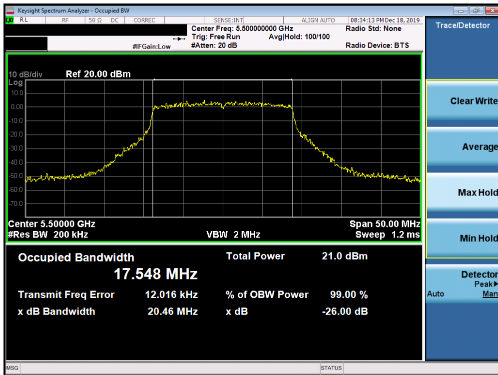
Plot 7-44. 26dB Bandwidth Plot SISO ANT1 (20MHz BW 802.11n (UNII Band 2C) – Ch. 100)
