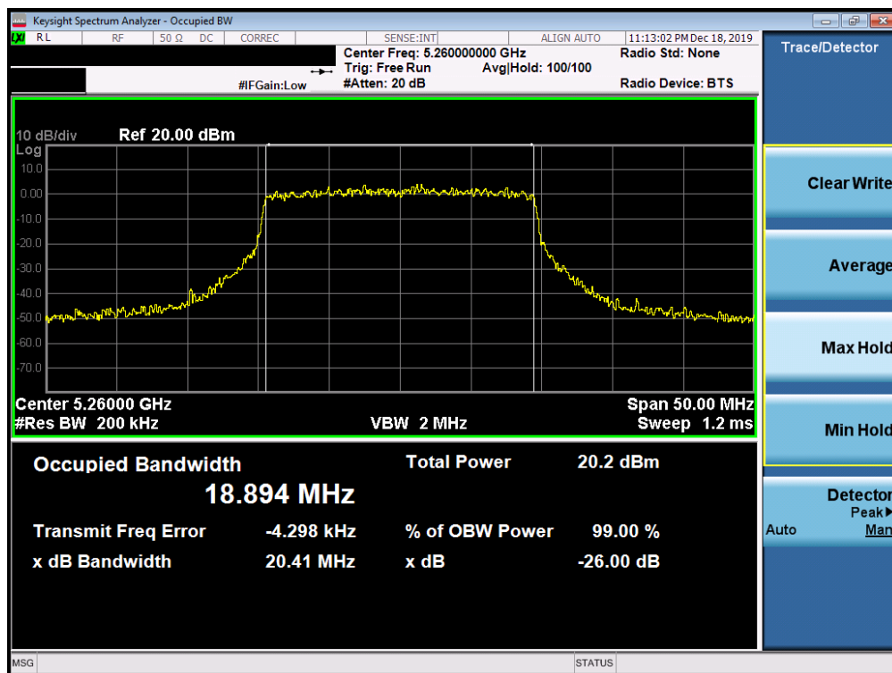
Plot 7-97. 26dB Bandwidth Plot SISO ANT2 (20MHz BW 802.11ax (UNII Band 2A) – Ch. 52)
