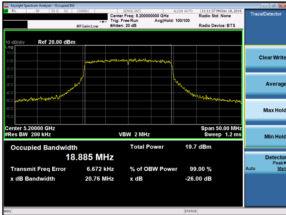
Plot 7-78. 26dB Bandwidth Plot SISO ANT2 (20MHz BW 802.11ax (UNII Band 1) – Ch. 40)
