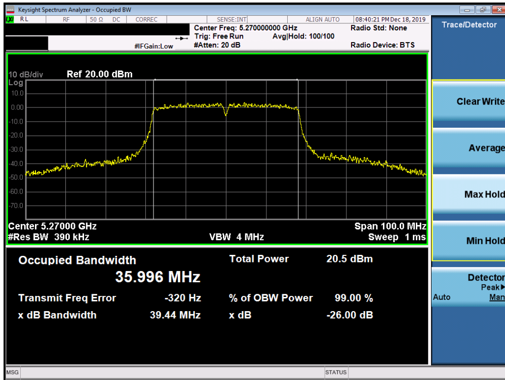
Plot 7-33. 26dB Bandwidth Plot SISO ANT1 (40MHz BW 802.11n (UNII Band 2A) – Ch. 54)
