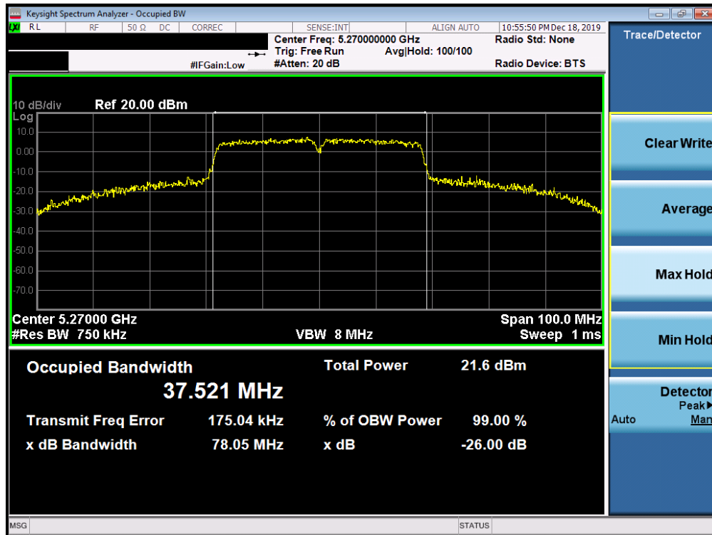
Plot 7-100. 26dB Bandwidth Plot SISO ANT2 (40MHz BW 802.11n (UNII Band 2A) – Ch. 54)
