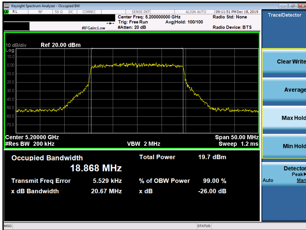
Plot 7-11. 26dB Bandwidth Plot SISO ANT1 (20MHz BW 802.11ax (UNII Band 1) – Ch. 40)
