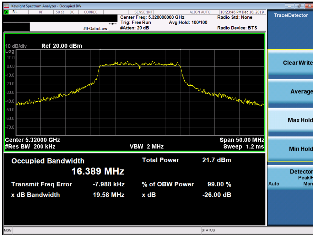
Plot 7-90. 26dB Bandwidth Plot SISO ANT2 (802.11a (UNII Band 2A) – Ch. 64)
