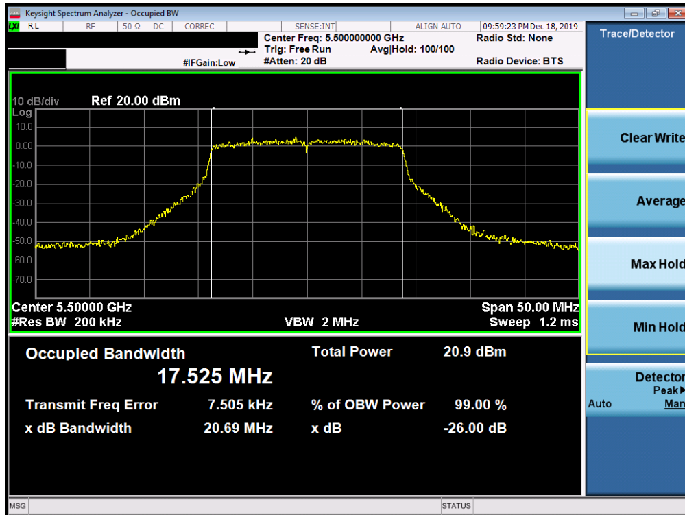
Plot 7-47. 26dB Bandwidth Plot SISO ANT1 (20MHz BW 802.11ac (UNII Band 2C) – Ch. 100)
