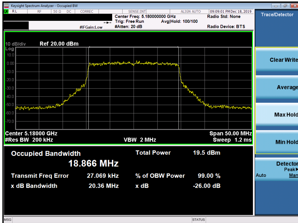
Plot 7-10. 26dB Bandwidth Plot SISO ANT1 (20MHz BW 802.11ax (UNII Band 1) – Ch. 36)
