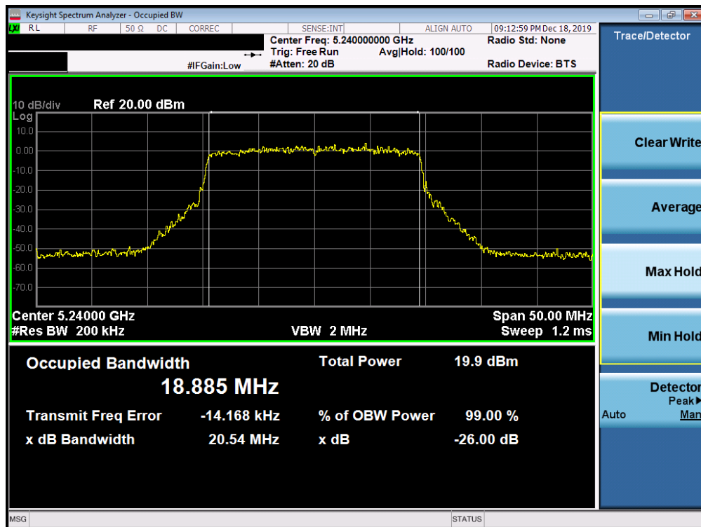
Plot 7-12. 26dB Bandwidth Plot SISO ANT1 (20MHz BW 802.11ax (UNII Band 1) – Ch. 48)
