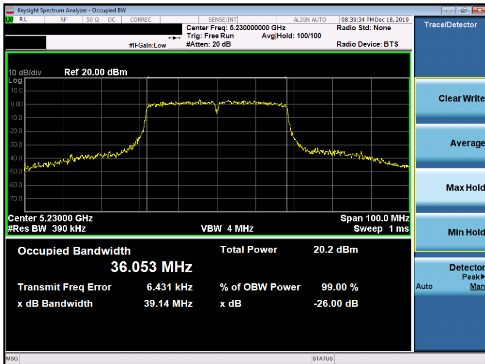
Plot 7-14. 26dB Bandwidth Plot SISO ANT1 (40MHz BW 802.11n (UNII Band 1) – Ch. 46)
