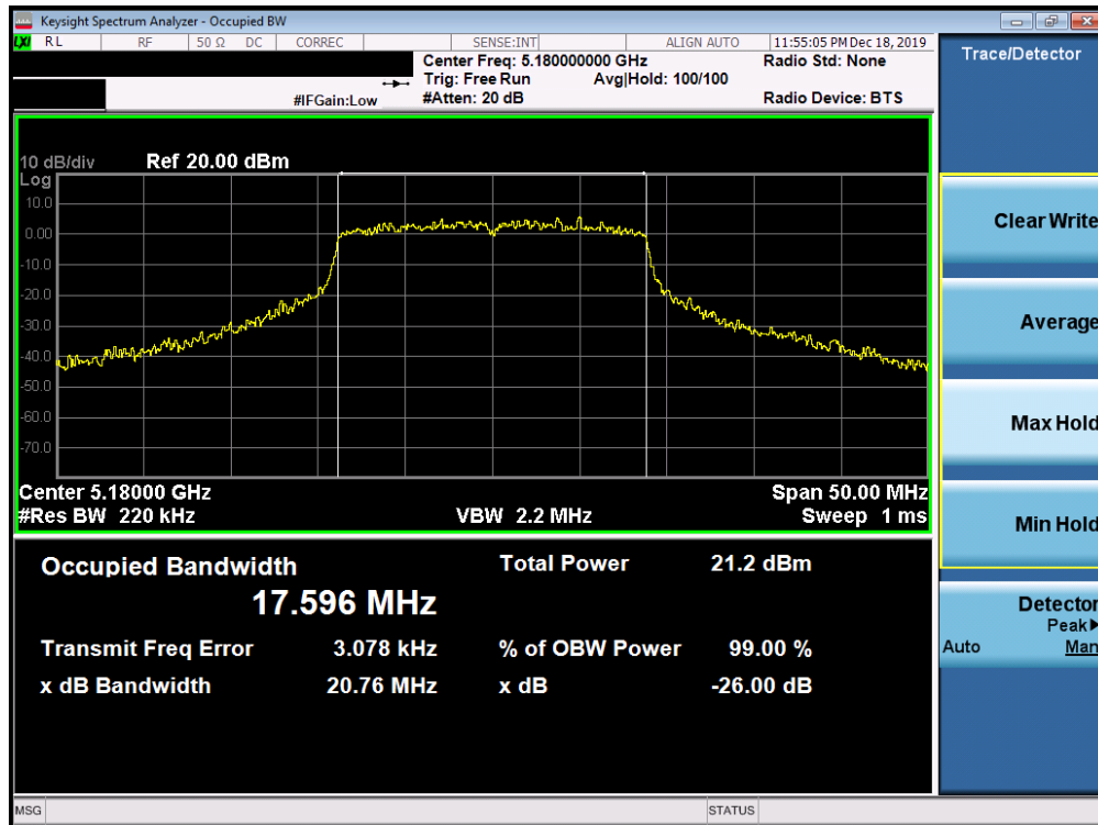
Plot 7-74. 26dB Bandwidth Plot SISO ANT2 (20MHz BW 802.11ac (UNII Band 1) – Ch. 36)
