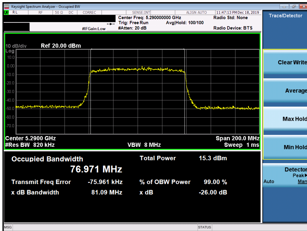
Plot 7-40. 26dB Bandwidth Plot SISO ANT1 (80MHz BW 802.11ax (UNII Band 2A) – Ch. 58)
