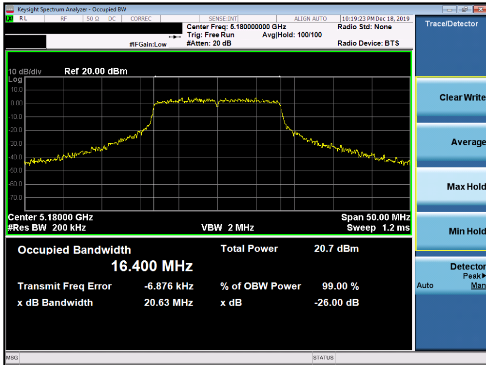
Plot 7-68. 26dB Bandwidth Plot SISO ANT2 (802.11a (UNII Band 1) – Ch. 36)
