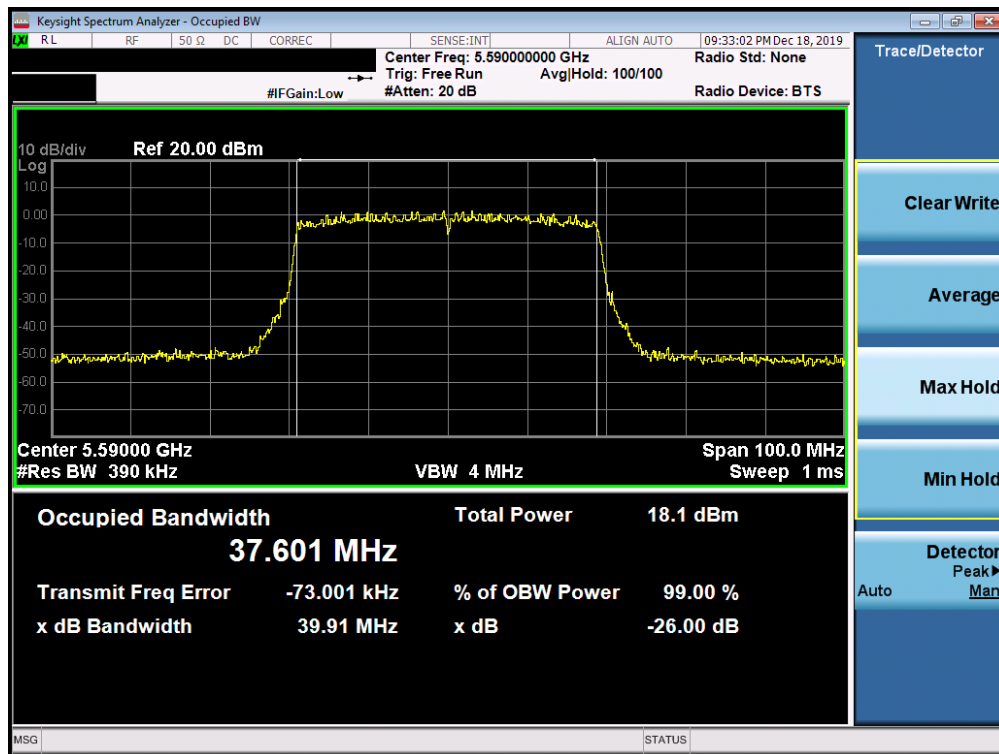
Plot 7-60. 26dB Bandwidth Plot SISO ANT1 (40MHz BW 802.11ax (UNII Band 2C) – Ch. 118)
