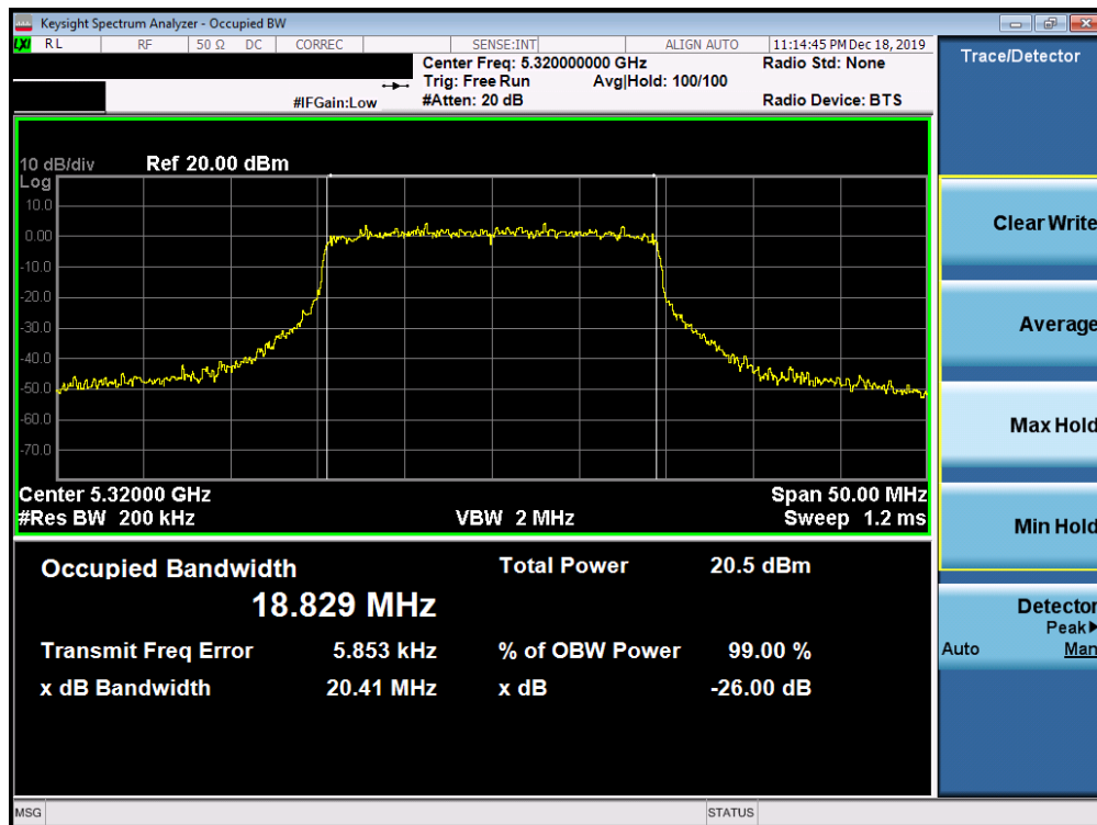
Plot 7-99. 26dB Bandwidth Plot SISO ANT2 (20MHz BW 802.11ax (UNII Band 2A) – Ch. 64)
