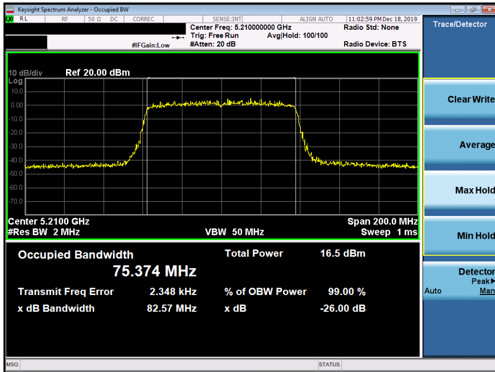
Plot 7-86. 26dB Bandwidth Plot SISO ANT2 (80MHz BW 802.11ac (UNII Band 1) – Ch. 42)
