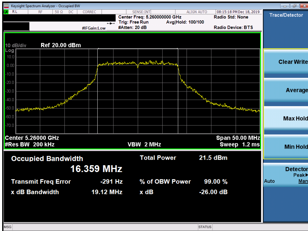
Plot 7-21. 26dB Bandwidth Plot SISO ANT1 (802.11a (UNII Band 2A) – Ch. 52)
