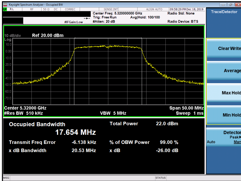
Plot 7-29. 26dB Bandwidth Plot SISO ANT1 (20MHz BW 802.11ac (UNII Band 2A) – Ch. 64)
