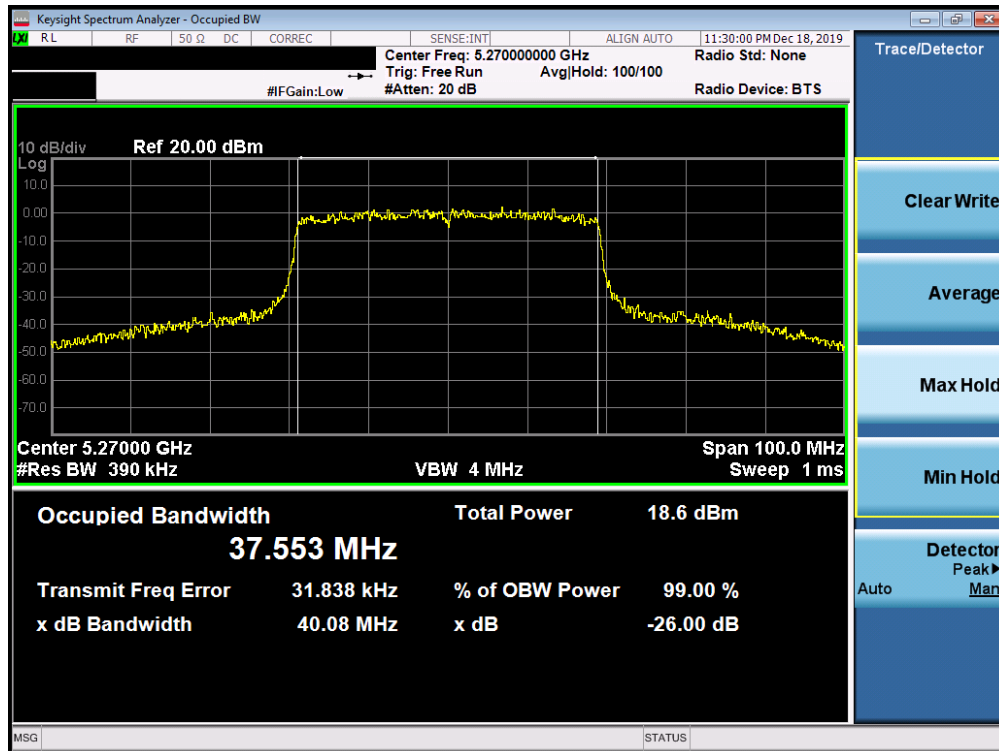
Plot 7-104. 26dB Bandwidth Plot SISO ANT2 (40MHz BW 802.11ax (UNII Band 2A) – Ch. 54)
