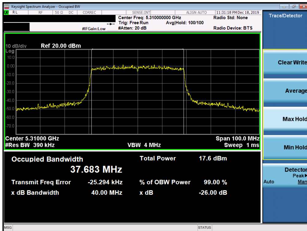
Plot 7-105. 26dB Bandwidth Plot SISO ANT2 (40MHz BW 802.11ax (UNII Band 2A) – Ch. 62)
