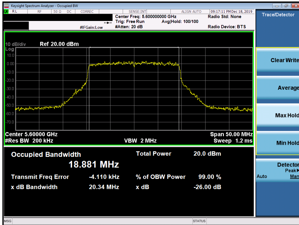
Plot 7-51. 26dB Bandwidth Plot SISO ANT1 (20MHz BW 802.11ax (UNII Band 2C) – Ch. 120)
