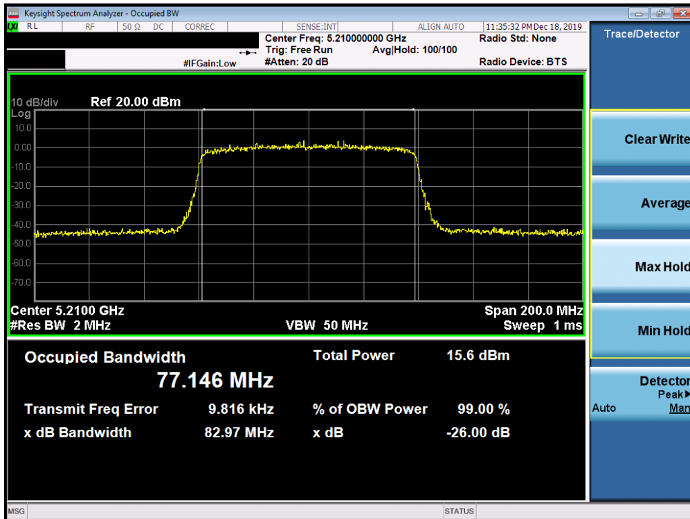
Plot 7-87. 26dB Bandwidth Plot SISO ANT2 (80MHz BW 802.11ax (UNII Band 1) – Ch. 42)
