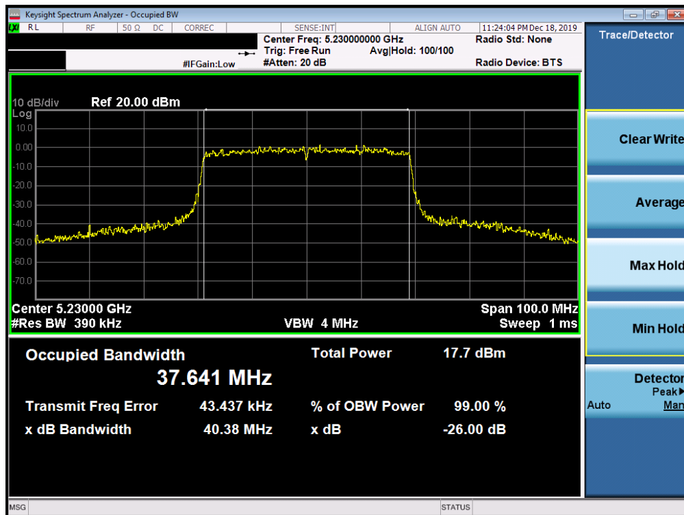
Plot 7-85. 26dB Bandwidth Plot SISO ANT2 (40MHz BW 802.11ax (UNII Band 1) – Ch. 46)
