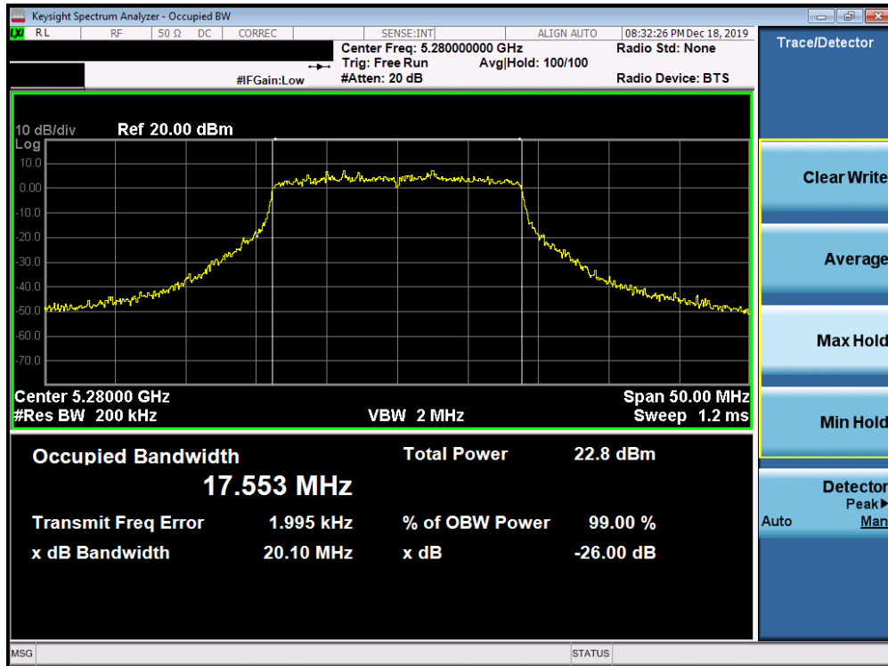
Plot 7-25. 26dB Bandwidth Plot SISO ANT1 (20MHz BW 802.11n (UNII Band 2A) – Ch. 56)
