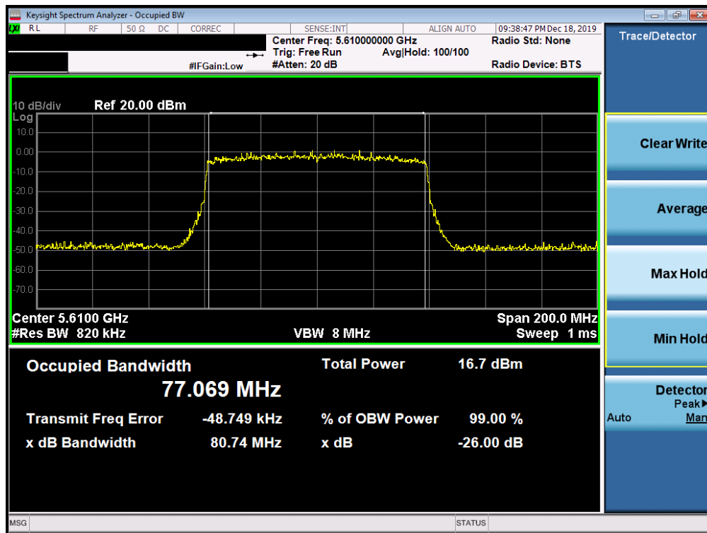
Plot 7-66. 26dB Bandwidth Plot SISO ANT1 (80MHz BW 802.11ax (UNII Band 2C) – Ch. 122)
