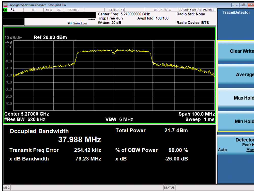
Plot 7-102. 26dB Bandwidth Plot SISO ANT2 (40MHz BW 802.11ac (UNII Band 2A) – Ch. 54)
