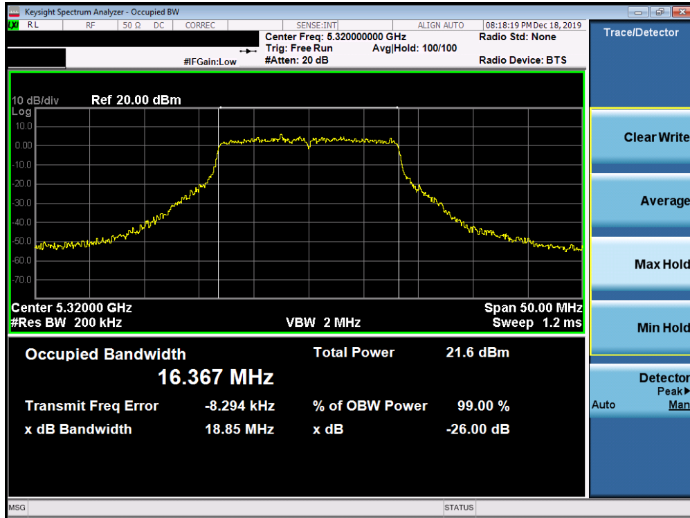
Plot 7-23. 26dB Bandwidth Plot SISO ANT1 (802.11a (UNII Band 2A) – Ch. 64)
