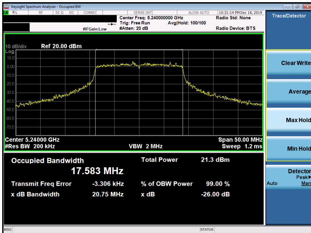
Plot 7-73. 26dB Bandwidth Plot SISO ANT2 (20MHz BW 802.11n (UNII Band 1) – Ch. 48)
