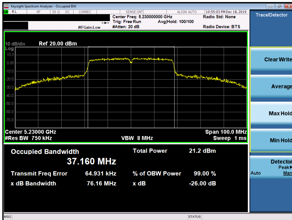
Plot 7-81. 26dB Bandwidth Plot SISO ANT2 (40MHz BW 802.11n (UNII Band 1) – Ch. 46)
