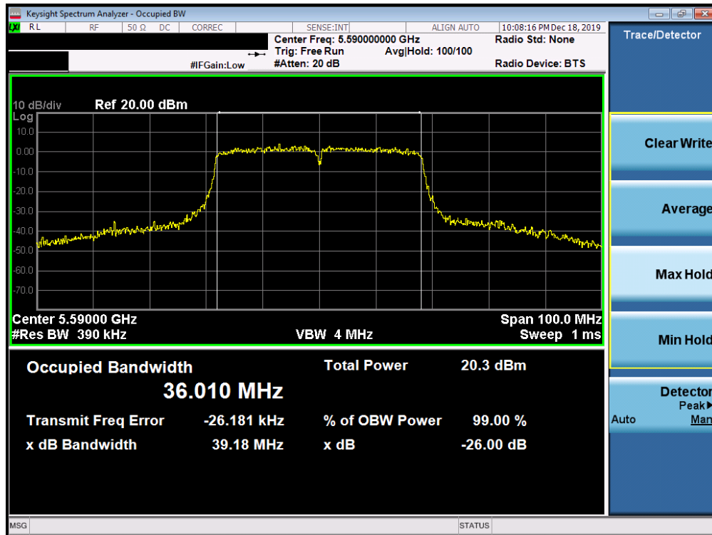
Plot 7-57. 26dB Bandwidth Plot SISO ANT1 (40MHz BW 802.11ac (UNII Band 2C) – Ch. 118)
