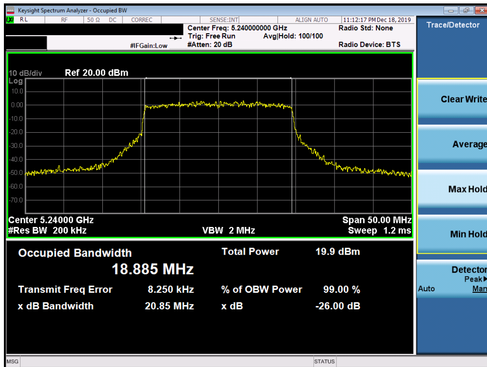
Plot 7-79. 26dB Bandwidth Plot SISO ANT2 (20MHz BW 802.11ax (UNII Band 1) – Ch. 48)
