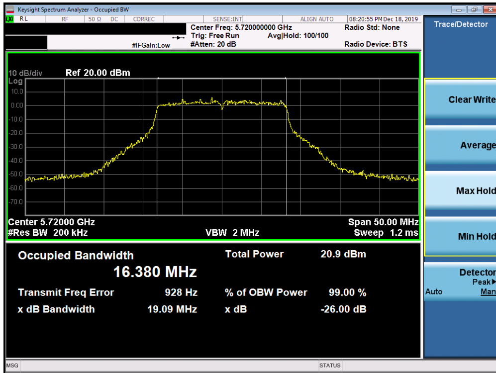
Plot 7-43. 26dB Bandwidth Plot SISO ANT1 (802.11a (UNII Band 2C) – Ch. 144)
