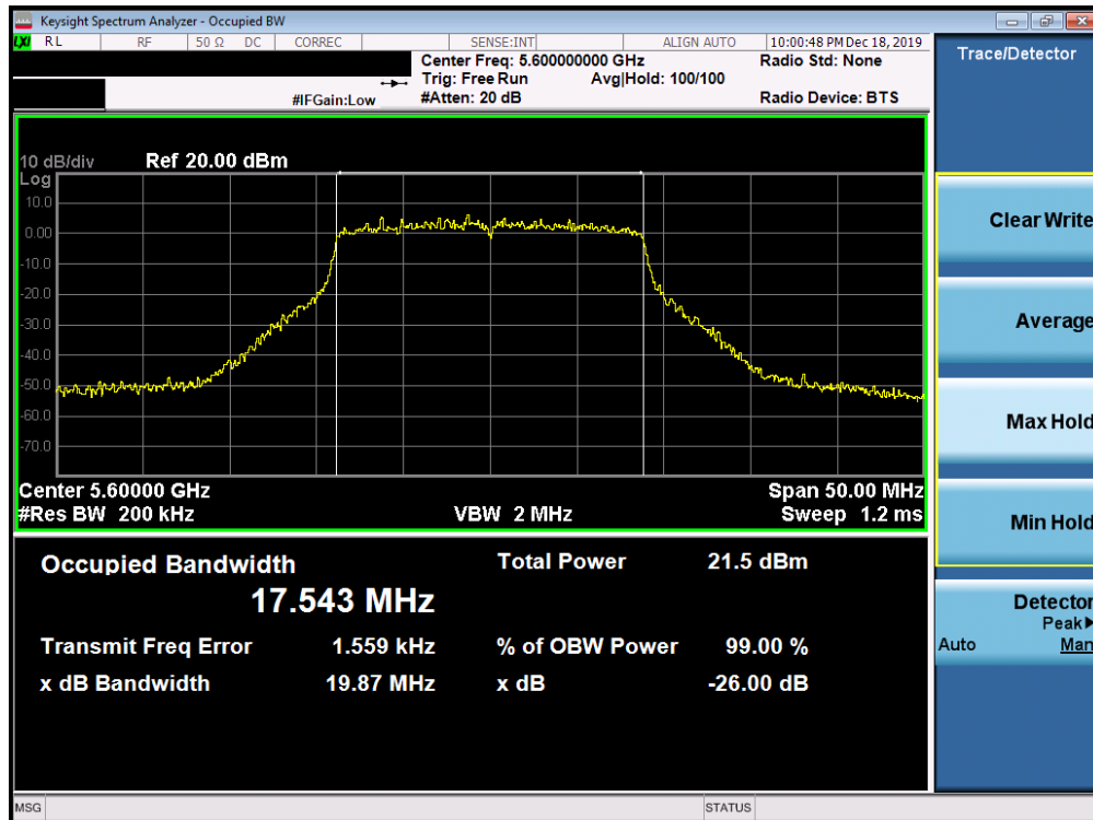
Plot 7-48. 26dB Bandwidth Plot SISO ANT1 (20MHz BW 802.11ac (UNII Band 2C) – Ch. 120)
