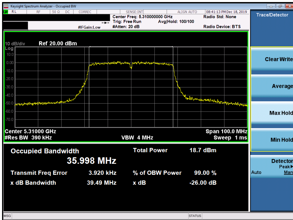
Plot 7-34. 26dB Bandwidth Plot SISO ANT1 (40MHz BW 802.11n (UNII Band 2A) – Ch. 62)
