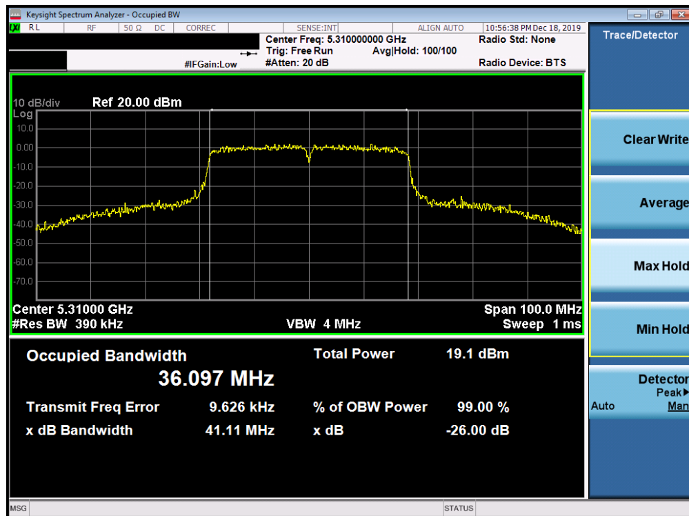
Plot 7-101. 26dB Bandwidth Plot SISO ANT2 (40MHz BW 802.11n (UNII Band 2A) – Ch. 62)
