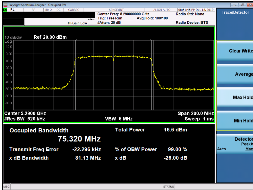
Plot 7-39. 26dB Bandwidth Plot SISO ANT1 (80MHz BW 802.11ac (UNII Band 2A) – Ch. 58)
