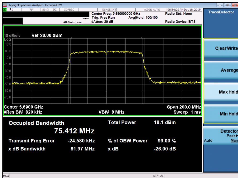
Plot 7-64. 26dB Bandwidth Plot SISO ANT1 (80MHz BW 802.11ac (UNII Band 2C) – Ch. 138)
