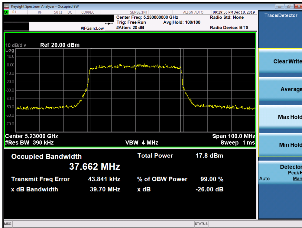
Plot 7-18. 26dB Bandwidth Plot SISO ANT1 (40MHz BW 802.11ax (UNII Band 1) – Ch. 46)
