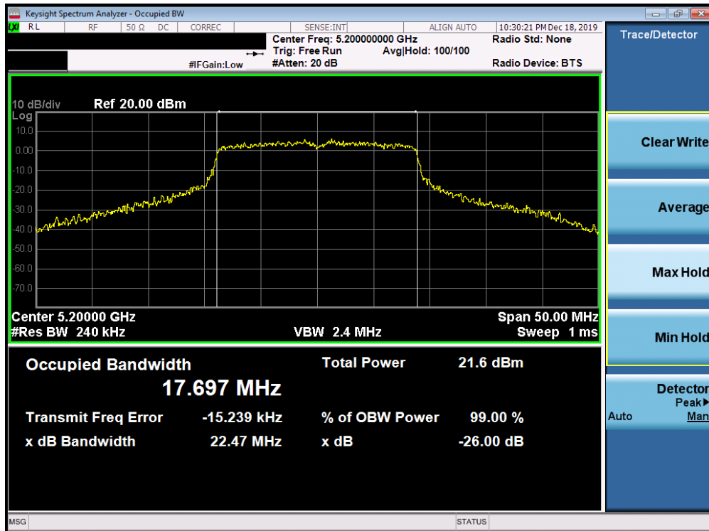
Plot 7-72. 26dB Bandwidth Plot SISO ANT2 (20MHz BW 802.11n (UNII Band 1) – Ch. 40)
