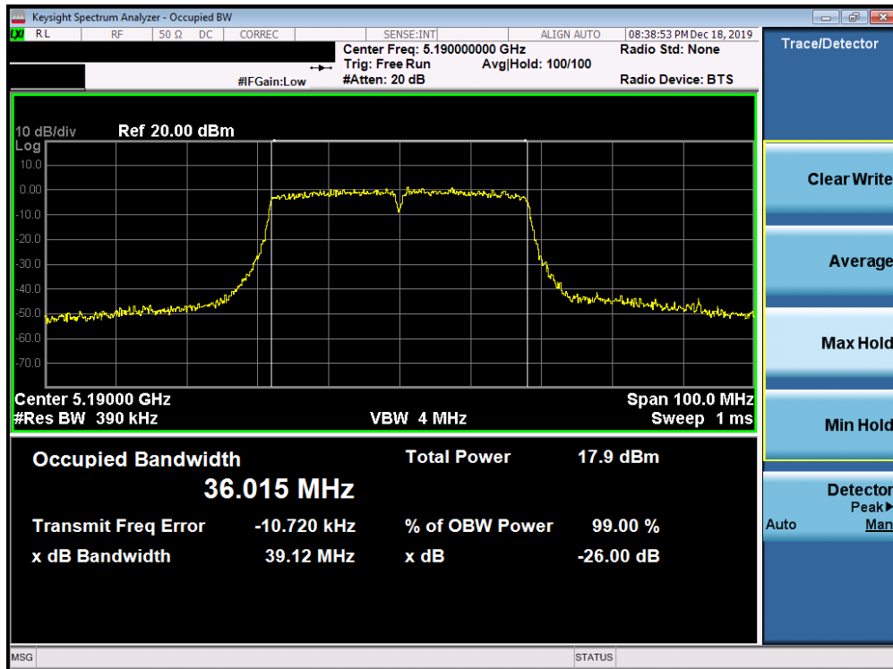
Plot 7-13. 26dB Bandwidth Plot SISO ANT1 (40MHz BW 802.11n (UNII Band 1) – Ch. 38)
