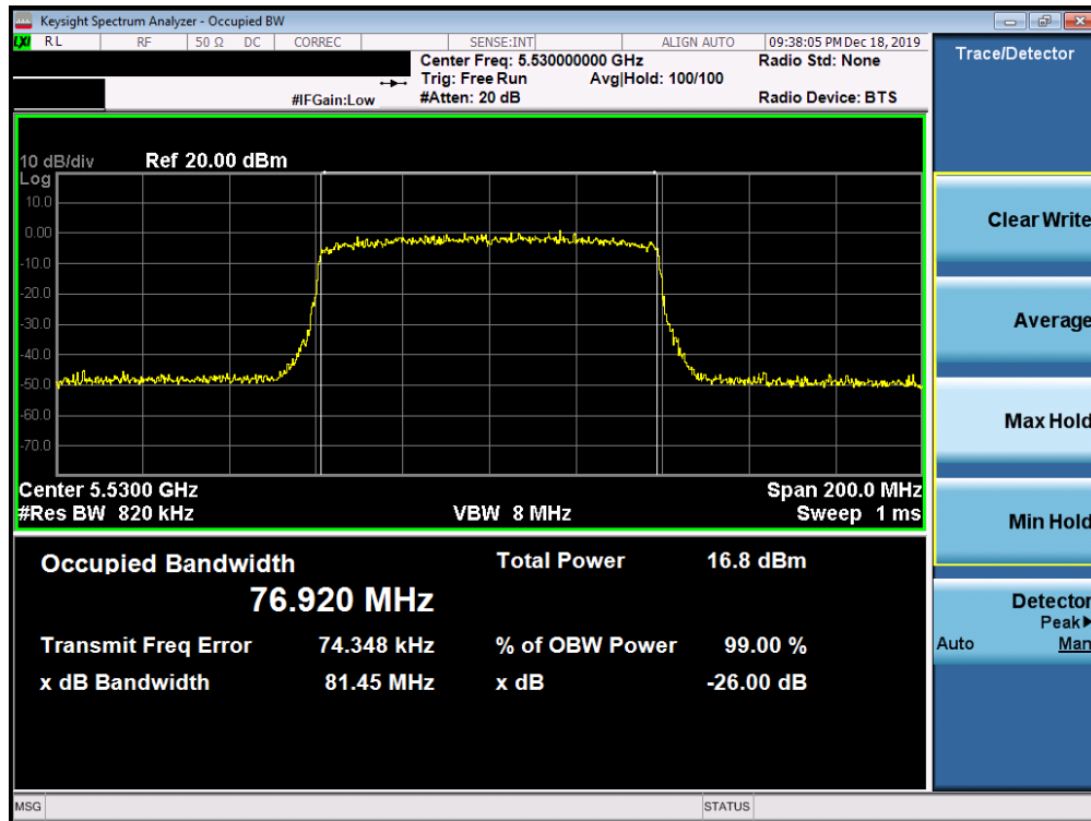
Plot 7-65. 26dB Bandwidth Plot SISO ANT1 (80MHz BW 802.11ax (UNII Band 2C) – Ch. 106)
