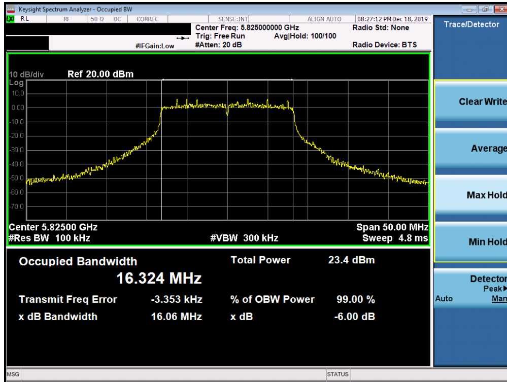
Plot 7-137. 6dB Bandwidth Plot SISO ANT1 (802.11a (UNII Band 3) – Ch. 165)
