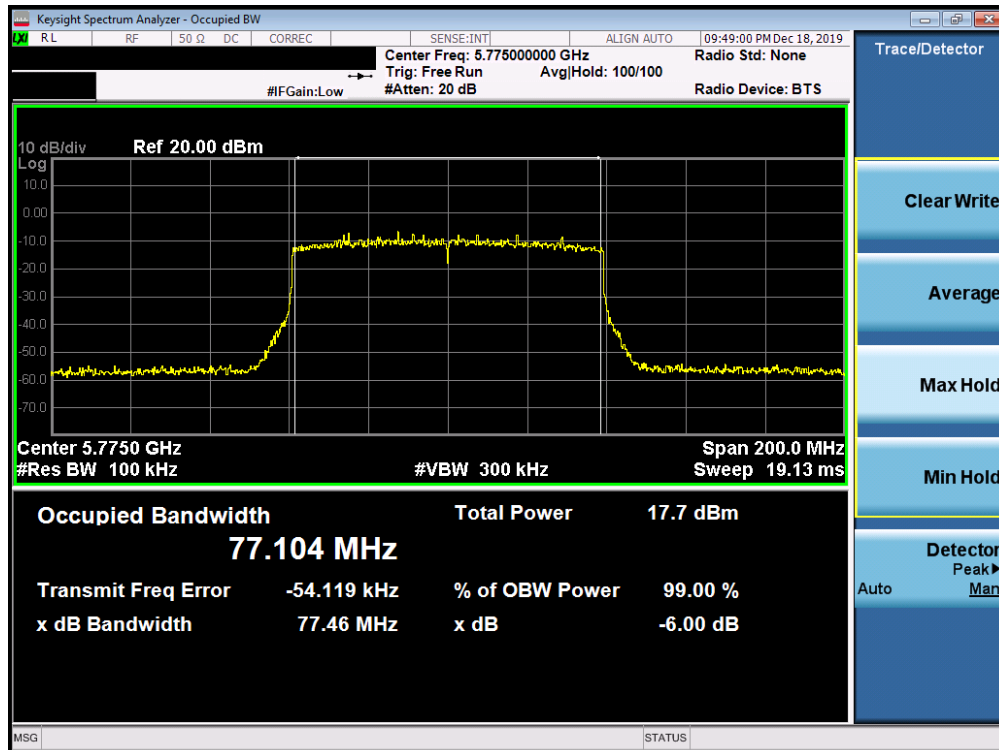
Plot 7-154. 6dB Bandwidth Plot SISO ANT1 (80MHz BW 802.11ax (UNII Band 3) – Ch. 155)
