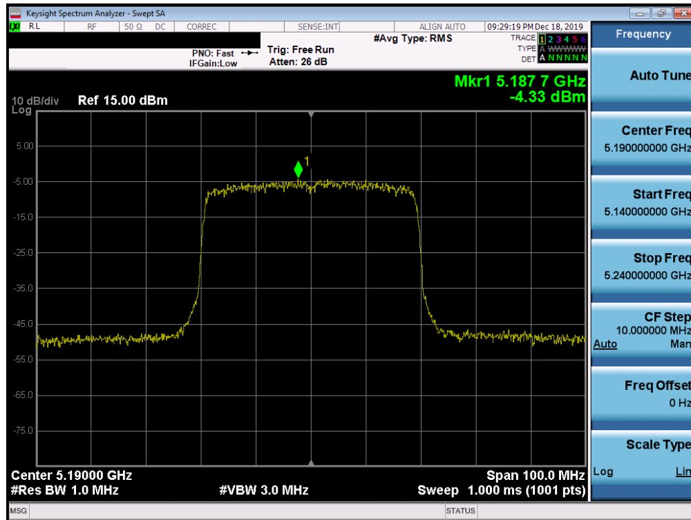
Plot 7-191. Power Spectral Density Plot SISO ANT1 (40MHz BW 802.11ax (UNII Band 1) – Ch. 38)
