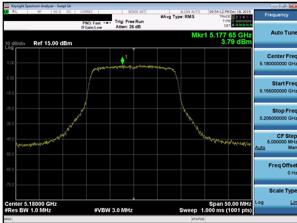
Plot 7-181. Power Spectral Density Plot SISO ANT1 (20MHz BW 802.11ac (UNII Band 1) – Ch. 36)
