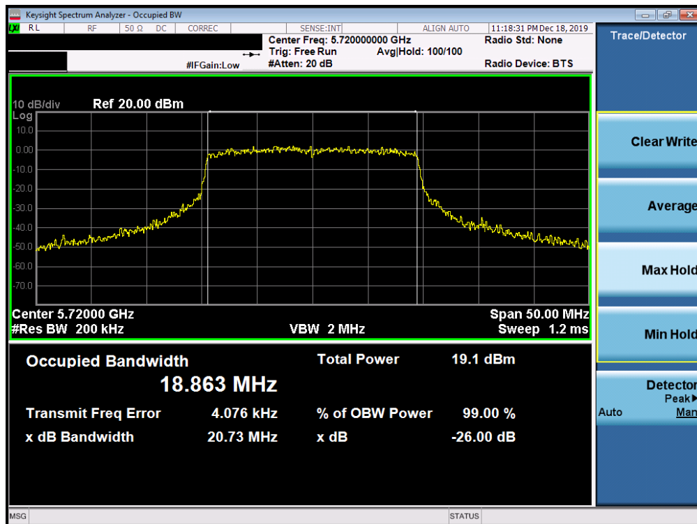
Plot 7-119. 26dB Bandwidth Plot SISO ANT2 (20MHz BW 802.11ax (UNII Band 2C) – Ch. 144)
