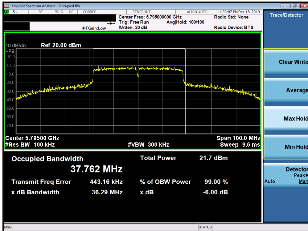
Plot 7-168. 6dB Bandwidth Plot SISO ANT2 (40MHz BW 802.11n (UNII Band 3) – Ch. 159)
