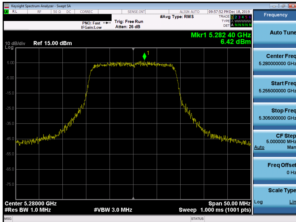
Plot 7-202. Power Spectral Density Plot SISO ANT1 (20MHz BW 802.11ac (UNII Band 2A) – Ch. 56)
