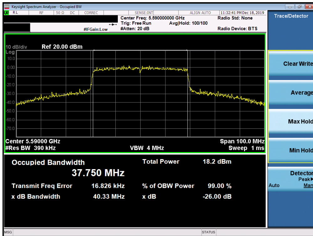
Plot 7-127. 26dB Bandwidth Plot SISO ANT2 (40MHz BW 802.11ax (UNII Band 2C) – Ch. 118)
