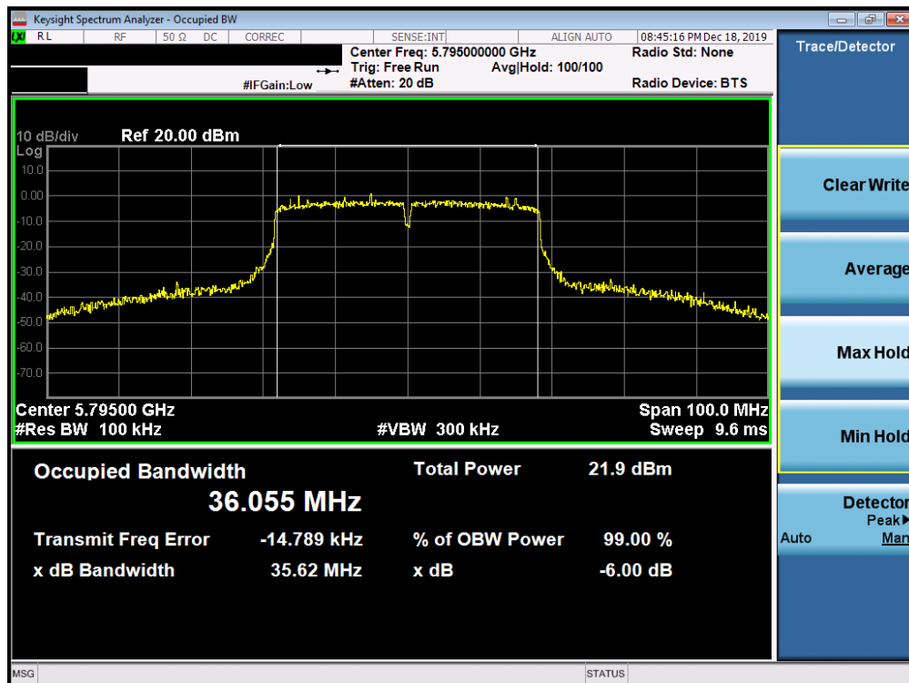
Plot 7-148. 6dB Bandwidth Plot SISO ANT1 (40MHz BW 802.11n (UNII Band 3) – Ch. 159)
