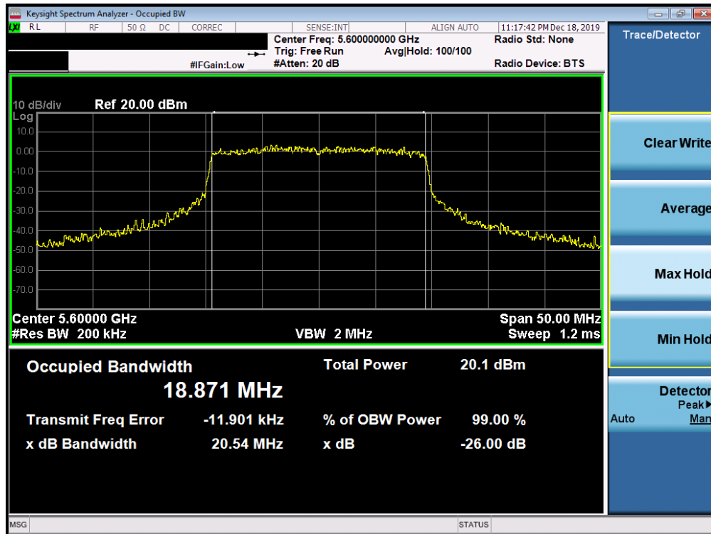
Plot 7-118. 26dB Bandwidth Plot SISO ANT2 (20MHz BW 802.11ax (UNII Band 2C) – Ch. 120)
