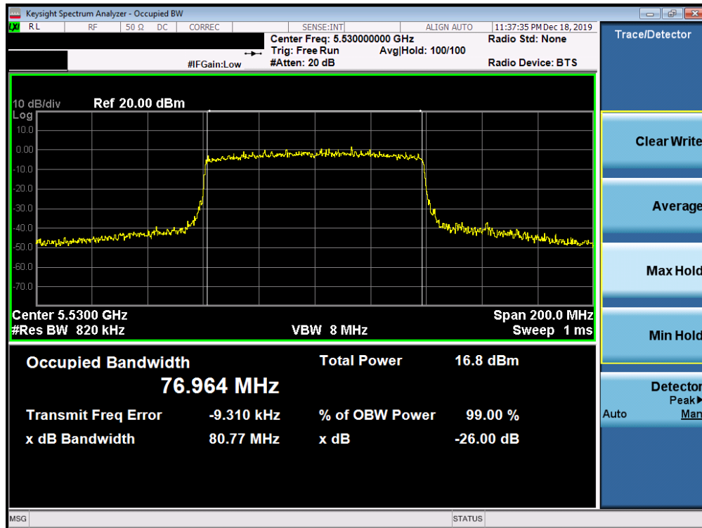
Plot 7-132. 26dB Bandwidth Plot SISO ANT2 (80MHz BW 802.11ax (UNII Band 2C) – Ch. 106)
