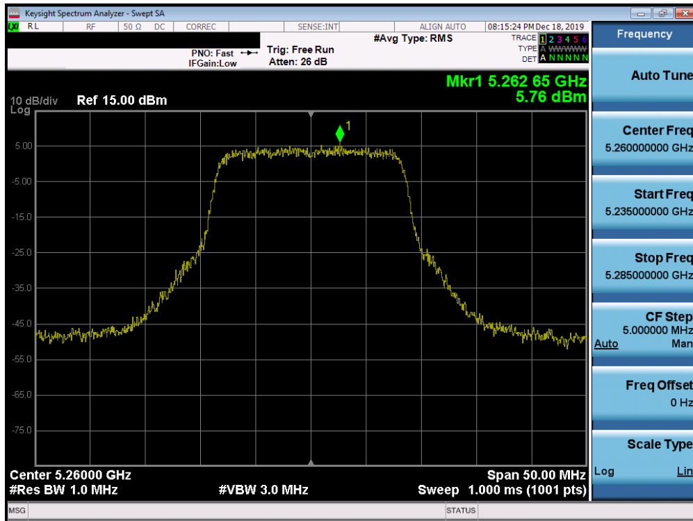
Plot 7-195. Power Spectral Density Plot SISO ANT1 (802.11a (UNII Band 2A) – Ch. 52)
