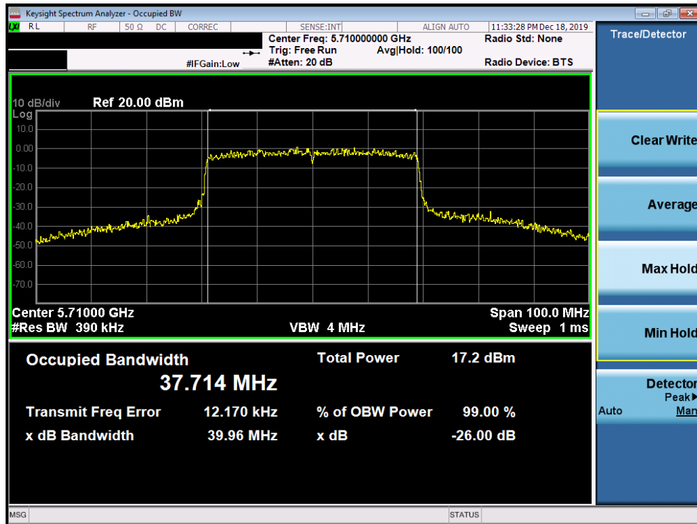
Plot 7-128. 26dB Bandwidth Plot SISO ANT2 (40MHz BW 802.11ax (UNII Band 2C) – Ch. 142)
