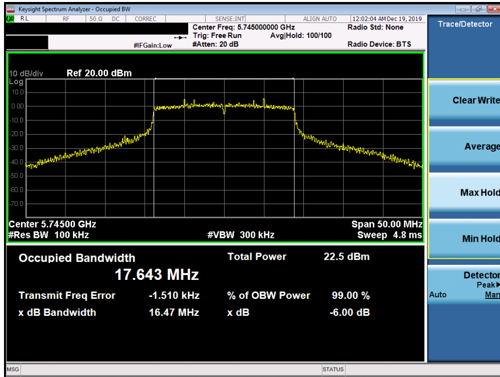
Plot 7-161. 6dB Bandwidth Plot SISO ANT2 (20MHz BW 802.11ac (UNII Band 3) – Ch. 149)
