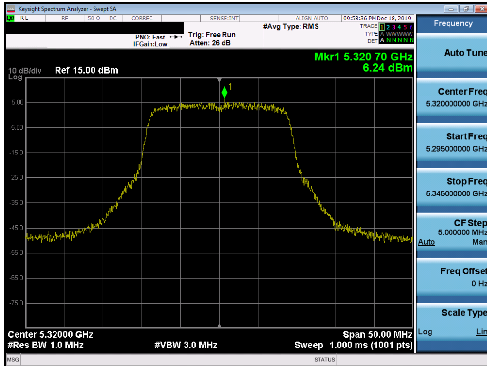
Plot 7-203. Power Spectral Density Plot SISO ANT1 (20MHz BW 802.11ac (UNII Band 2A) – Ch. 64)
