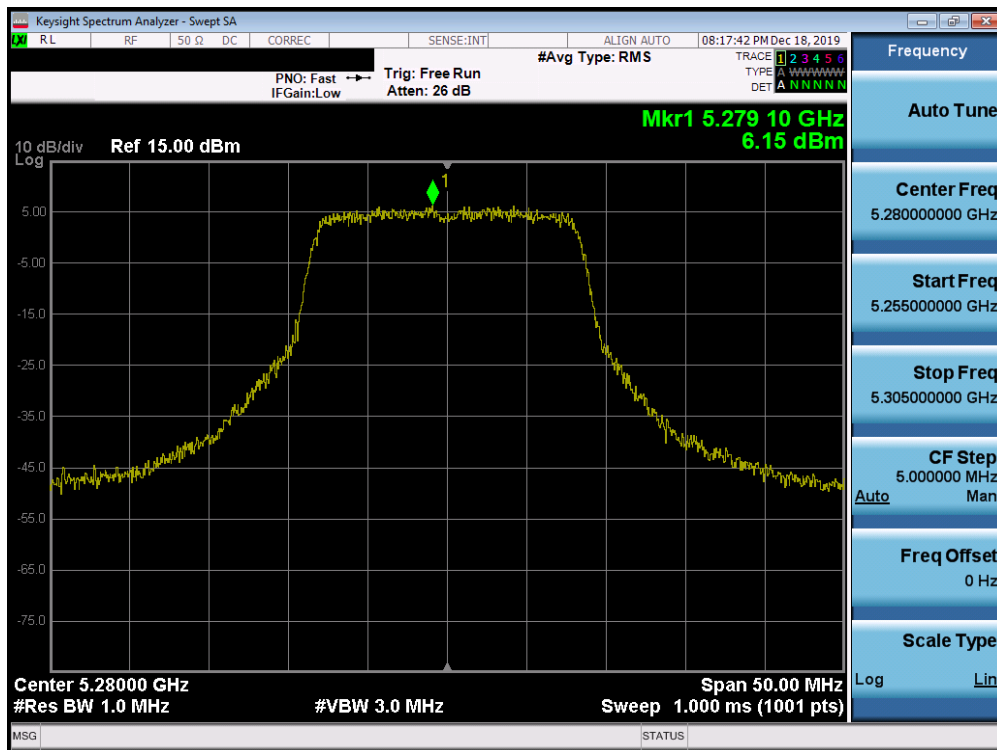
Plot 7-196. Power Spectral Density Plot SISO ANT1 (802.11a (UNII Band 2A) – Ch. 56)
