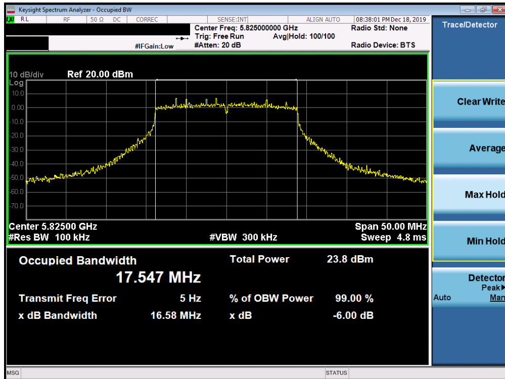
Plot 7-140. 6dB Bandwidth Plot SISO ANT1 (20MHz BW 802.11n (UNII Band 3) – Ch. 165)
