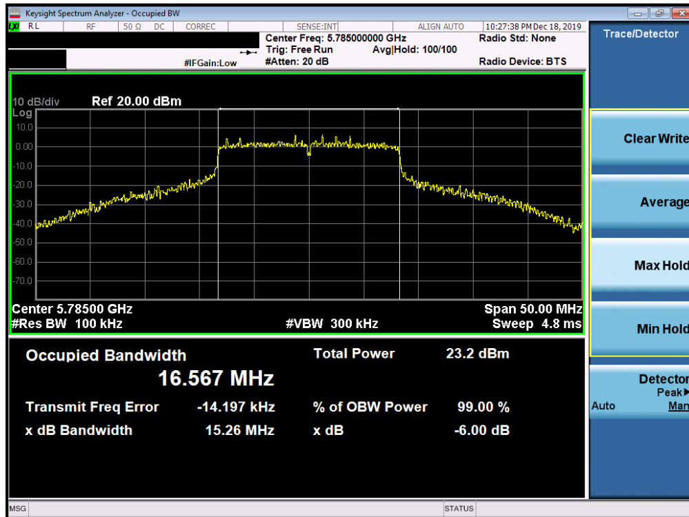
Plot 7-156. 6dB Bandwidth Plot SISO ANT2 (802.11a (UNII Band 3) – Ch. 157)
