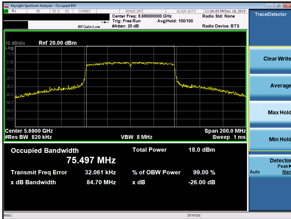
Plot 7-131. 26dB Bandwidth Plot SISO ANT2 (80MHz BW 802.11ac (UNII Band 2C) – Ch. 138)
