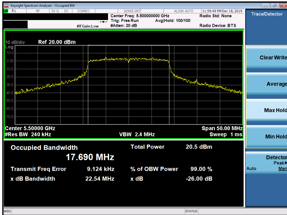
Plot 7-114. 26dB Bandwidth Plot SISO ANT2 (20MHz BW 802.11ac (UNII Band 2C) – Ch. 100)
