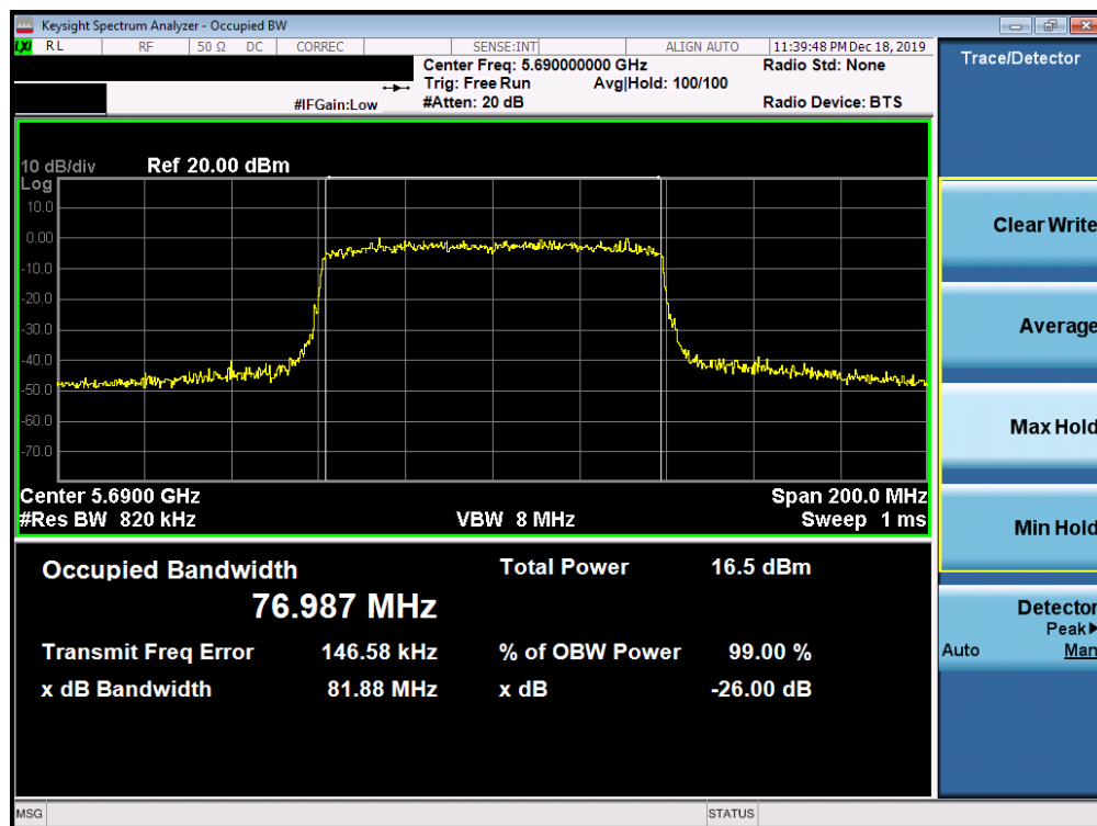
Plot 7-134. 26dB Bandwidth Plot SISO ANT2 (80MHz BW 802.11ax (UNII Band 2C) – Ch. 138
