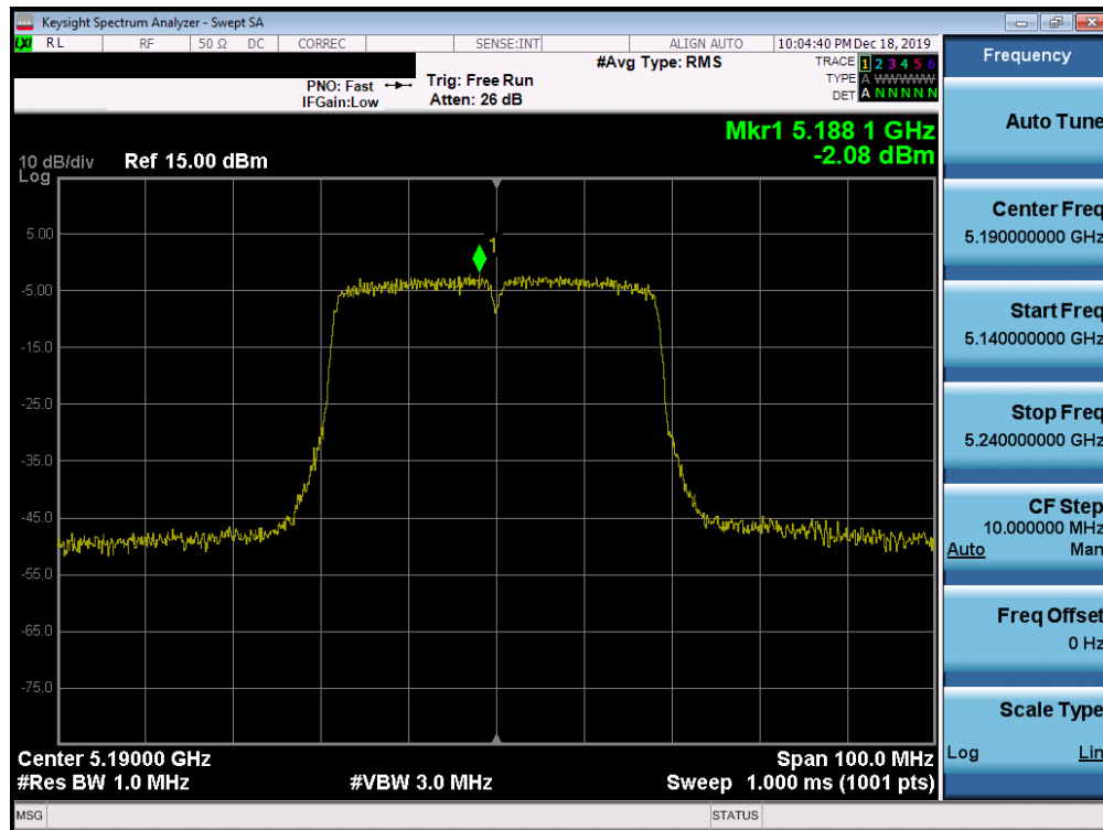
Plot 7-189. Power Spectral Density Plot SISO ANT1 (40MHz BW 802.11ac (UNII Band 1) – Ch. 38)
