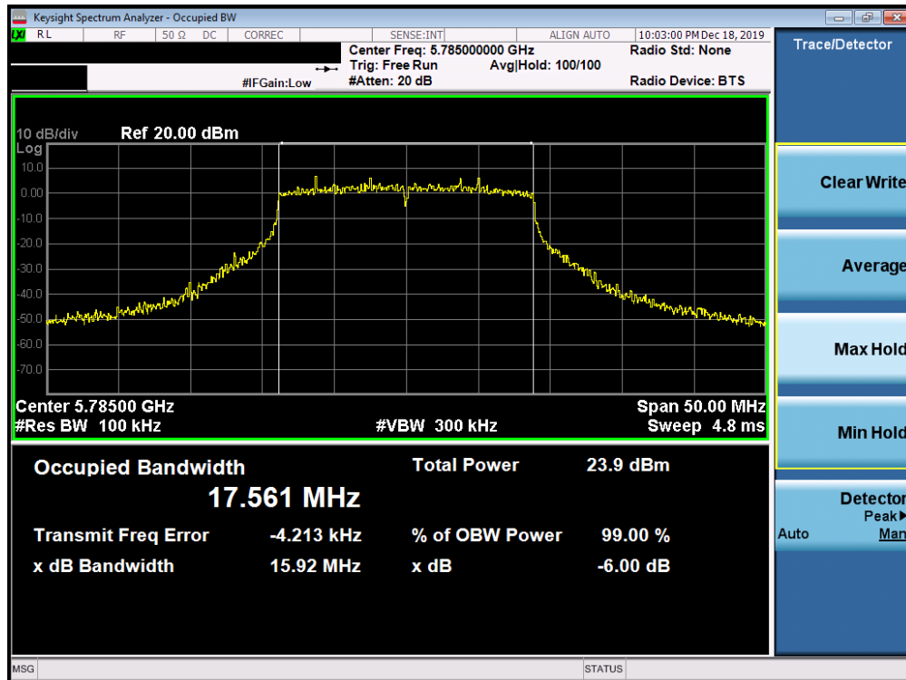
Plot 7-142. 6dB Bandwidth Plot SISO ANT1 (20MHz BW 802.11ac (UNII Band 3) – Ch. 157)
