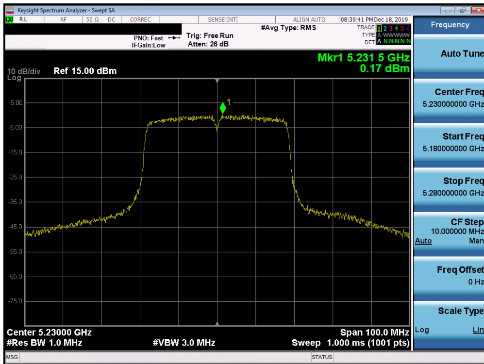
Plot 7-188. Power Spectral Density Plot SISO ANT1 (40MHz BW 802.11n (UNII Band 1) – Ch. 46)
