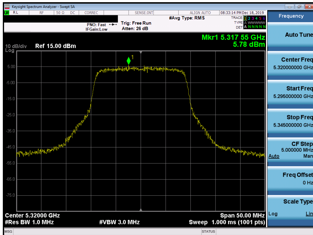
Plot 7-200. Power Spectral Density Plot SISO ANT1 (20MHz BW 802.11n (UNII Band 2A) – Ch. 64)
