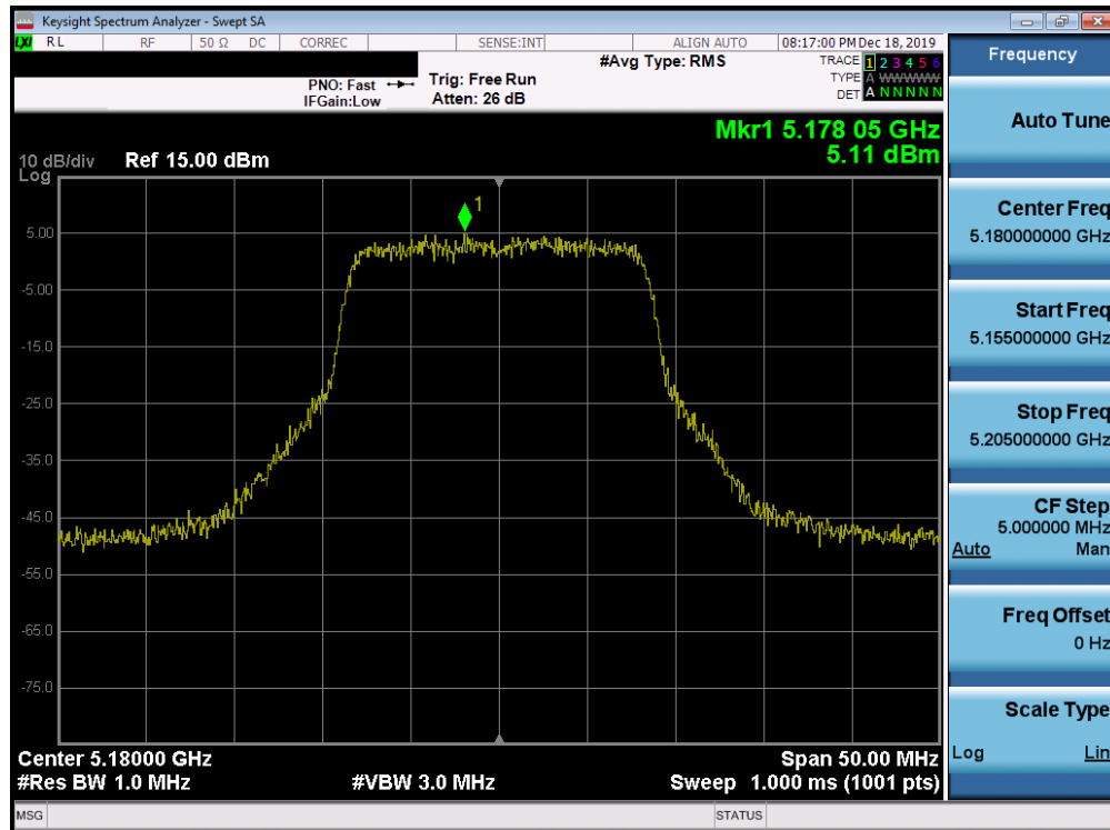
Plot 7-175. Power Spectral Density Plot SISO ANT1 (802.11a (UNII Band 1) – Ch. 36)
