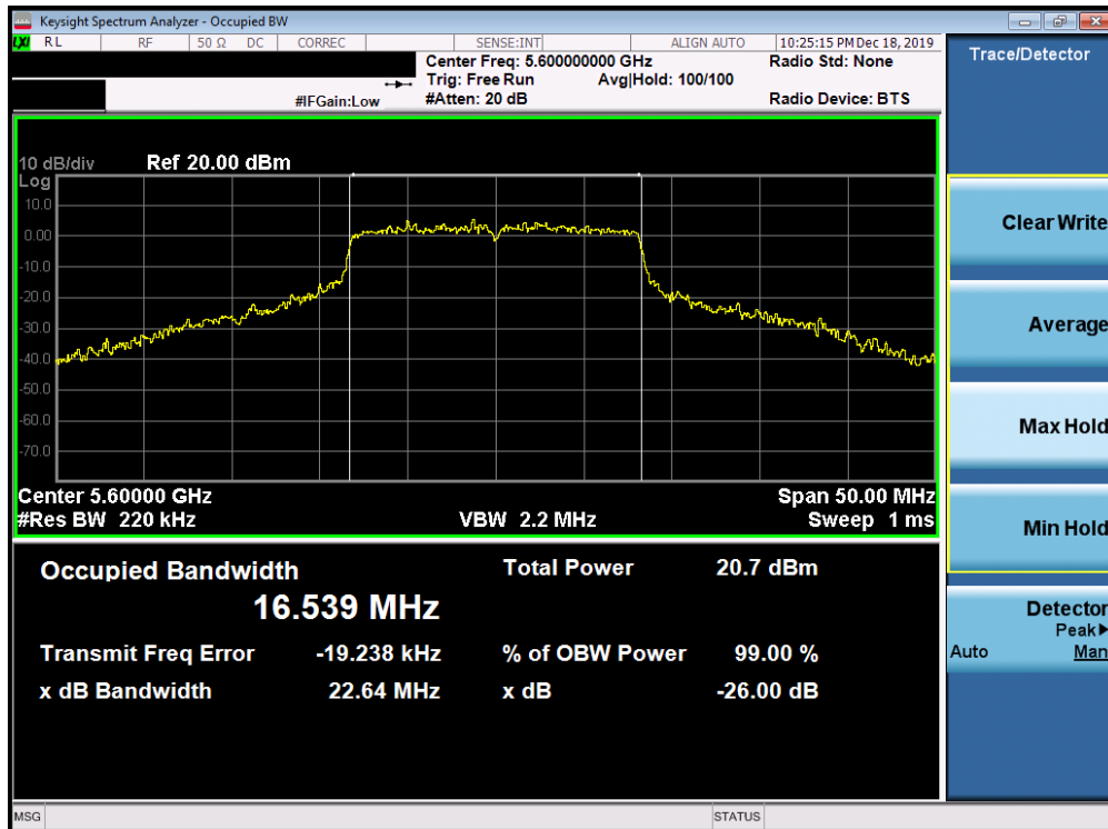
Plot 7-109. 26dB Bandwidth Plot SISO ANT2 (802.11a (UNII Band 2C) – Ch. 120)
