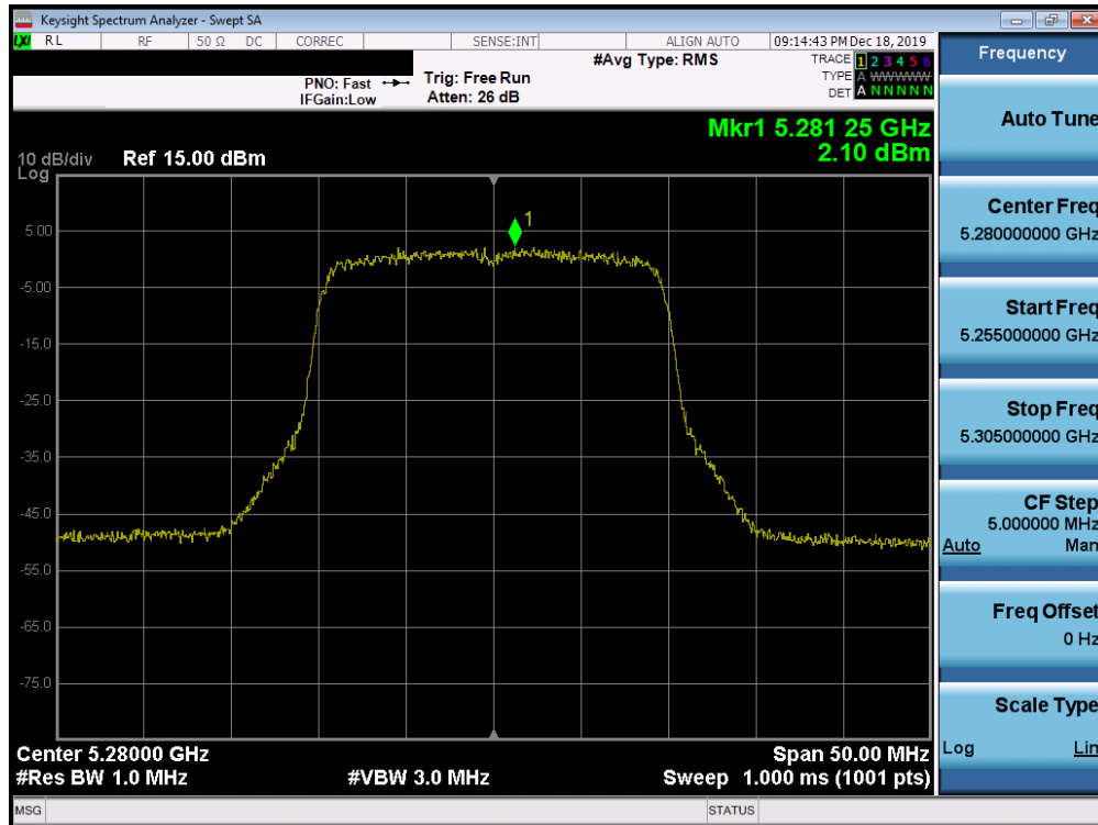
Plot 7-205. Power Spectral Density Plot SISO ANT1 (20MHz BW 802.11ax (UNII Band 2A) – Ch. 56)
