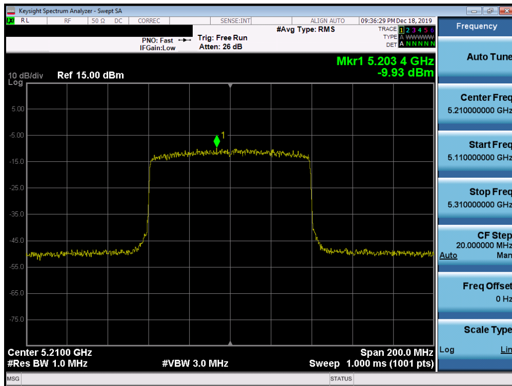
Plot 7-194. Power Spectral Density Plot SISO ANT1 (80MHz BW 802.11ax (UNII Band 1) – Ch. 42)
