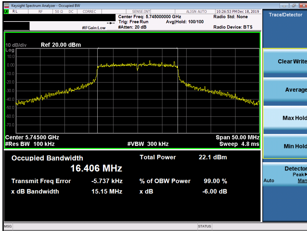
Plot 7-155. 6dB Bandwidth Plot SISO ANT2 (802.11a (UNII Band 3) – Ch. 149)
