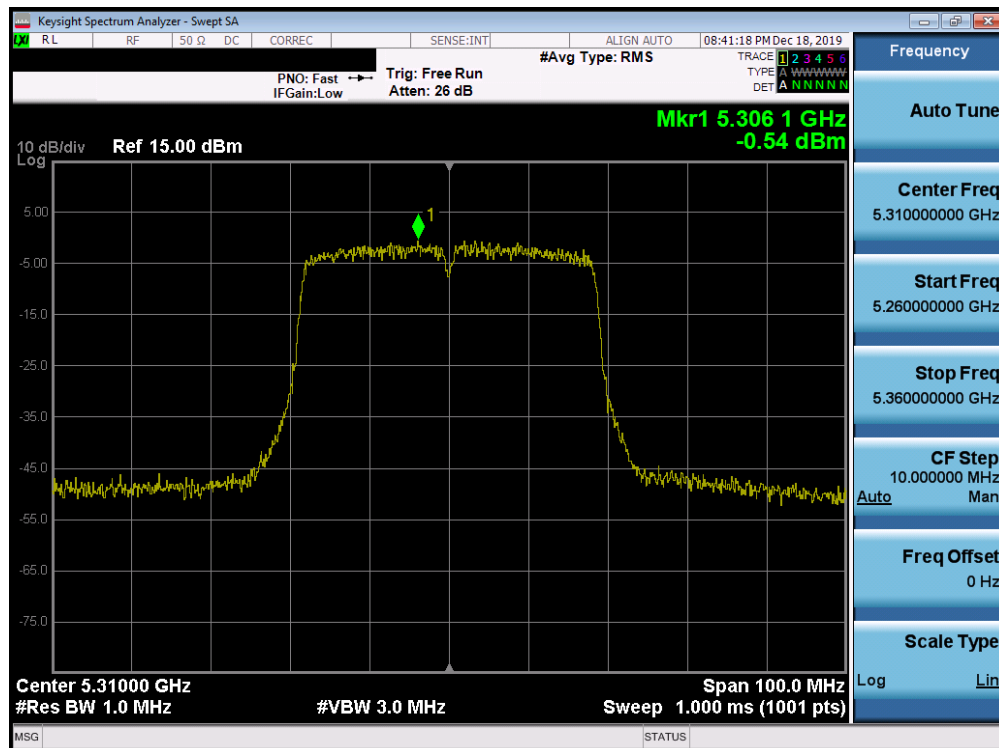
Plot 7-208. Power Spectral Density Plot SISO ANT1 (40MHz BW 802.11n (UNII Band 2A) – Ch. 62)
