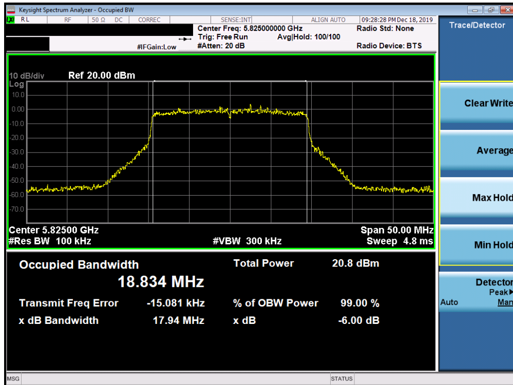
Plot 7-146. 6dB Bandwidth Plot SISO ANT1 (20MHz BW 802.11ax (UNII Band 3) – Ch. 165)
