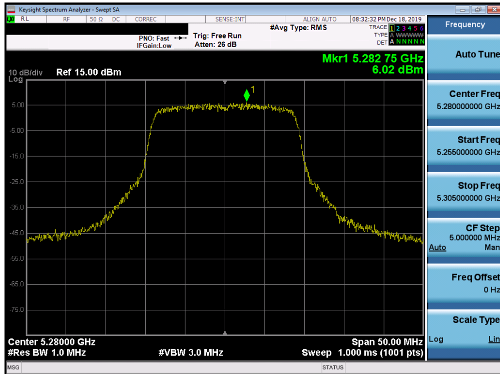
Plot 7-199. Power Spectral Density Plot SISO ANT1 (20MHz BW 802.11n (UNII Band 2A) – Ch. 56)
