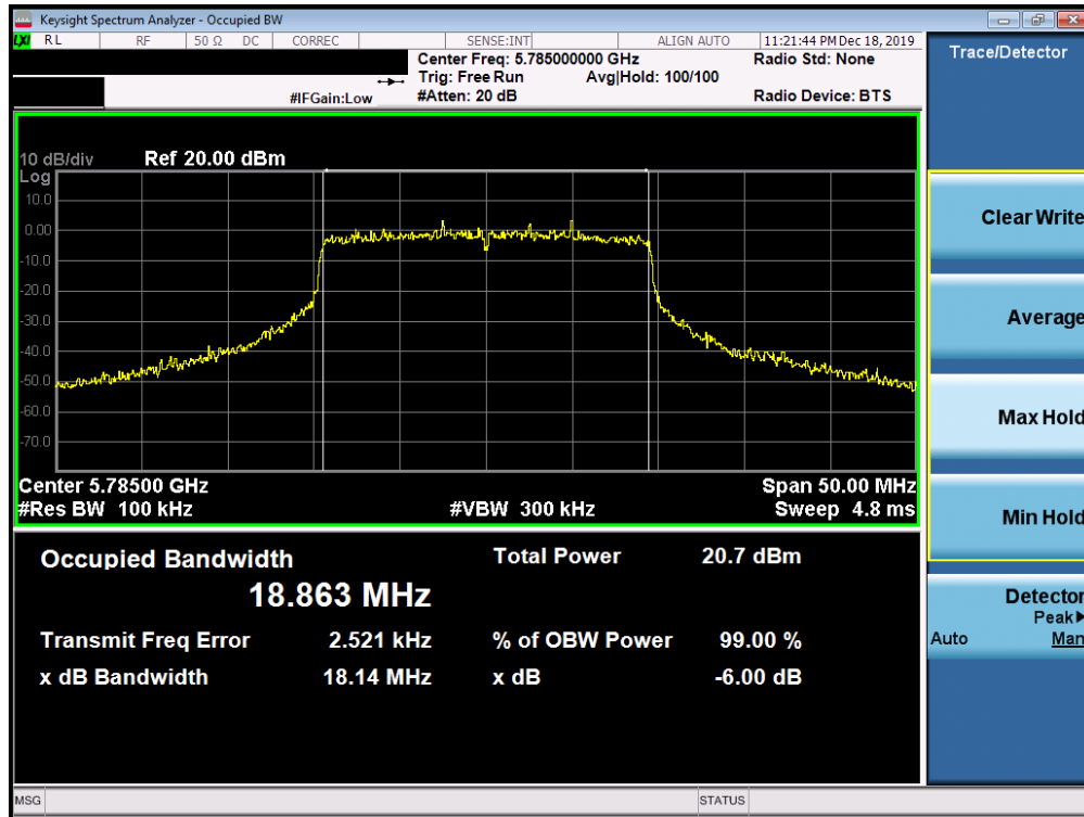
Plot 7-165. 6dB Bandwidth Plot SISO ANT2 (20MHz BW 802.11ax (UNII Band 3) – Ch. 157)
