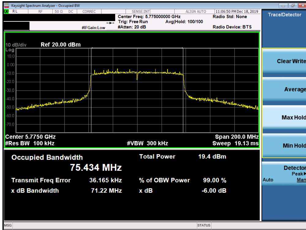
Plot 7-173. 6dB Bandwidth Plot SISO ANT2 (80MHz BW 802.11ac (UNII Band 3) – Ch. 155)
