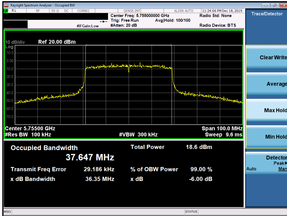
Plot 7-171. 6dB Bandwidth Plot SISO ANT2 (40MHz BW 802.11ax (UNII Band 3) – Ch. 151)
