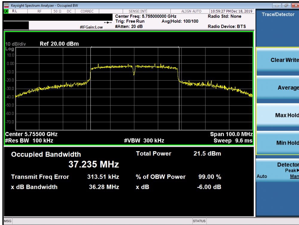
Plot 7-167. 6dB Bandwidth Plot SISO ANT2 (40MHz BW 802.11n (UNII Band 3) – Ch. 151)
