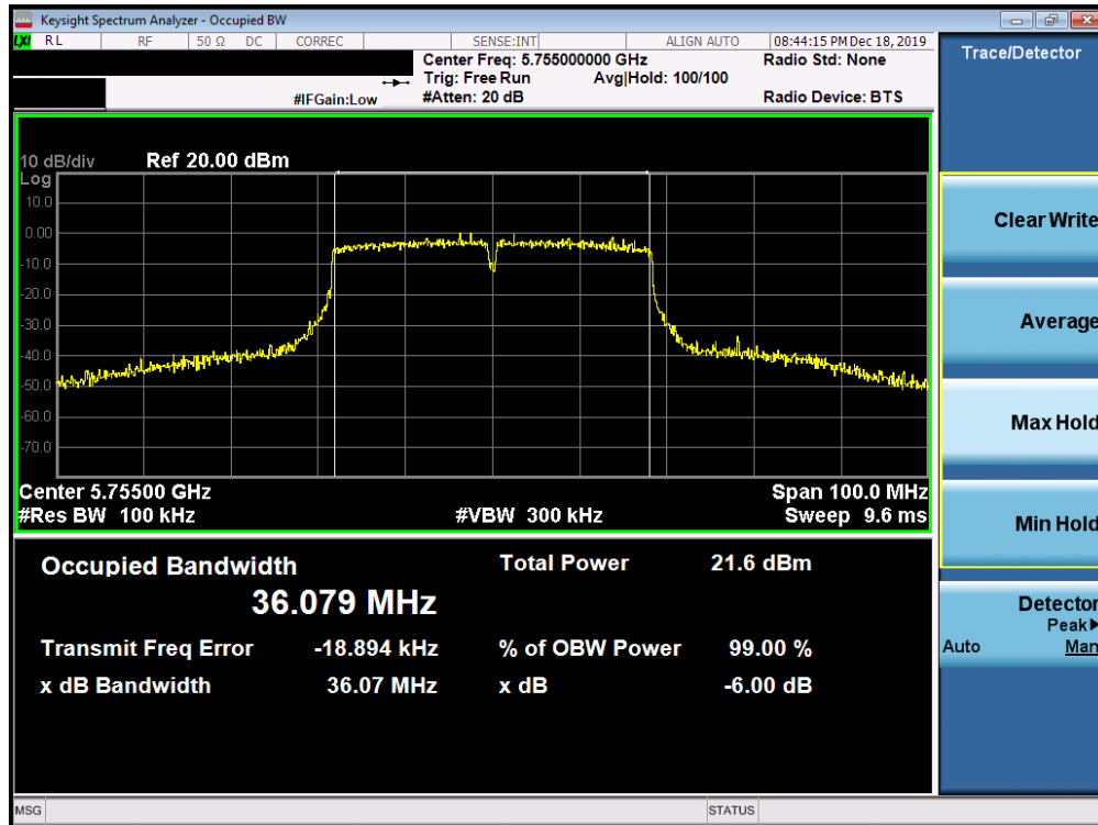
Plot 7-147. 6dB Bandwidth Plot SISO ANT1 (40MHz BW 802.11n (UNII Band 3) – Ch. 151)
