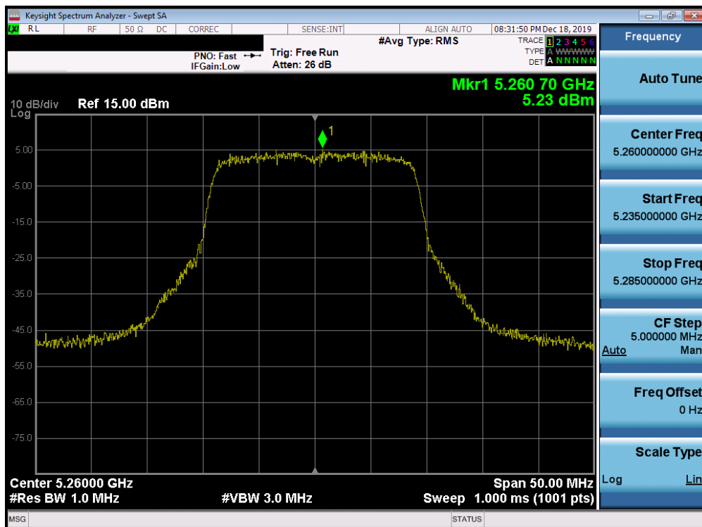
Plot 7-198. Power Spectral Density Plot SISO ANT1 (20MHz BW 802.11n (UNII Band 2A) – Ch. 52)
