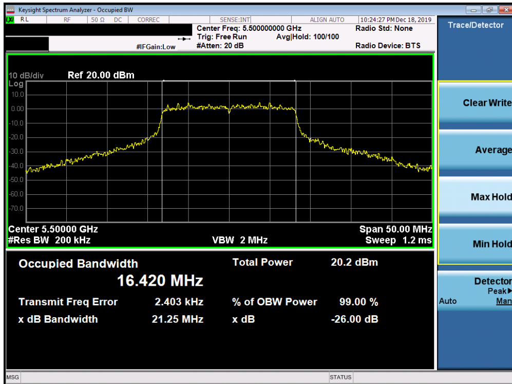
Plot 7-108. 26dB Bandwidth Plot SISO ANT2 (802.11a (UNII Band 2C) – Ch. 100)
