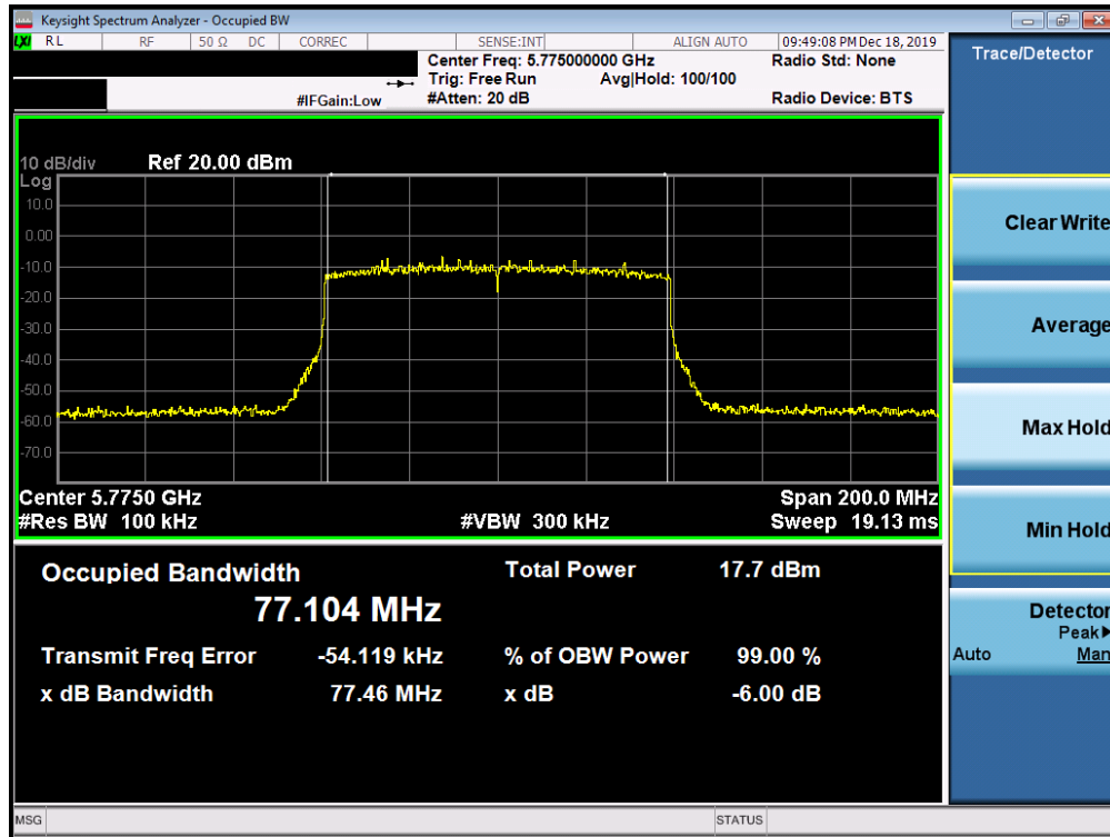
Plot 7-153. 6dB Bandwidth Plot SISO ANT1 (80MHz BW 802.11ac (UNII Band 3) – Ch. 155)
