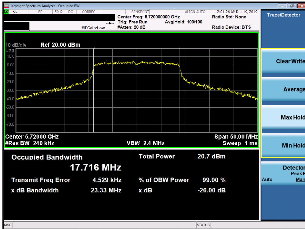
Plot 7-116. 26dB Bandwidth Plot SISO ANT2 (20MHz BW 802.11ac (UNII Band 2C) – Ch. 144)
