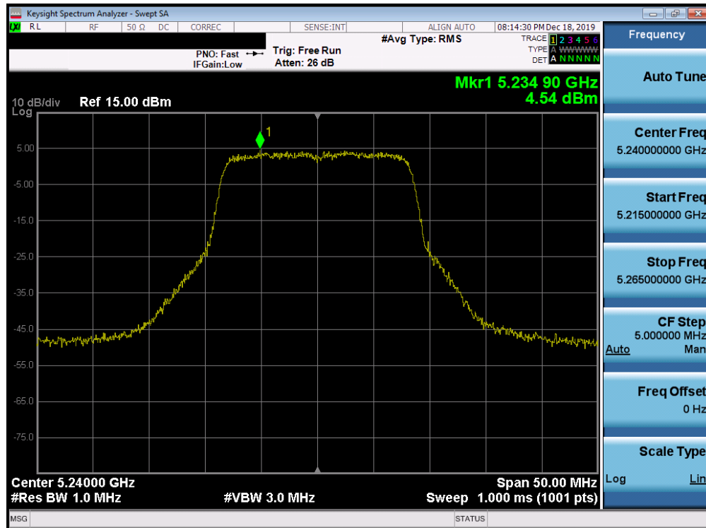
Plot 7-177. Power Spectral Density Plot SISO ANT1 (802.11a (UNII Band 1) – Ch. 48)
