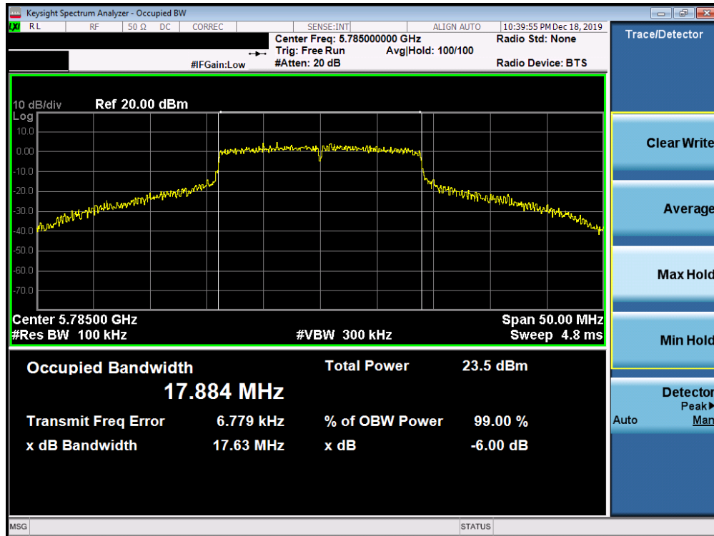
Plot 7-159. 6dB Bandwidth Plot SISO ANT2 (20MHz BW 802.11n (UNII Band 3) – Ch. 157)
