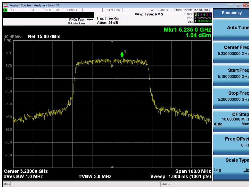
Plot 7-190. Power Spectral Density Plot SISO ANT1 (40MHz BW 802.11ac (UNII Band 1) – Ch. 46)
