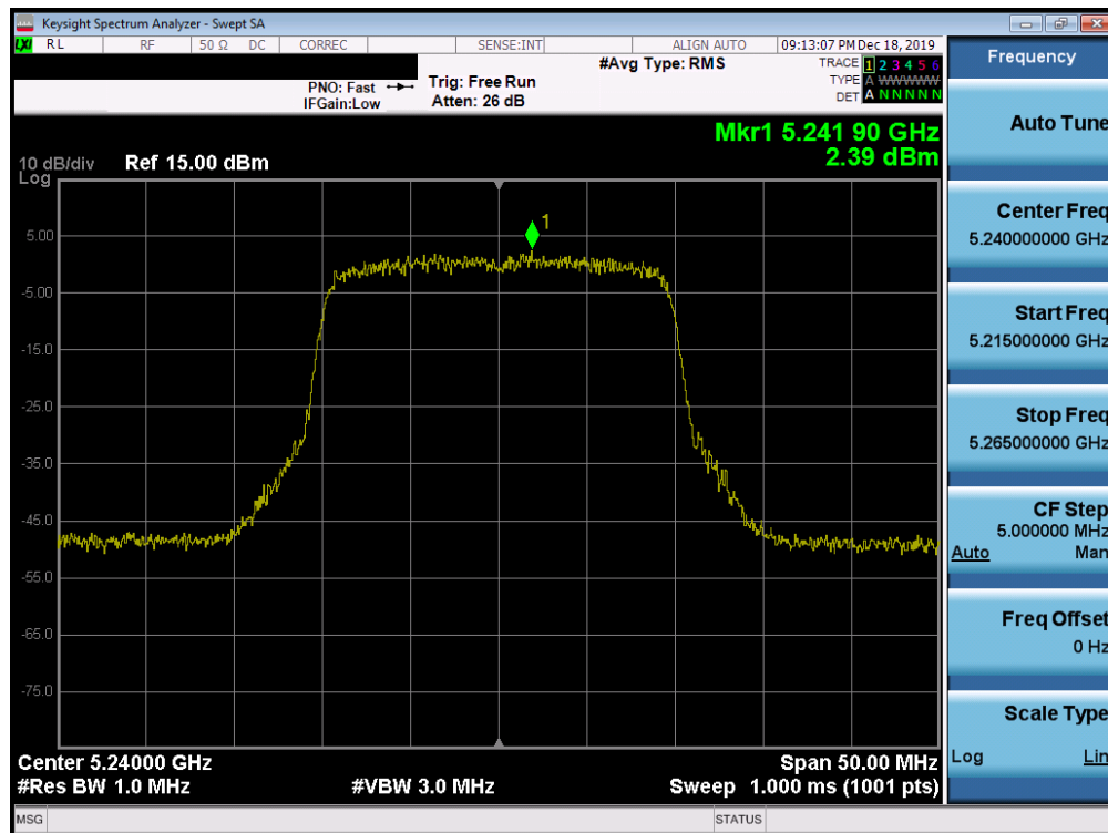
Plot 7-186. Power Spectral Density Plot SISO ANT1 (20MHz BW 802.11ax (UNII Band 1) – Ch. 48)
