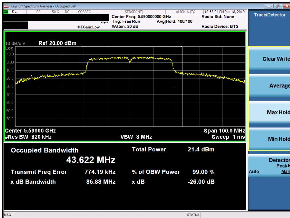
Plot 7-121. 26dB Bandwidth Plot SISO ANT2 (40MHz BW 802.11n (UNII Band 2C) – Ch. 118)
