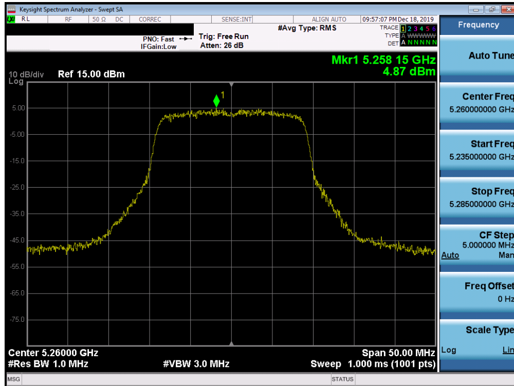
Plot 7-201. Power Spectral Density Plot SISO ANT1 (20MHz BW 802.11ac (UNII Band 2A) – Ch. 52)
