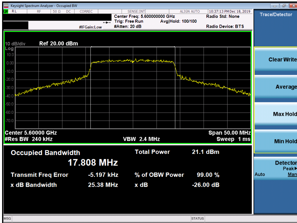
Plot 7-112. 26dB Bandwidth Plot SISO ANT2 (20MHz BW 802.11n (UNII Band 2C) – Ch. 120)
