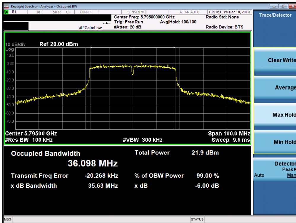
Plot 7-150. 6dB Bandwidth Plot SISO ANT1 (40MHz BW 802.11ac (UNII Band 3) – Ch. 159)
