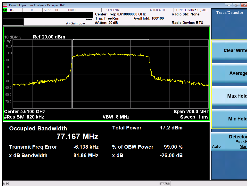
Plot 7-133. 26dB Bandwidth Plot SISO ANT2 (80MHz BW 802.11ax (UNII Band 2C) – Ch. 122)
