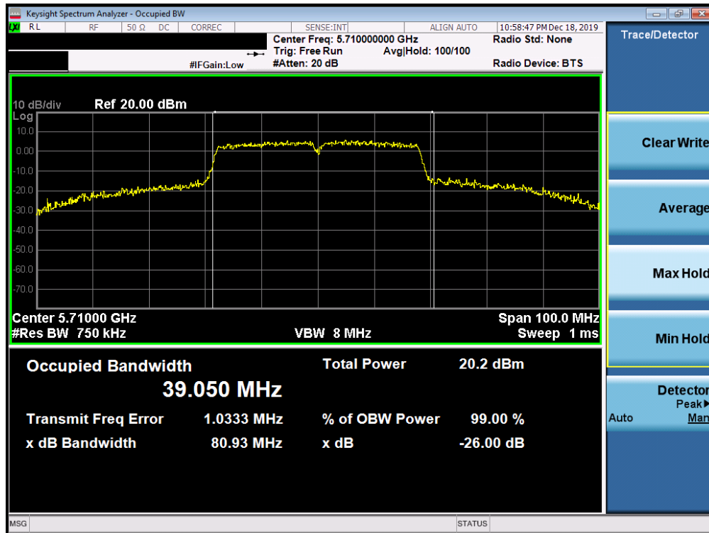
Plot 7-122. 26dB Bandwidth Plot SISO ANT2 (40MHz BW 802.11n (UNII Band 2C) – Ch. 142)
