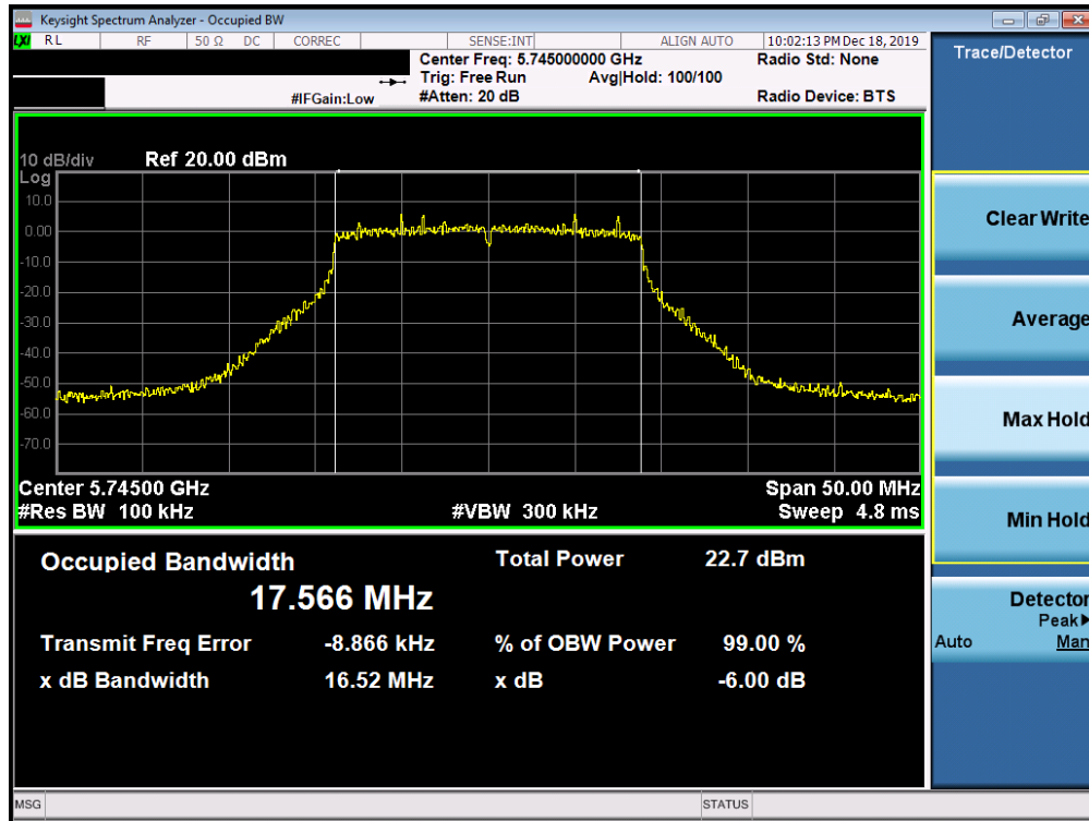
Plot 7-141. 6dB Bandwidth Plot SISO ANT1 (20MHz BW 802.11ac (UNII Band 3) – Ch. 149)
