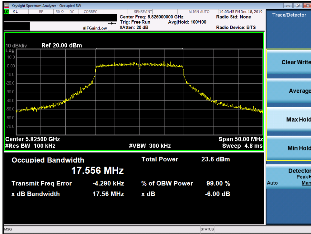
Plot 7-143. 6dB Bandwidth Plot SISO ANT1 (20MHz BW 802.11ac (UNII Band 3) – Ch. 165)
