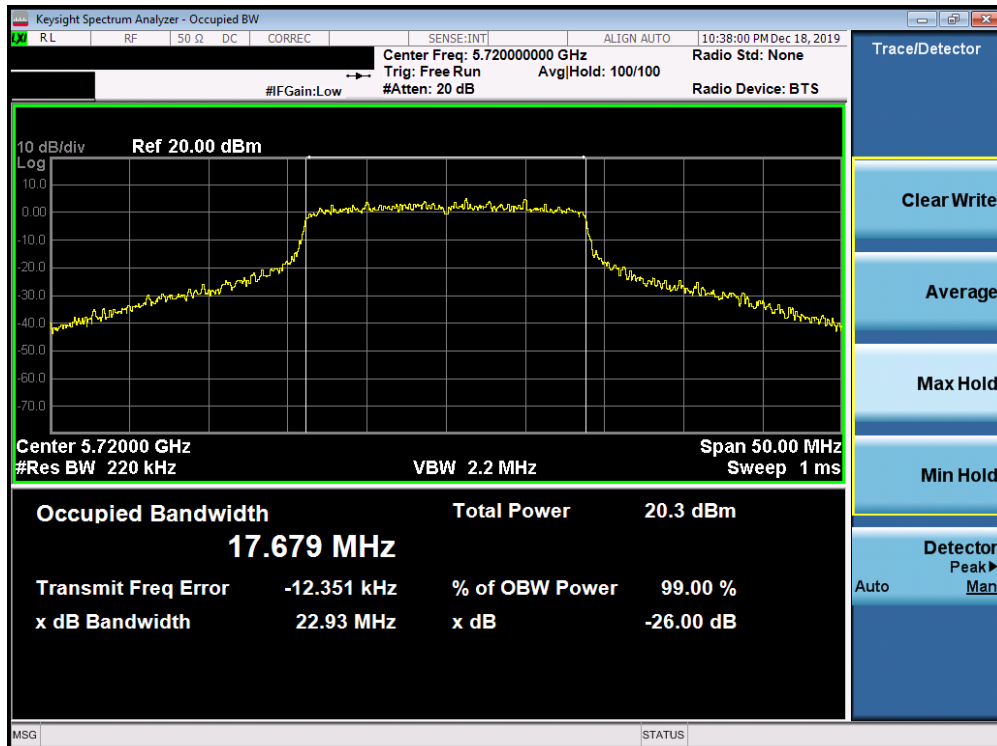
Plot 7-113. 26dB Bandwidth Plot SISO ANT2 (20MHz BW 802.11n (UNII Band 2C) – Ch. 144)
