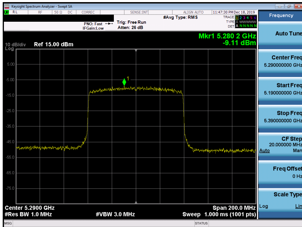
Plot 7-214. Power Spectral Density Plot SISO ANT1 (80MHz BW 802.11ax (UNII Band 2A) – Ch. 58)
