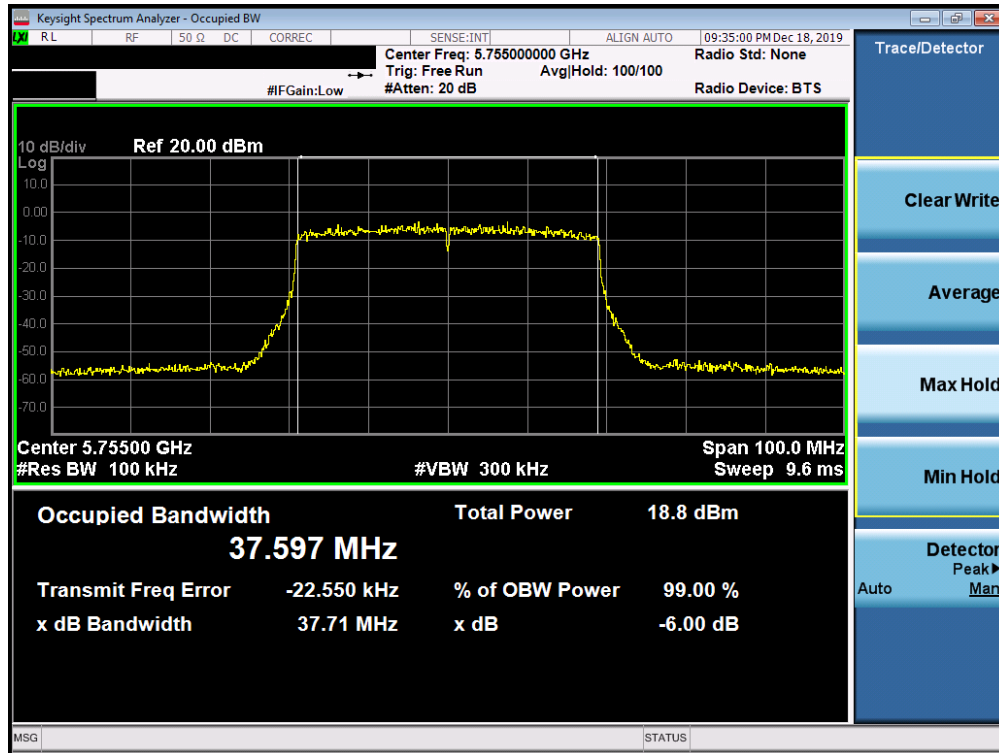
Plot 7-151. 6dB Bandwidth Plot SISO ANT1 (40MHz BW 802.11ax (UNII Band 3) – Ch. 151)
