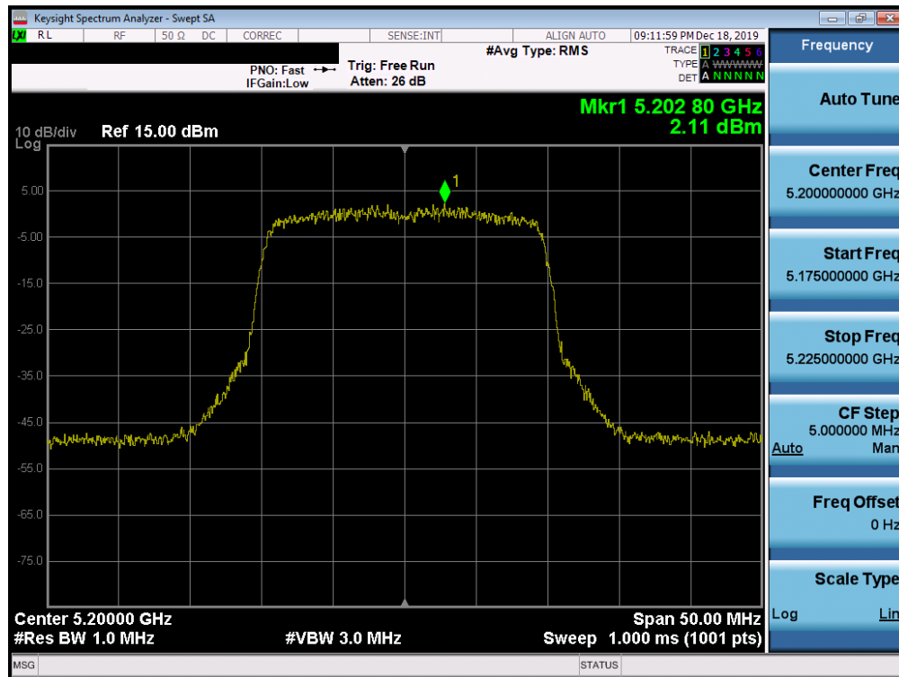
Plot 7-185. Power Spectral Density Plot SISO ANT1 (20MHz BW 802.11ax (UNII Band 1) – Ch. 40)
