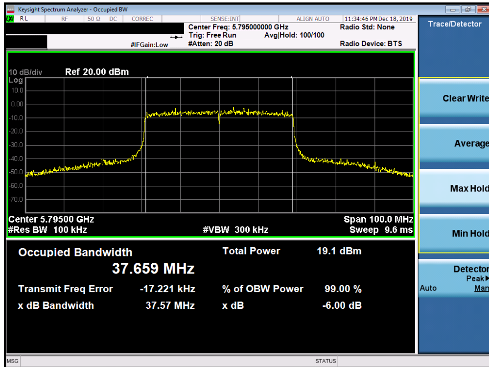
Plot 7-172. 6dB Bandwidth Plot SISO ANT1 (40MHz BW 802.11ax (UNII Band 3) – Ch. 159)
