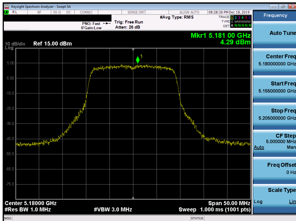
Plot 7-178. Power Spectral Density Plot SISO ANT1 (20MHz BW 802.11n (UNII Band 1) – Ch. 36)
