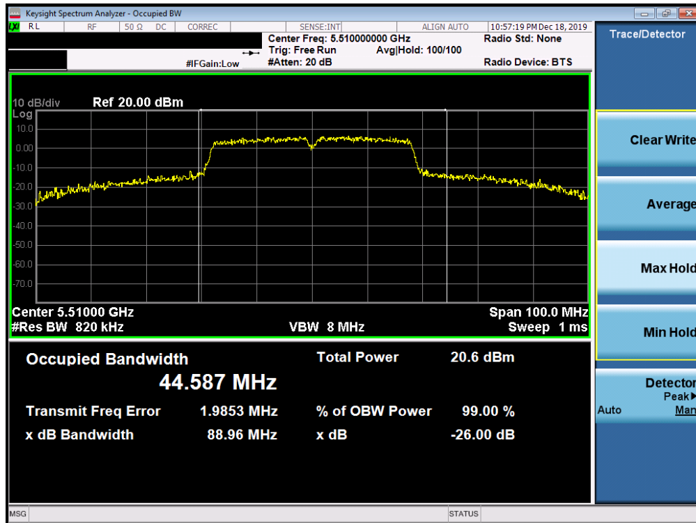
Plot 7-120. 26dB Bandwidth Plot SISO ANT2 (40MHz BW 802.11n (UNII Band 2C) – Ch. 102)
