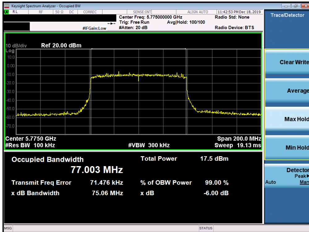
Plot 7-174. 6dB Bandwidth Plot SISO ANT2 (80MHz BW 802.11ax (UNII Band 3) – Ch. 155)
