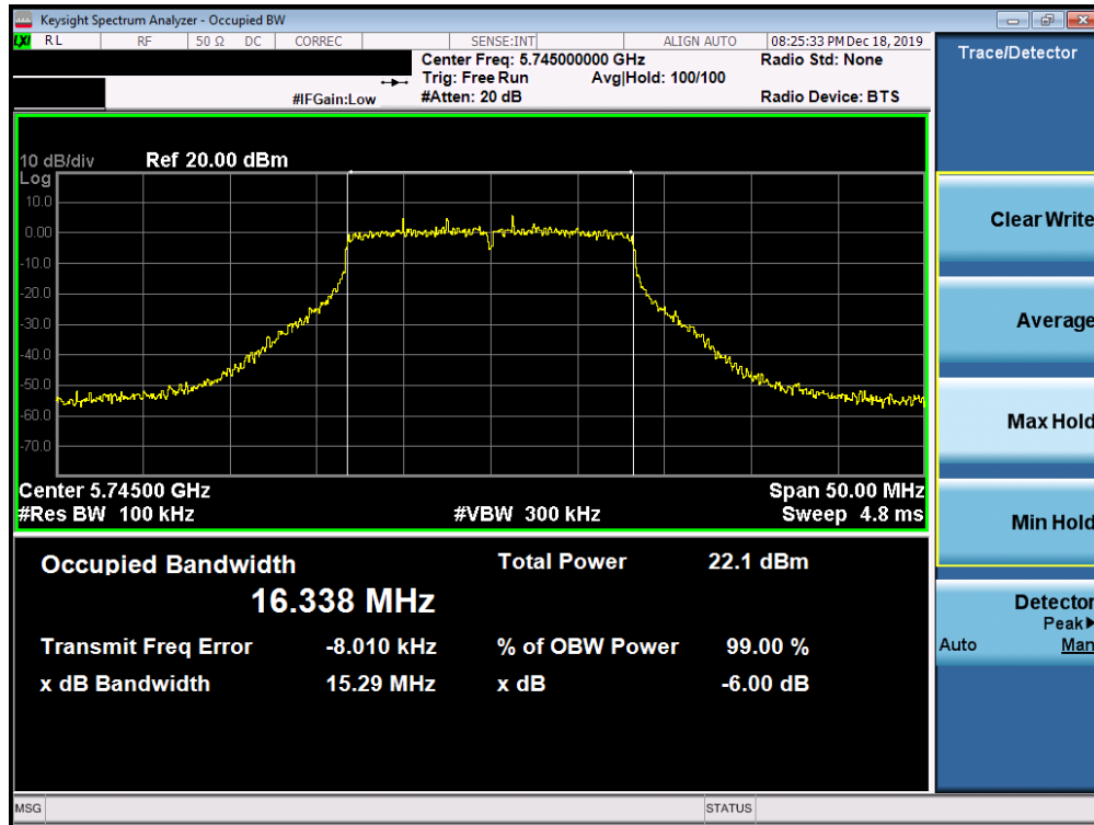
Plot 7-135. 6dB Bandwidth Plot SISO ANT1 (802.11a (UNII Band 3) – Ch. 149)
