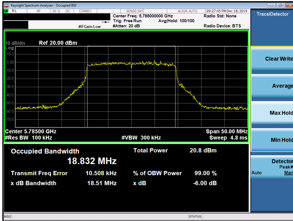
Plot 7-145. 6dB Bandwidth Plot SISO ANT1 (20MHz BW 802.11ax (UNII Band 3) – Ch. 157)
