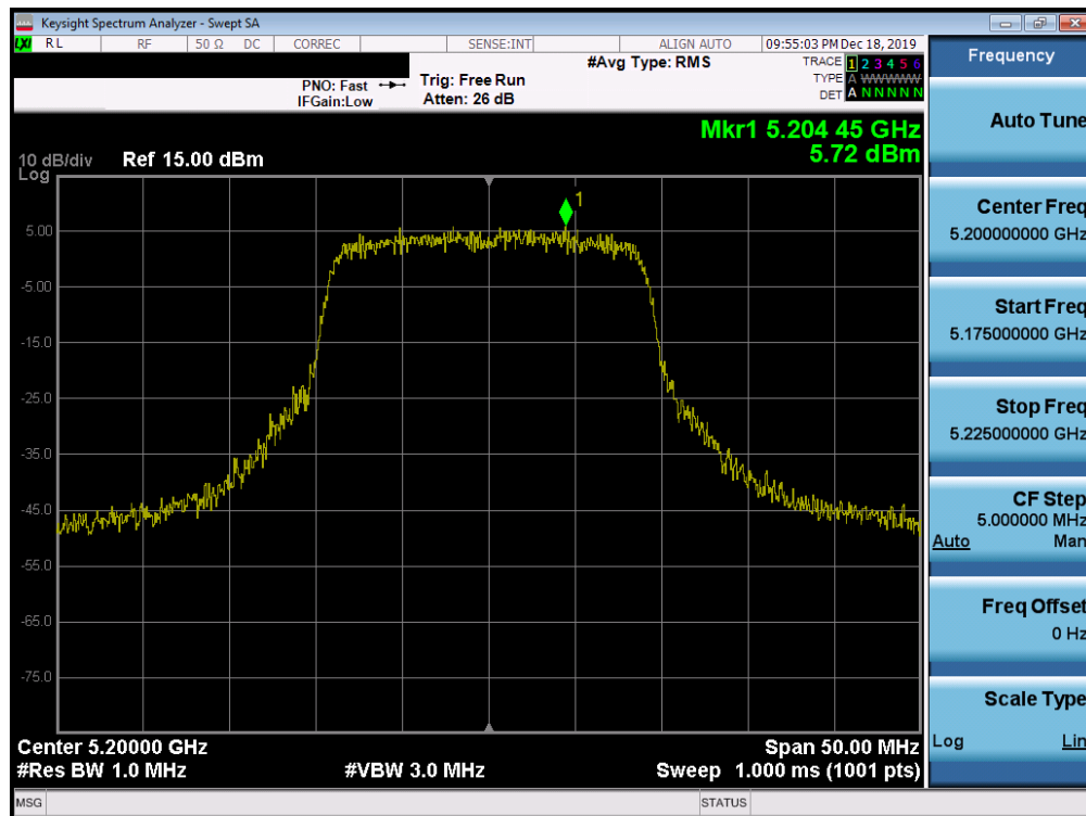
Plot 7-182. Power Spectral Density Plot SISO ANT1 (20MHz BW 802.11ac (UNII Band 1) – Ch. 40)
