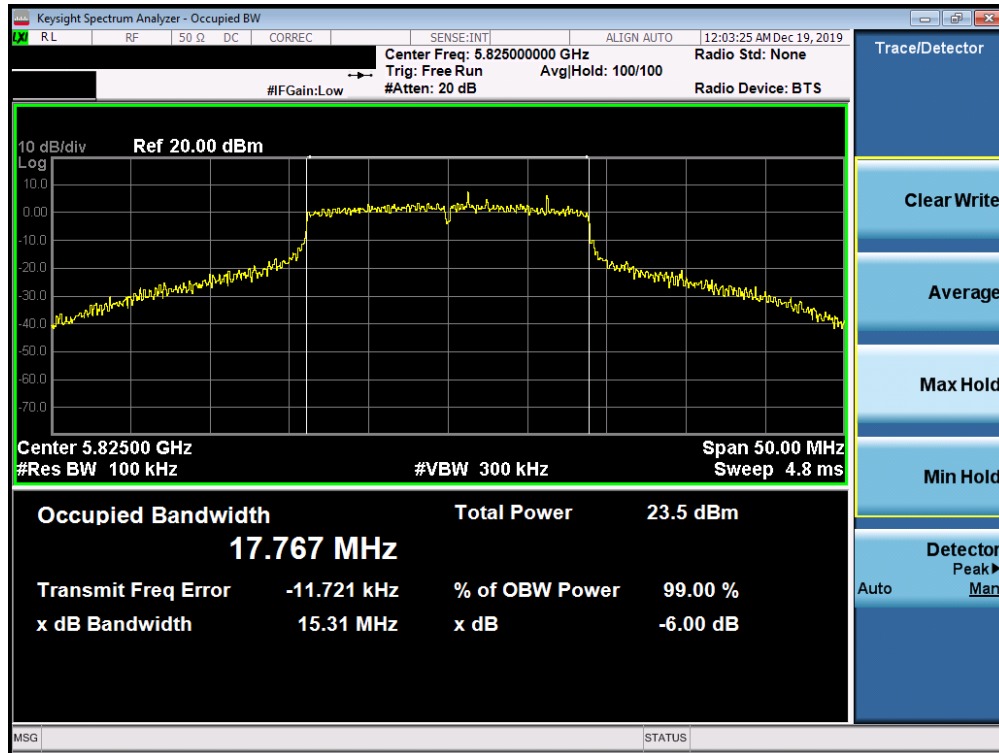
Plot 7-163. 6dB Bandwidth Plot SISO ANT2 (20MHz BW 802.11ac (UNII Band 3) – Ch. 165)
