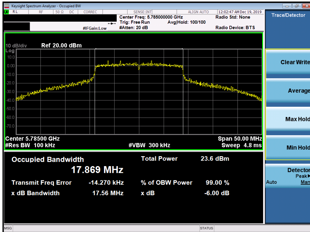
Plot 7-162. 6dB Bandwidth Plot SISO ANT2 (20MHz BW 802.11ac (UNII Band 3) – Ch. 157)
