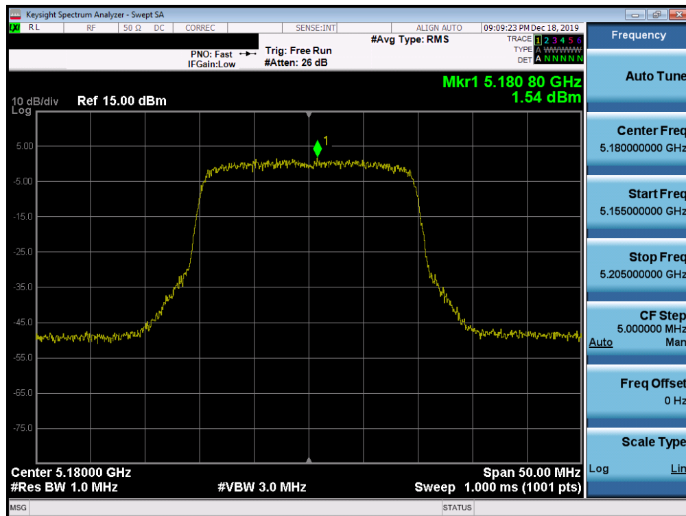
Plot 7-184. Power Spectral Density Plot SISO ANT1 (20MHz BW 802.11ax (UNII Band 1) – Ch. 36)
