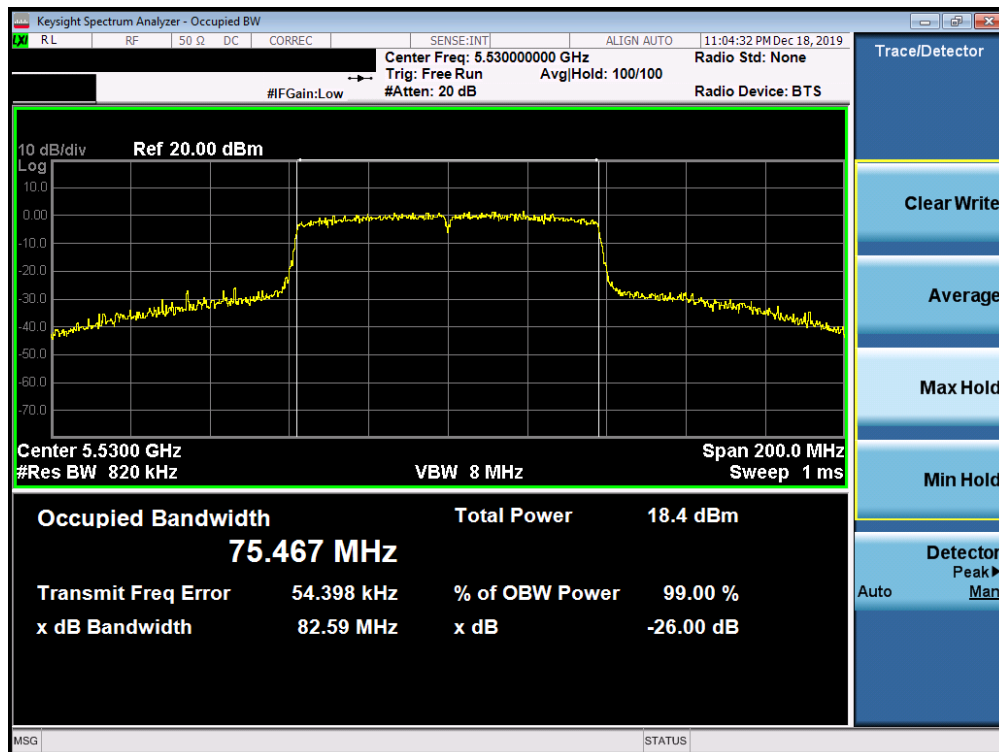
Plot 7-129. 26dB Bandwidth Plot SISO ANT2 (80MHz BW 802.11ac (UNII Band 2C) – Ch. 106)
