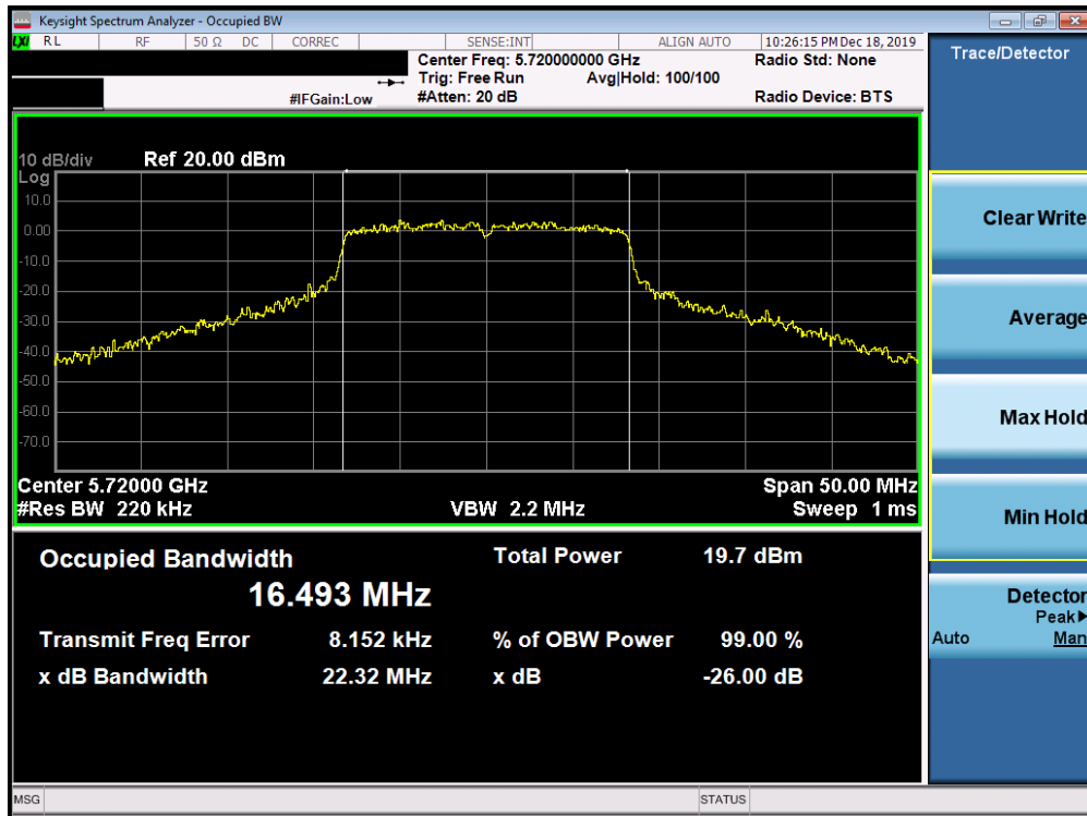
Plot 7-110. 26dB Bandwidth Plot SISO ANT2 (802.11a (UNII Band 2C) – Ch. 144)
