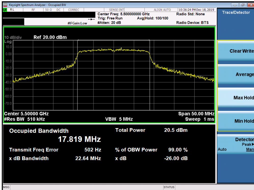
Plot 7-111. 26dB Bandwidth Plot SISO ANT2 (20MHz BW 802.11n (UNII Band 2C) – Ch. 100)
