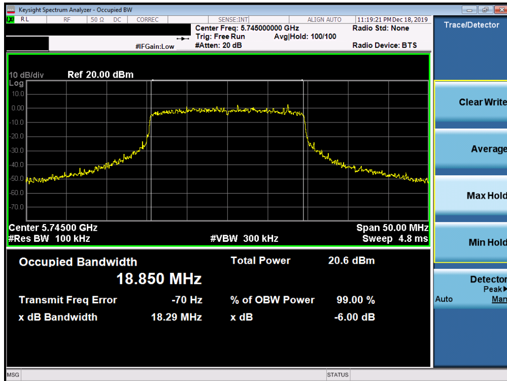
Plot 7-164. 6dB Bandwidth Plot SISO ANT2 (20MHz BW 802.11ax (UNII Band 3) – Ch. 149)
