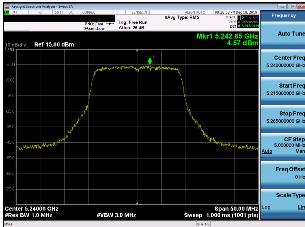
Plot 7-180. Power Spectral Density Plot SISO ANT1 (20MHz BW 802.11n (UNII Band 1) – Ch. 48)
