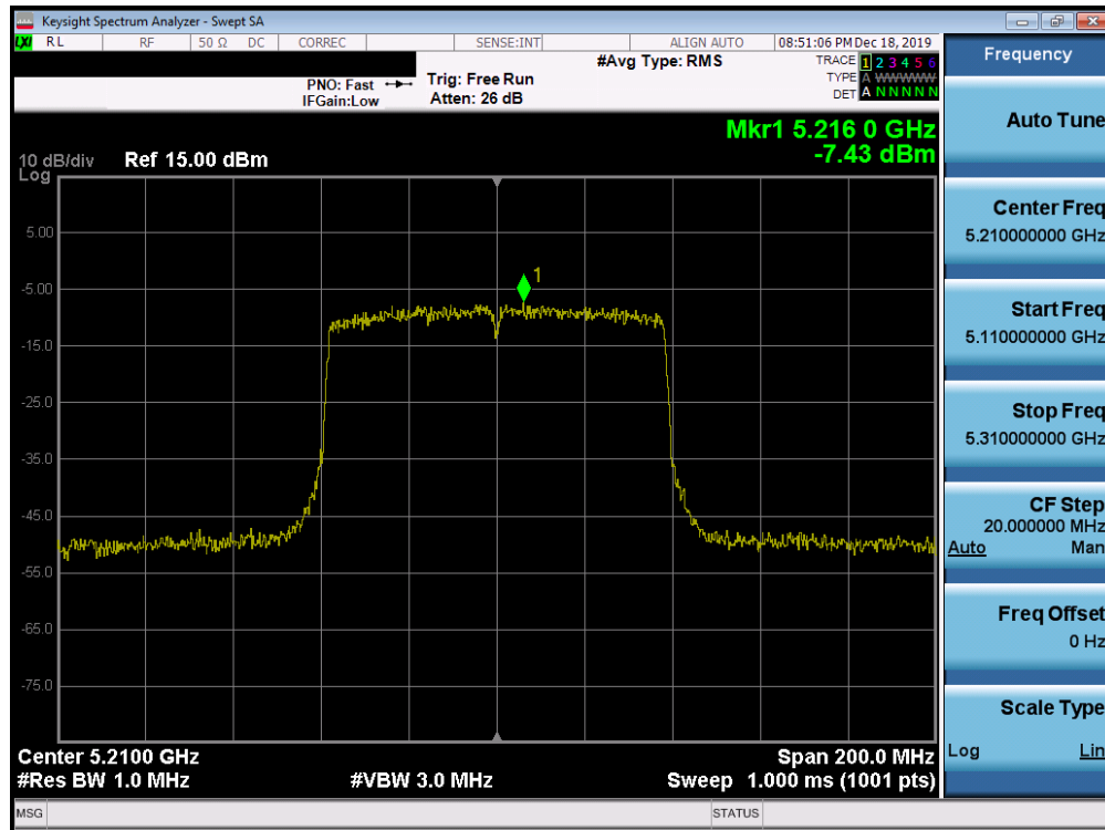
Plot 7-193. Power Spectral Density Plot SISO ANT1 (80MHz BW 802.11ac (UNII Band 1) – Ch. 42)
