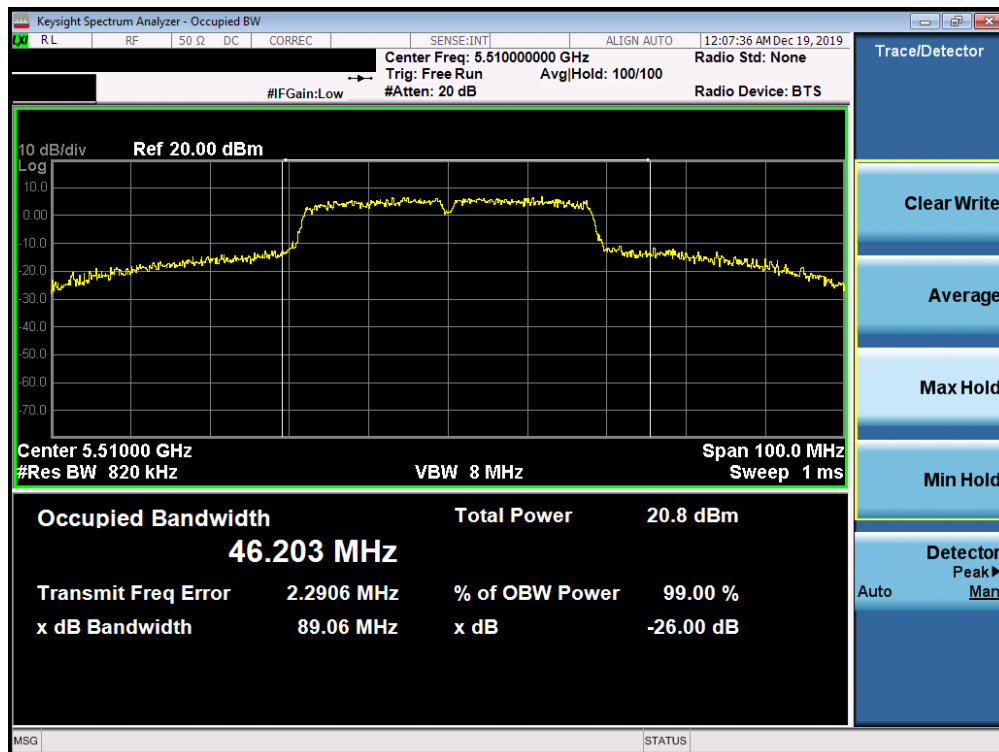
Plot 7-123. 26dB Bandwidth Plot SISO ANT2 (40MHz BW 802.11ac (UNII Band 2C) – Ch. 102)
