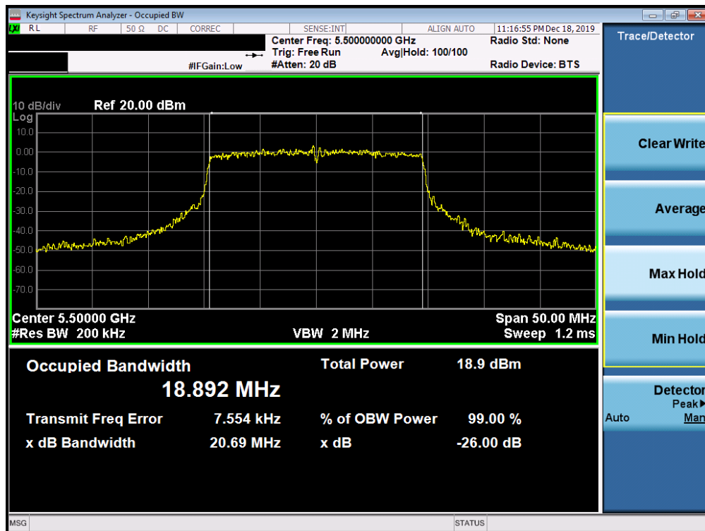
Plot 7-117. 26dB Bandwidth Plot SISO ANT2 (20MHz BW 802.11ax (UNII Band 2C) – Ch. 100)
