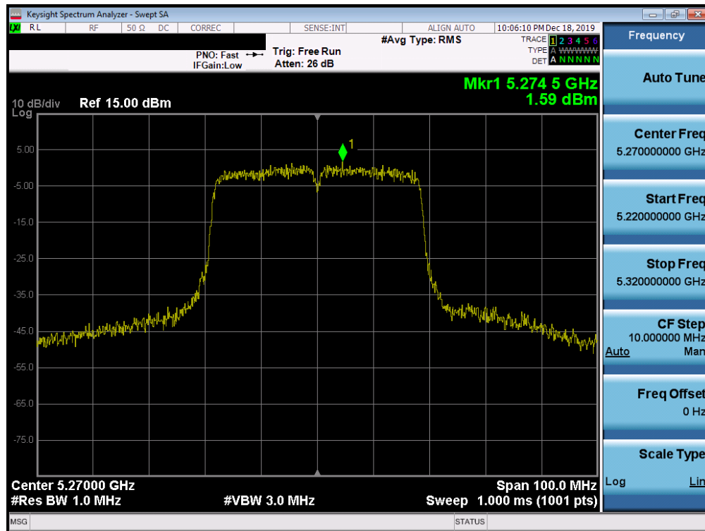
Plot 7-209. Power Spectral Density Plot SISO ANT1 (40MHz BW 802.11ac (UNII Band 2A) – Ch. 54)
