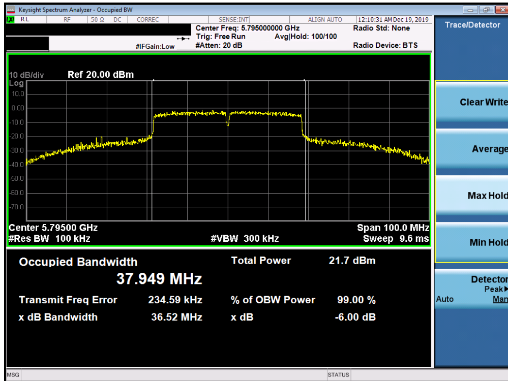
Plot 7-170. 6dB Bandwidth Plot SISO ANT2 (40MHz BW 802.11ac (UNII Band 3) – Ch. 159)
