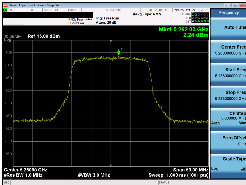
Plot 7-204. Power Spectral Density Plot SISO ANT1 (20MHz BW 802.11ax (UNII Band 2A) – Ch. 52)
