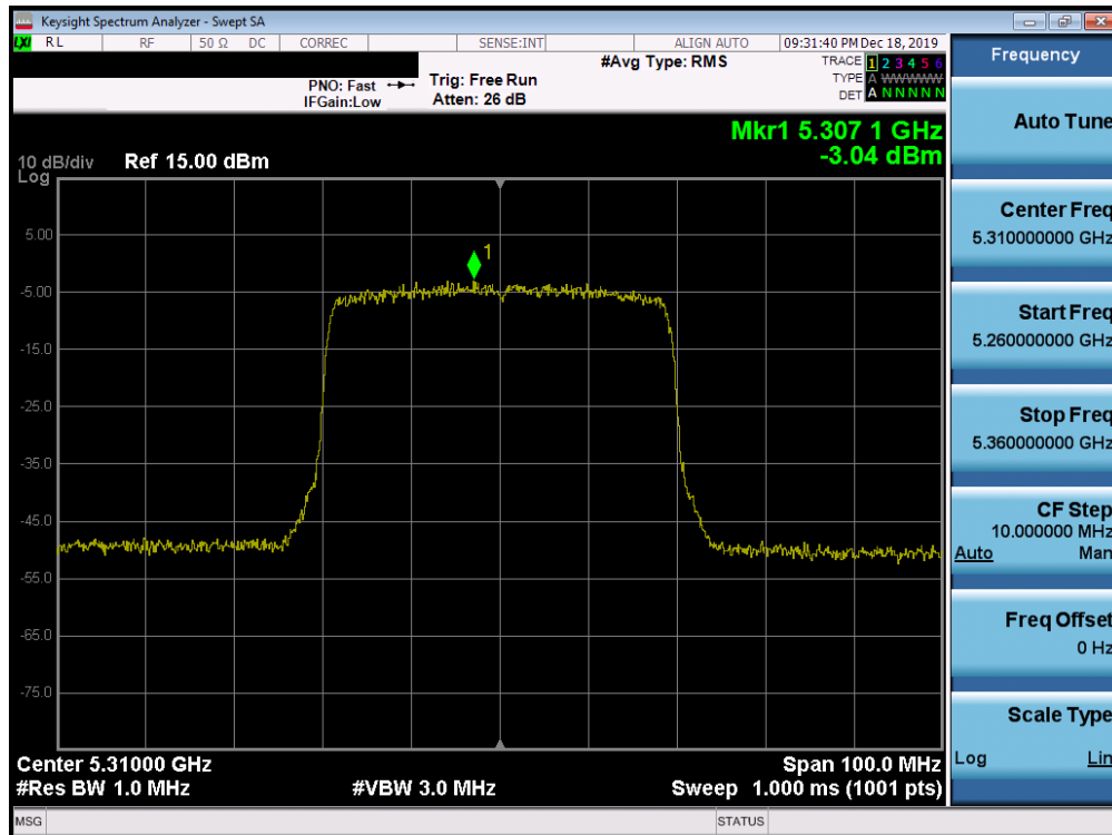
Plot 7-212. Power Spectral Density Plot SISO ANT1 (40MHz BW 802.11ax (UNII Band 2A) – Ch. 62)
