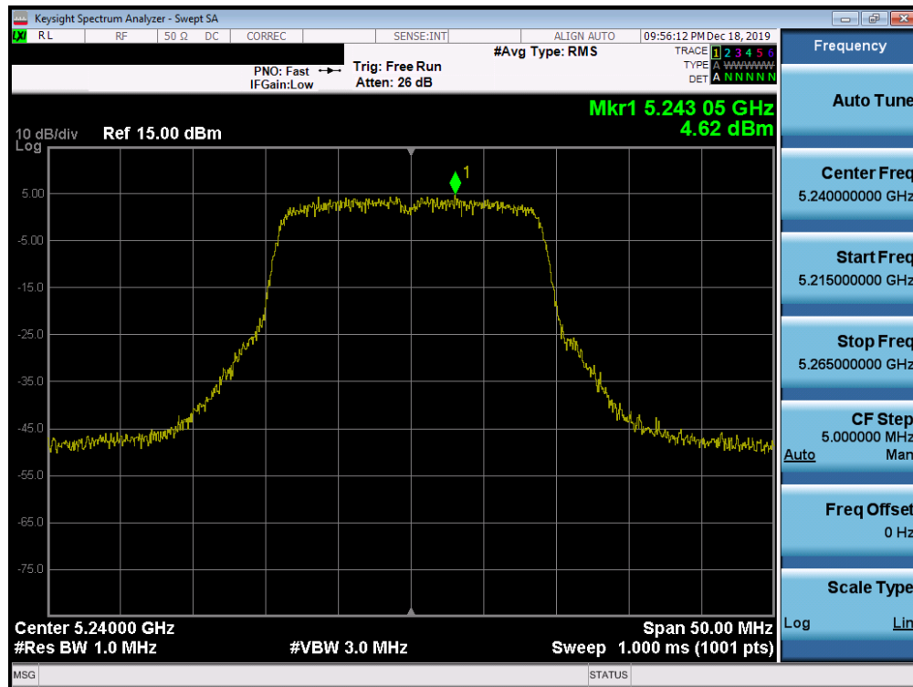
Plot 7-183. Power Spectral Density Plot SISO ANT1 (20MHz BW 802.11ac (UNII Band 1) – Ch. 48)
