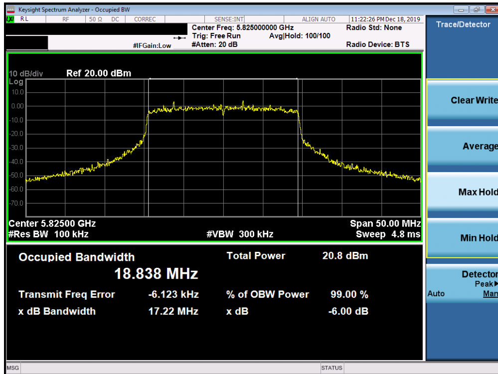
Plot 7-166. 6dB Bandwidth Plot SISO ANT2 (20MHz BW 802.11ax (UNII Band 3) – Ch. 165)
