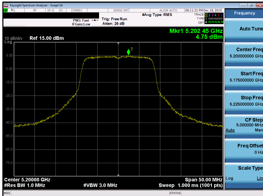
Plot 7-176. Power Spectral Density Plot SISO ANT1 (802.11a (UNII Band 1) – Ch. 40)
