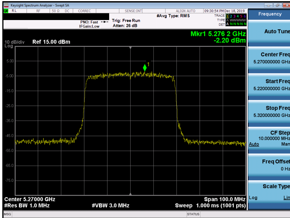
Plot 7-211. Power Spectral Density Plot SISO ANT1 (40MHz BW 802.11ax (UNII Band 2A) – Ch. 54)
