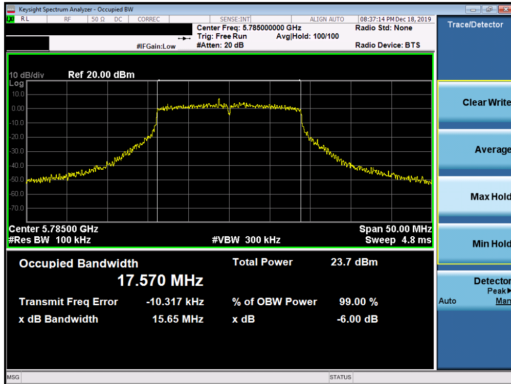
Plot 7-139. 6dB Bandwidth Plot SISO ANT1 (20MHz BW 802.11n (UNII Band 3) – Ch. 157)
