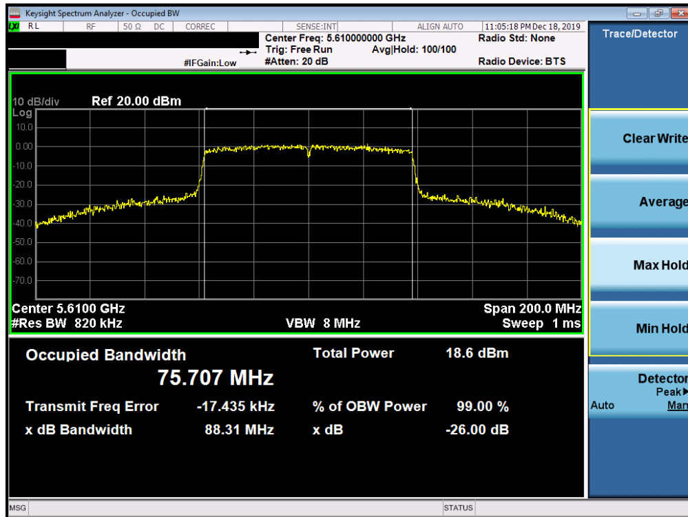
Plot 7-130. 26dB Bandwidth Plot SISO ANT2 (80MHz BW 802.11ac (UNII Band 2C) – Ch. 122)
