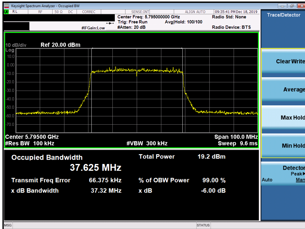
Plot 7-152. 6dB Bandwidth Plot SISO ANT1 (40MHz BW 802.11ax (UNII Band 3) – Ch. 159)
