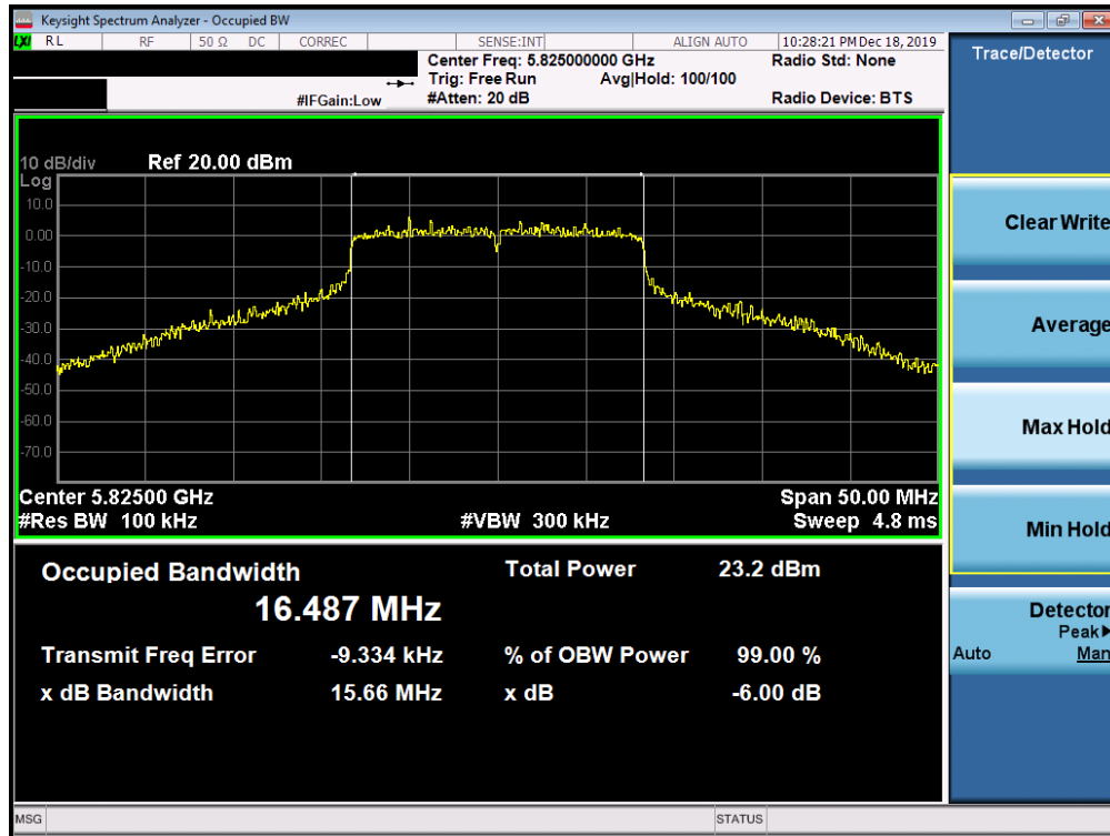
Plot 7-157. 6dB Bandwidth Plot SISO ANT2 (802.11a (UNII Band 3) – Ch. 165)
