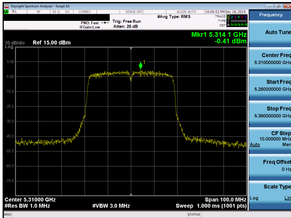
Plot 7-210. Power Spectral Density Plot SISO ANT1 (40MHz BW 802.11ac (UNII Band 2A) – Ch. 62)
