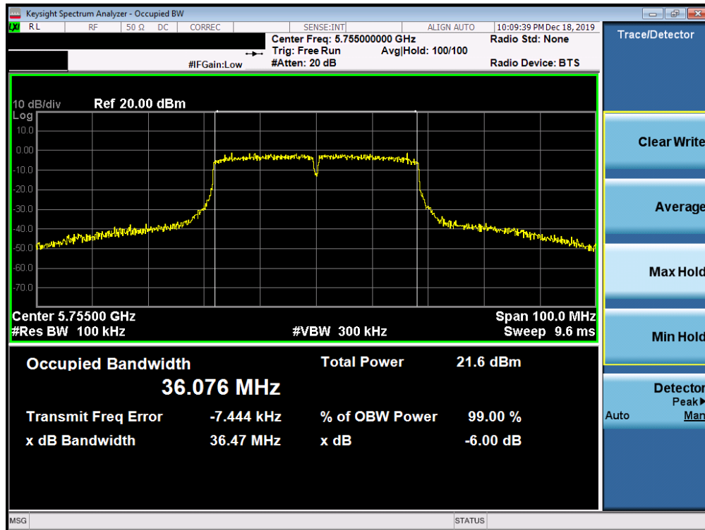
Plot 7-149. 6dB Bandwidth Plot SISO ANT1 (40MHz BW 802.11ac (UNII Band 3) – Ch. 151)
