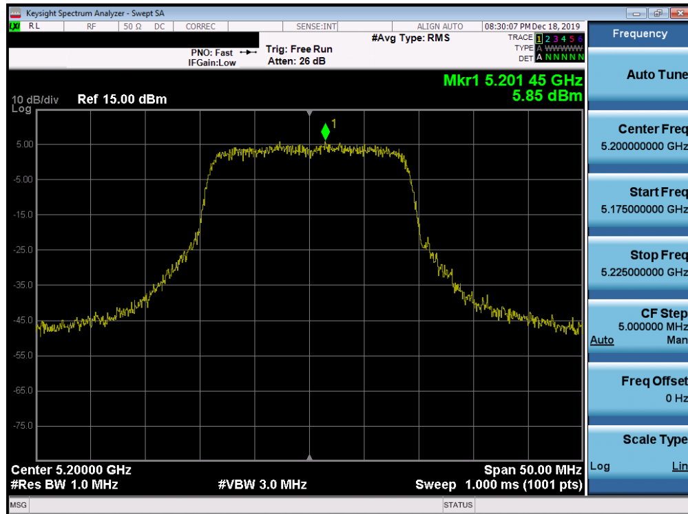
Plot 7-179. Power Spectral Density Plot SISO ANT1 (20MHz BW 802.11n (UNII Band 1) – Ch. 40)
