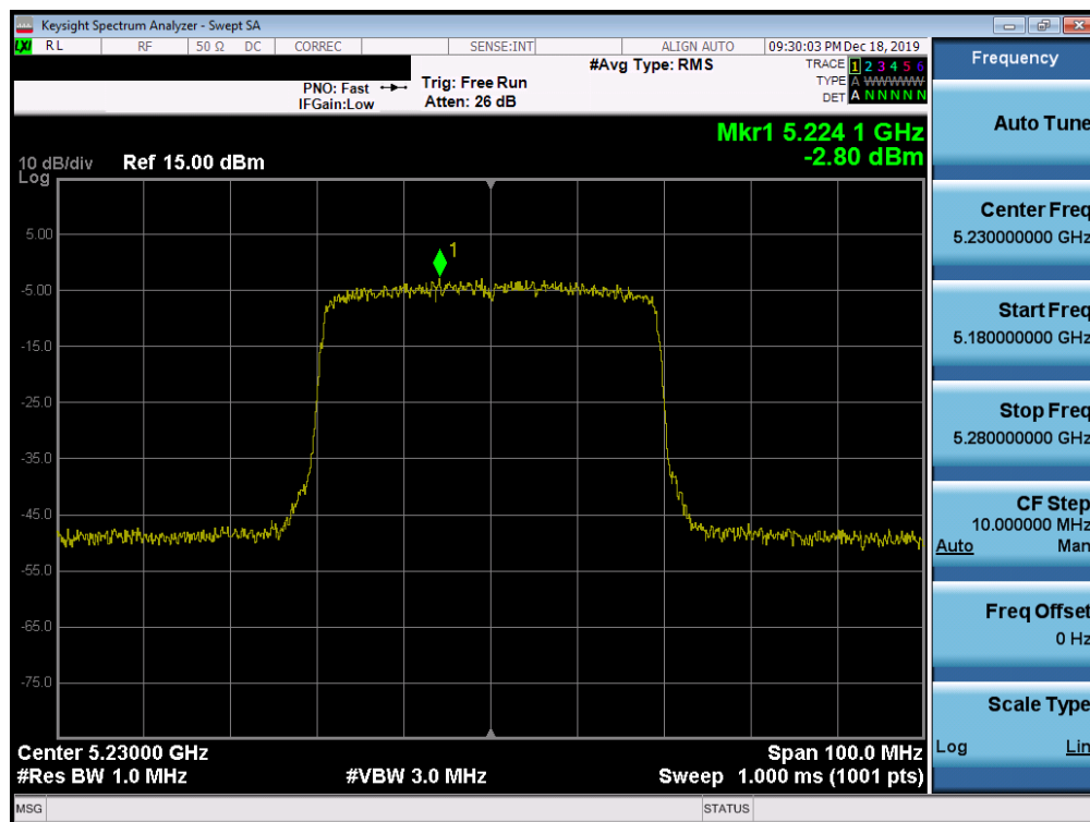
Plot 7-192. Power Spectral Density Plot SISO ANT1 (40MHz BW 802.11ax (UNII Band 1) – Ch. 46)
