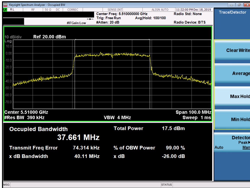
Plot 7-126. 26dB Bandwidth Plot SISO ANT2 (40MHz BW 802.11ax (UNII Band 2C) – Ch. 102)
