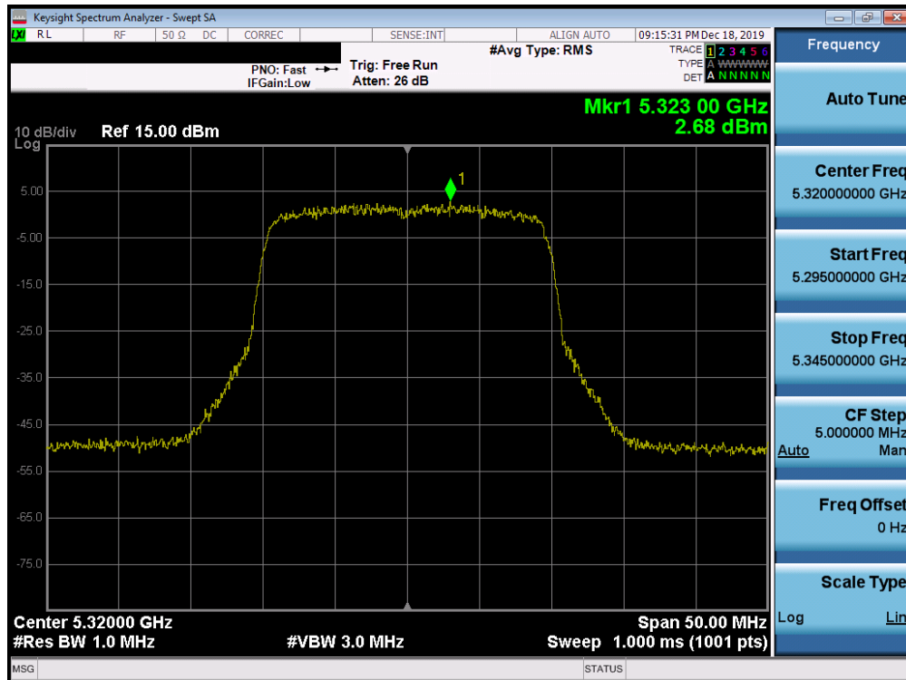
Plot 7-206. Power Spectral Density Plot SISO ANT1 (20MHz BW 802.11ax (UNII Band 2A) – Ch. 64)
