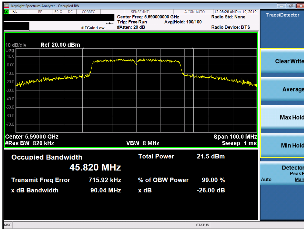
Plot 7-124. 26dB Bandwidth Plot SISO ANT2 (40MHz BW 802.11ac (UNII Band 2C) – Ch. 118)
