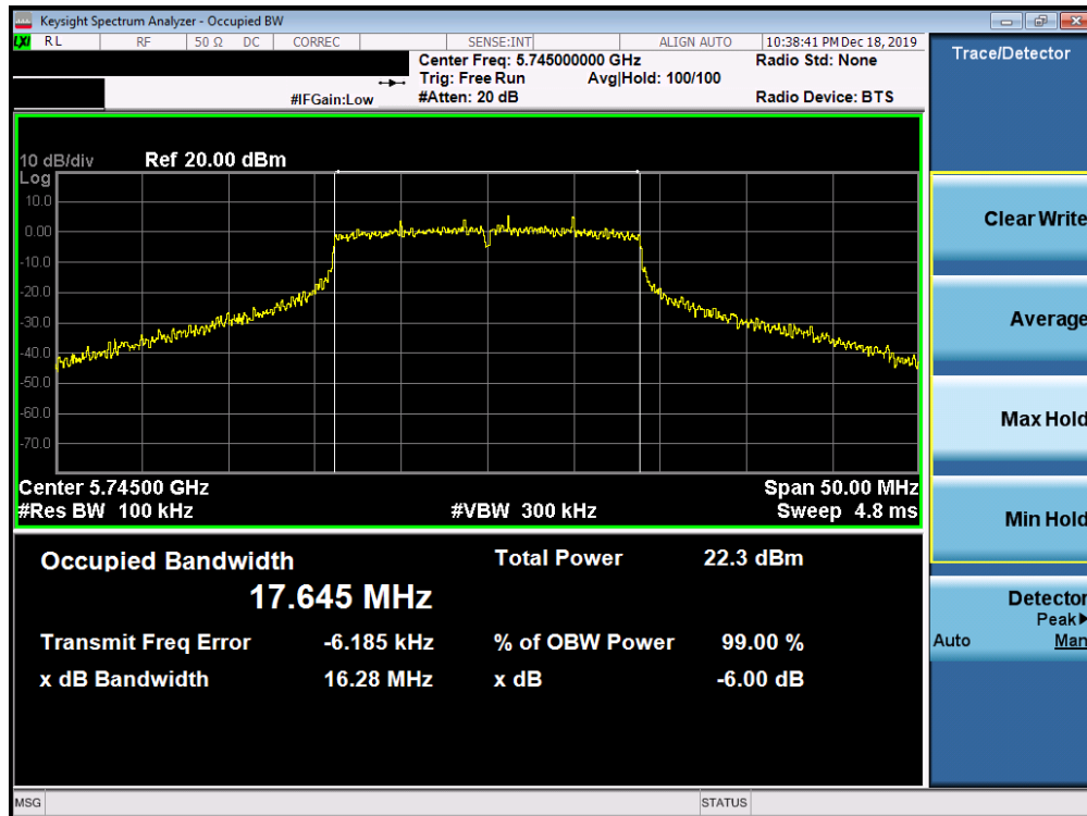
Plot 7-158. 6dB Bandwidth Plot SISO ANT2 (20MHz BW 802.11n (UNII Band 3) – Ch. 149)
