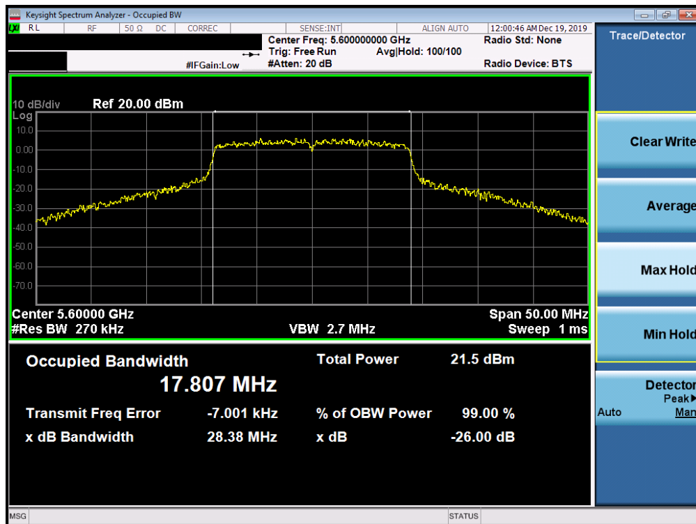
Plot 7-115. 26dB Bandwidth Plot SISO ANT2 (20MHz BW 802.11ac (UNII Band 2C) – Ch. 120)
