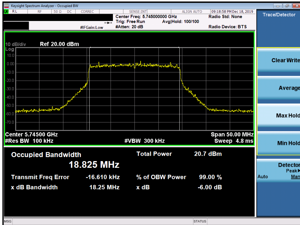
Plot 7-144. 6dB Bandwidth Plot SISO ANT1 (20MHz BW 802.11ax (UNII Band 3) – Ch. 149)
