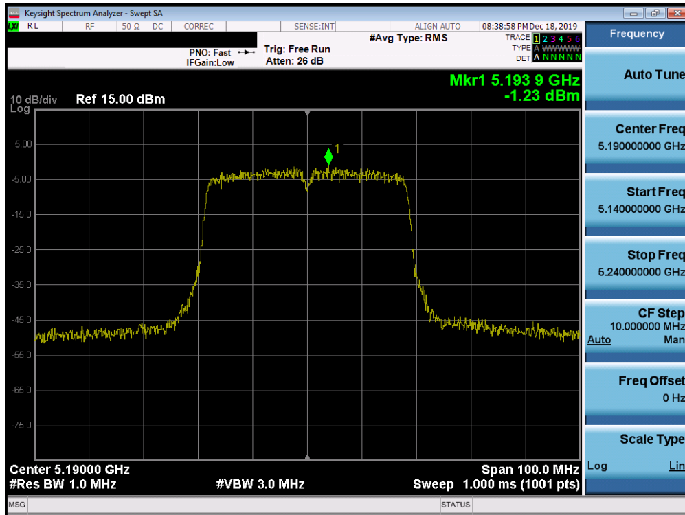
Plot 7-187. Power Spectral Density Plot SISO ANT1 (40MHz BW 802.11n (UNII Band 1) – Ch. 38)
