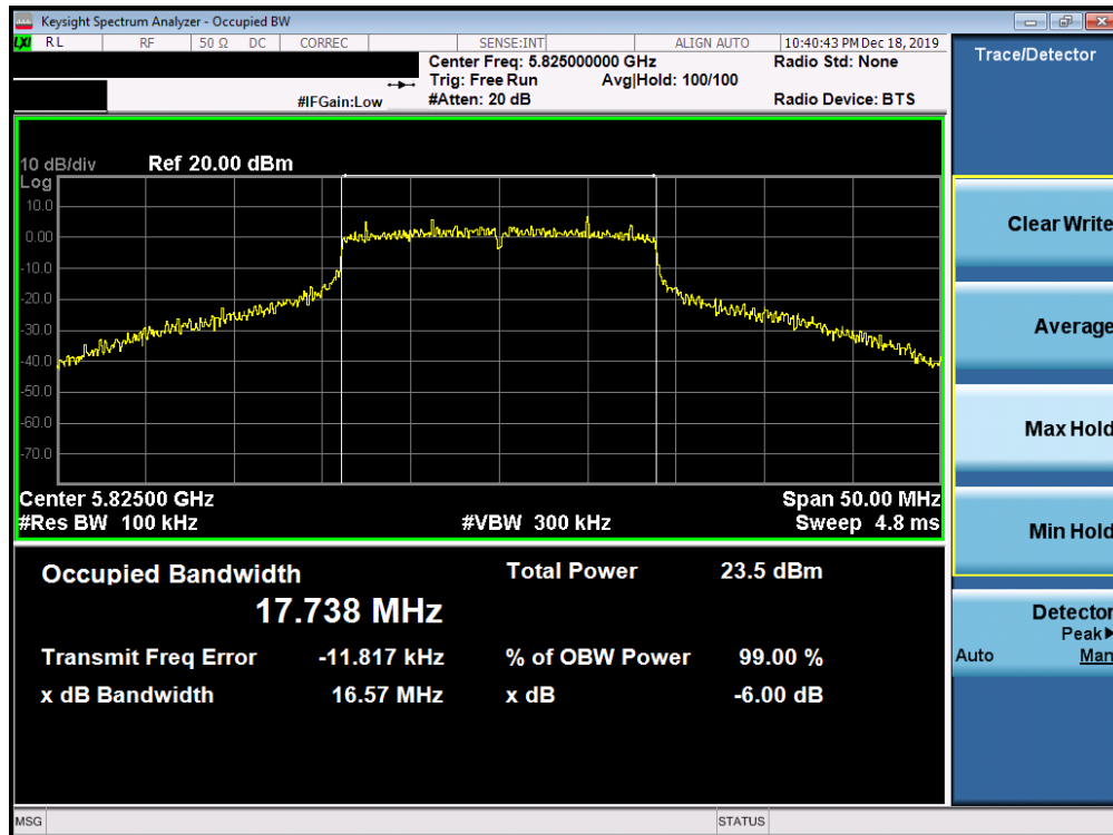
Plot 7-160. 6dB Bandwidth Plot SISO ANT2 (20MHz BW 802.11n (UNII Band 3) – Ch. 165)
