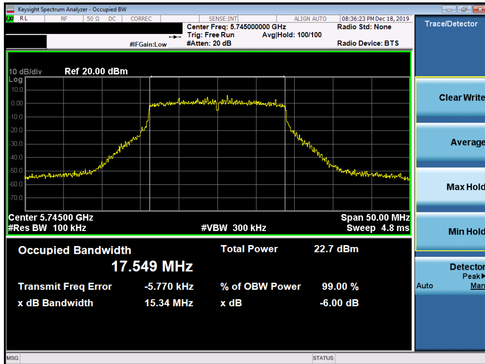
Plot 7-138. 6dB Bandwidth Plot SISO ANT1 (20MHz BW 802.11n (UNII Band 3) – Ch. 149)
