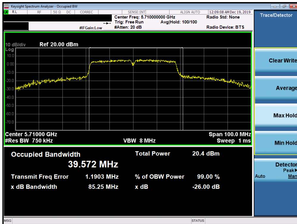
Plot 7-125. 26dB Bandwidth Plot SISO ANT2 (40MHz BW 802.11ac (UNII Band 2C) – Ch. 142)
