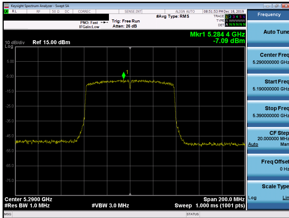
Plot 7-213. Power Spectral Density Plot SISO ANT1 (80MHz BW 802.11ac (UNII Band 2A) – Ch. 58)
