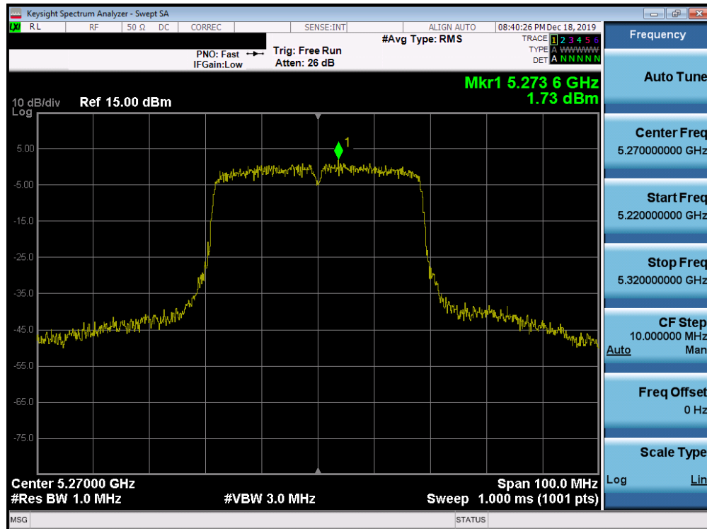
Plot 7-207. Power Spectral Density Plot SISO ANT1 (40MHz BW 802.11n (UNII Band 2A) – Ch. 54)
