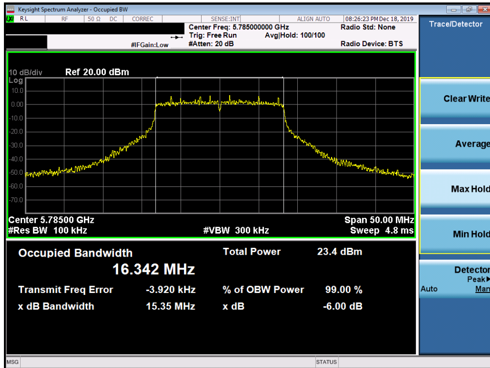
Plot 7-136. 6dB Bandwidth Plot SISO ANT1 (802.11a (UNII Band 3) – Ch. 157)
