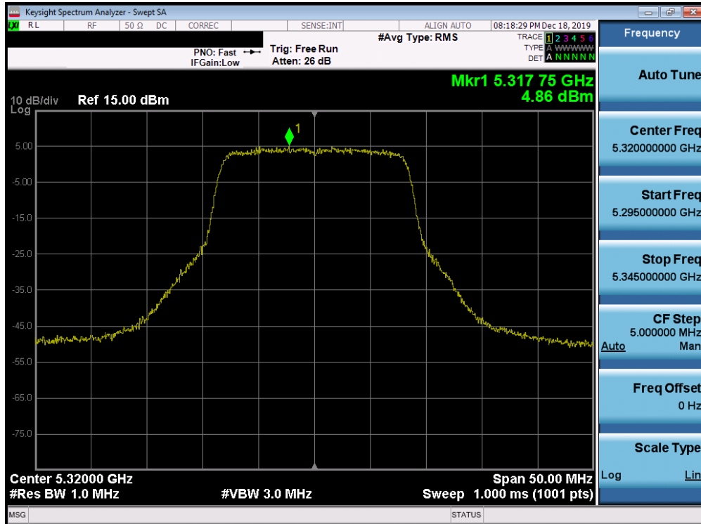
Plot 7-197. Power Spectral Density Plot SISO ANT1 (802.11a (UNII Band 2A) – Ch. 64)
