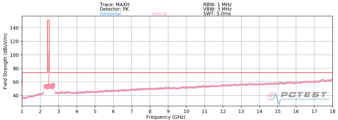
Plot 7-11. Radiated Spurious Plot above 1GHz SISO ANT2 (802.11ax OFDMA – 106 Tones – Ch. 11)
