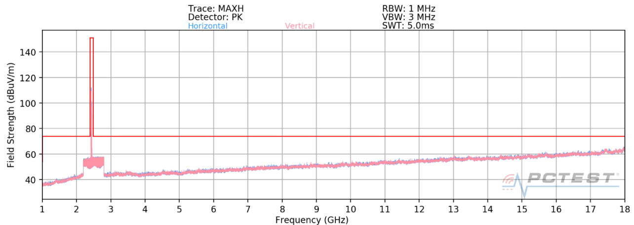
Plot 7-2. Radiated Spurious Plot above 1GHz SISO ANT1 (802.11ax OFDMA – 106 Tones – Ch. 6)
