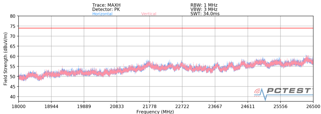
Plot 7-15. Radiated Spurious Plot above 18GHz SISO ANT2 (802.11ax OFDMA – 106 Tones)
