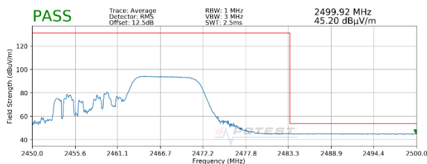
Plot 7-43. Radiated Restricted Upper Band Edge Measurement MIMO (Average – 106 Tones)
