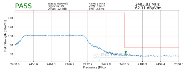
Plot 7-48. Radiated Restricted Upper Band Edge Measurement MIMO (Peak – 242 Tones)
