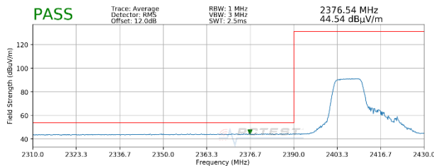
Plot 7-33. Radiated Restricted Lower Band Edge Measurement SISO ANT2 (Average – 106 Tones)
