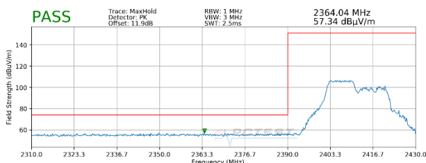
Plot 7-42. Radiated Restricted Lower Band Edge Measurement MIMO (Peak – 106 Tones)
