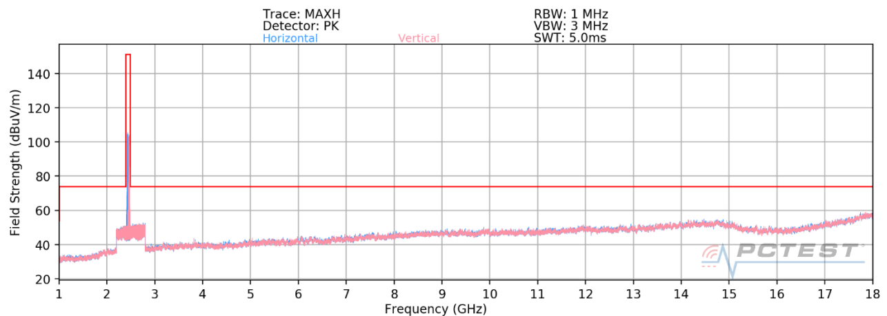
Plot 7-21. Radiated Spurious Plot above 1GHz MIMO (802.11ax OFDMA – 242 Tones – Ch. 6)
