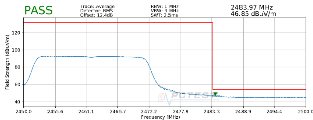
Plot 7-31. Radiated Restricted Upper Band Edge Measurement SISO ANT1 (Average – 242 Tones)
