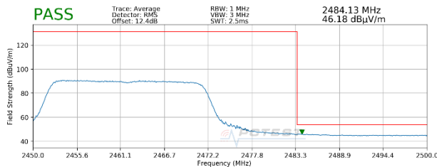
Plot 7-47. Radiated Restricted Upper Band Edge Measurement MIMO (Average – 242 Tones)
