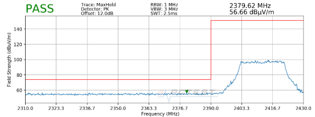
Plot 7-38. Radiated Restricted Lower Band Edge Measurement SISO ANT2 (Peak – 242 Tones)
