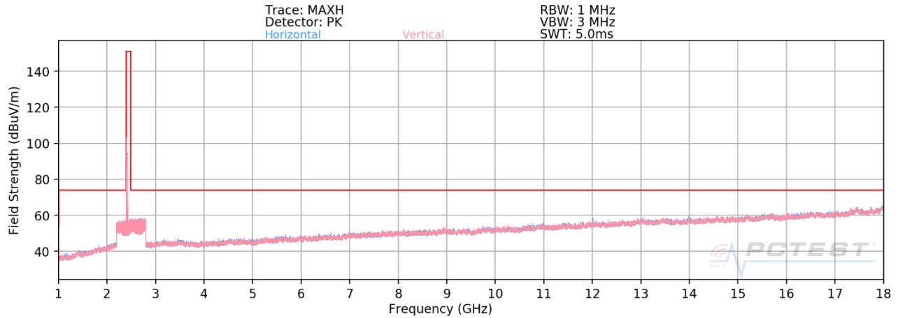
Plot 7-9. Radiated Spurious Plot above 1GHz SISO ANT2 (802.11ax OFDMA – 106 Tones – Ch. 1)
