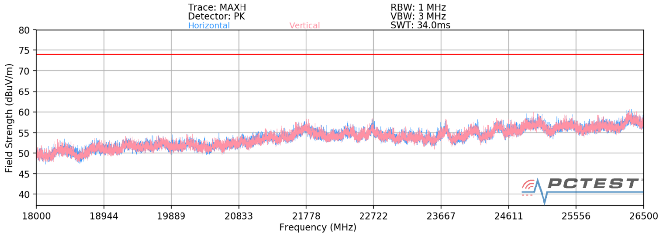
Plot 7-23. Radiated Spurious Plot above 18GHz MIMO (802.11ax OFDMA – 106 Tones)
