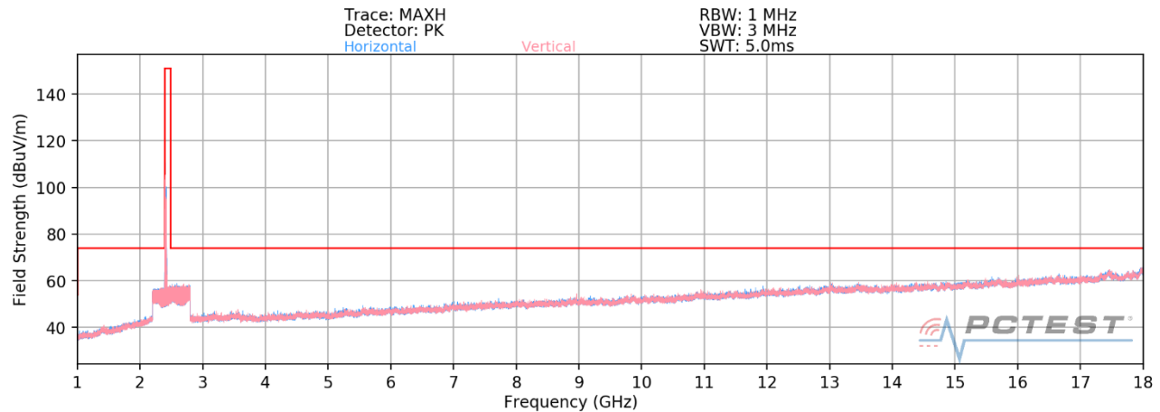
Plot 7-1. Radiated Spurious Plot above 1GHz SISO ANT1 (802.11ax OFDMA – 106 Tones – Ch. 1)
