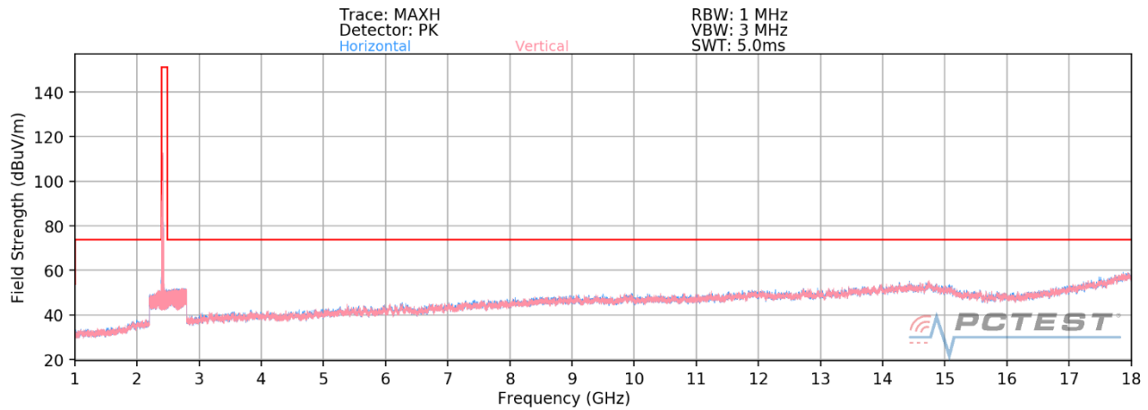
Plot 7-17. Radiated Spurious Plot above 1GHz MIMO (802.11ax OFDMA – 106 Tones – Ch. 1)
