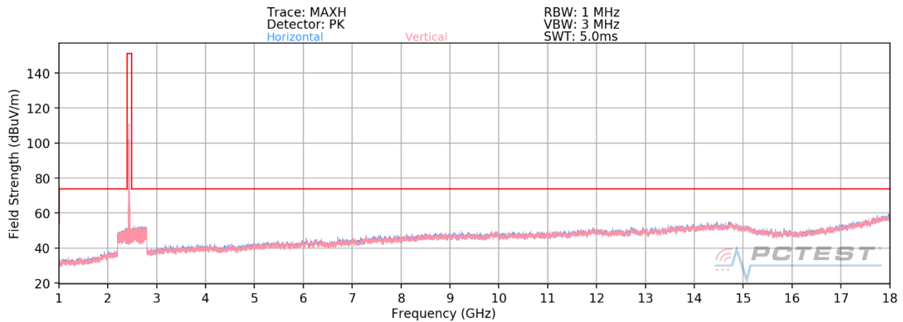
Plot 7-18. Radiated Spurious Plot above 1GHz MIMO (802.11ax OFDMA – 106 Tones – Ch. 6)
