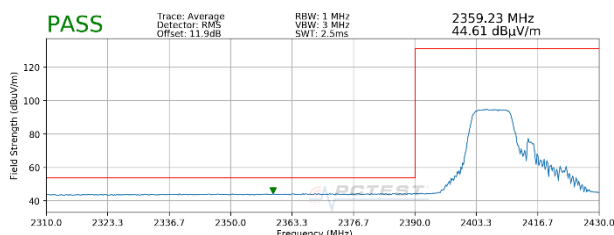
Plot 7-41. Radiated Restricted Lower Band Edge Measurement MIMO (Average – 106 Tones)
