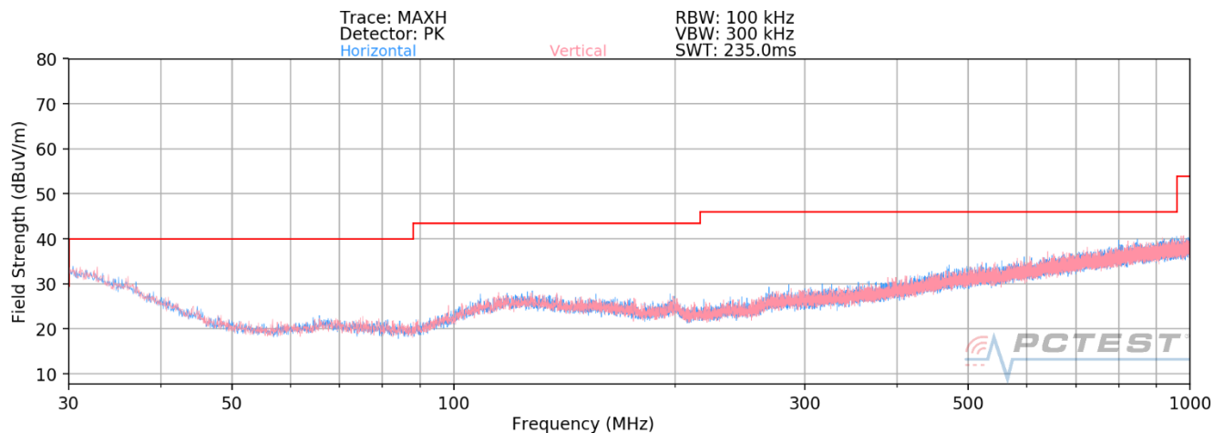
Plot 7-49. Radiated Spurious Plot below 1GHz MIMO (106 Tones)
