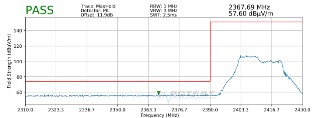
Plot 7-26. Radiated Restricted Lower Band Edge Measurement SISO ANT1 (Peak – 106 Tones)
