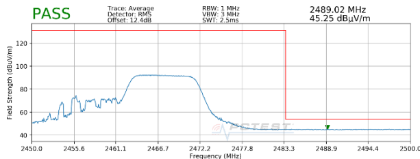
Plot 7-35. Radiated Restricted Upper Band Edge Measurement SISO ANT2 (Average – 106 Tones)
