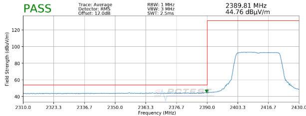
Plot 7-29. Radiated Restricted Lower Band Edge Measurement SISO ANT1 (Average – 242 Tones)
