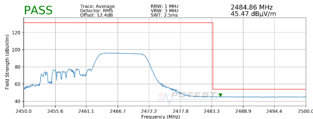
Plot 7-27. Radiated Restricted Upper Band Edge Measurement SISO ANT1 (Average – 106 Tones)
