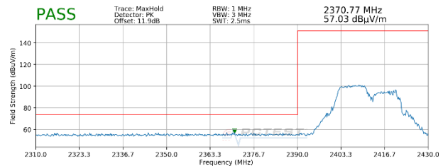
Plot 7-34. Radiated Restricted Lower Band Edge Measurement SISO ANT2 (Peak – 106 Tones)
