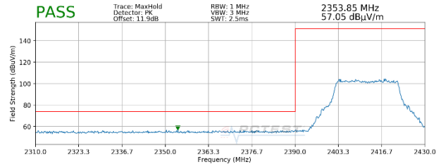
Plot 7-30. Radiated Restricted Lower Band Edge Measurement SISO ANT1 (Peak – 242 Tones)
