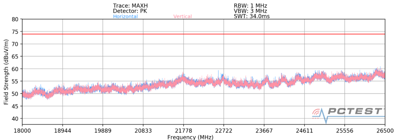
Plot 7-7. Radiated Spurious Plot above 18GHz SISO ANT1 (802.11ax OFDMA – 106 Tones)
