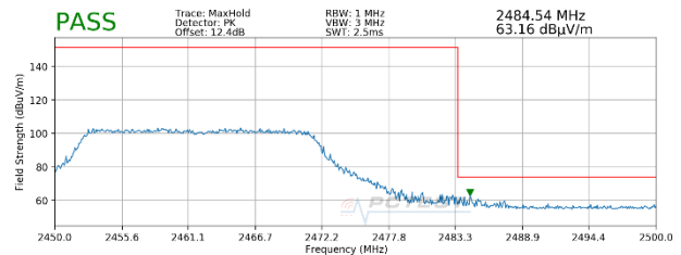
Plot 7-32. Radiated Restricted Upper Band Edge Measurement SISO ANT1 (Peak – 242 Tones)
