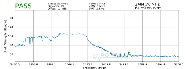
Plot 7-28. Radiated Restricted Upper Band Edge Measurement SISO ANT1 (Peak – 106 Tones)
