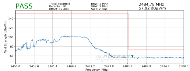
Plot 7-36. Radiated Restricted Upper Band Edge Measurement SISO ANT2 (Peak – 106 Tones)
