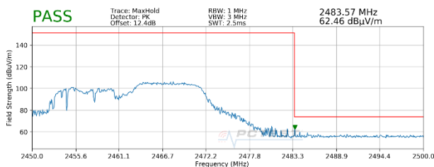
Plot 7-44. Radiated Restricted Upper Band Edge Measurement MIMO (Peak – 106 Tones)
