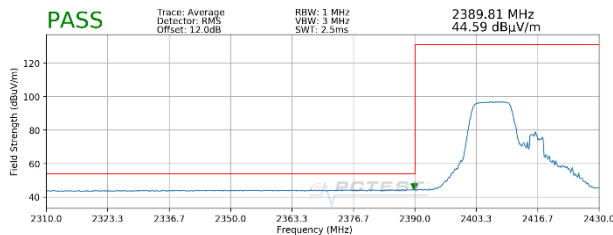
Plot 7-25. Radiated Restricted Lower Band Edge Measurement SISO ANT1 (Average – 106 Tones)
