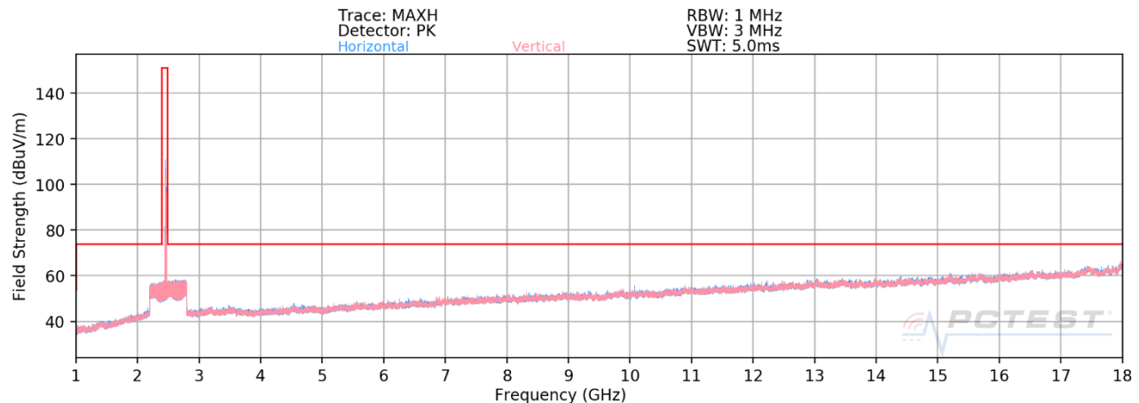
Plot 7-3. Radiated Spurious Plot above 1GHz SISO ANT1 (802.11ax OFDMA – 106 Tones – Ch. 11)
