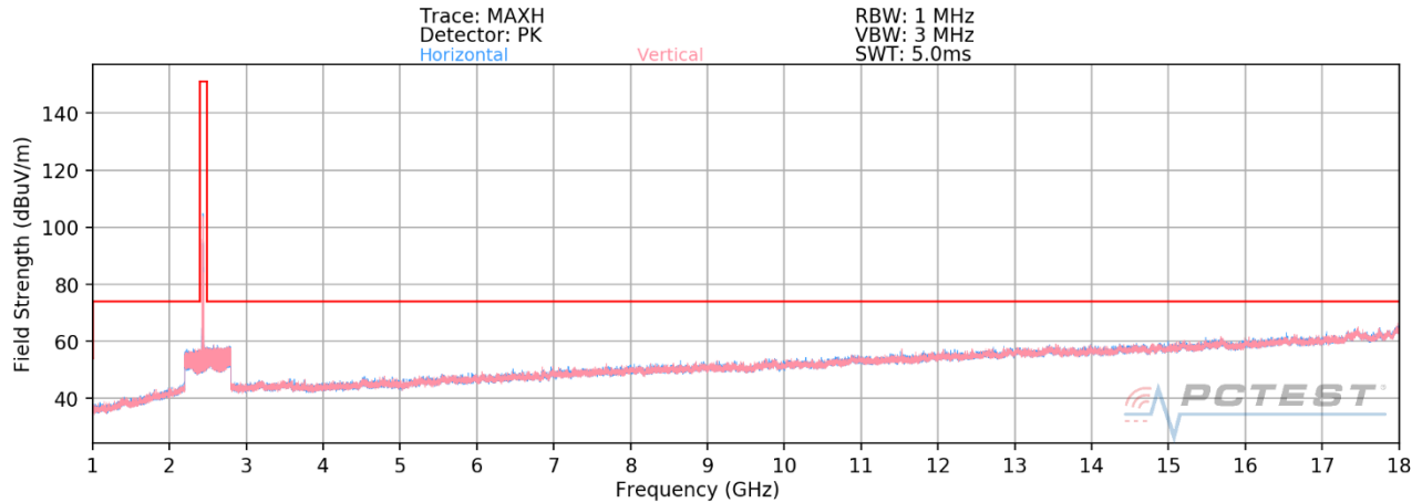
Plot 7-10. Radiated Spurious Plot above 1GHz SISO ANT2 (802.11ax OFDMA – 106 Tones – Ch. 6)
