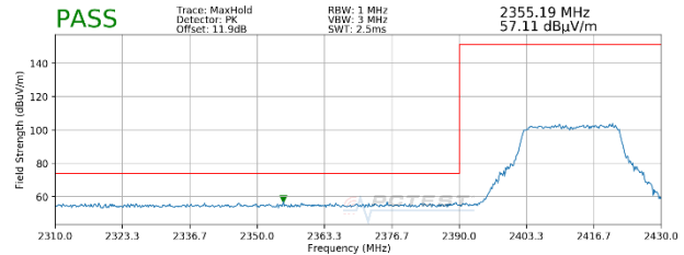
Plot 7-46. Radiated Restricted Lower Band Edge Measurement MIMO (Peak – 242 Tones)
