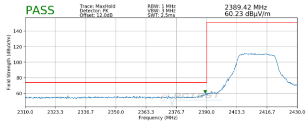
Plot 7-22. Radiated Restricted Lower Band Edge Measurement SISO ANT2 (Peak)
