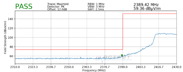
Plot 7-24. Radiated Restricted Lower Band Edge Measurement SISO ANT2 (Peak)
