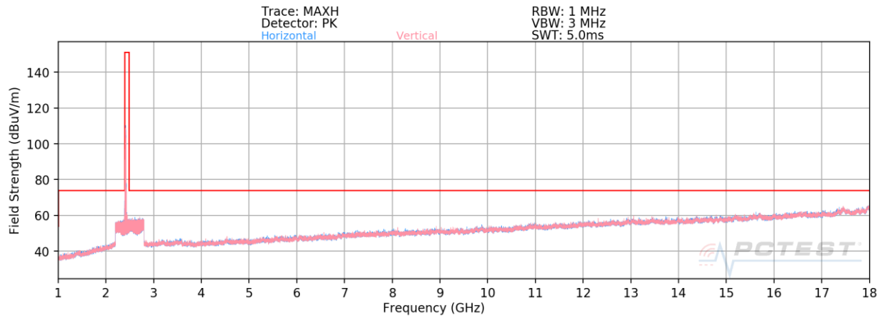
Plot 7-1. Radiated Spurious Plot above 1GHz SISO ANT1 (802.11b – Ch. 1)
