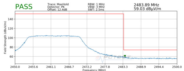
Plot 7-28. Radiated Restricted Upper Band Edge Measurement SISO ANT2 (Peak)
