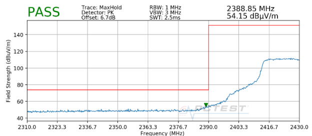
Plot 7-16. Radiated Restricted Lower Band Edge Measurement SISO ANT1 (Peak)
