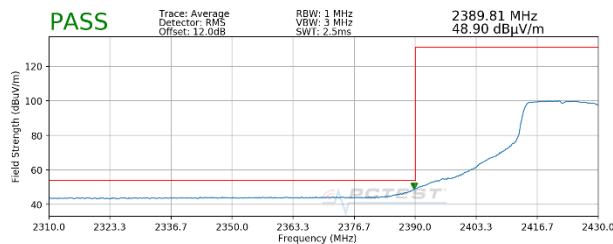
Plot 7-23. Radiated Restricted Lower Band Edge Measurement SISO ANT2 (Average)
