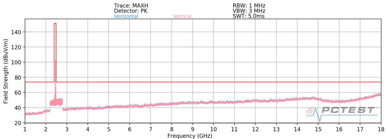
Plot 7-7. Radiated Spurious Plot above 1GHz SISO ANT2 (802.11b – Ch. 11)
