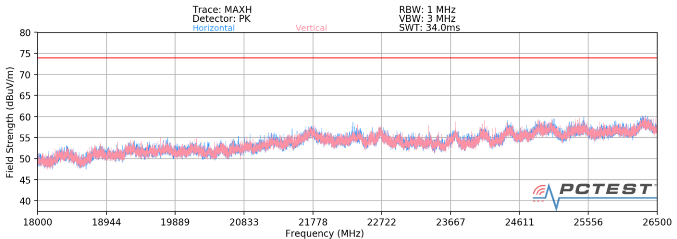
Plot 7-12. Radiated Spurious Plot above 18GHz MIMO/CDD
