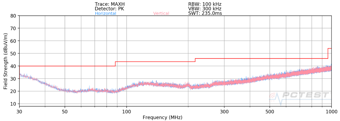
Plot 7-39. Radiated Spurious Plot below 1GHz SISO ANT1
