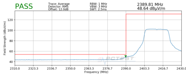
Plot 7-21. Radiated Restricted Lower Band Edge Measurement SISO ANT2 (Average)
