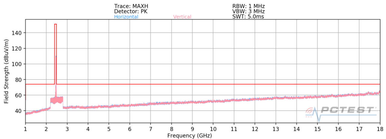
Plot 7-3. Radiated Spurious Plot above 1GHz SISO ANT1 (802.11b – Ch. 11)
