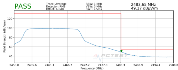
Plot 7-19. Radiated Restricted Upper Band Edge Measurement SISO ANT1 (Average)
