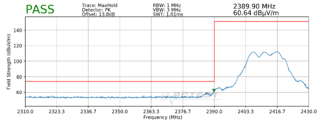
Plot 7-38. Radiated Restricted Band Edge Measurement MIMO with WCP + DD (Peak)
