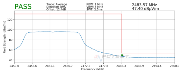
Plot 7-27. Radiated Restricted Upper Band Edge Measurement SISO ANT2 (Average)
