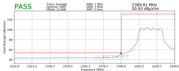
Plot 7-29. Radiated Restricted Lower Band Edge Measurement MIMO (Average)
