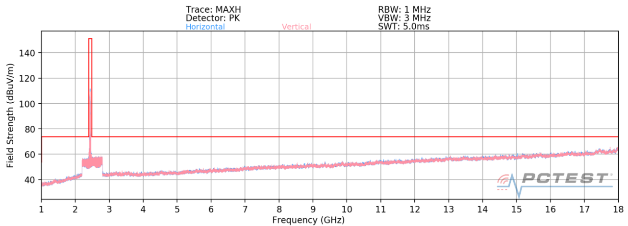
Plot 7-2. Radiated Spurious Plot above 1GHz SISO ANT1 (802.11b – Ch. 6)
