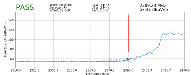
Plot 7-32. Radiated Restricted Lower Band Edge Measurement MIMO (Peak)
