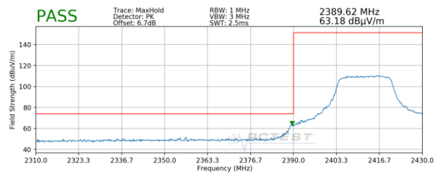
Plot 7-14. Radiated Restricted Lower Band Edge Measurement SISO ANT1 (Peak)
