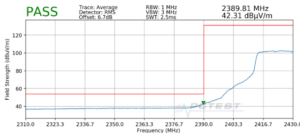
Plot 7-15. Radiated Restricted Lower Band Edge Measurement SISO ANT1 (Average)
