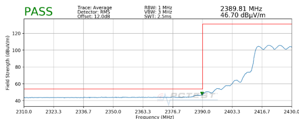
Plot 7-31. Radiated Restricted Lower Band Edge Measurement MIMO (Average)
