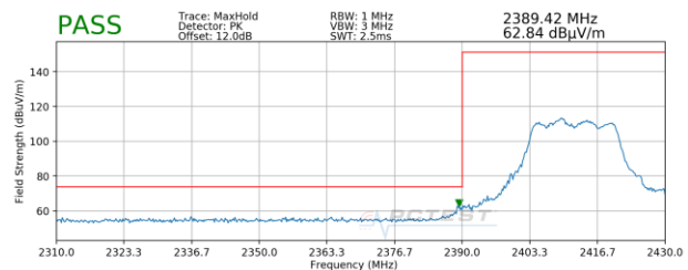
Plot 7-30. Radiated Restricted Lower Band Edge Measurement MIMO (Peak)
