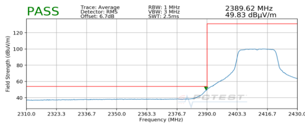
Plot 7-13. Radiated Restricted Lower Band Edge Measurement SISO ANT1 (Average)
