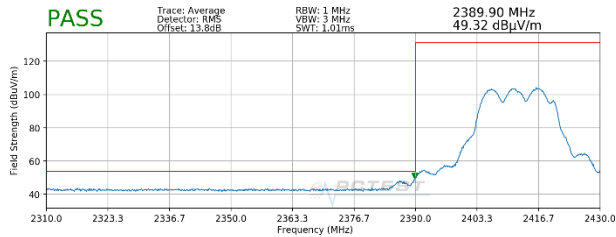
Plot 7-37. Radiated Restricted Band Edge Measurement MIMO with WCP + DD (Average)
