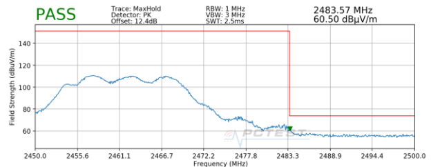
Plot 7-36. Radiated Restricted Upper Band Edge Measurement MIMO (Peak)
