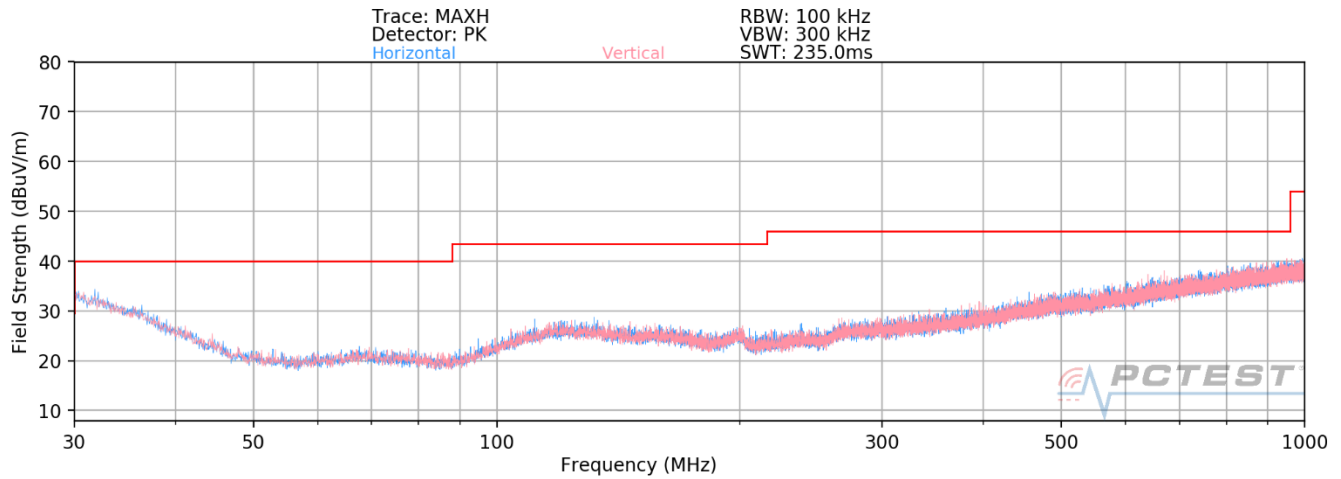
Plot 7-40. Radiated Spurious Plot below 1GHz SISO ANT2
