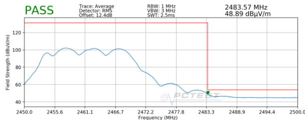
Plot 7-35. Radiated Restricted Upper Band Edge Measurement MIMO (Average)
