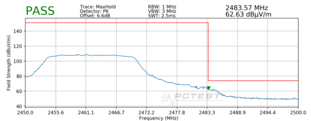
Plot 7-20. Radiated Restricted Upper Band Edge Measurement SISO ANT1 (Peak)
