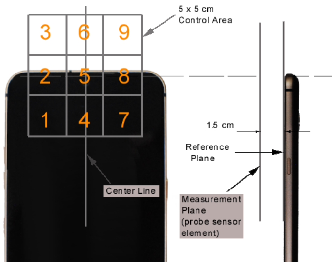
Figure 18-7 5x5 Scan grid above WD (Acoustic Scan Area Pictured)
