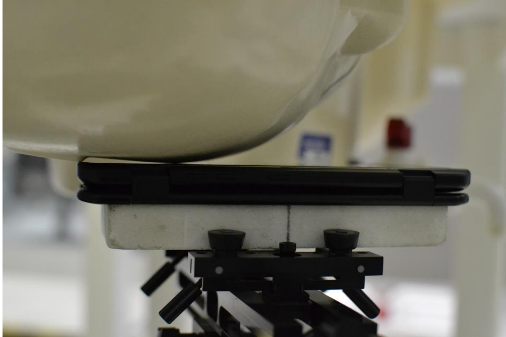
SAR Test Setup Photo 3 – Right Cheek with Dual Display Cover Position 3
