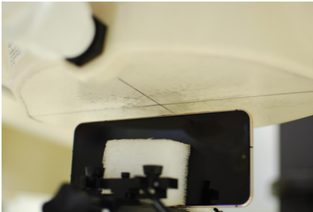
SAR Test Setup Photo 26 – Left Edge at 10 mm
