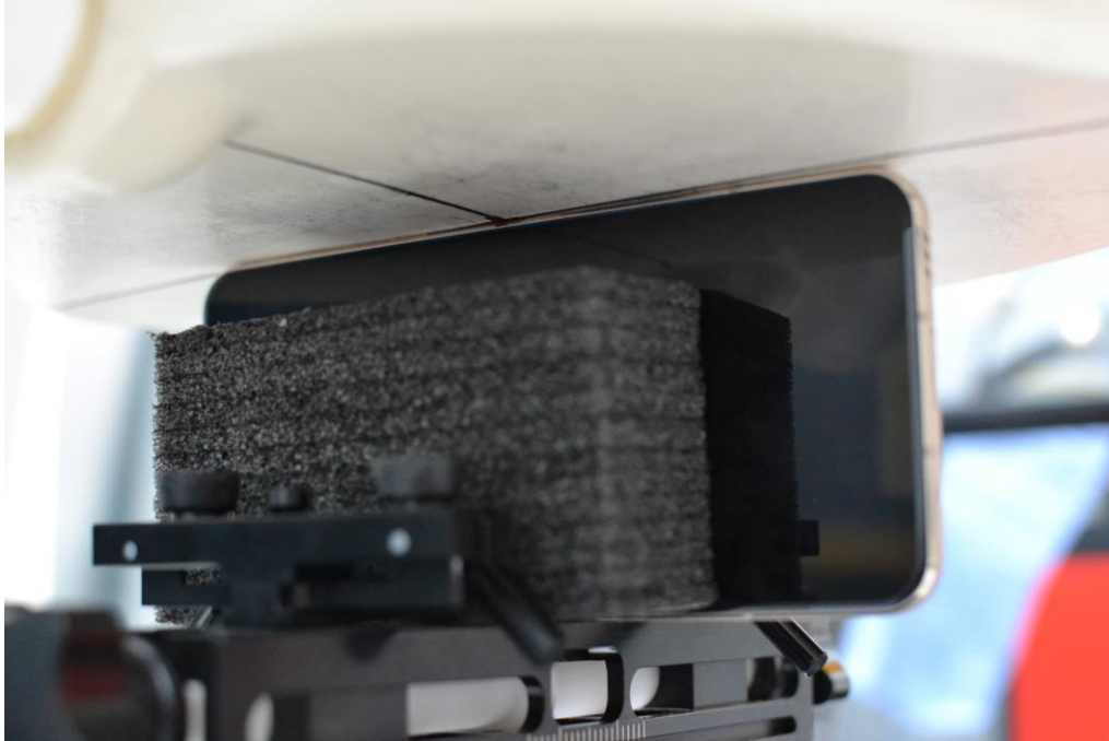
SAR Test Setup Photo 25 – Right Edge at 0 mm
