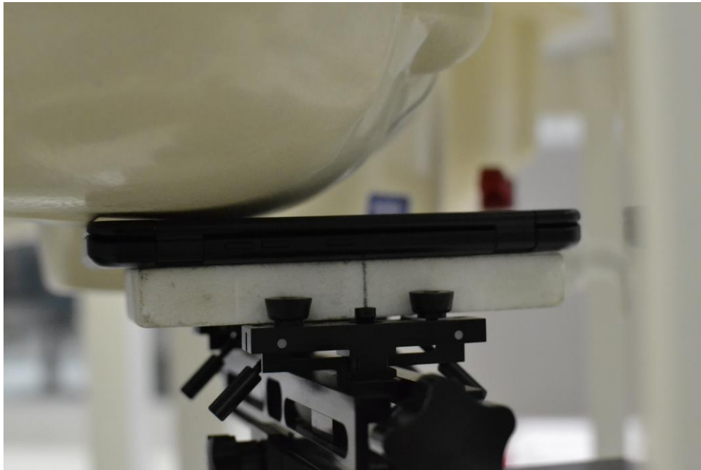
SAR Test Setup Photo 2 – Right Cheek with Dual Display Cover Position 1
