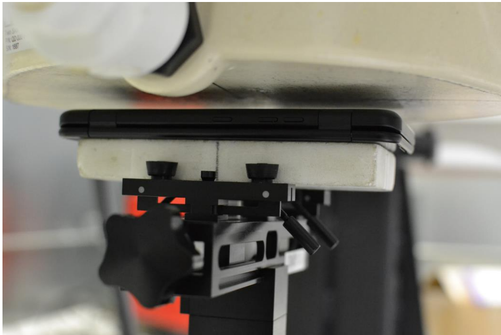
SAR Test Setup Photo 8 – Back Side at 10 mm with Dual Display Cover Position 1
