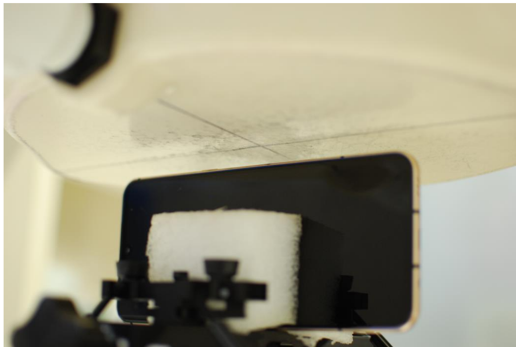
SAR Test Setup Photo 24 – Right Edge at 10 mm
