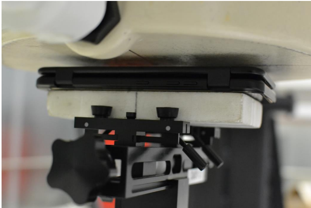
SAR Test Setup Photo 10 – Back Side at 10 mm with Dual Display Cover Position 3
