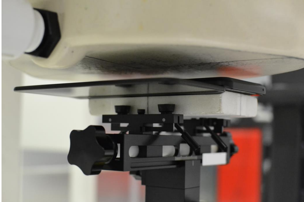
SAR Test Setup Photo 9 – Back Side at 10 mm with Dual Display Cover Position 2
