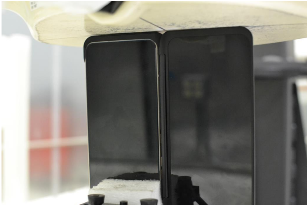
SAR Test Setup Photo 22 – Bottom Edge at 0 mm with Dual Display Cover Position 2
