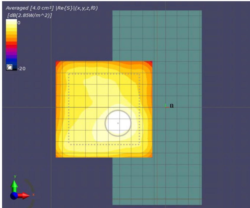
Figure 8-2: 4cm2-averaged power density distribution measured at input.power.limit of -0.03 dBm on the back surface for n261 beam 39
