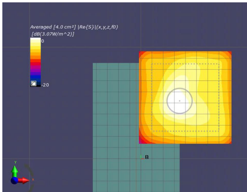
Figure 8-3: 4cm2-averaged power density distribution measured at input.power.limit of 1.92 dBm on the back surface for n260 beam 28
