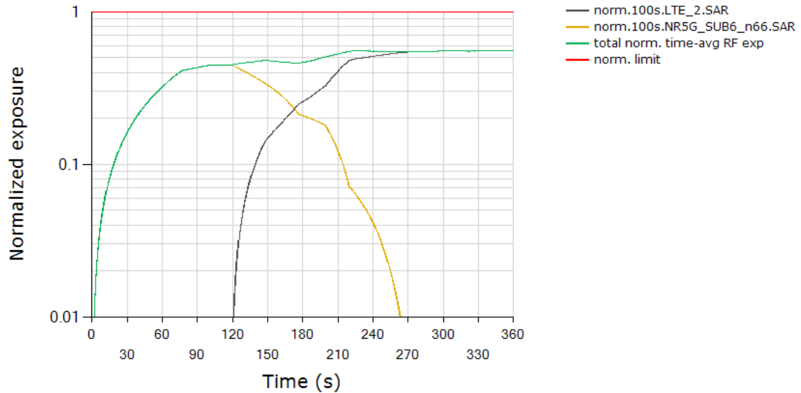
Total Normalized Time-averaged RF Exposure Tech: LTE, Band 2 / Tech: NR5G SUB6, Band n66
