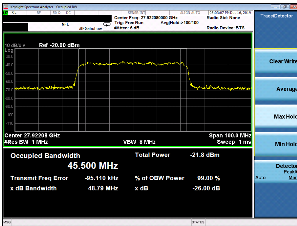
Plot 7-15. Ant2 Occupied Bandwidth Plot (50MHz-1CC – 64QAM – Mid Channel)
