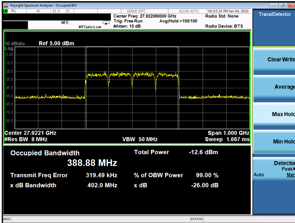
Plot 7-24. Ant2 Occupied Bandwidth Plot (100MHz-4CC – 64QAM – Mid Channel)
