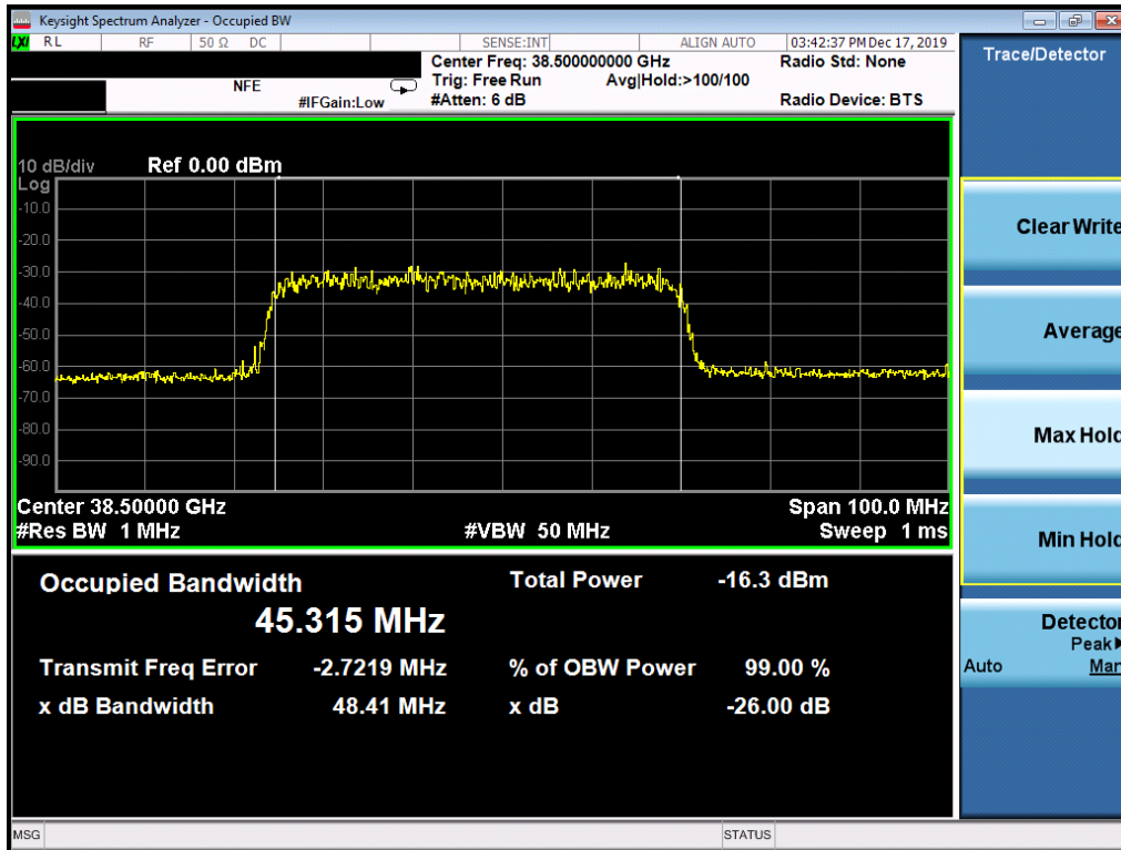
Plot 7-50. Ant2 Occupied Bandwidth Plot (50MHz-1CC – 16QAM – Mid Channel)
