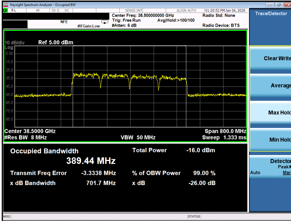
Plot 7-70. Ant3 Occupied Bandwidth Plot (100MHz-4CC – QPSK – Mid Channel)
