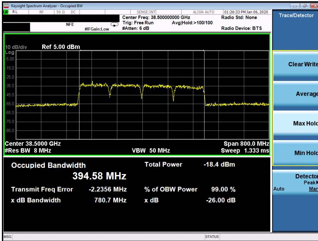
Plot 7-72. Ant3 Occupied Bandwidth Plot (100MHz-4CC – 64QAM – Mid Channel)
