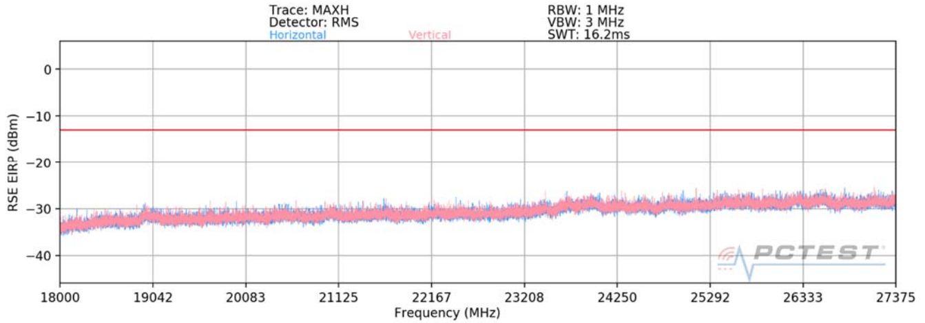
Plot 7-82. Ant2-n261 Radiated Spurious Plot (1CC QPSK Mid Channel V Beam)
