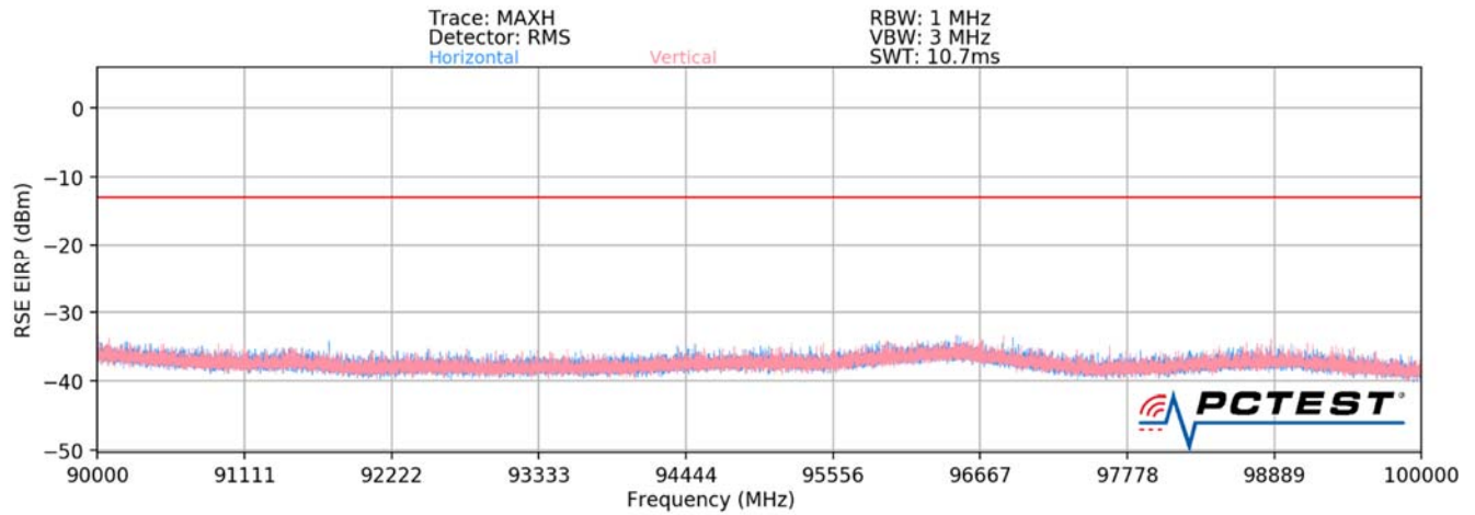
Plot 7-79. Ant1-n261 Radiated Spurious Plot (1CC QPSK Mid Channel V Beam)
