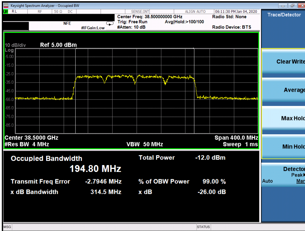
Plot 7-42. Ant1 Occupied Bandwidth Plot (50MHz-4CC – 64QAM – Mid Channel)
