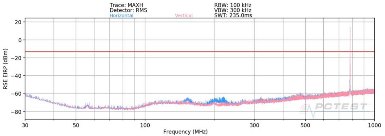
Plot 7-73. Ant1-n261 Radiated Spurious Plot (1CC QPSK Mid Channel V Beam)
