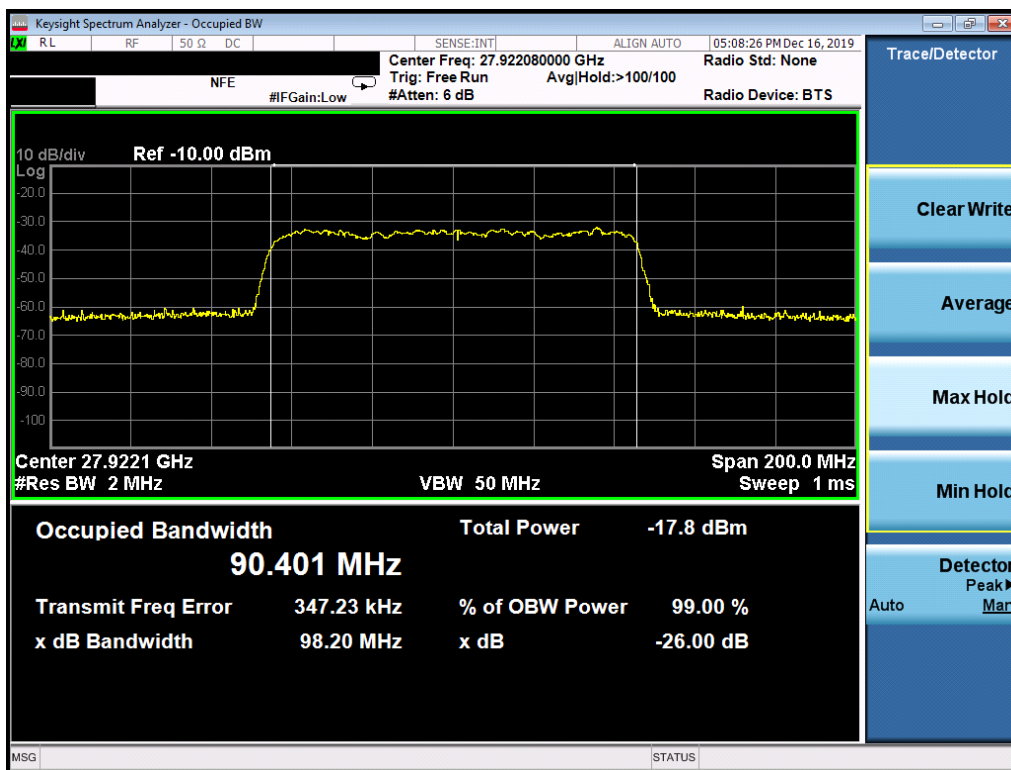
Plot 7-19. Ant2 Occupied Bandwidth Plot (100MHz-1CC – QPSK – Mid Channel)
