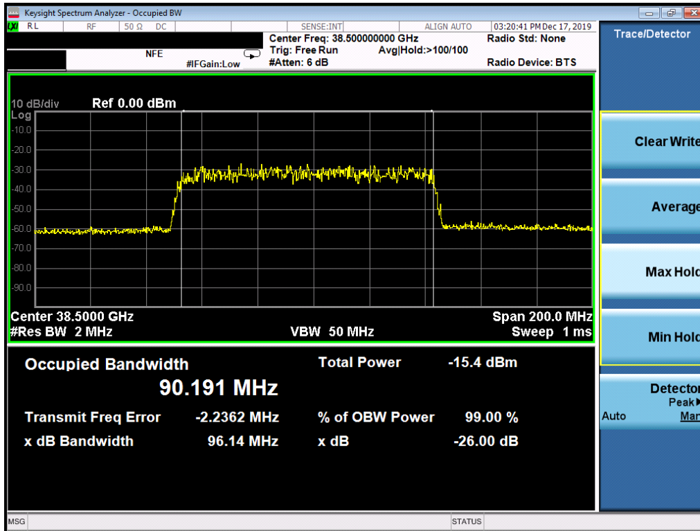
Plot 7-44. Ant1 Occupied Bandwidth Plot (100MHz-1CC – 16QAM – Mid Channel)
