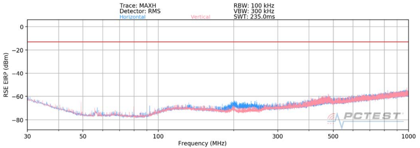
Plot 7-80. Ant2-n261 Radiated Spurious Plot (1CC QPSK Mid Channel V Beam)
