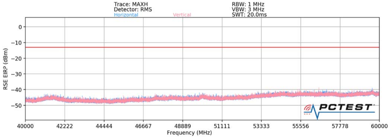
Plot 7-84. Ant2-n261 Radiated Spurious Plot (1CC QPSK Mid Channel V Beam)
