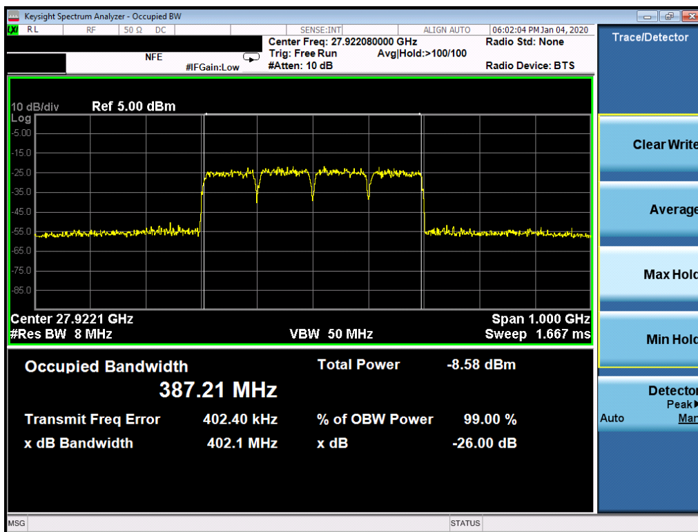
Plot 7-23. Ant2 Occupied Bandwidth Plot (100MHz-4CC – 16QAM – Mid Channel)
