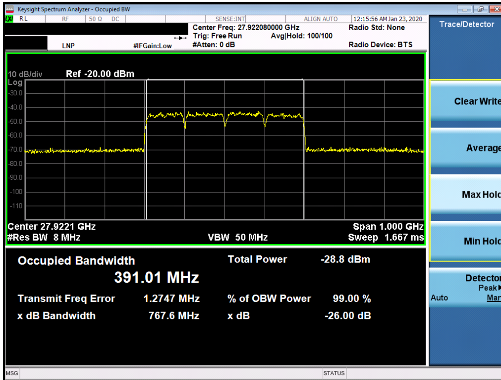
Plot 7-12. Ant1 Occupied Bandwidth Plot (100MHz-4CC – 64QAM – Mid Channel)
