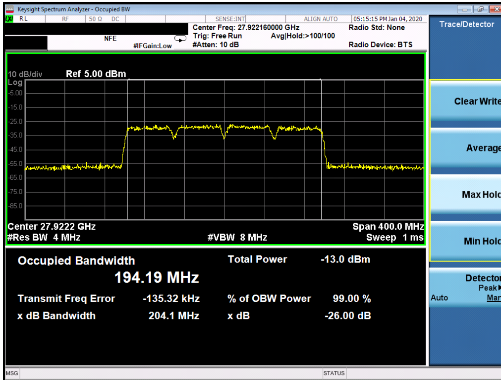
Plot 7-4. Ant1 Occupied Bandwidth Plot (50MHz-4CC – QPSK – Mid Channel)
