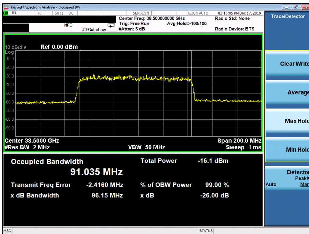
Plot 7-57. Ant2 Occupied Bandwidth Plot (100MHz-1CC – 64QAM – Mid Channel)
