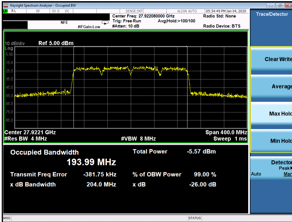
Plot 7-16. Ant2 Occupied Bandwidth Plot (50MHz-4CC – QPSK – Mid Channel)
