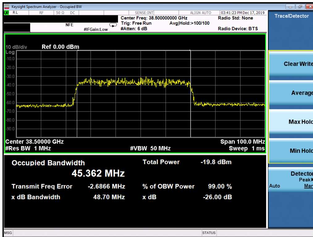
Plot 7-49. Ant2 Occupied Bandwidth Plot (50MHz-1CC – QPSK – Mid Channel)
