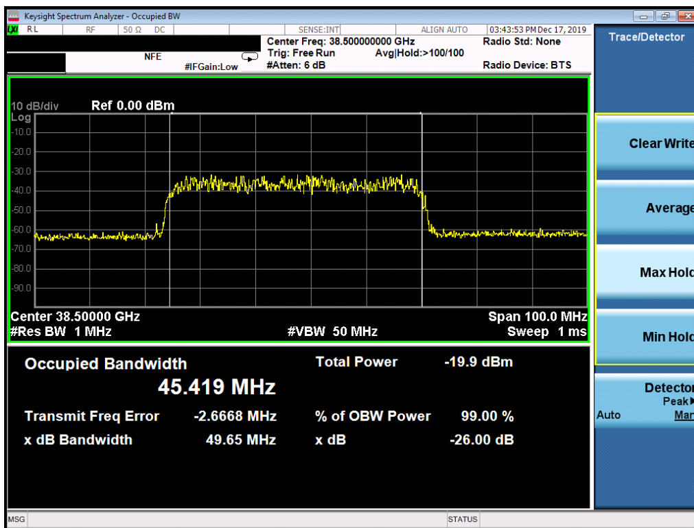
Plot 7-51. Ant2 Occupied Bandwidth Plot (50MHz-1CC – 64QAM – Mid Channel)
