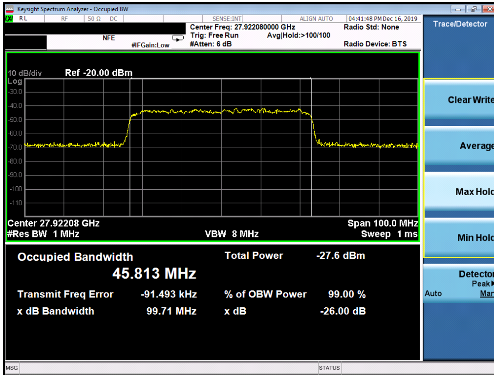
Plot 7-2. Ant1 Occupied Bandwidth Plot (50MHz-1CC – 16QAM – Mid Channel)
