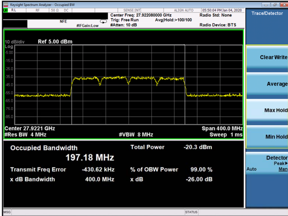
Plot 7-30. Ant3 Occupied Bandwidth Plot (50MHz-4CC – 64QAM – Mid Channel)
