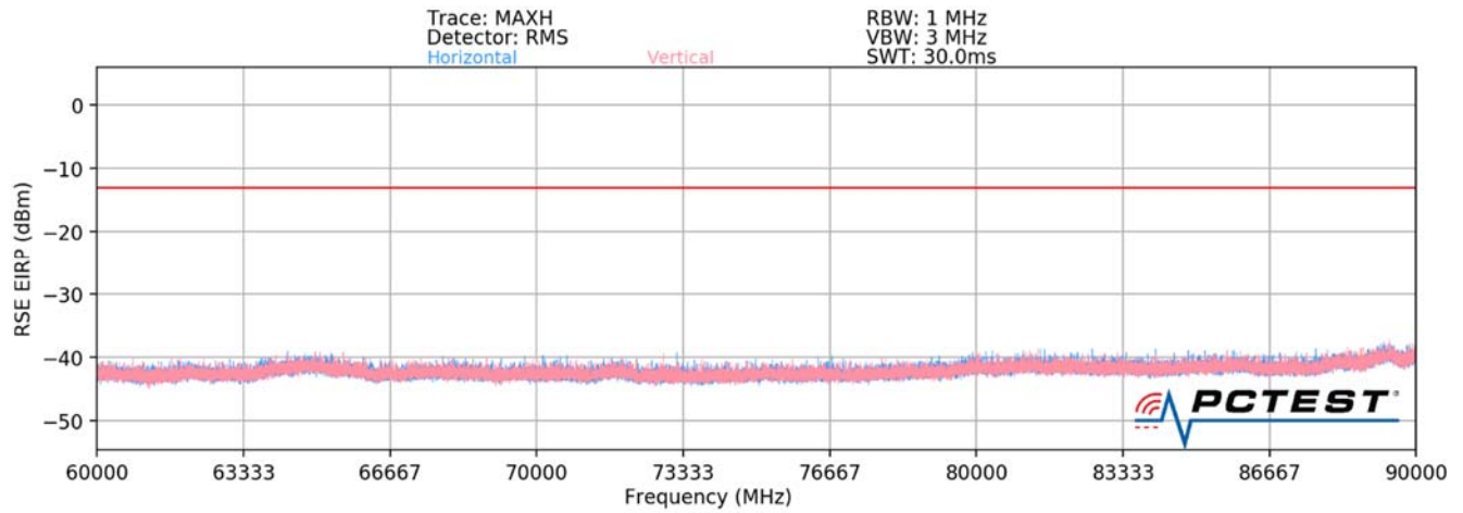
Plot 7-85. Ant2-n261 Radiated Spurious Plot (1CC QPSK Mid Channel V Beam)
