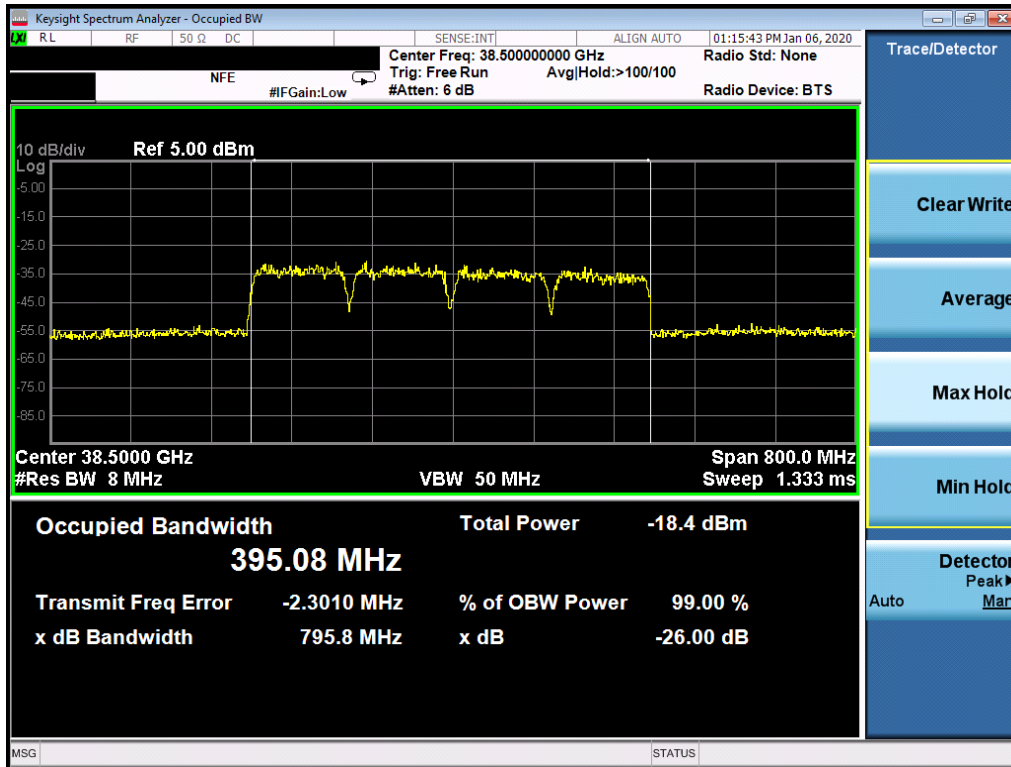
Plot 7-60. Ant2 Occupied Bandwidth Plot (100MHz-4CC – 64QAM – Mid Channel)
