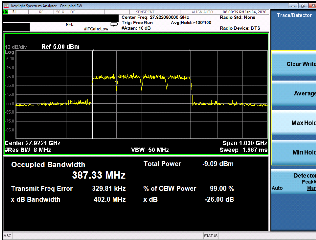
Plot 7-22. Ant2 Occupied Bandwidth Plot (100MHz-4CC – QPSK – Mid Channel)
