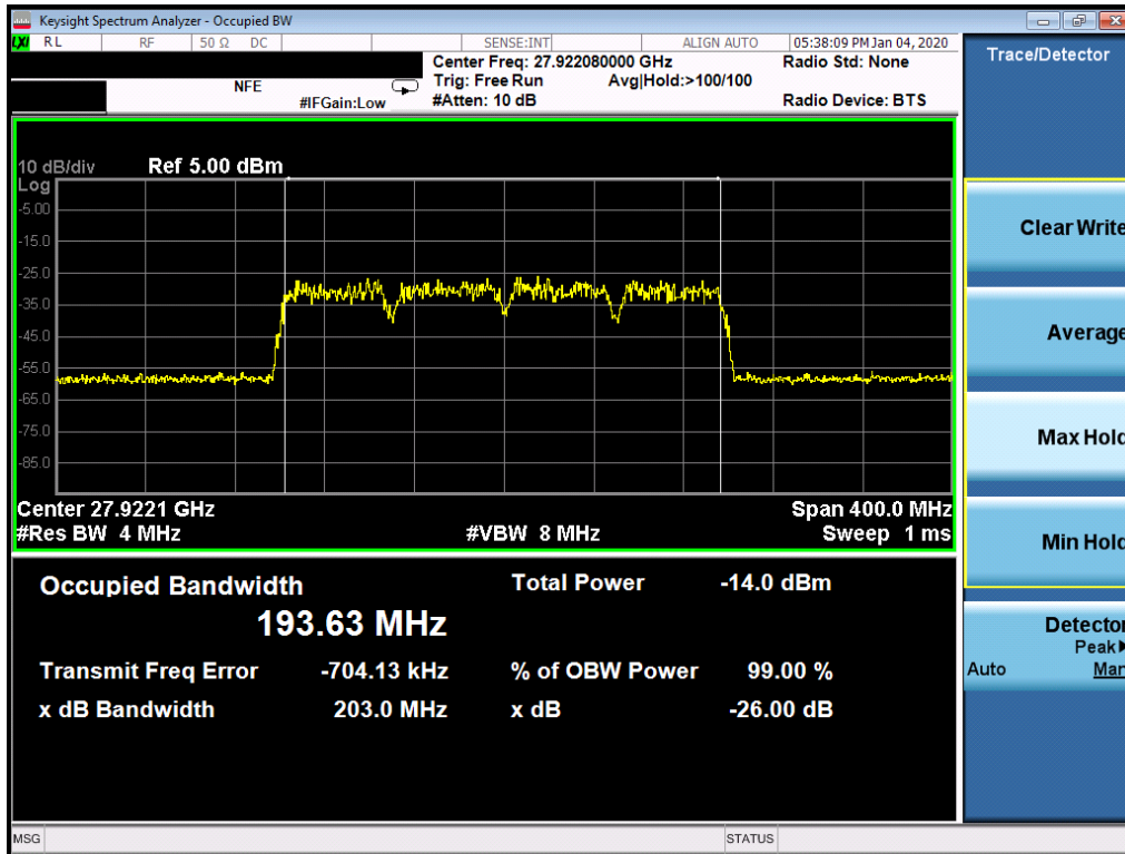
Plot 7-18. Ant2 Occupied Bandwidth Plot (50MHz-4CC – 64QAM – Mid Channel)
