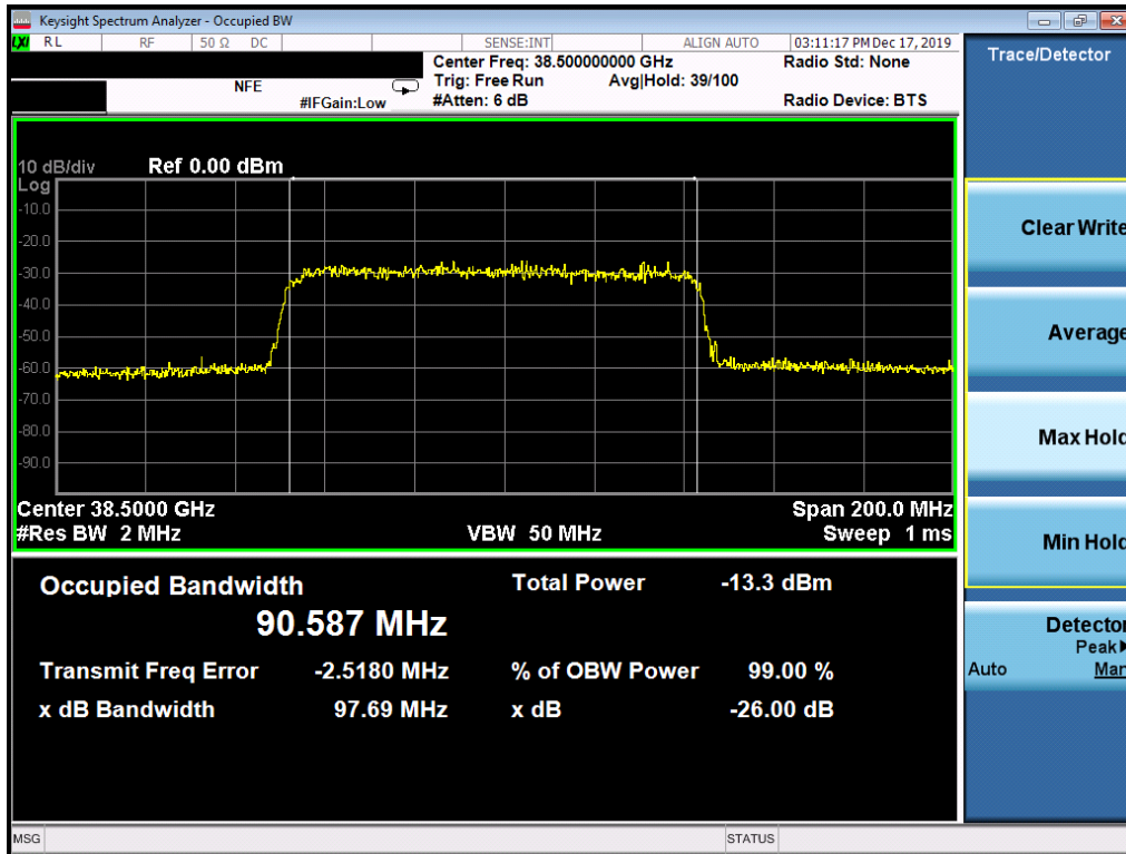
Plot 7-56. Ant2 Occupied Bandwidth Plot (100MHz-1CC – 16QAM – Mid Channel)
