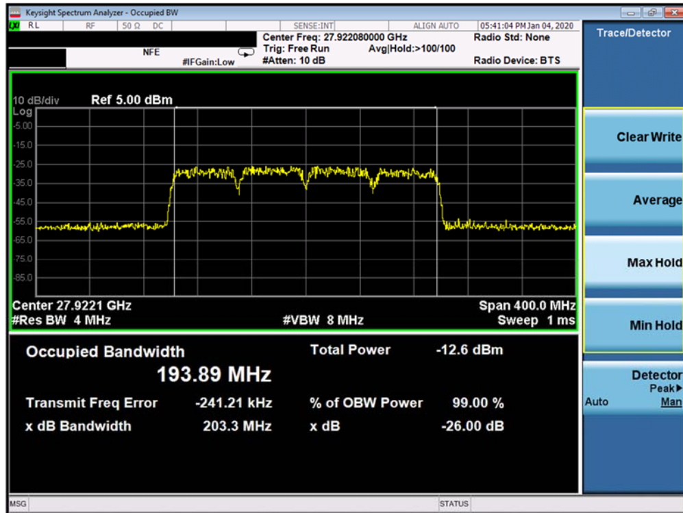
Plot 7-28. Ant3 Occupied Bandwidth Plot (50MHz-4CC – QPSK – Mid Channel)
