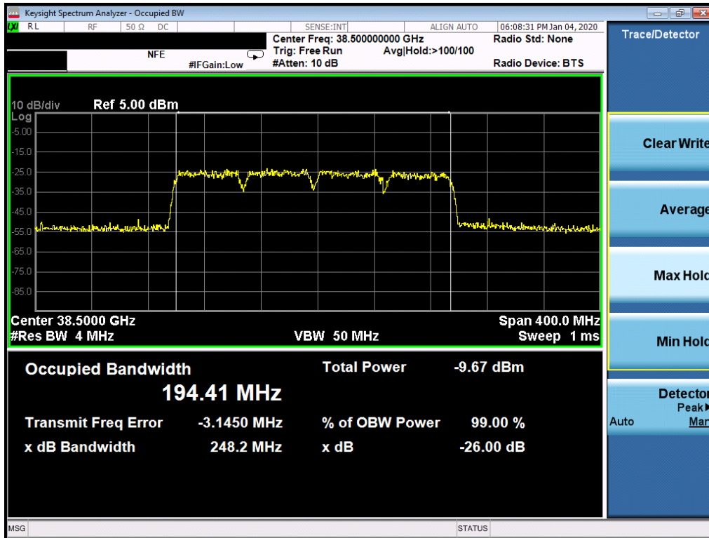
Plot 7-40. Ant1 Occupied Bandwidth Plot (50MHz-4CC – QPSK – Mid Channel)
