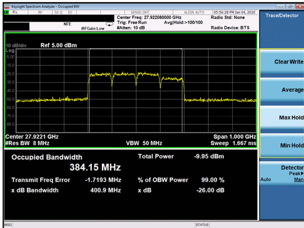
Plot 7-35. Ant3 Occupied Bandwidth Plot (100MHz-4CC – 16QAM – Mid Channel)
