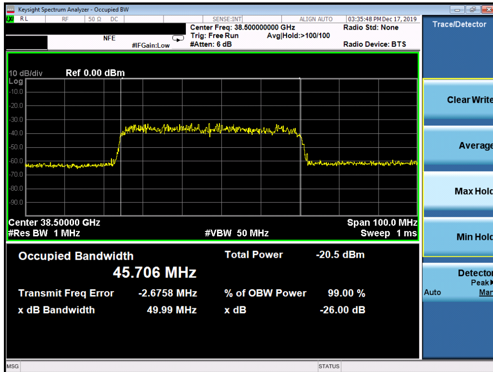
Plot 7-61. Ant3 Occupied Bandwidth Plot (50MHz-1CC – QPSK – Mid Channel)
