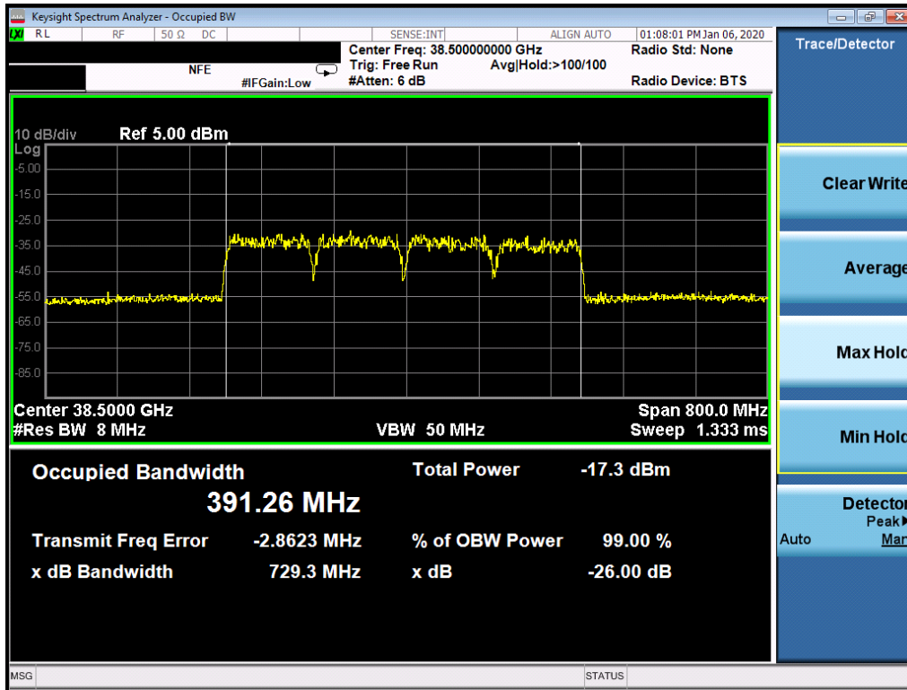
Plot 7-58. Ant2 Occupied Bandwidth Plot (100MHz-4CC – QPSK – Mid Channel)
