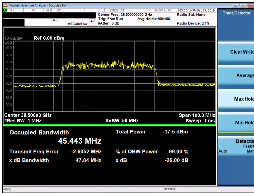
Plot 7-37. Ant1 Occupied Bandwidth Plot (50MHz-1CC – QPSK – Mid Channel)
