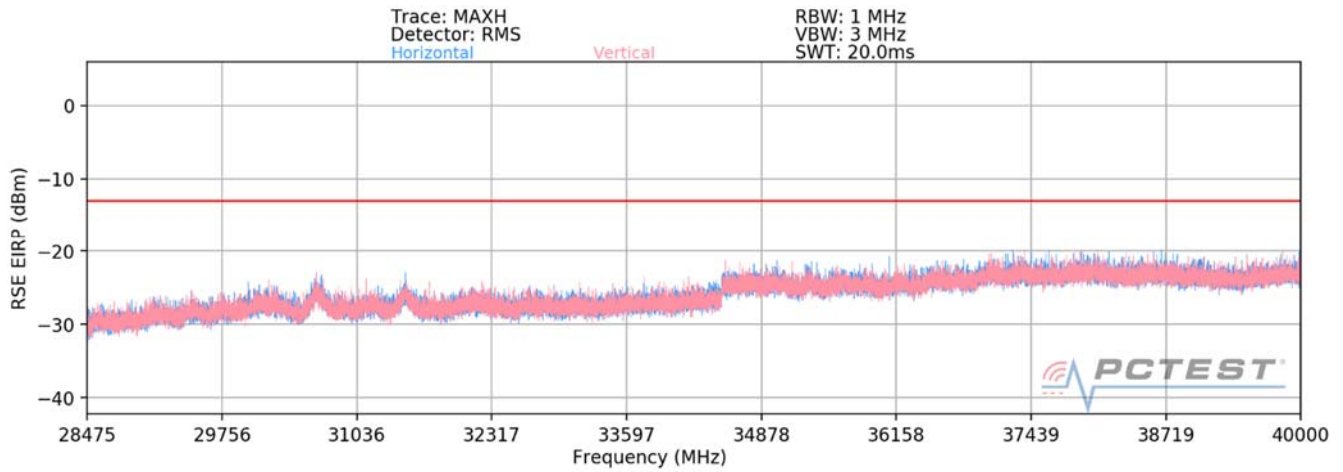
Plot 7-76. Ant1-n261 Radiated Spurious Plot (1CC QPSK Mid Channel V Beam)
