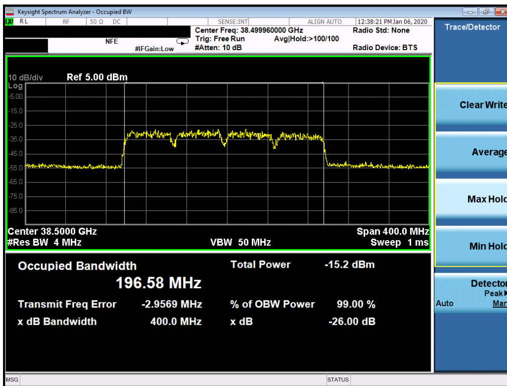
Plot 7-65. Ant3 Occupied Bandwidth Plot (50MHz-4CC – 16QAM – Mid Channel)
