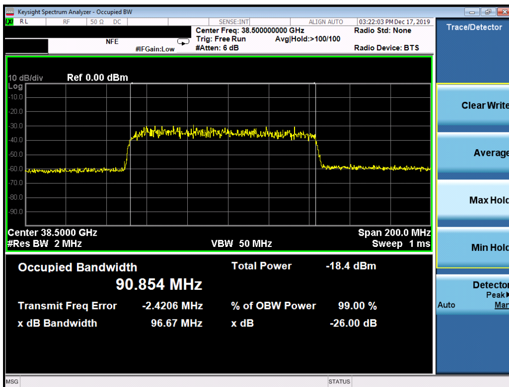
Plot 7-45. Ant1 Occupied Bandwidth Plot (100MHz-1CC – 64QAM – Mid Channel)
