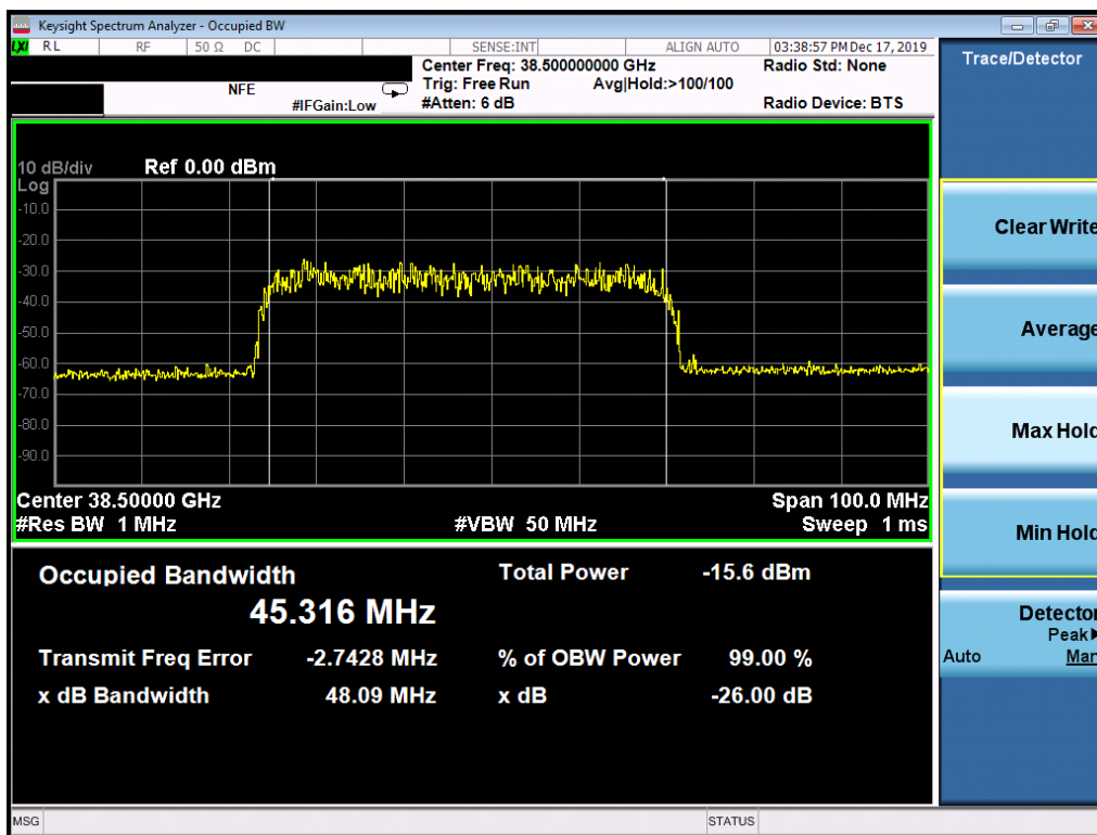
Plot 7-63. Ant3 Occupied Bandwidth Plot (50MHz-1CC – 64QAM – Mid Channel)
