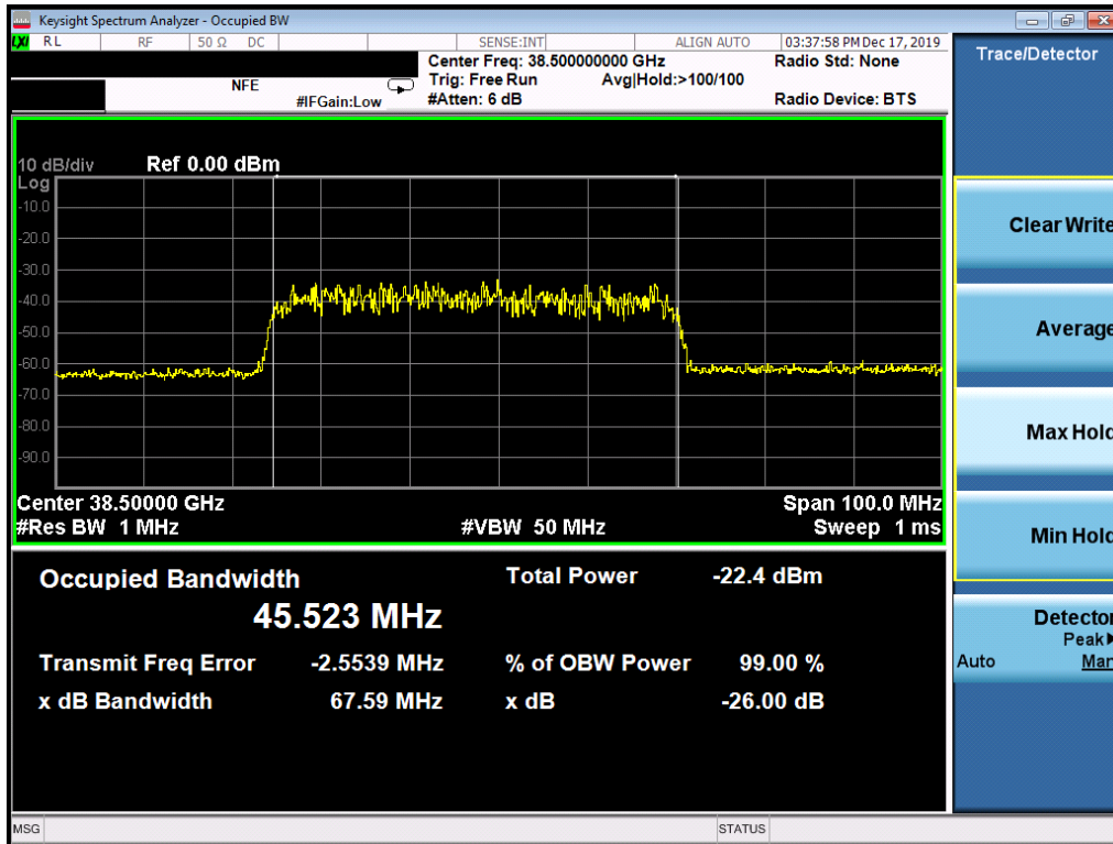
Plot 7-62. Ant3 Occupied Bandwidth Plot (50MHz-1CC – 16QAM – Mid Channel)
