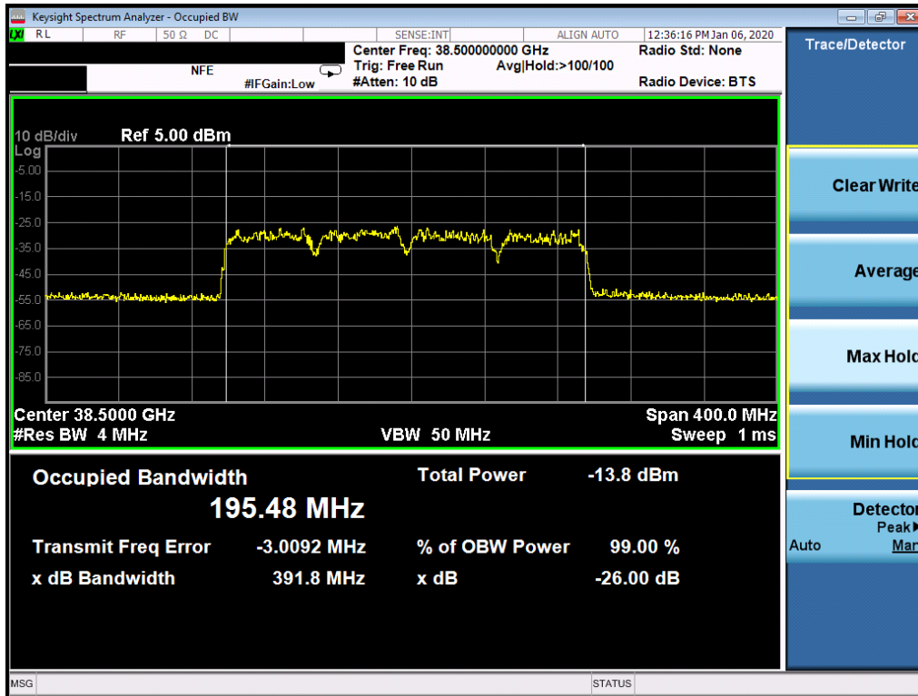
Plot 7-64. Ant3 Occupied Bandwidth Plot (50MHz-4CC – QPSK – Mid Channel)
