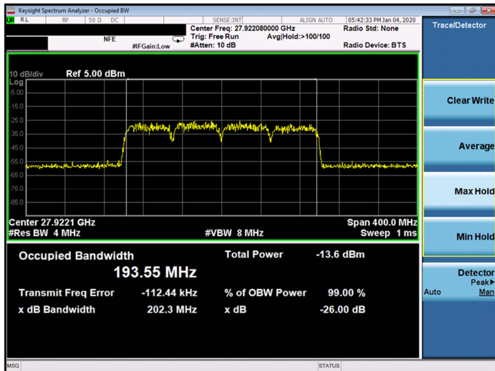
Plot 7-29. Ant3 Occupied Bandwidth Plot (50MHz-4CC – 16QAM – Mid Channel)
