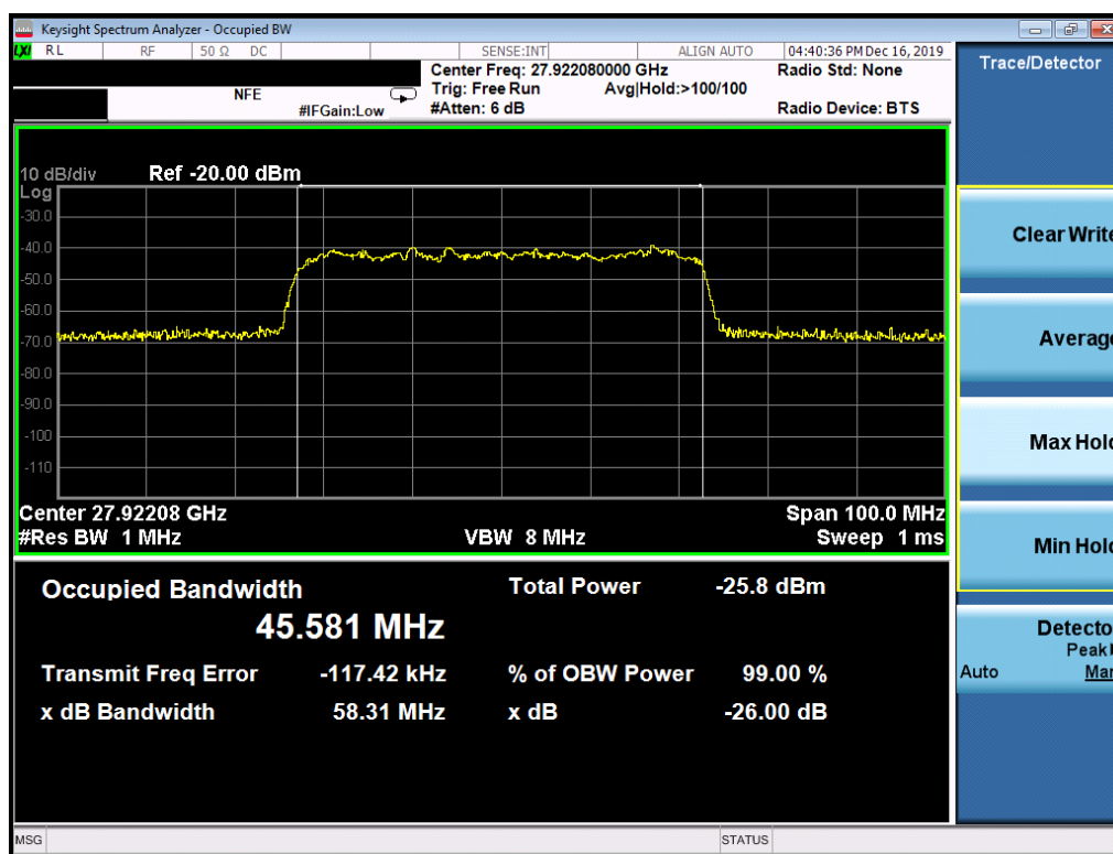
Plot 7-1. Ant1 Occupied Bandwidth Plot (50MHz-1CC – QPSK – Mid Channel)
