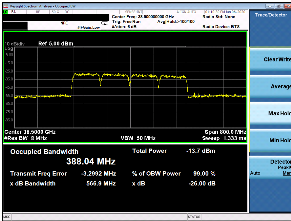
Plot 7-59. Ant2 Occupied Bandwidth Plot (100MHz-4CC – 16QAM – Mid Channel)
