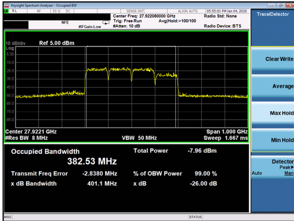
Plot 7-34. Ant3 Occupied Bandwidth Plot (100MHz-4CC – QPSK – Mid Channel)
