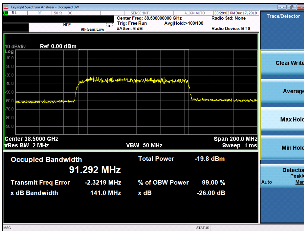
Plot 7-69. Ant3 Occupied Bandwidth Plot (100MHz-1CC – 64QAM – Mid Channel)
