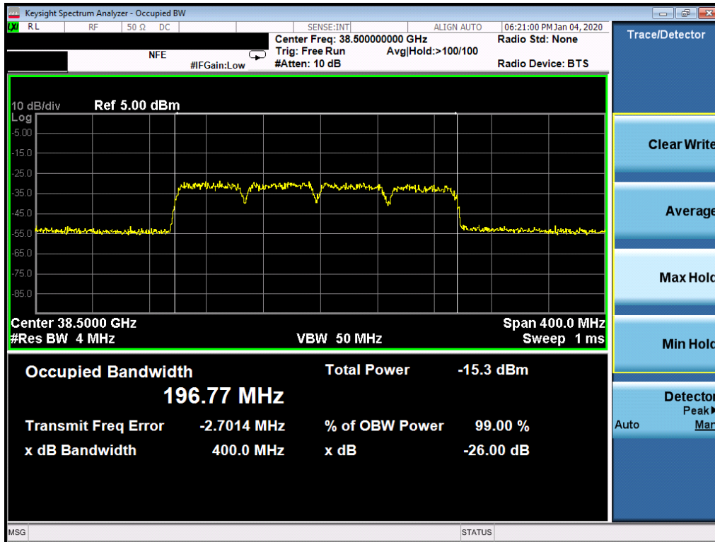
Plot 7-54. Ant2 Occupied Bandwidth Plot (50MHz-4CC – 64QAM – Mid Channel)
