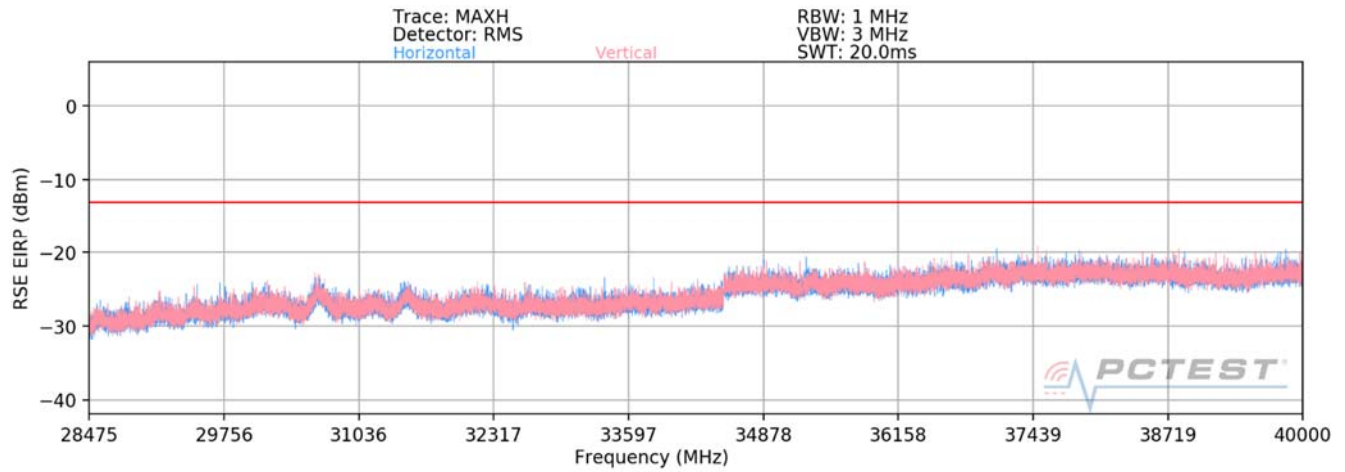
Plot 7-83. Ant2-n261 Radiated Spurious Plot (1CC QPSK Mid Channel V Beam)
