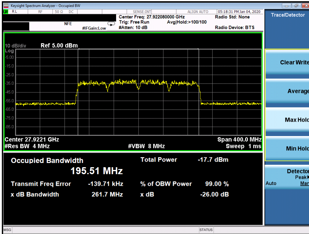
Plot 7-6. Ant1 Occupied Bandwidth Plot (50MHz-4CC – 64QAM – Mid Channel)
