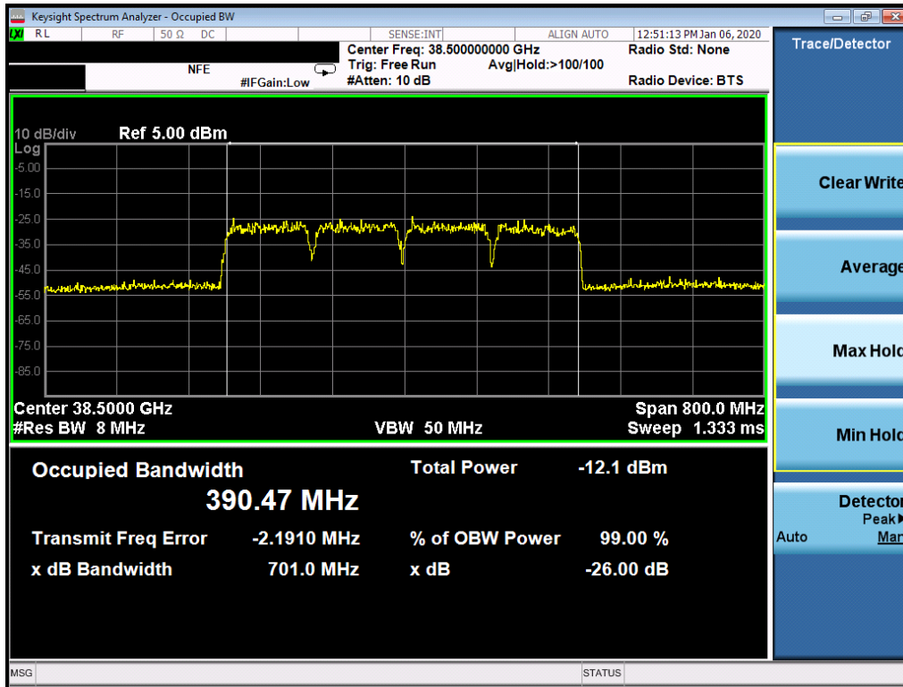
Plot 7-46. Ant1 Occupied Bandwidth Plot (100MHz-4CC – QPSK – Mid Channel)
