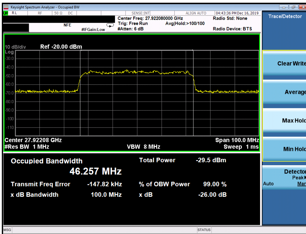
Plot 7-3. Ant1 Occupied Bandwidth Plot (50MHz-1CC – 64QAM – Mid Channel)
