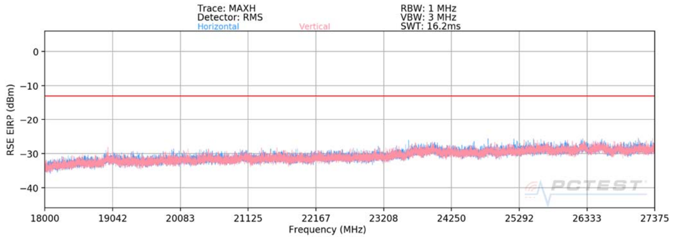
Plot 7-75. Ant1-n261 Radiated Spurious Plot (1CC QPSK Mid Channel V Beam)
