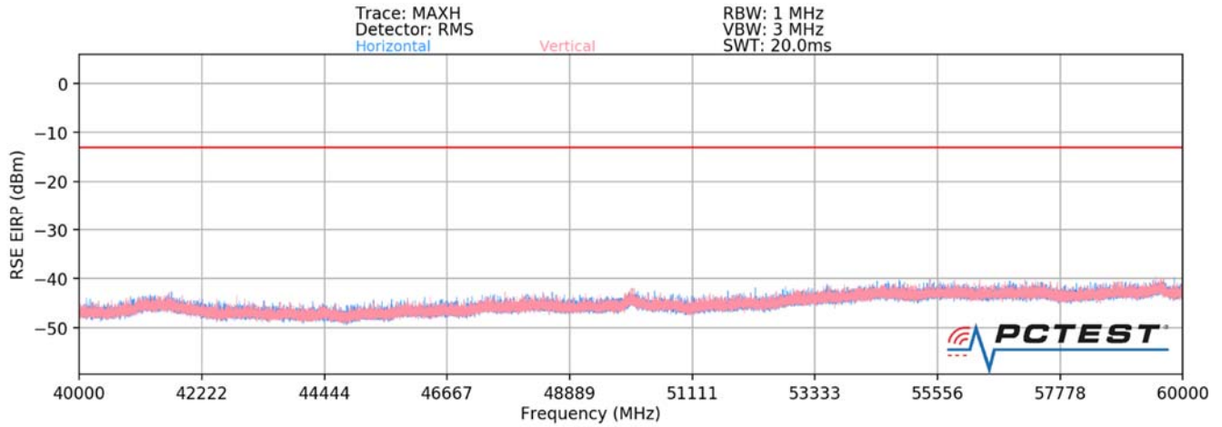
Plot 7-77. Ant1-n261 Radiated Spurious Plot (1CC QPSK Mid Channel V Beam)
