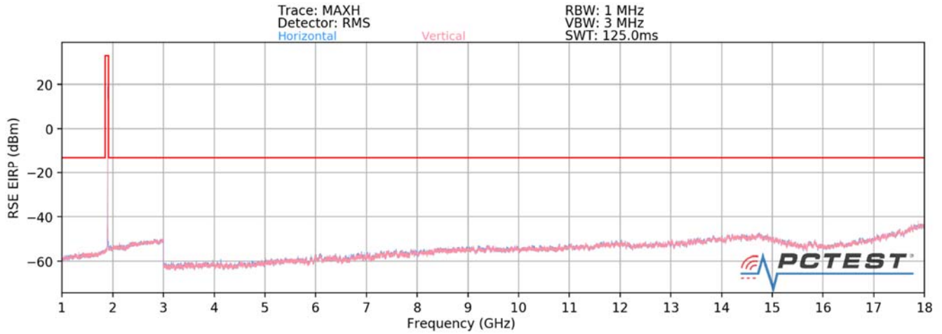
Plot 7-81. Ant2-n261 Radiated Spurious Plot 1GHz - 18GHz (1CC QPSK Mid Channel V Beam)
