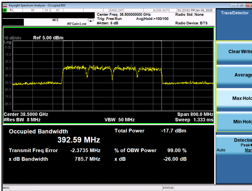
Plot 7-71. Ant3 Occupied Bandwidth Plot (100MHz-4CC – 16QAM – Mid Channel)
