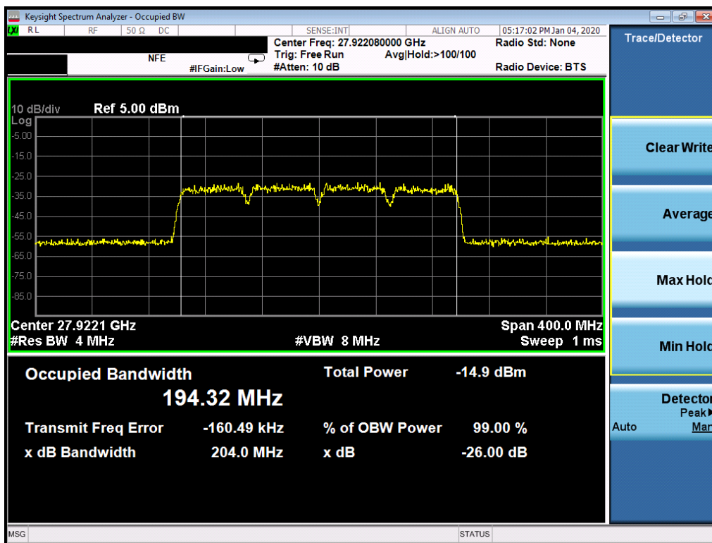
Plot 7-5. Ant1 Occupied Bandwidth Plot (50MHz-4CC – 16QAM – Mid Channel)
