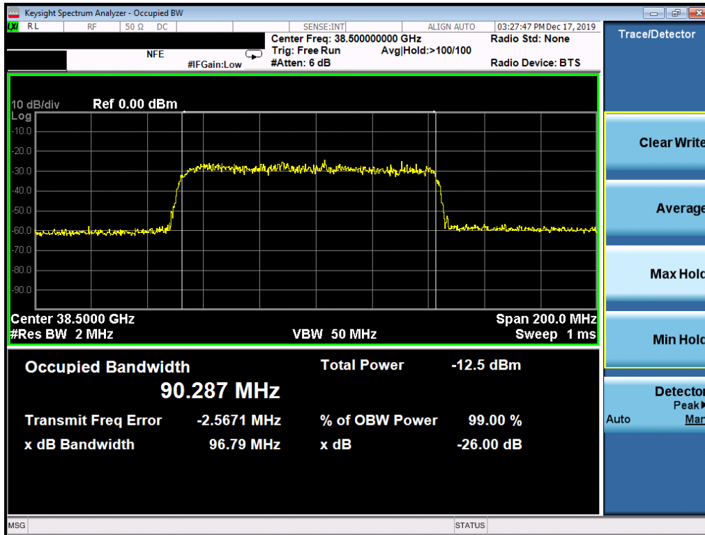
Plot 7-68. Ant3 Occupied Bandwidth Plot (100MHz-1CC – 16QAM – Mid Channel)
