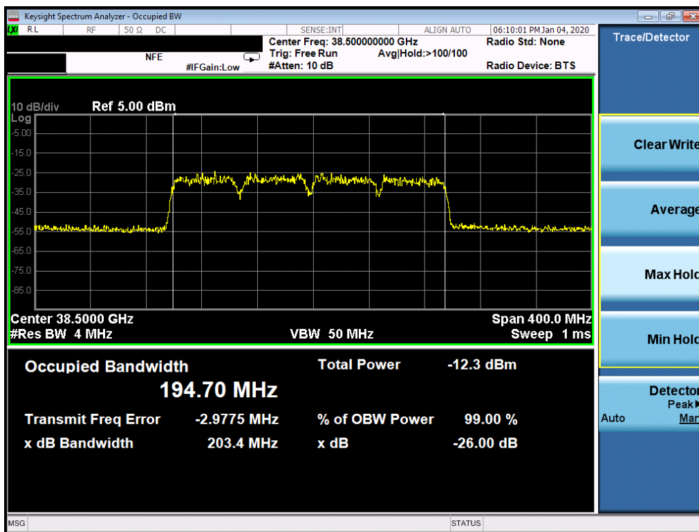
Plot 7-41. Ant1 Occupied Bandwidth Plot (50MHz-4CC – 16QAM – Mid Channel)
