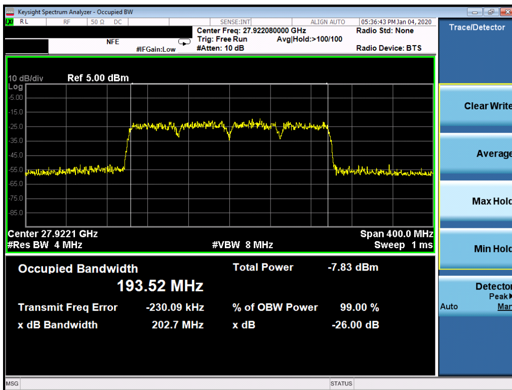
Plot 7-17. Ant2 Occupied Bandwidth Plot (50MHz-4CC – 16QAM – Mid Channel)
