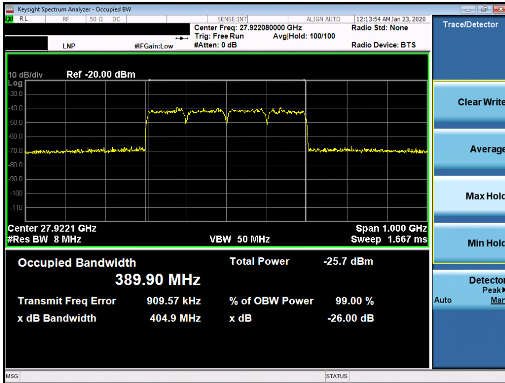
Plot 7-10. Ant1 Occupied Bandwidth Plot (100MHz-4CC – QPSK – Mid Channel)
