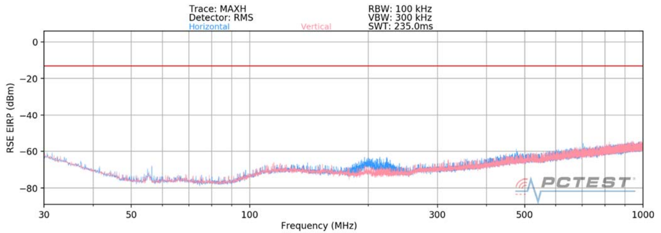
Plot 7-87. Ant3-n261 Radiated Spurious Plot (1CC QPSK Mid Channel V Beam)
