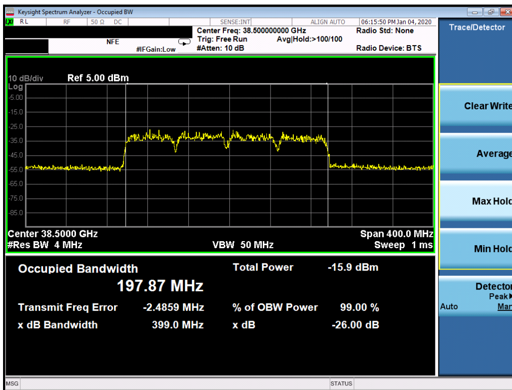
Plot 7-53. Ant2 Occupied Bandwidth Plot (50MHz-4CC – 16QAM – Mid Channel)
