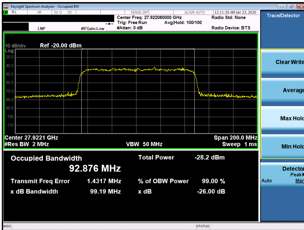
Plot 7-9. Ant1 Occupied Bandwidth Plot (100MHz-1CC – 64QAM – Mid Channel)
