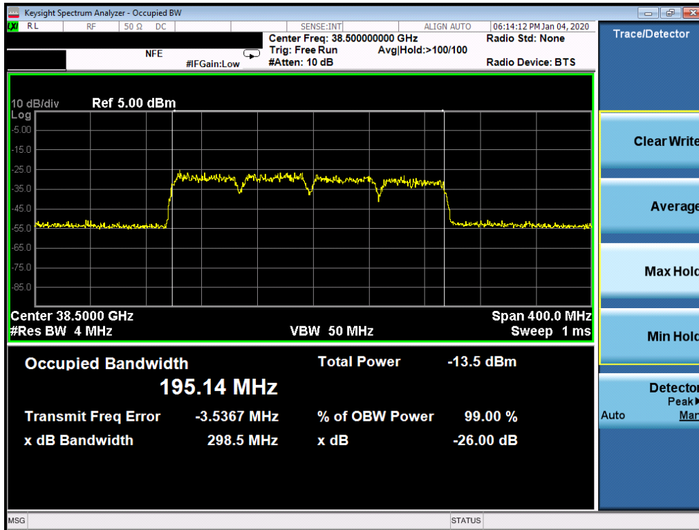
Plot 7-52. Ant2 Occupied Bandwidth Plot (50MHz-4CC – QPSK – Mid Channel)
