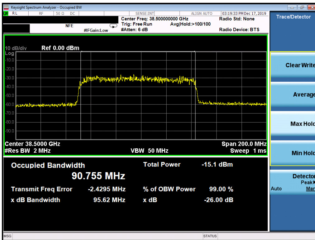
Plot 7-43. Ant1 Occupied Bandwidth Plot (100MHz-1CC – QPSK – Mid Channel)
