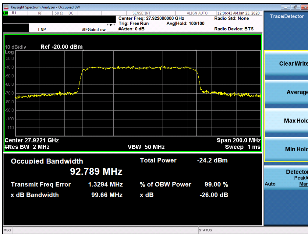
Plot 7-7. Ant1 Occupied Bandwidth Plot (100MHz-1CC – QPSK – Mid Channel)
