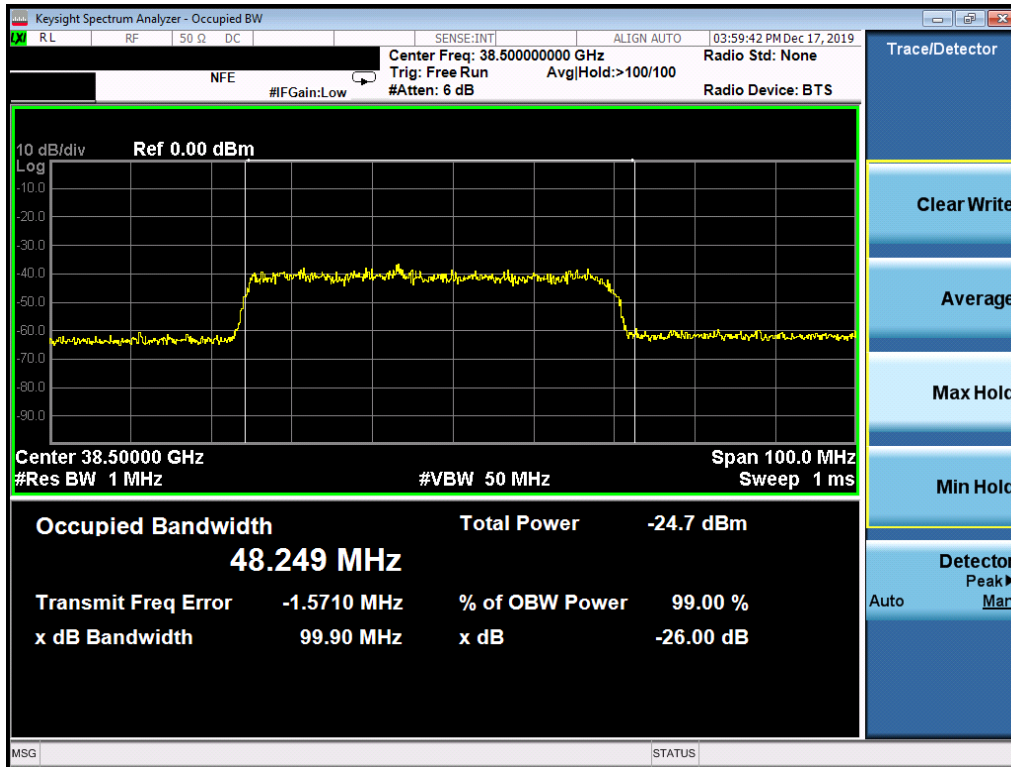
Plot 7-38. Ant1 Occupied Bandwidth Plot (50MHz-1CC – 16QAM – Mid Channel)
