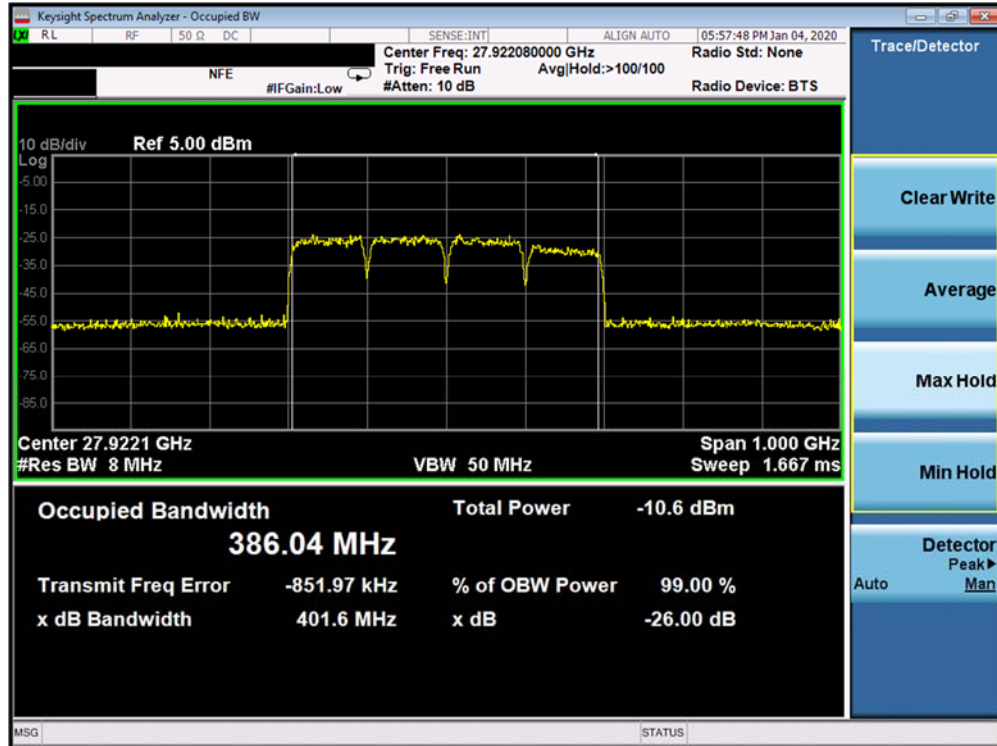
Plot 7-36. Ant3 Occupied Bandwidth Plot (100MHz-4CC – 64QAM – Mid Channel)
