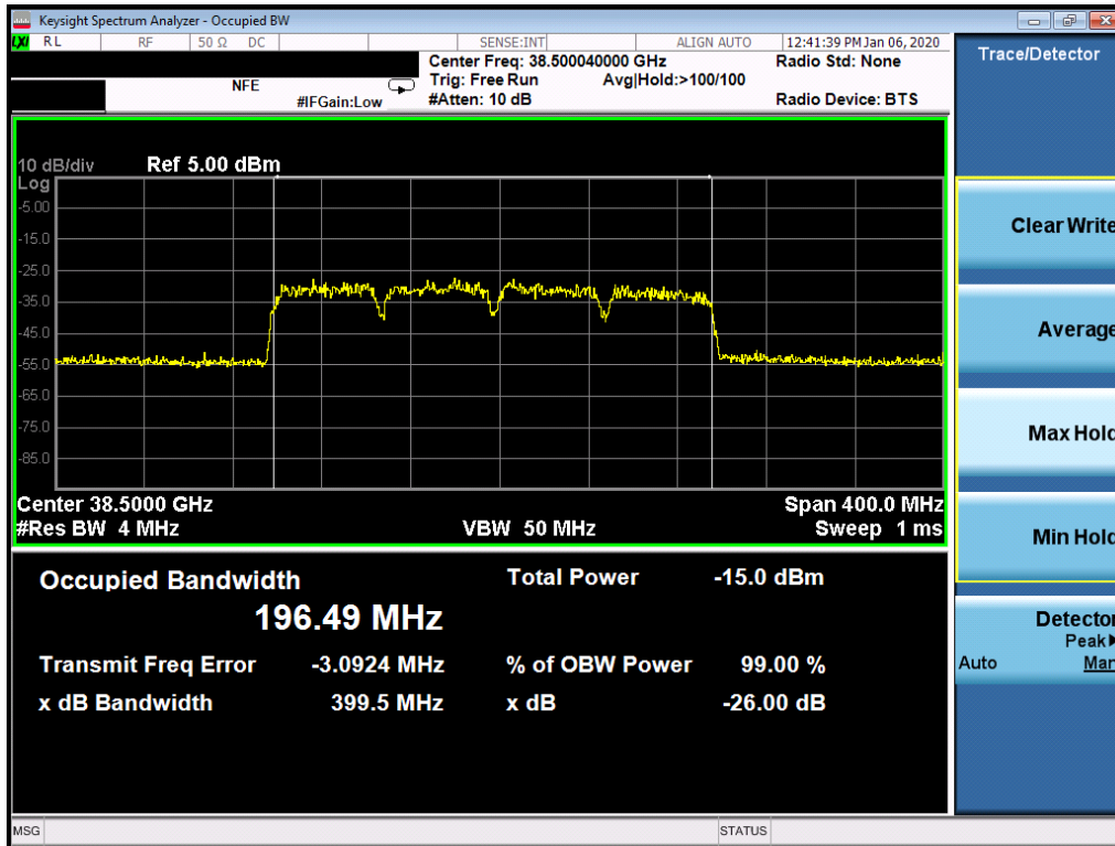
Plot 7-66. Ant3 Occupied Bandwidth Plot (50MHz-4CC – 64QAM – Mid Channel)
