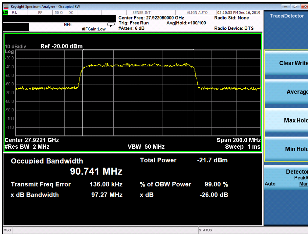
Plot 7-21. Ant2 Occupied Bandwidth Plot (100MHz-1CC – 64QAM – Mid Channel)
