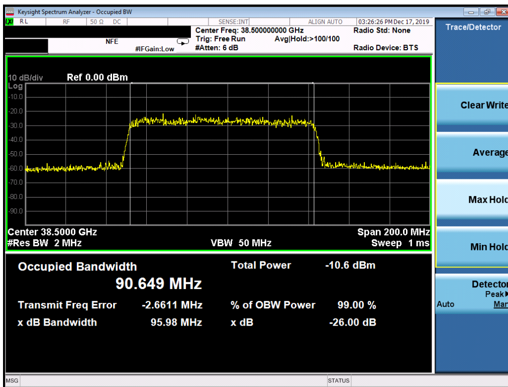
Plot 7-67. Ant3 Occupied Bandwidth Plot (100MHz-1CC – QPSK – Mid Channel)
