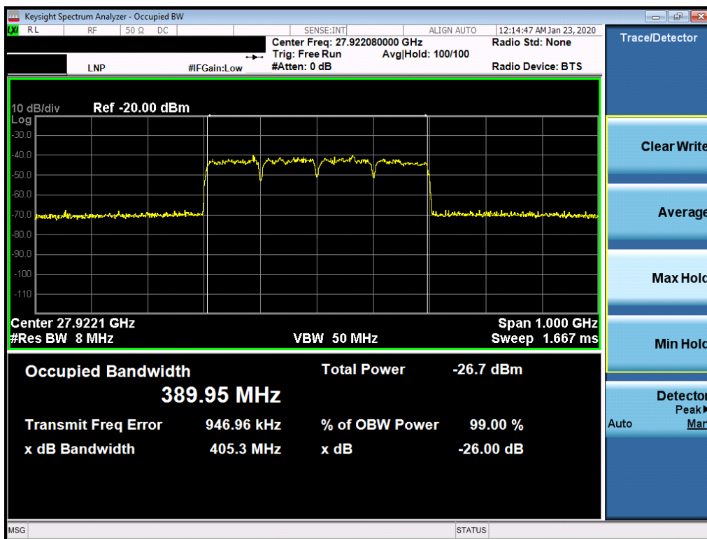
Plot 7-11. Ant1 Occupied Bandwidth Plot (100MHz-4CC – 16QAM – Mid Channel)
