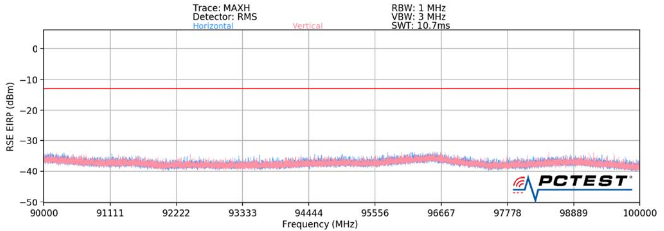
Plot 7-86. Ant2-n261 Radiated Spurious Plot (1CC QPSK Mid Channel V Beam)
