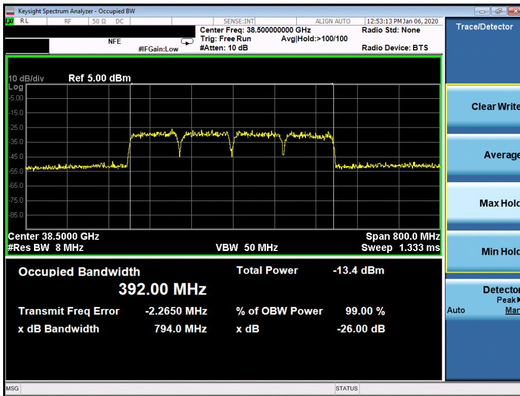
Plot 7-47. Ant1 Occupied Bandwidth Plot (100MHz-4CC – 16QAM – Mid Channel)
