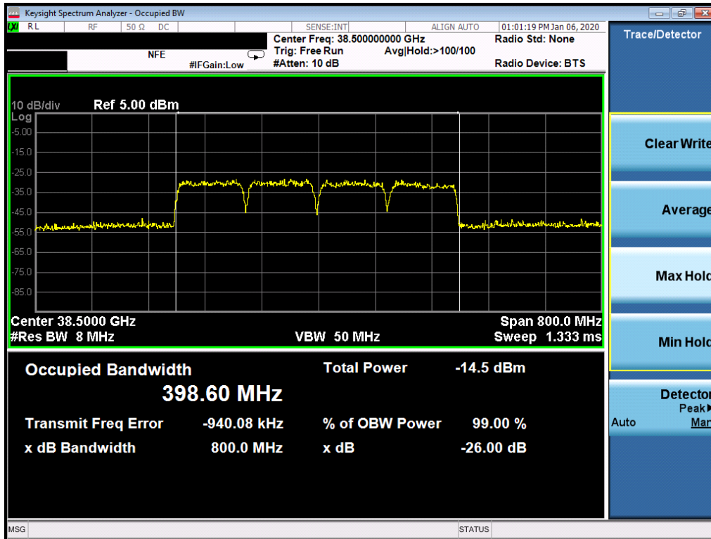
Plot 7-48. Ant1 Occupied Bandwidth Plot (100MHz-4CC – 64QAM – Mid Channel)
