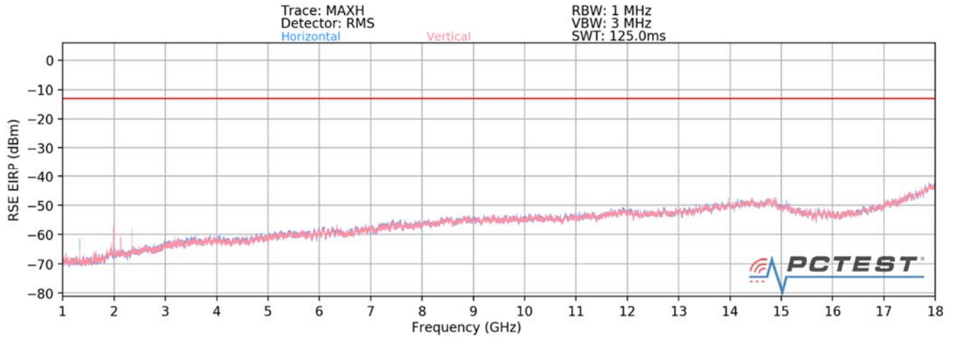
Plot 7-74. Ant1-n261 Radiated Spurious Plot 1GHz - 18GHz (1CC QPSK Mid Channel V Beam)
