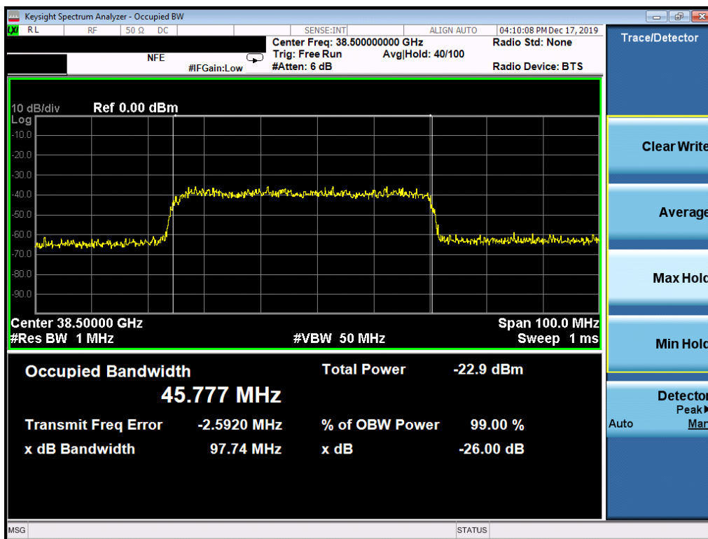
Plot 7-39. Ant1 Occupied Bandwidth Plot (50MHz-1CC – 64QAM – Mid Channel)
