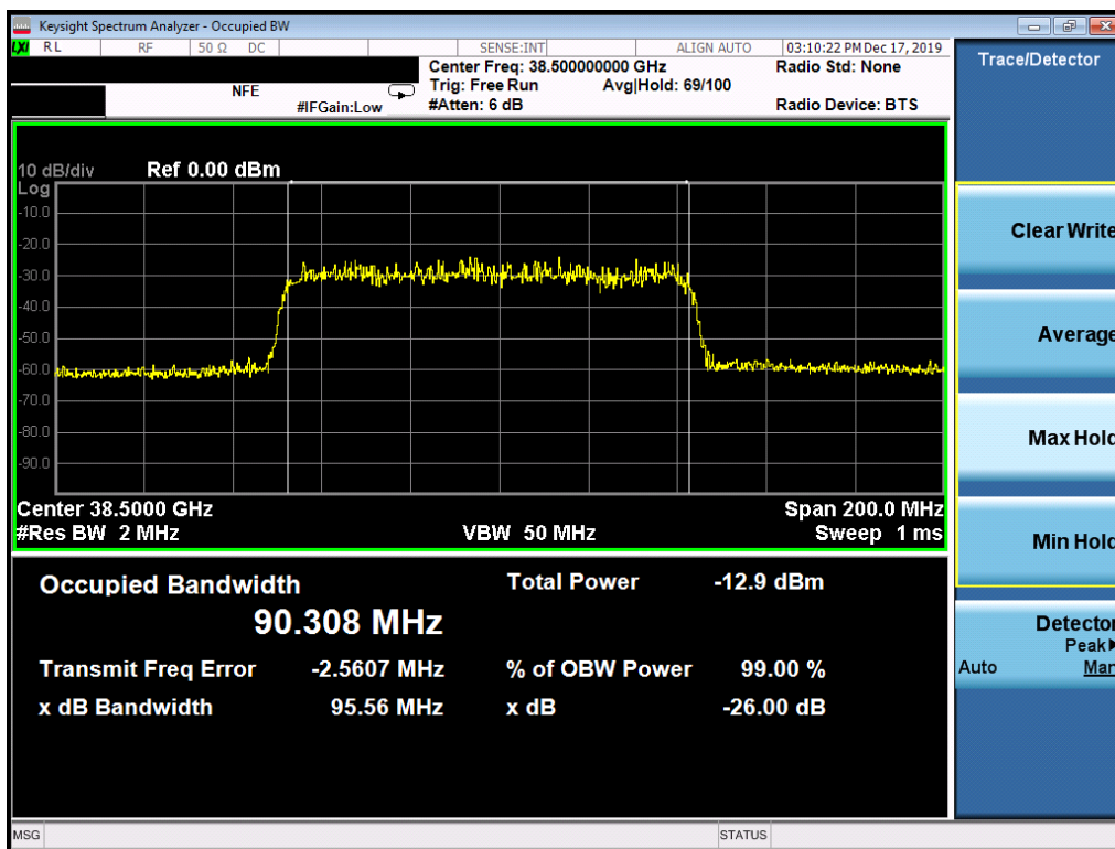
Plot 7-55. Ant2 Occupied Bandwidth Plot (100MHz-1CC – QPSK – Mid Channel)
