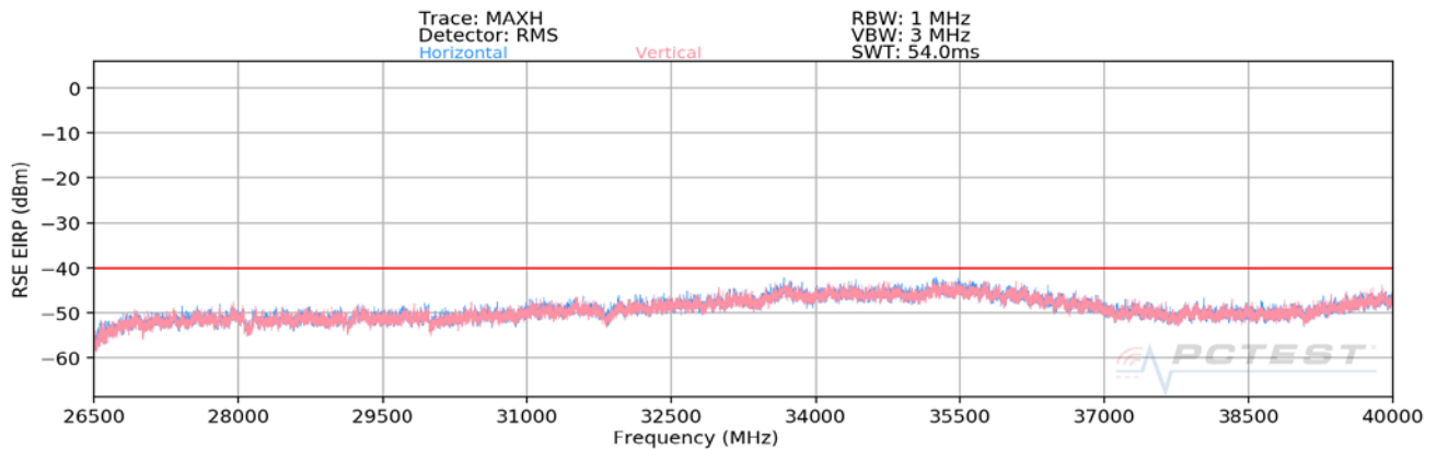
Plot 7-3. Radiated Spurious Plot 26.5 - 40GHz (Band 48)
