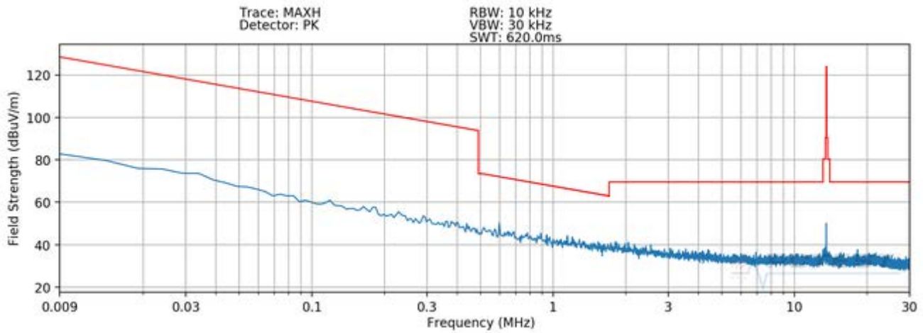
Plot 7-2. Radiated Spurious Plot 9kHz – 30MHz (Pol. Y)
