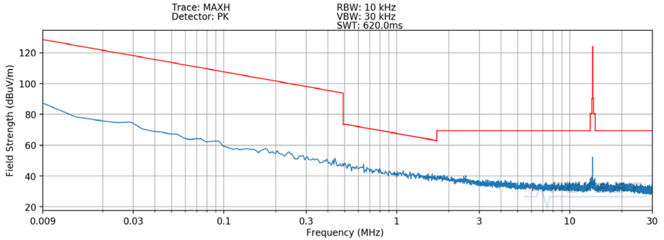
Plot 7-1. Radiated Spurious Plot 9kHz – 30MHz (Pol. X)
