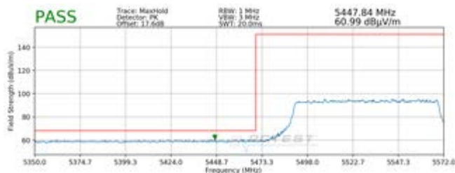
Plot 7-56. Radiated Lower Band Edge Plot SISO ANT1 (Peak – UNII Band 2C – 996 Tones)
