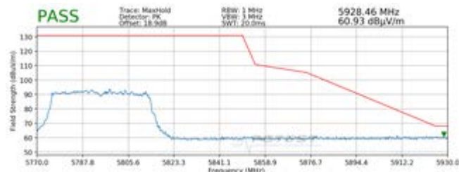
Plot 7-50. Radiated Upper Band Edge Plot SISO ANT1 (Peak – UNII Band 3 – 484 Tones)
