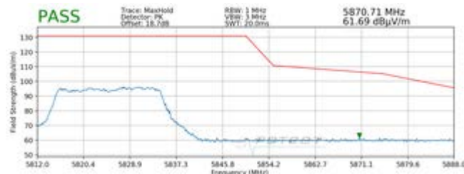
Plot 7-43. Radiated Upper Band Edge Plot SISO ANT1 (Peak - UNII Band 3 - 242 Tones)
