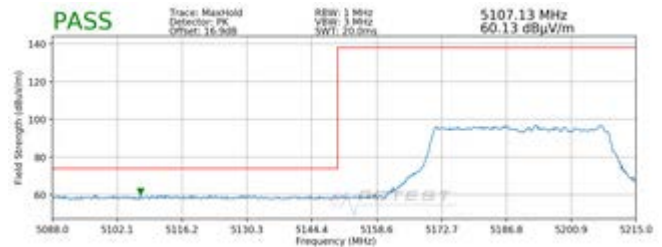
Plot 7-45. Radiated Lower Band Edge Plot SISO ANT1 (Peak - UNII Band 1 - 484 Tones)
