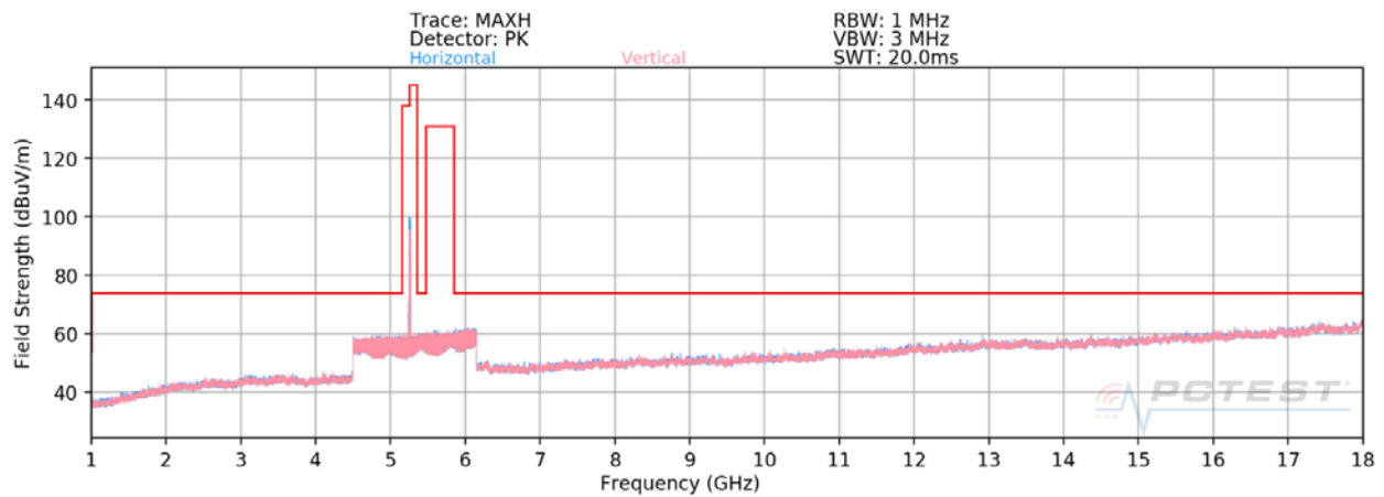
Plot 7-8. Radiated Spurious Plot above 1GHz SISO ANT1 (802.11ax – U2A Ch. 56 – 242 Tones)
