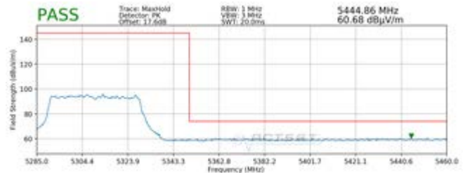
Plot 7-47. Radiated Upper Band Edge Plot SISO ANT1 (Peak - UNII Band 2A - 484 Tones)
