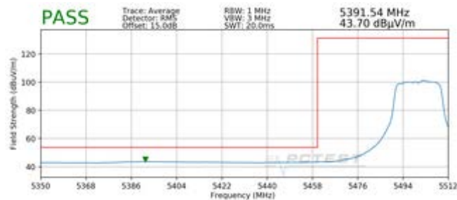
Plot 7-74. Radiated Lower Band Edge Plot MIMO (Average – UNII Band 2C)
