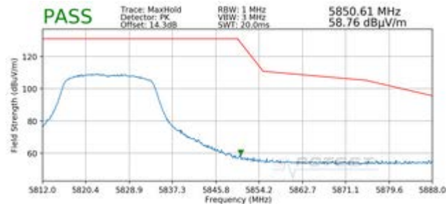
Plot 7-76. Radiated Upper Band Edge Plot MIMO (Peak – UNII Band 3)
