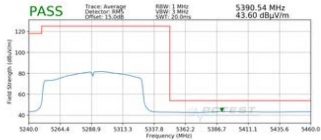
Plot 7-95. Radiated Band Edge Plot MIMO (Average – WCP+DD)
