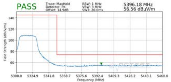
Plot 7-52. Radiated Upper Band Edge Plot SISO ANT2 (Peak – UNII Band 2A)
