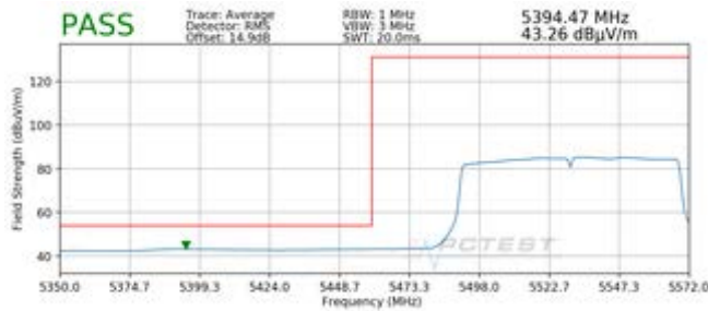
Plot 7-67. Radiated Lower Band Edge Plot SISO ANT2 (Average – UNII Band 2C)
