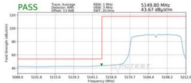
Plot 7-79. Radiated Lower Band Edge Plot MIMO (Average – UNII Band 1)
