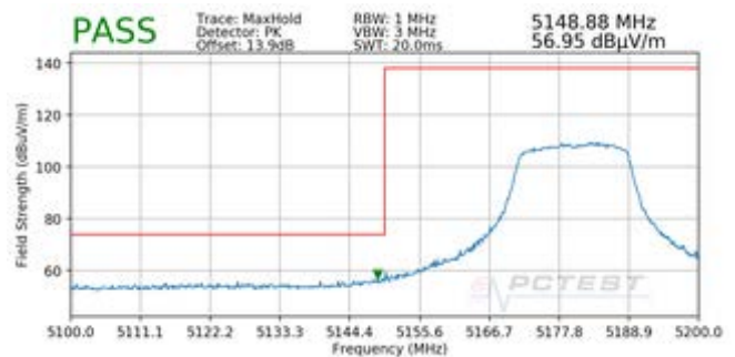
Plot 7-50. Radiated Lower Band Edge Plot SISO ANT2 (Peak – UNII Band 1)
