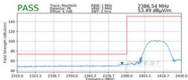
Plot 7-22. Radiated Restricted Lower Band Edge Measurement SISO ANT2 (Peak)
