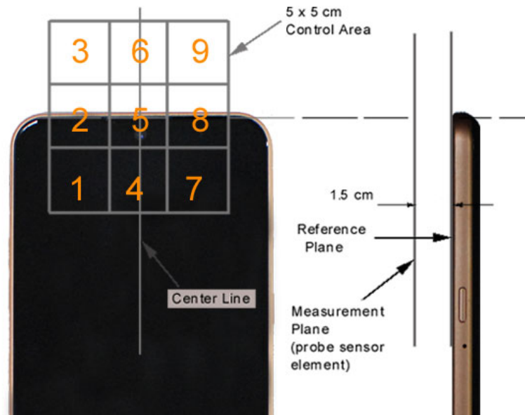
Figure 18-7 5x5 Scan grid above WD (Acoustic Centered Scan Area Pictured)
