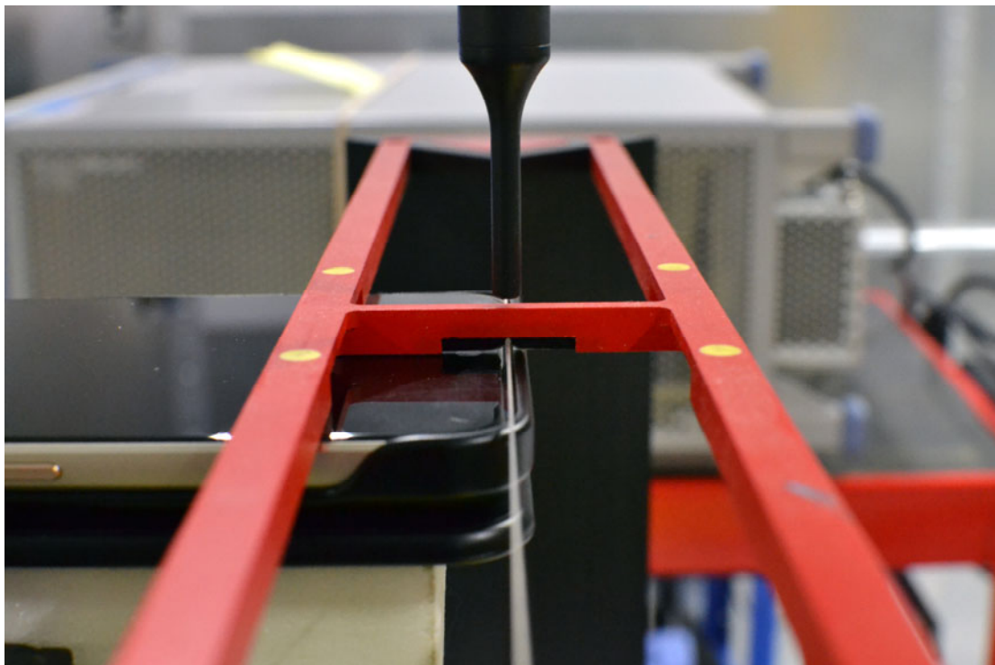
Figure 18-6 HAC Phantom Plane Alignment – Dual Display Open
