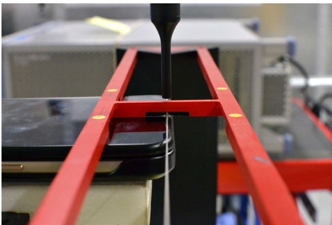
Figure 18-4 HAC Phantom Plane Alignment – Dual Display Closed
