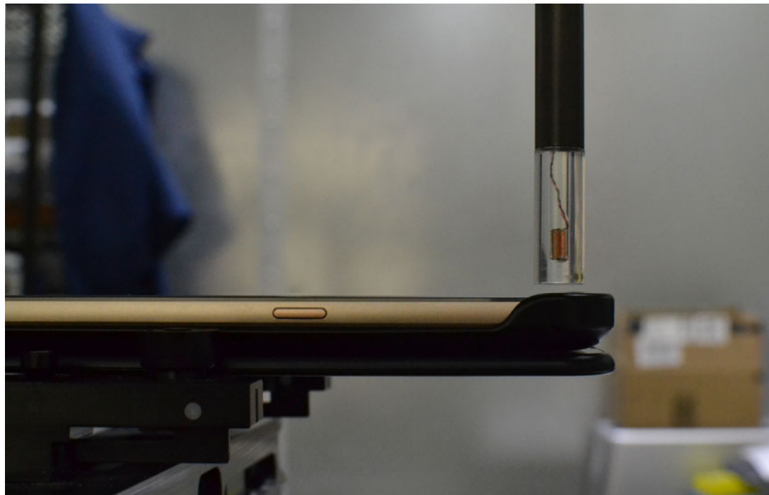
Figure 16-6 Test Setup for Wireless Device with Dual Display - Open
