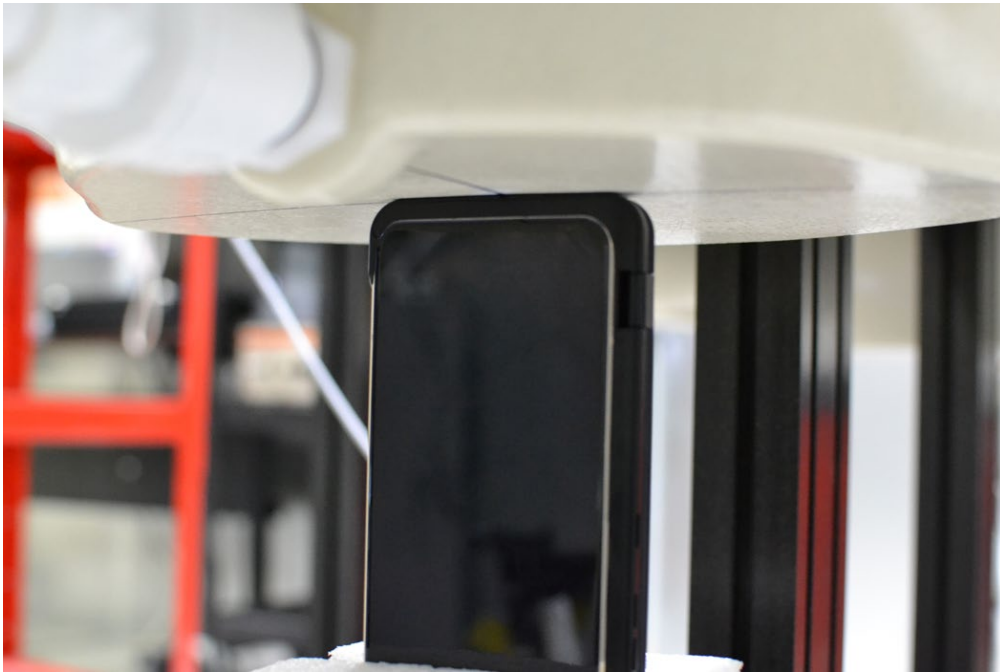
SAR Test Setup Photo 23 – Bottom Side at 0 mm with Dual Display Cover Position #3 (360 degrees)
