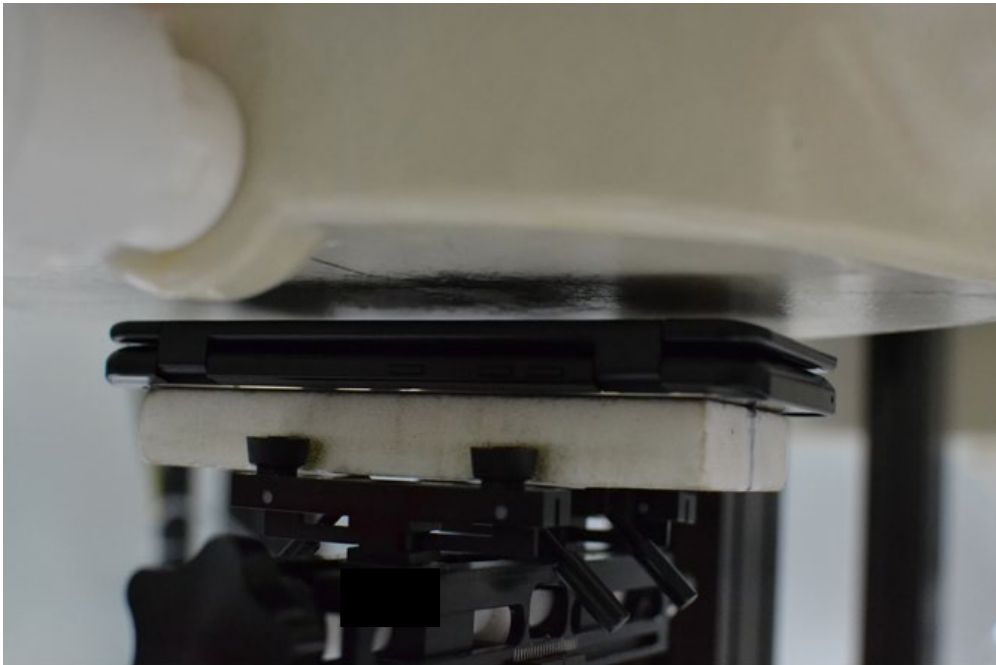
SAR Test Setup Photo 10 – Back Side at 10 mm with Dual Display Cover Position #3 (360 degrees)
