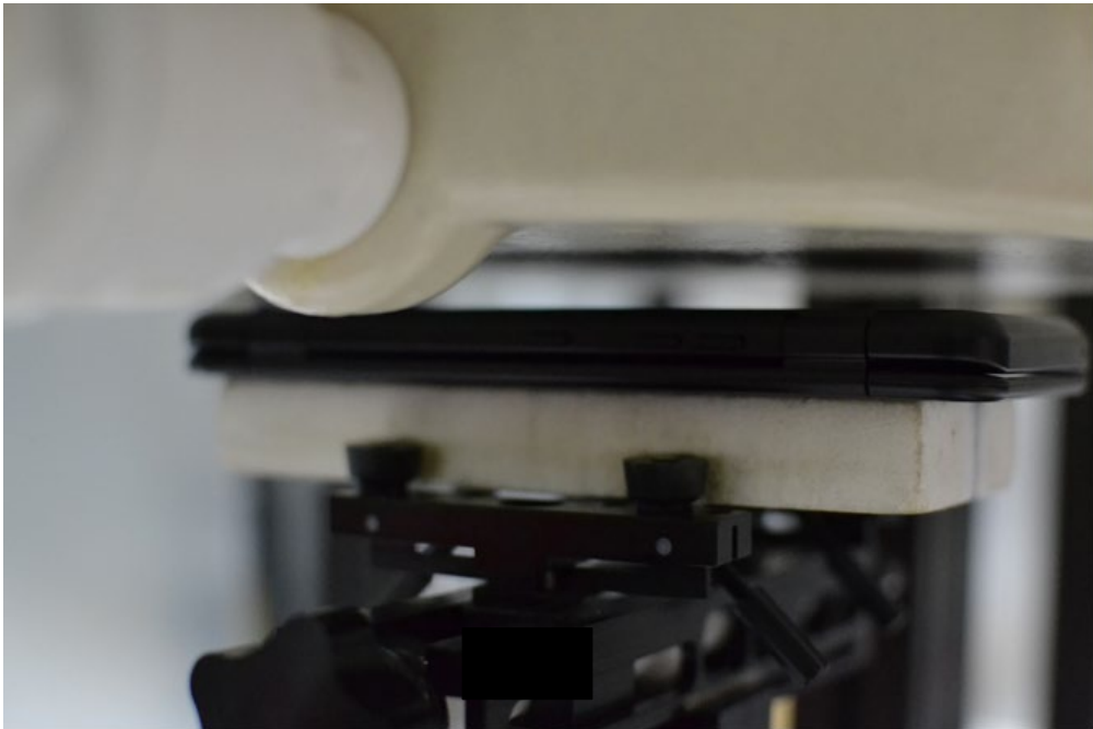
SAR Test Setup Photo 8 – Back Side at 10 mm with Dual Display Cover Position #1 (0 degrees)
