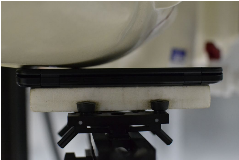
SAR Test Setup Photo 2 – Right Cheek with Dual Display cover Position #1 (0 degrees)
