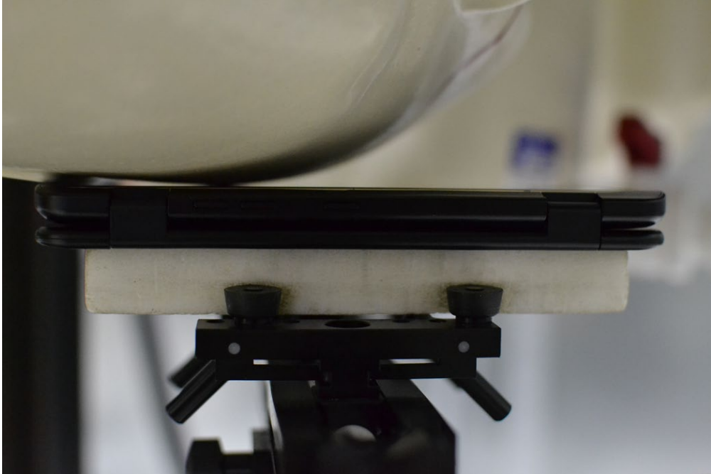
SAR Test Setup Photo 3 – Right Cheek with Dual Display Cover Position #3 (360 degrees)
