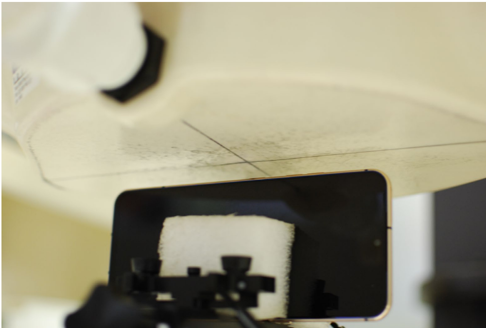
SAR Test Setup Photo 25 – Left Edge at 10 mm
