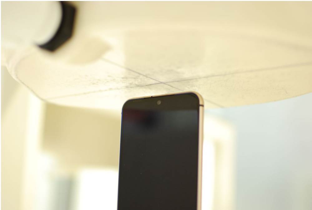
SAR Test Setup Photo 4 – Top Edge at 10 mm
