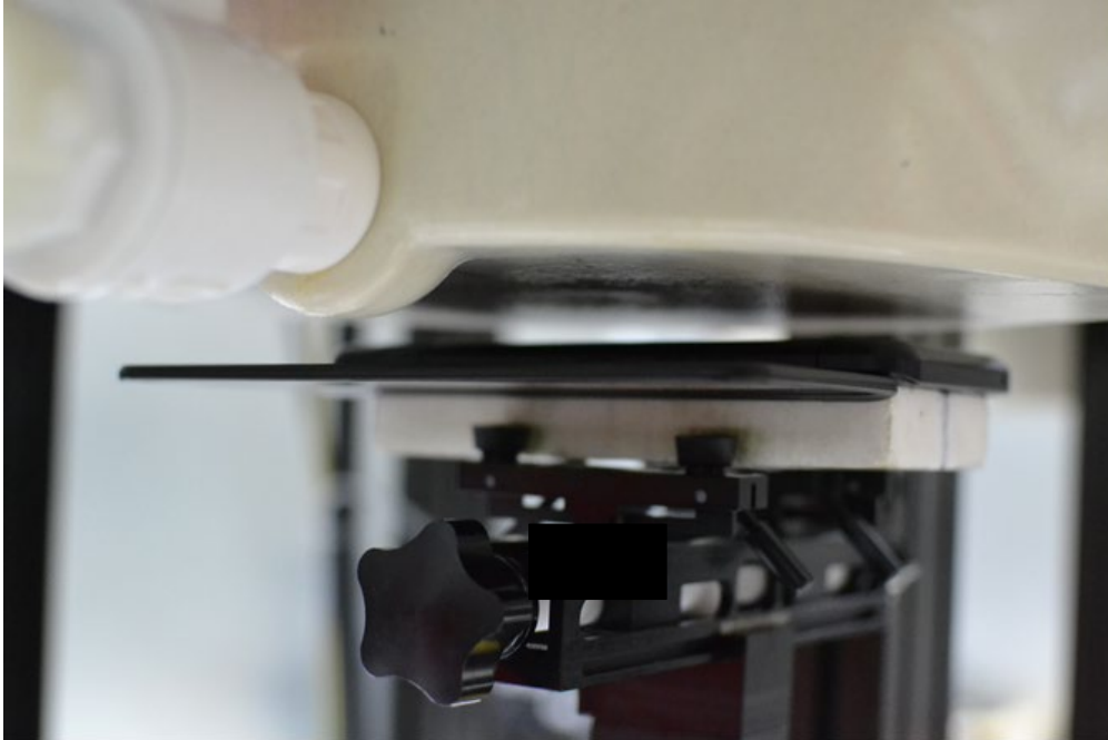
SAR Test Setup Photo 9 – Back Side at 10 mm with Dual Display Cover Position #2 (180 degrees)
