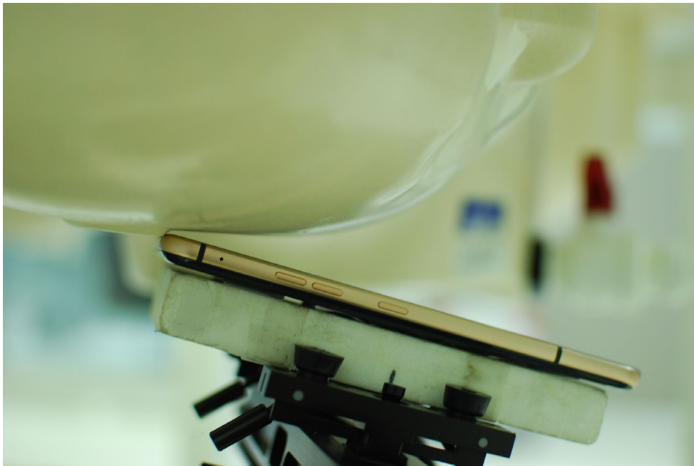
SAR Test Setup Photo 4 – Right Tilt
