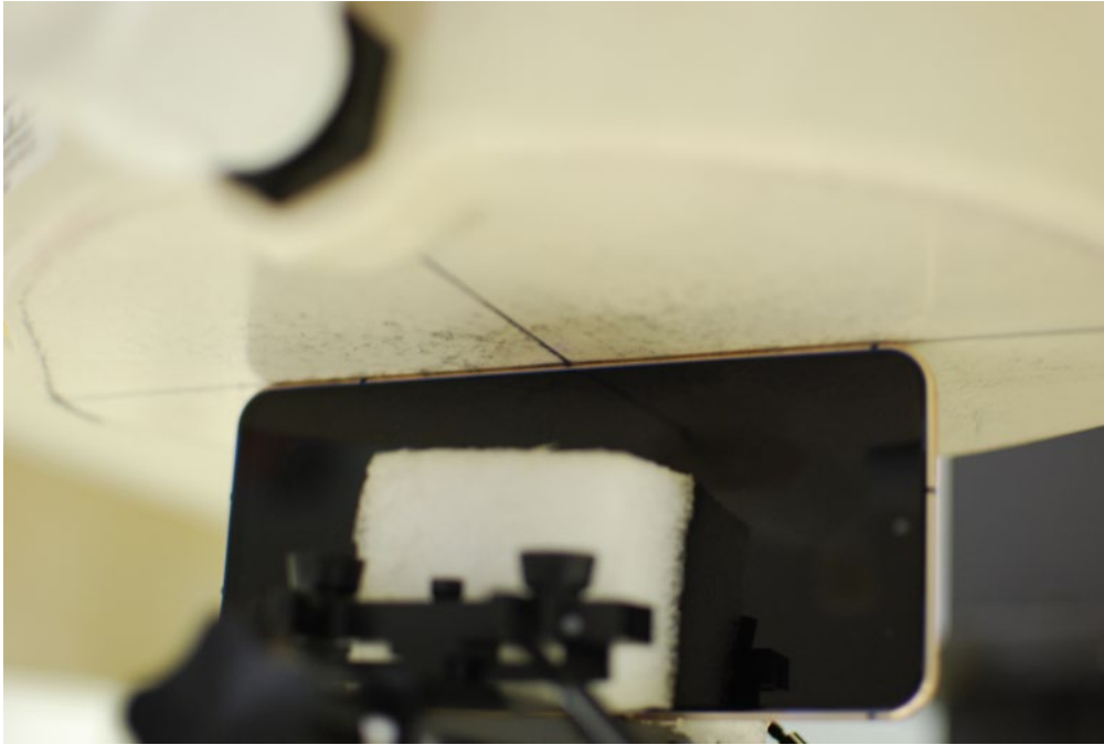
SAR Test Setup Photo 26 – Left Edge at 0 mm
