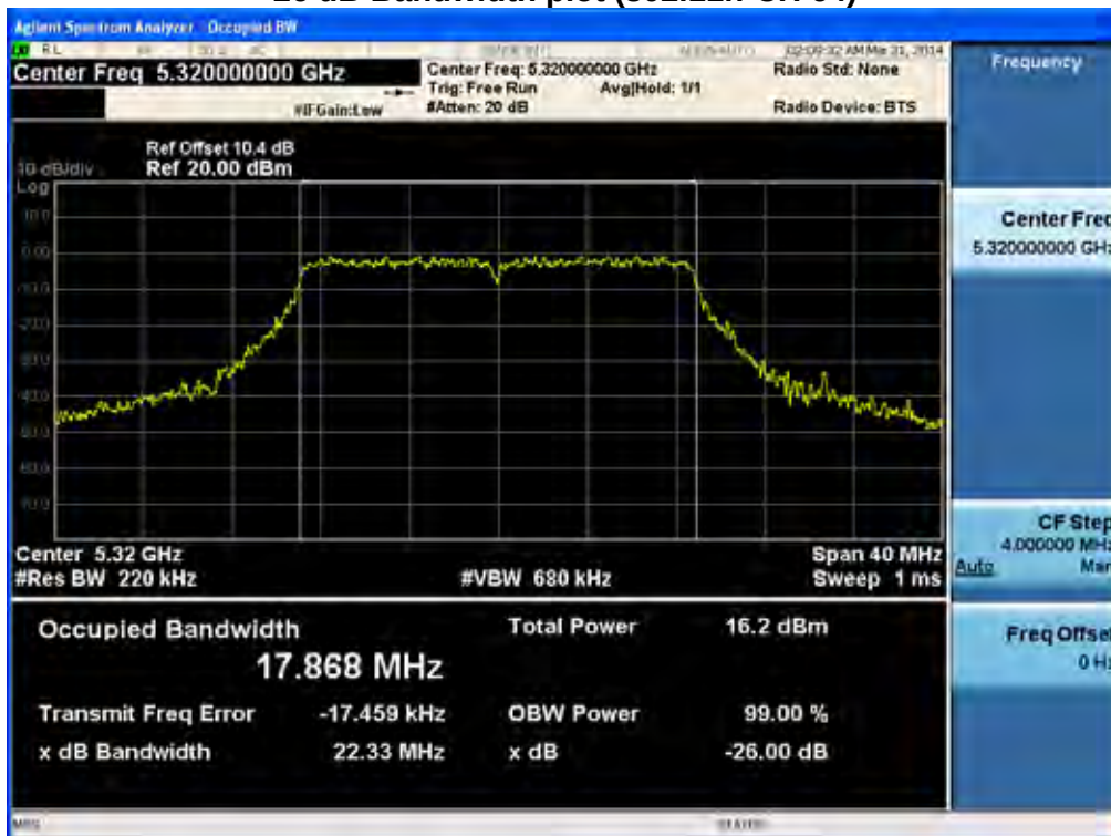
26 dB Bandwidth plot (802.11n-CH 64)
