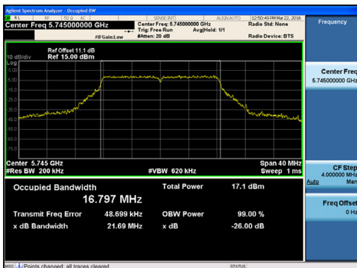
802.11a UNII 3 BAND 99% Bandwidth (Ch.149)
