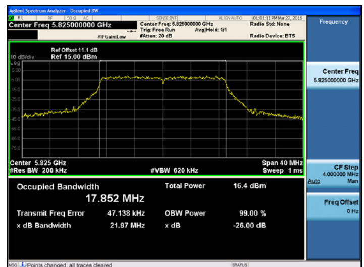
802.11n_20MHz UNII 3 BAND 99% Bandwidth (Ch.165)
