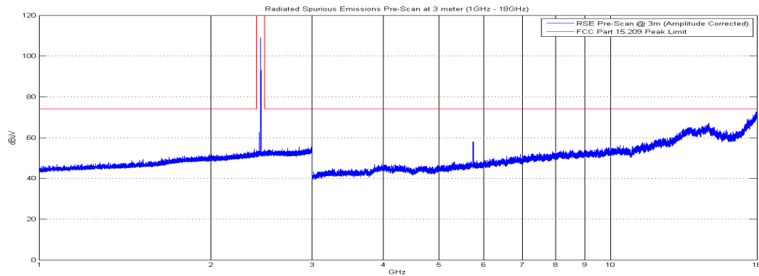
Plot 6-44. Radiated Spurious Plot above 1GHz (BT – Ch. 39, Ant. Pol. H)
