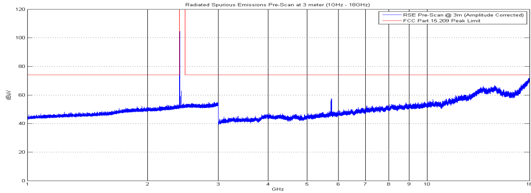
Plot 6-42. Radiated Spurious Plot above 1GHz (BT – Ch. 0, Ant. Pol. H)
