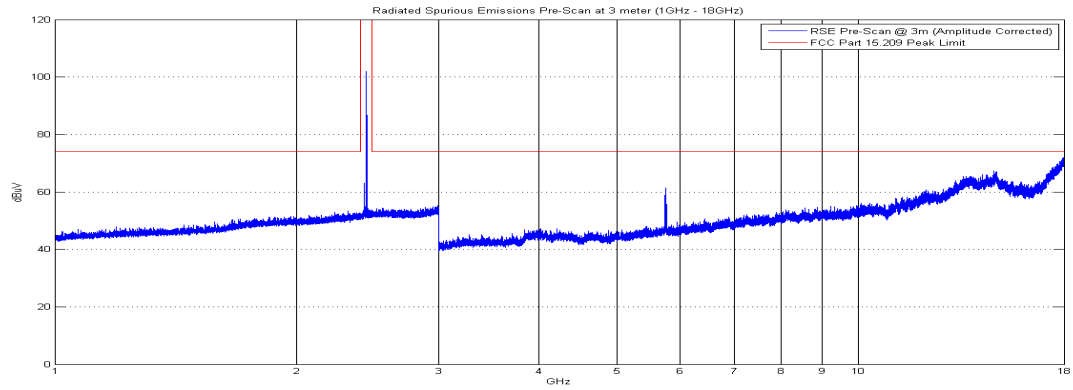
Plot 6-45. Radiated Spurious Plot above 1GHz (BT – Ch. 39, Ant. Pol. V)
