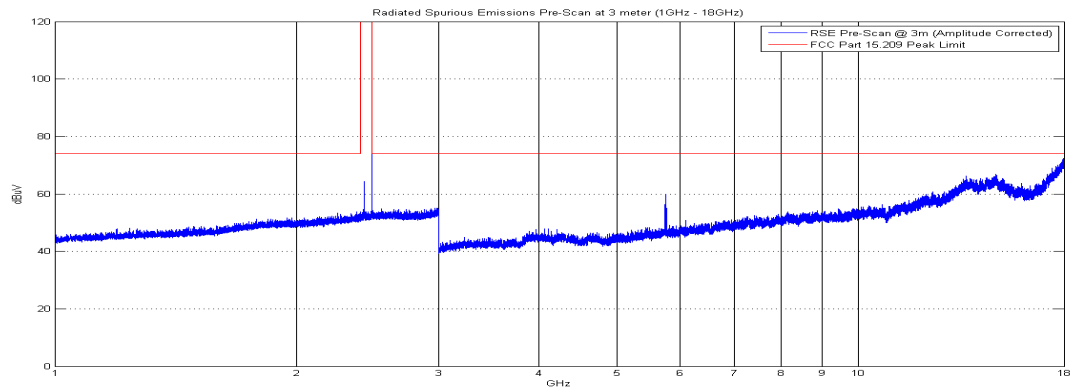
Plot 6-47. Radiated Spurious Plot above 1GHz (BT – Ch. 78, Ant. Pol. V)
