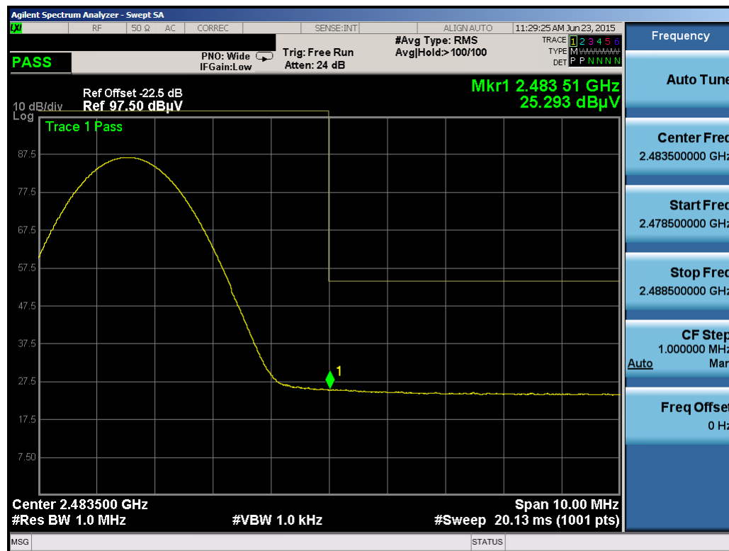
Plot 6-50. Radiated Restricted Upper Band Edge Measurement (Average)
