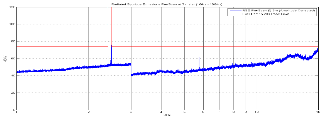
Plot 6-46. Radiated Spurious Plot above 1GHz (BT – Ch. 78, Ant. Pol. H)
