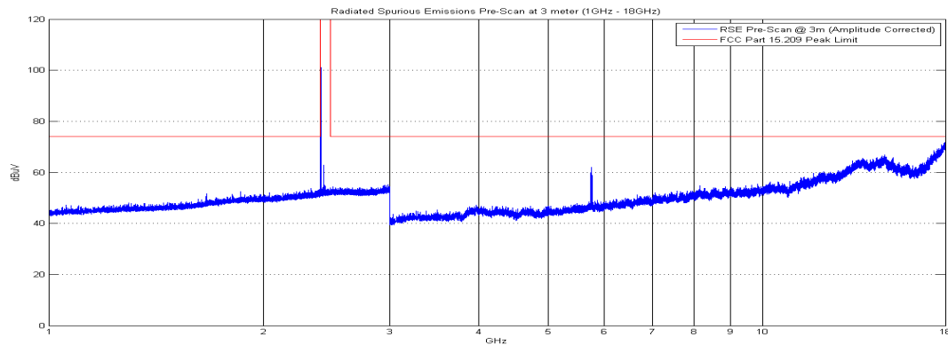
Plot 6-43. Radiated Spurious Plot above 1GHz (BT – Ch. 0, Ant. Pol. V)
