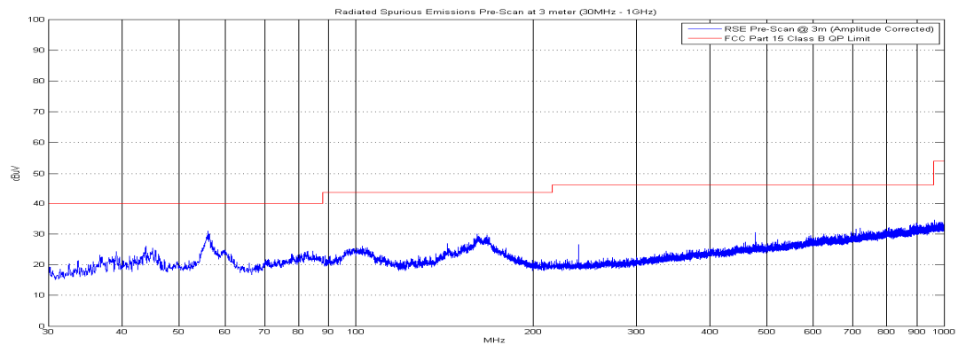
Plot 6-53. Radiated Spurious Plot below 1GHz (Pol. V)
