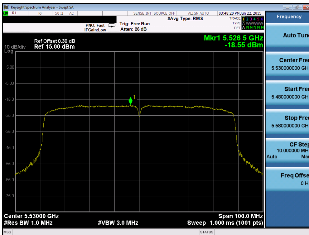
Plot 6-65. Power Spectral Density Plot (80MHz BW 802.11ac (UNII Band 2C) – Ch. 106)
